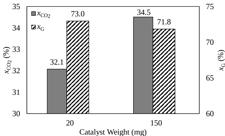
Figure 4.19. Effect of residence time on \text{CO}_2 and glycerol conversions of RuLZ ( T=750\text{ }^\circ\text{C} and \text{CO}_2/\text{G} = 3 ).
