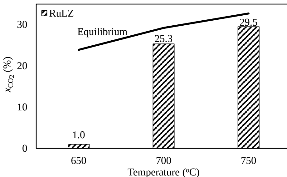
Figure 4.14. \text{CO}_2 conversions over RuLZ at reaction temperatures from 650 to 750 °C ( \text{CO}_2/\text{G} = 4 , and \tau = 0.5 \text{ mg min NmL}^{-1} ).
