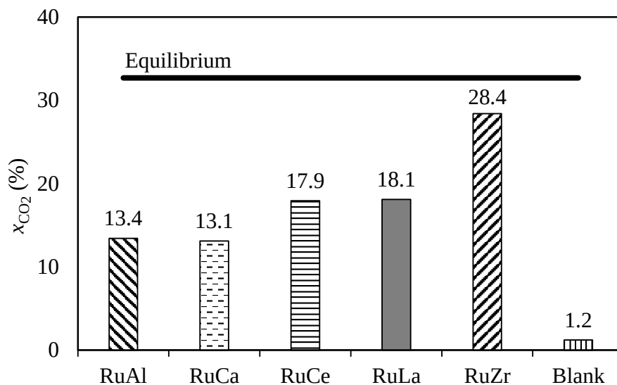
Figure 4.1. Carbon dioxide conversions over Ru supported on single oxide supports ( T=750 °C, \text{CO}_2/\text{G} = 4 , and \tau = 3.75 mg min \text{NmL}^{-1} ).
