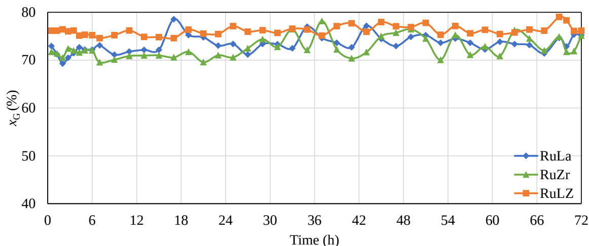
Figure 4.21. Glycerol conversions of RuLa, RuZr and RuLZ in stability experiments ( T=750\text{ }^{\circ}\text{C} , \text{CO}_2/\text{G} = 3 and \tau = 3.75\text{ mg min NmL}^{-1} ).
