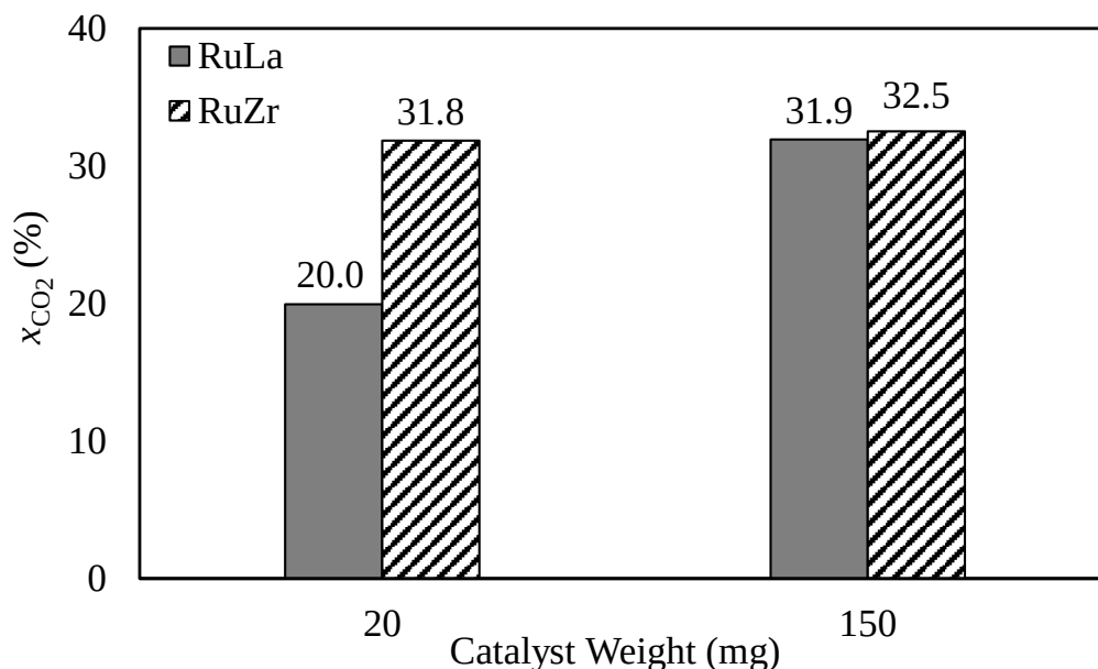
Figure 4.9. Effect of residence time on \text{CO}_2 conversions ( T = 750\text{ }^\circ\text{C} , \text{CO}_2/\text{G} = 3 ).
