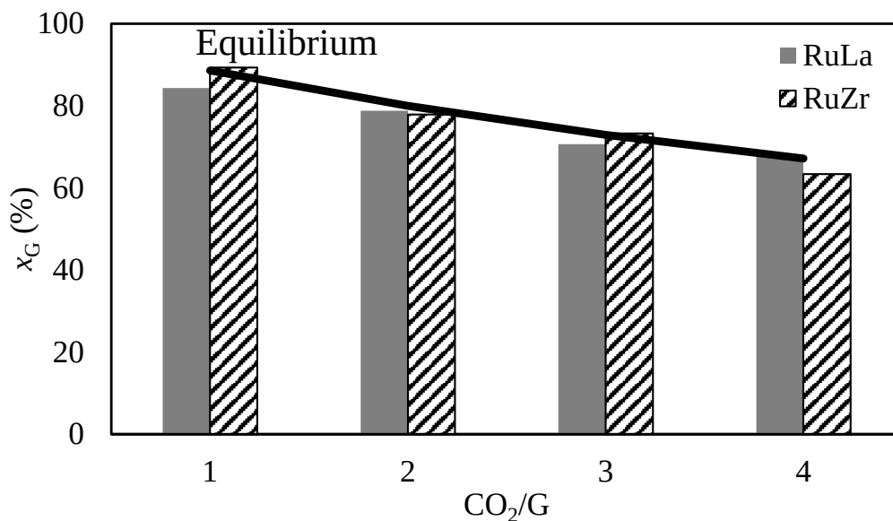
Figure 4.6. Glycerol conversions of RuLa and RuZr over \text{CO}_2/\text{G} ( T=750 °C).
