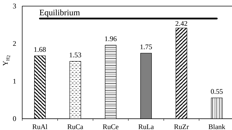
Figure 4.3. H_2 yields over single oxide supported catalysts in screening experiments ( T=750\text{ }^{\circ}\text{C} , CO_2/G = 4 , and \tau = 3.75\text{ mg min NmL}^{-1} ).
