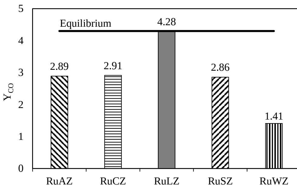
Figure 4.13. CO yields over binary oxide supported catalysts in screening experiments ( T=750\text{ }^{\circ}\text{C} , \text{CO}_2/\text{G} = 4 , and \tau = 3.75\text{ mg min NmL}^{-1} ).
