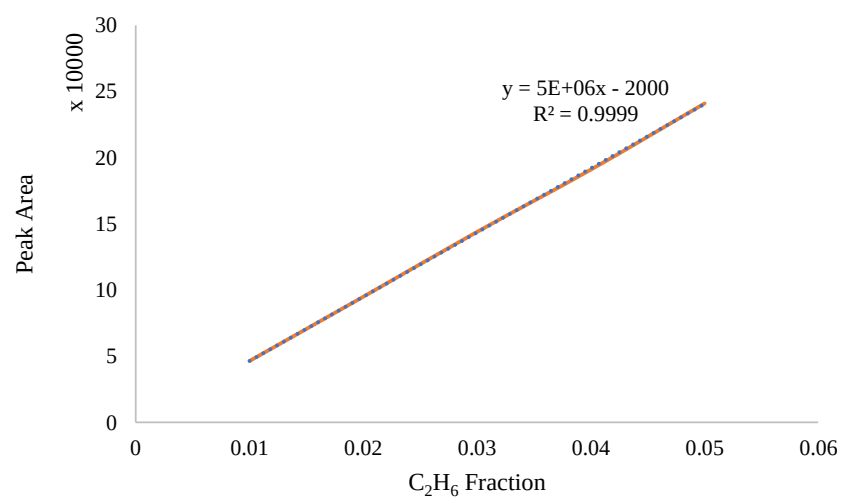
Figure B.8. C_2H_6 calibration curve of GC-2.
