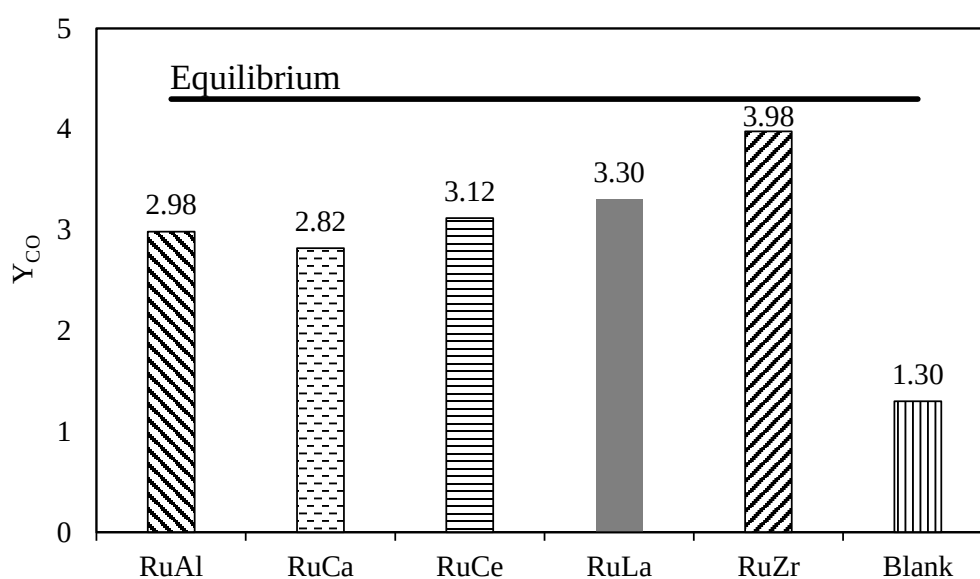
Figure 4.4. CO yields over single oxide supported catalysts in screening experiments ( T=750\text{ }^{\circ}\text{C} , CO_2/G = 4 , and \tau = 3.75\text{ mg min NmL}^{-1} ).
