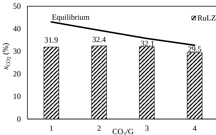
Figure 4.16. Carbon dioxide conversions over RuLZ at different \text{CO}_2 to glycerol ratios ( T=750\text{ }^\circ\text{C} , and \tau = 0.5\text{ mg min NmL}^{-1} ).
