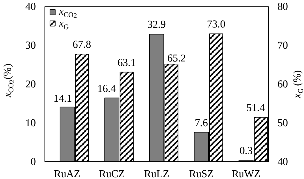
Figure 4.11. CO 2 and glycerol conversions over Ru supported on binary-oxide supports ( T=750 °C, \text{CO}_2/\text{G} = 4 , and \tau = 3.75 mg min NmL -1 ).
