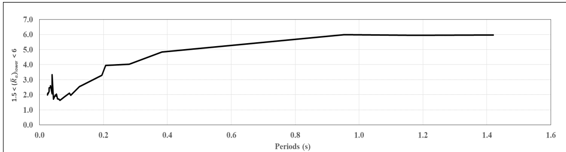
Figure 2.7. (\bar{R}_a)_{lower} obtained from each mode at Y-direction.
