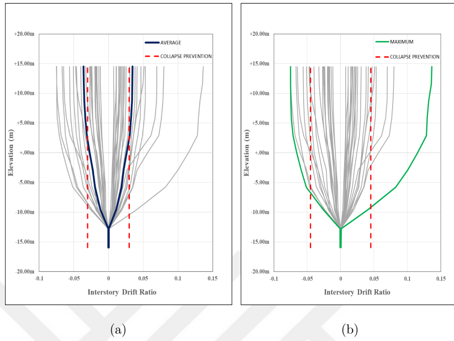
Figure A.7. Station 3 inter-story drift controls for H2 direction.
