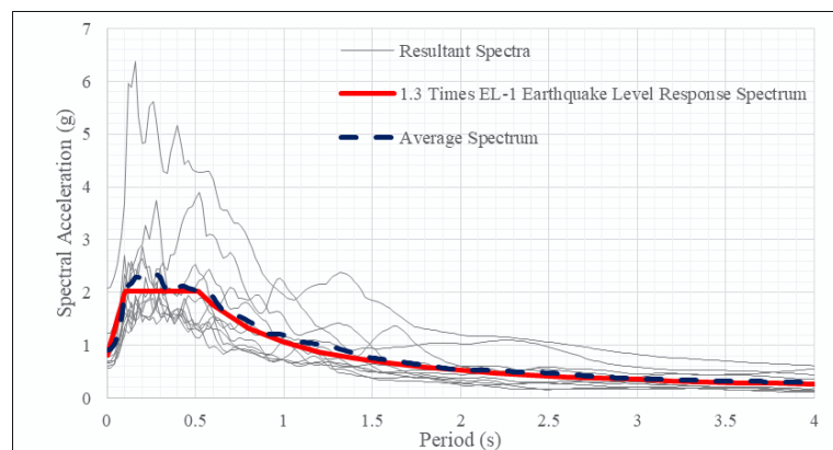
Figure 2.29. EL-1 Level SRSS acceleration spectra of selected ground motions.
