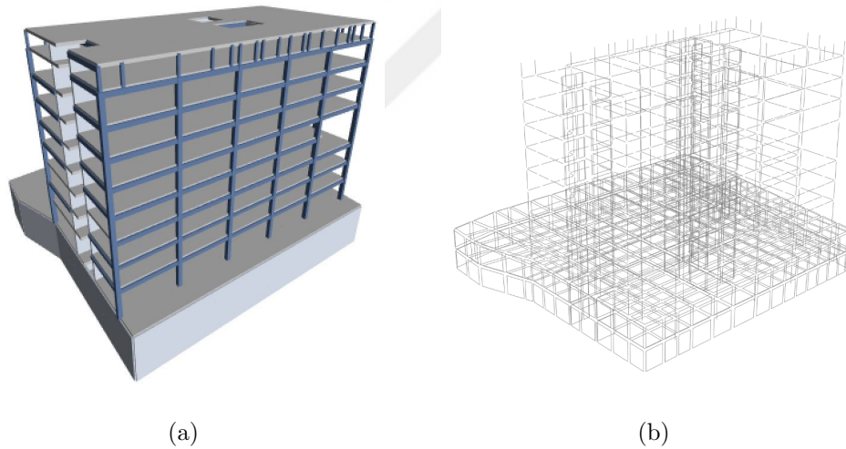
Figure 2.23. Etabs linear model (a), Perform 3D nonlinear model (b).
