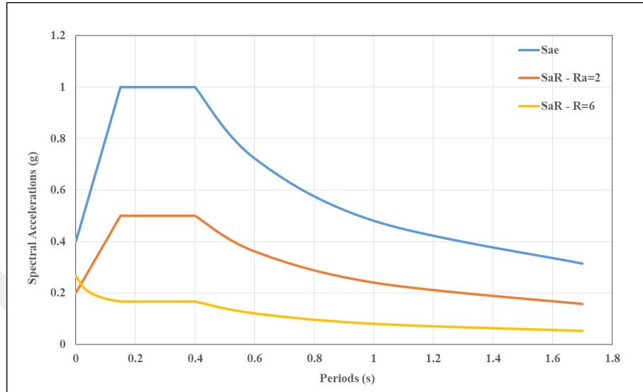
Figure 2.10. Response spectra based on TEC 2007.
