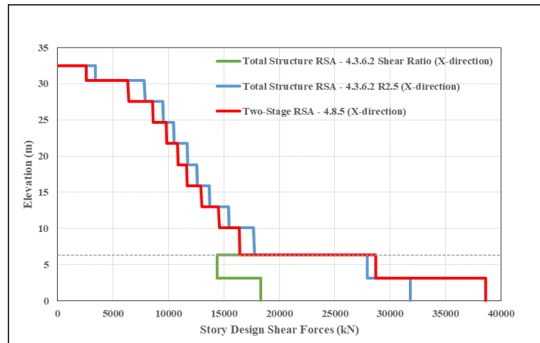
Figure 3.6. Comparison of RSA methods (4.8.5 and 4.3.6.2) based on TBSC 2018 in X-direction.
