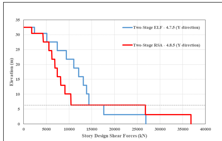
Figure 3.3. Comparison of TBSC 2018 two-stage methods (4.8.5 and 4.7.5) in Y-direction.
