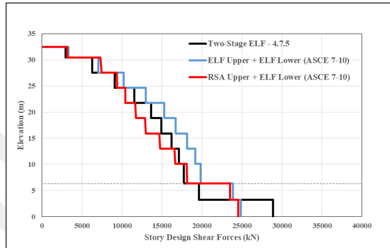
Figure 3.12. Comparison of story design shear forces based on ASCE 7-10 methods in X-direction.
