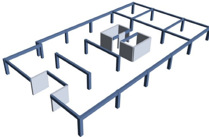
Figure 2.25. Sample superstructure story.
