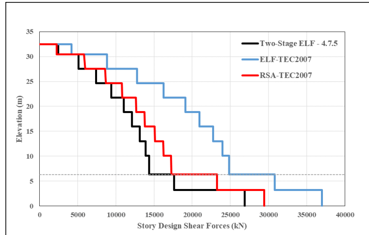
Figure 3.11. Comparison of story design shear forces based on TEC 2007 methodologies for Y-direction.
