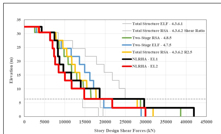
Figure 3.16. Comparison of linear and nonlinear results based on TBSC 2018 in X-direction.
