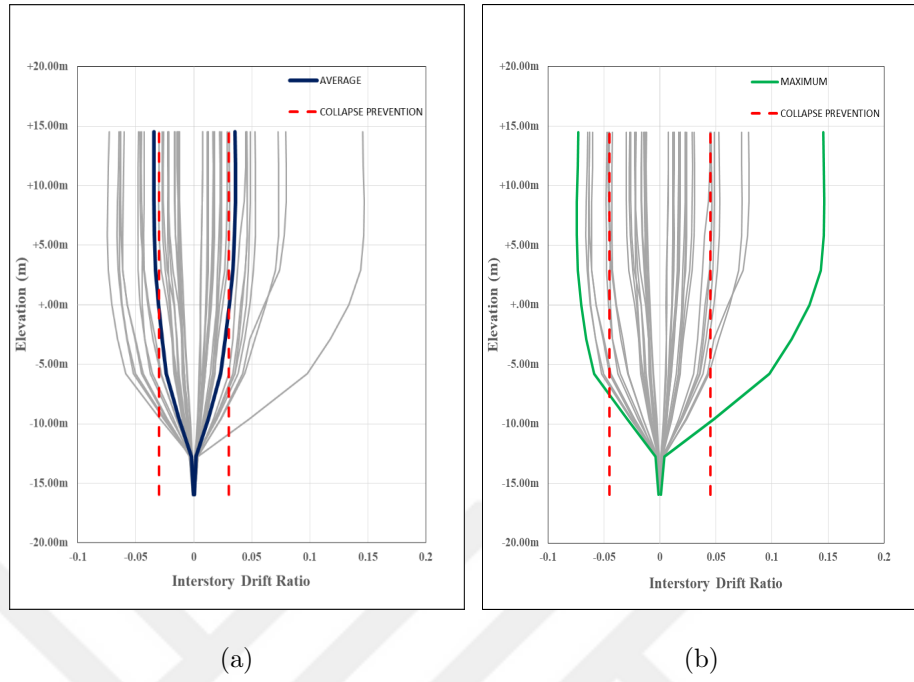
Figure A.3. Station 1 inter-story drift controls for H2 direction.
