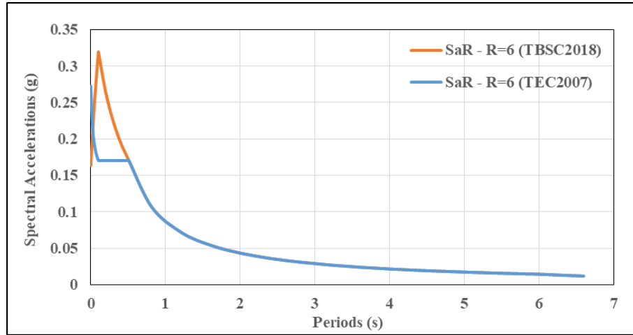
Figure 2.12. Comparison of reduced design spectra TBSC 2018 vs. TEC 2007 for the flexible superstructure.
