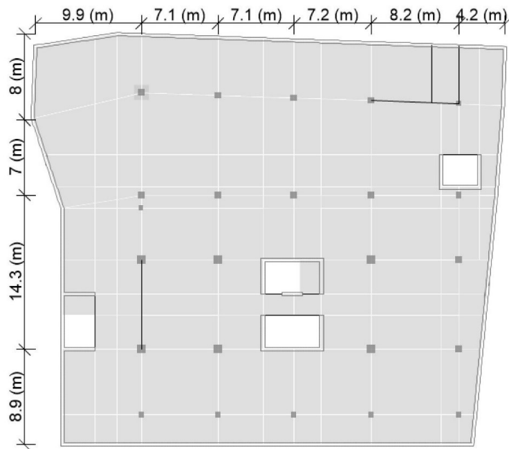
Figure 2.2. Typical basement plan view.
