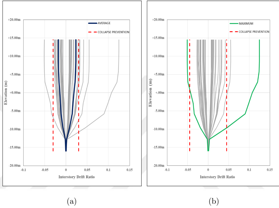
Figure A.2. Station 1 inter-story drift controls for H1 direction.
