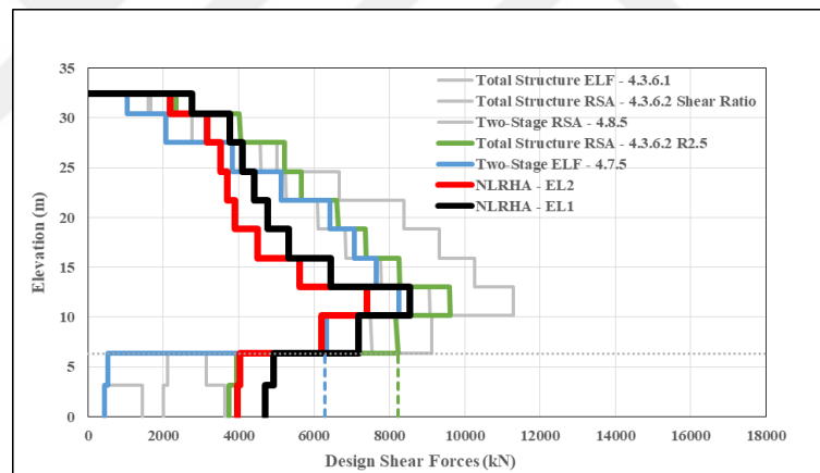
Figure 3.21. Comparison of design shear forces of PC02 in X-direction.
