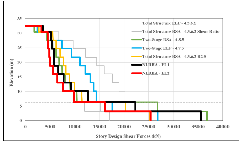
Figure 3.17. Comparison of linear and nonlinear results based on TBSC 2018 in Y-direction.
