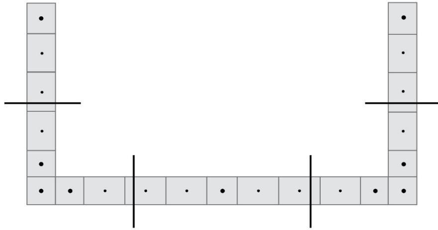
Figure 2.22. Fiber modeling of a structural wall in Perform3D.
