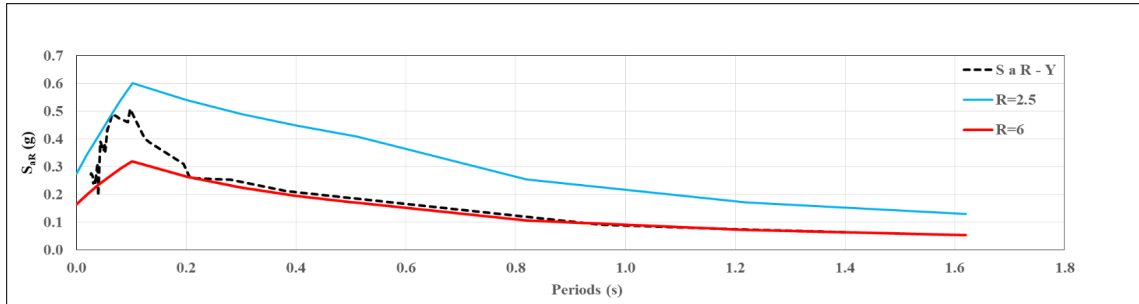
Figure 2.9. Reduced response spectrum based on 4.3.6.2 for Y-direction.
