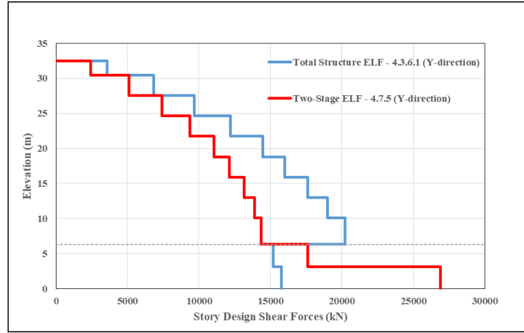
Figure 3.5. Comparison of ELF methods provided by TBSC 2018 in Y-direction.
