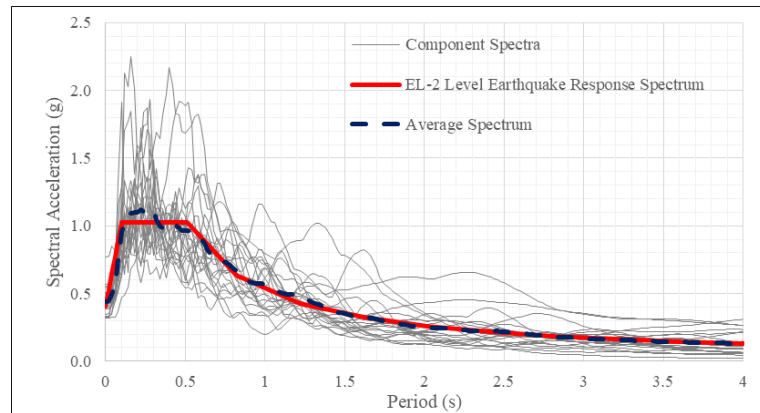
Figure 2.30. EL-2 level acceleration response spectra of selected ground motions.
