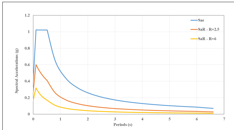
Figure 2.11. Response spectra based on TBSC 2018.
