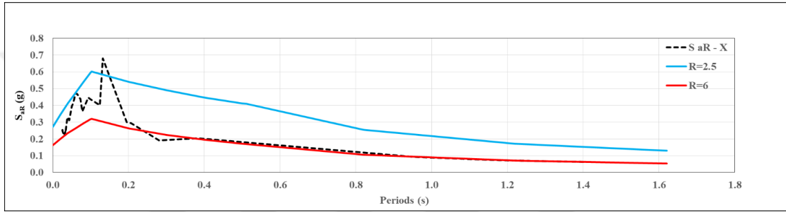
Figure 2.8. Reduced response spectrum based on 4.3.6.2 for X-direction.
