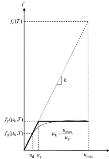
Figure 1.1. Stipulated Ductility Capacity – Strength Demand.
