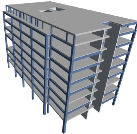
Figure 2.14. Upper portion fixed supported in transition.
