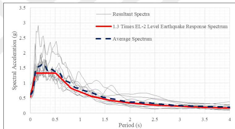
Figure 2.31. EL-2 Level SRSS acceleration spectra of selected ground motions.
