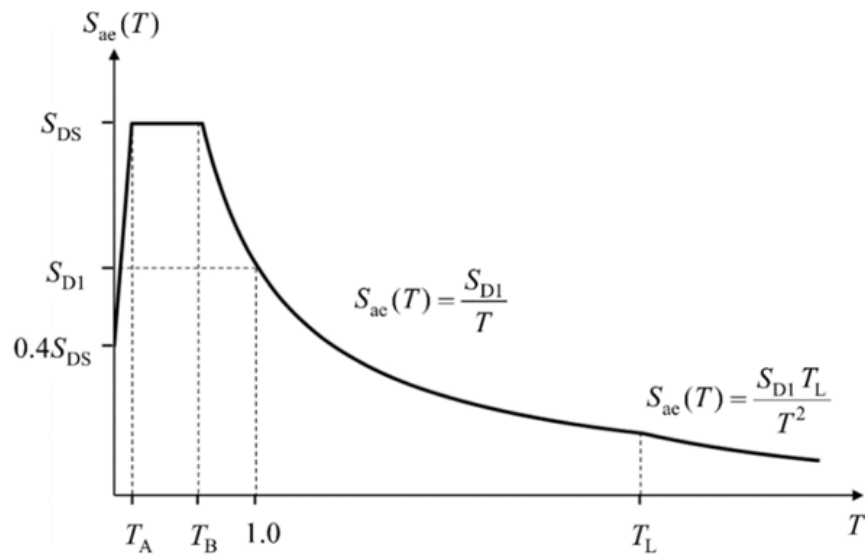
Figure 2.5. Horizontal elastic spectrum based on TBSC 2018.
