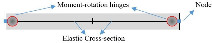
Figure 2.20. Modeling of beams using moment rotation hinges.
