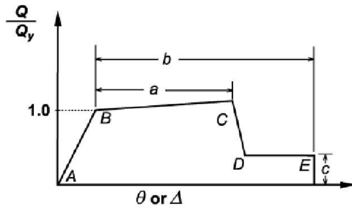
Figure 2.19. Backbone curve for nonlinear modeling.
