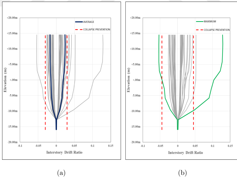
Figure A.6. Station 3 inter-story drift controls for H1 direction.
