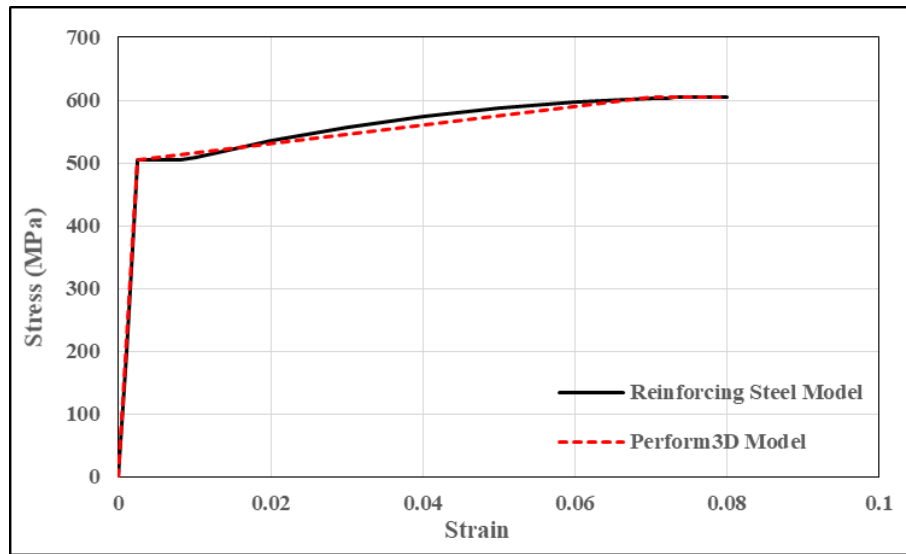
Figure 2.17. Reinforcing steel stress-strain relationship.
