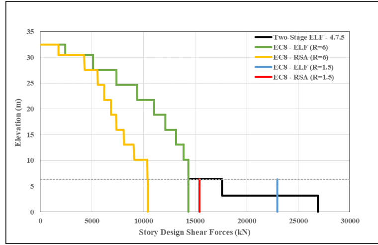
Figure 3.15. Comparison of Eurocode 8 approaches in Y-direction.
