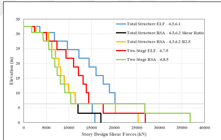
Figure 3.9. Comparison of all methods based on TBSC 2018 methodologies for Y-direction.
