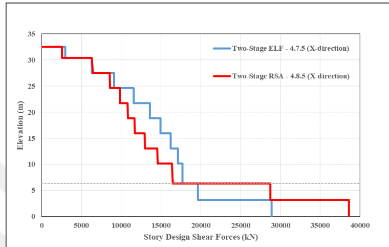
Figure 3.2. Comparison of TBSC 2018 two-stage methods (4.8.5 and 4.7.5) in X-direction.
