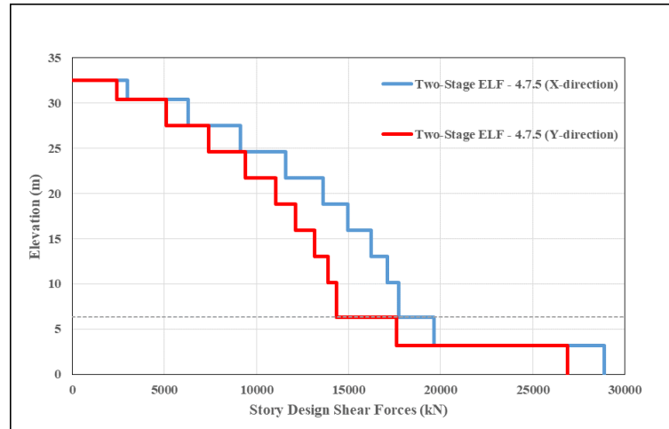
Figure 3.1. Story Forces Based on 4.7.5 Method for X and Y directions.
