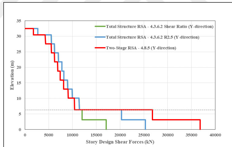
Figure 3.7. Comparison of RSA methods (4.8.5 and 4.3.6.2) based on TBSC 2018 in Y-direction.
