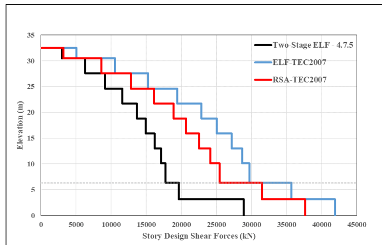
Figure 3.10. Comparison of story design shear forces based on TEC 2007 methodologies for X-direction.
