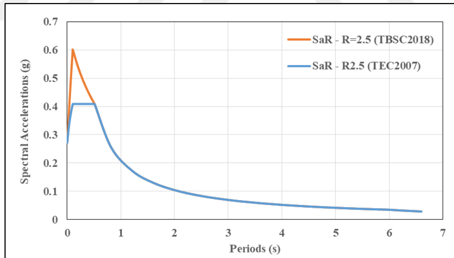
Figure 2.13. Comparison of reduced design spectra TBSC 2018 vs. TEC 2007 for rigid basement.
