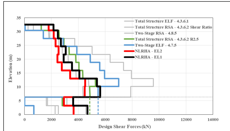
Figure 3.22. Comparison of design shear forces of PC02 in Y-direction.
