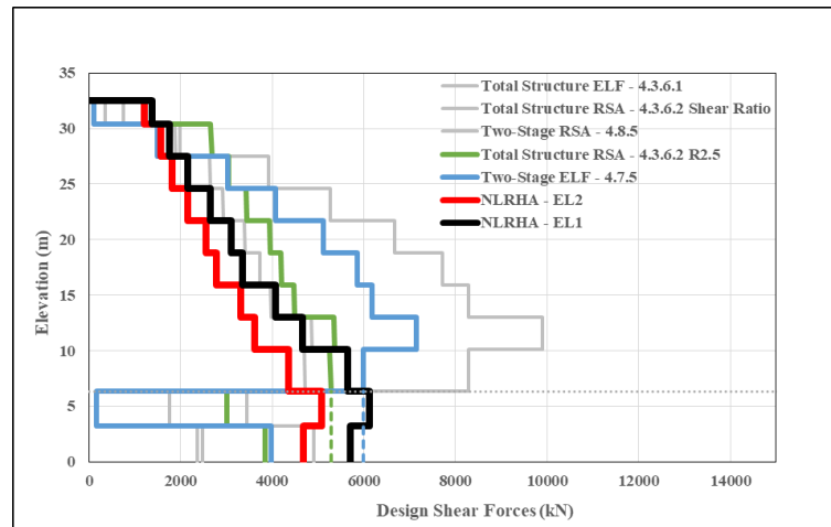
Figure 3.20. Comparison of design shear forces of PC01 in Y-direction.
