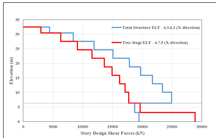
Figure 3.4. Comparison of ELF methods provided by TBSC 2018 in X-direction.
