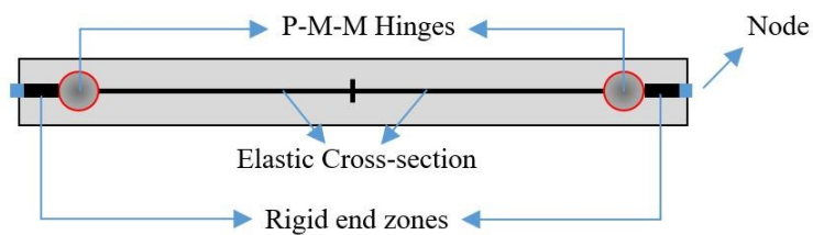
Figure 2.18. Modeling of columns using PMM hinges.
