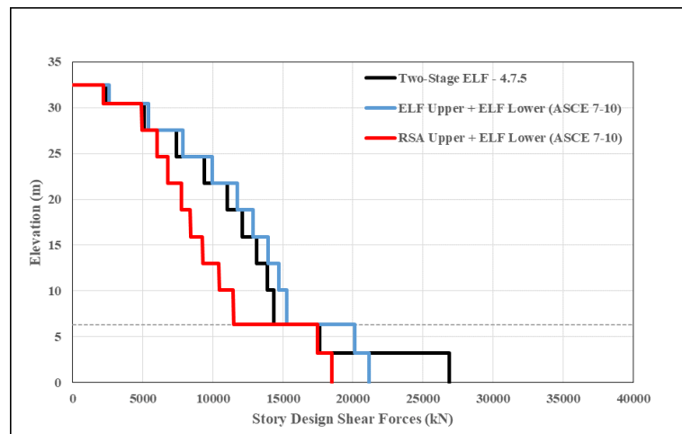
Figure 3.13. Comparison of story design shear forces based on ASCE 7-10 methods in Y-direction.
