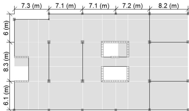
Figure 2.3. Typical superstructure plan view.
