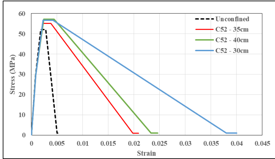
Figure 2.16. Linearized stress-strain relationship of concrete material.
