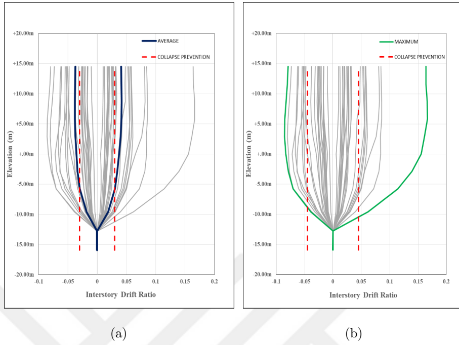
Figure A.5. Station 2 inter-story drift controls for H2 direction.
