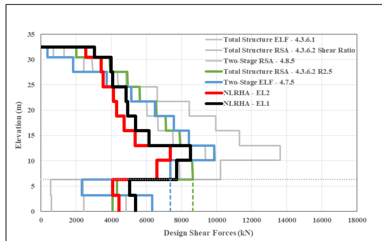
Figure 3.19. Comparison of design shear forces of PC01 in X-direction.
