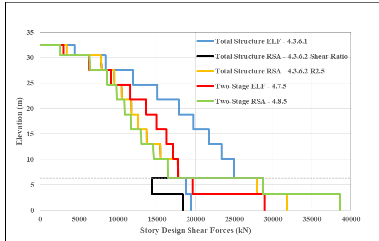
Figure 3.8. Comparison of all methods based on TBSC 2018 methodologies for X-direction.
