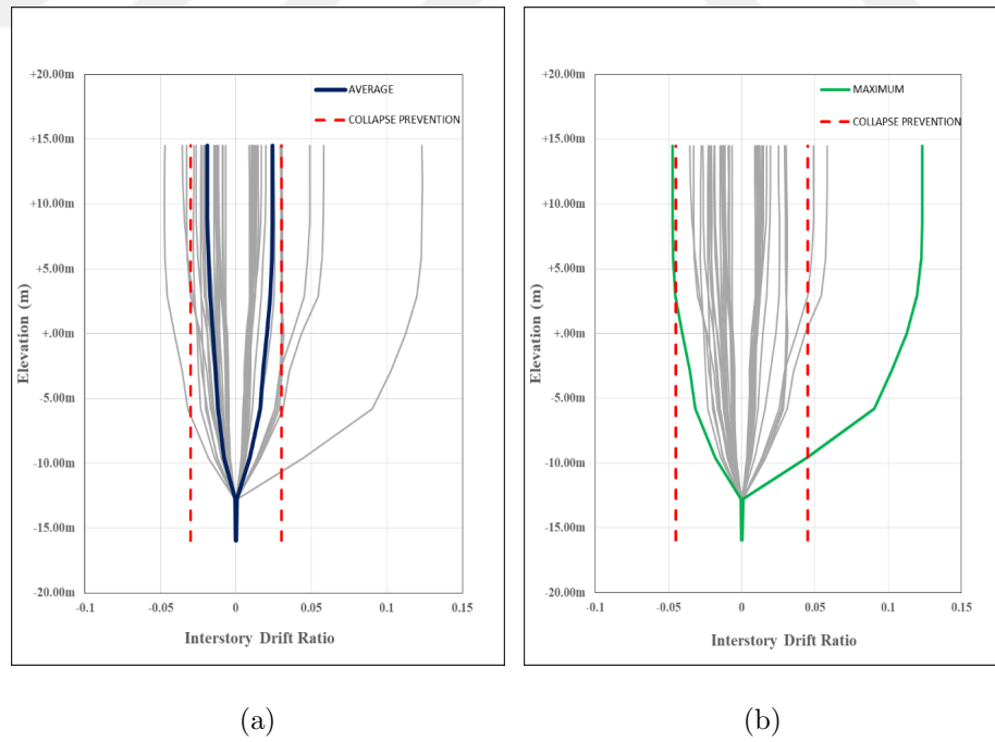
Figure A.4. Station 2 inter-story drift controls for H1 direction.
