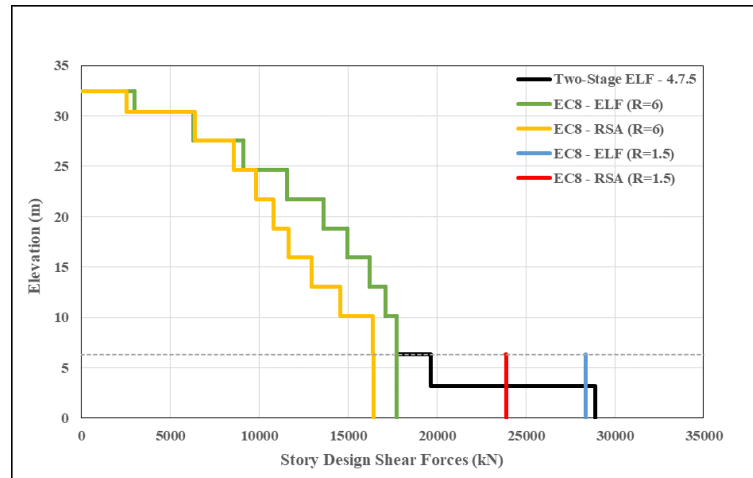
Figure 3.14. Comparison of Eurocode 8 approaches in X-direction.
