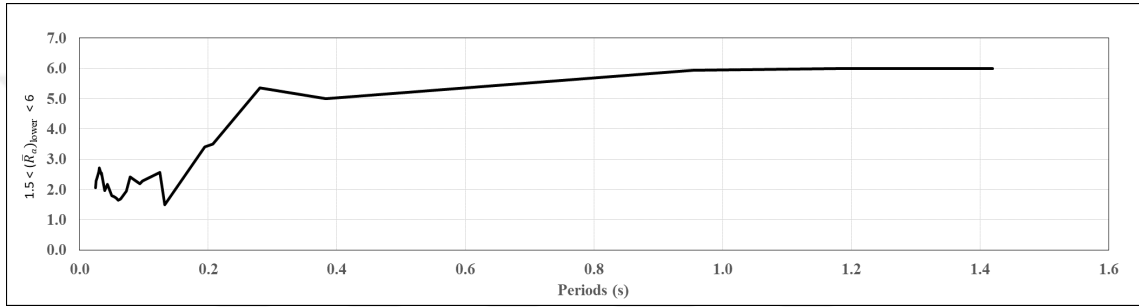
Figure 2.6. (\bar{R}_a)_{lower} obtained from each mode at X-direction.
