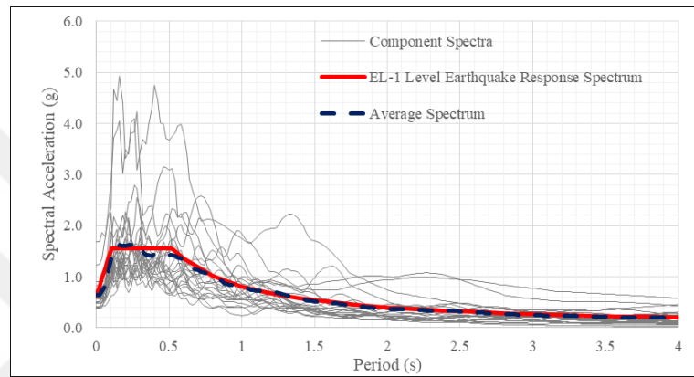
Figure 2.28. EL-1 level acceleration response spectra of selected ground motions.
