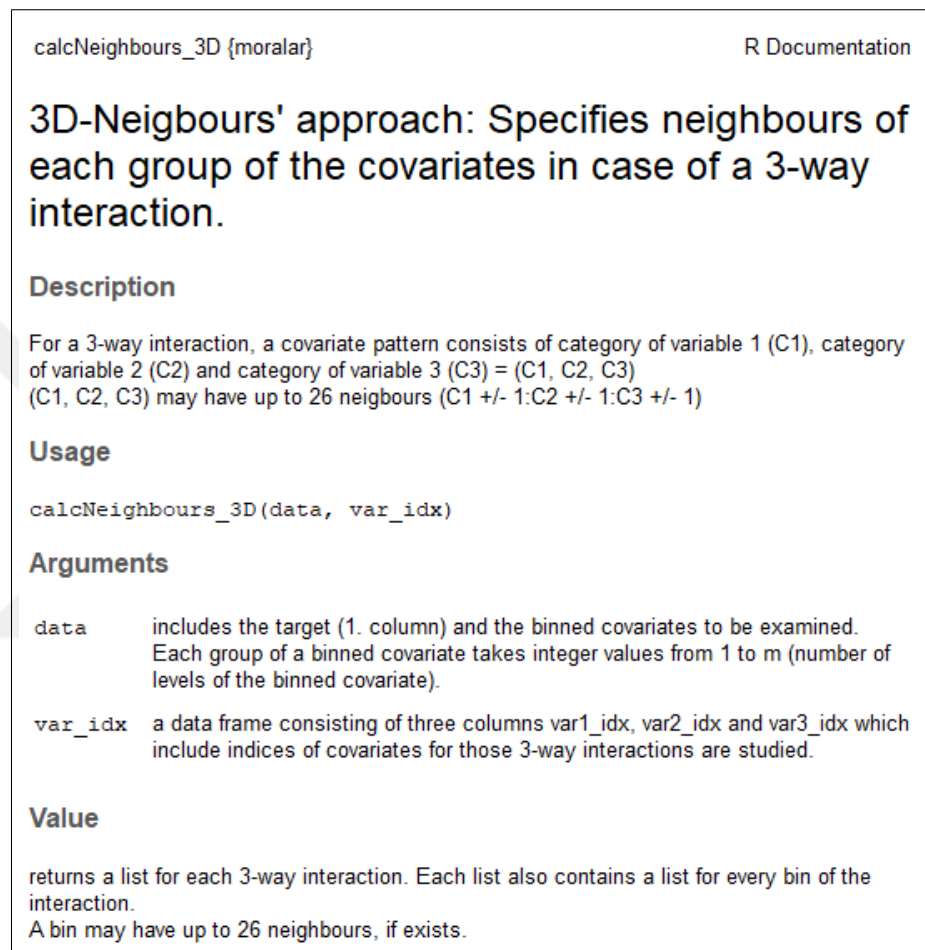
Figure 8.41. Screenshot from the R documentation of calcNeighbours_3D() function.
