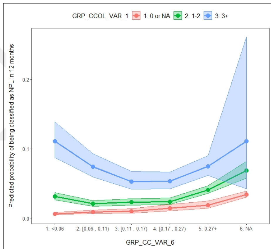
Figure 8.4. Plot of marginal effects, when GRP_CC_VAR_6 and GRP_CC_COL_VAR_1 are NPL_IN_12M predictors.
