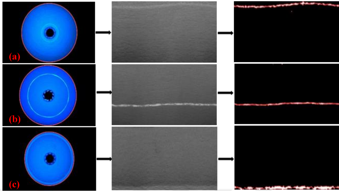
Figure 4.6 Algorithm results prepared by Local Thresholding method (a) abrade at the beginning of the bobbin (b) abrade in the middle of the bobbin (c) abrade at the end of the bobbin
