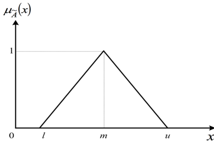
Figure 4.2. Triangular Fuzzy Number Graph
