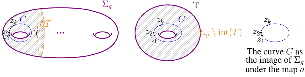
Figure 3.5: The map a : \Sigma_g \rightarrow C
