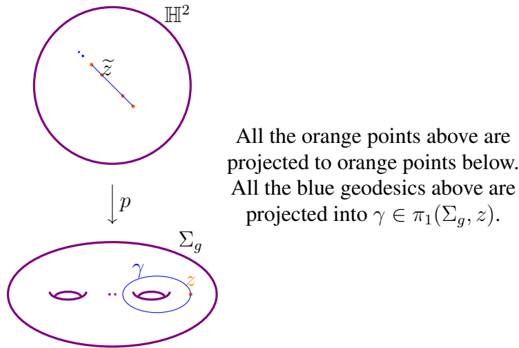
Figure 3.2: \mathbb{H}^2 as the universal cover of \Sigma_g
