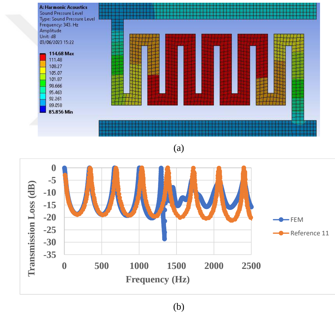
Figure 3.2. (a) Sound pressure level at the first resonance frequency, (b) The resulting transmission loss graphs of the space-coiled channel with length 500 mm and width 7 mm via FEM, and reference article [11]. The width of the overall design domain is 129 mm.
