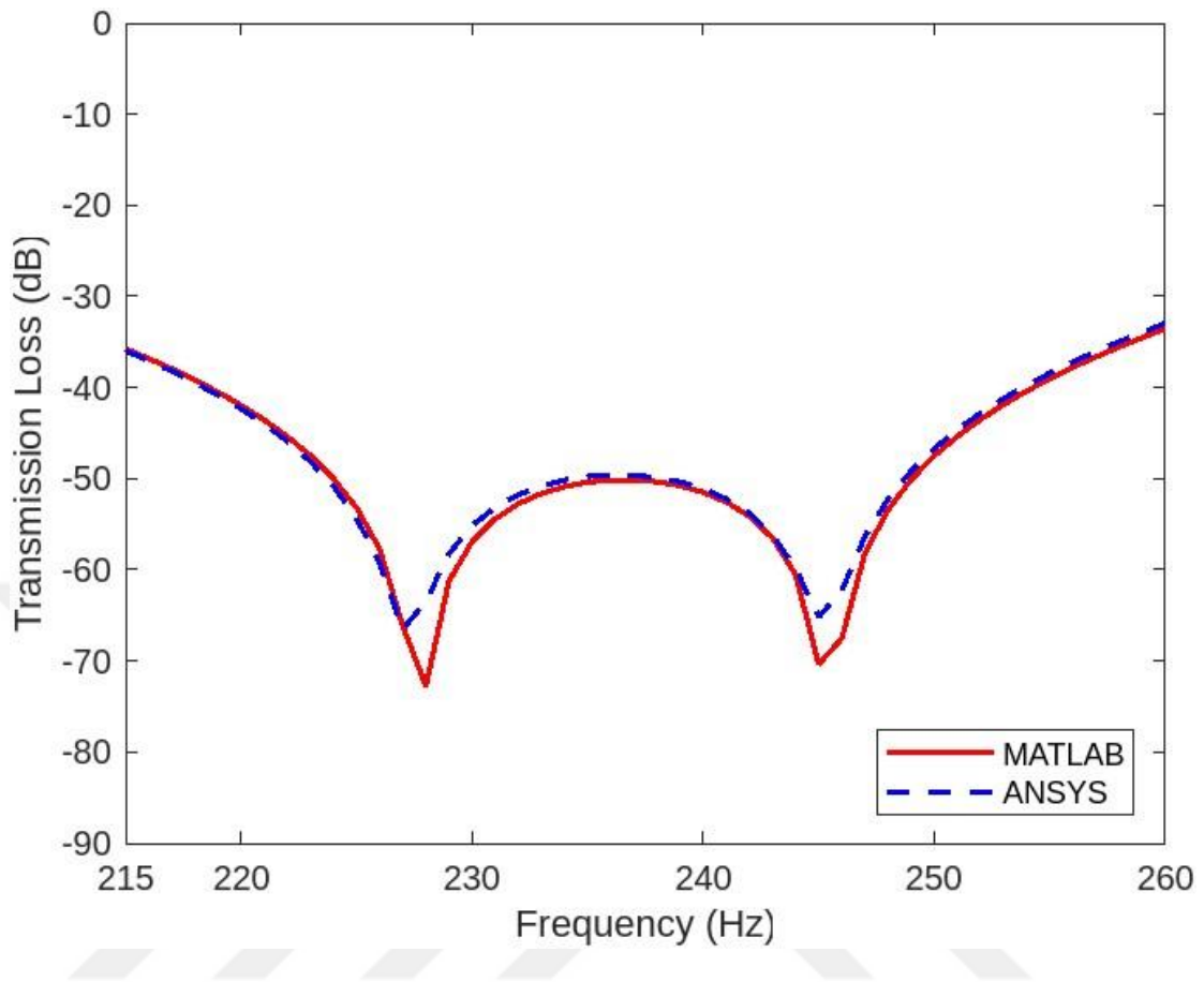
Figure 5.24. Transmission loss graphs of the design involving one straight channel and one space-coiled channel with rounded corners via MATLAB and ANSYS for 250 mm overall design domain width, 250 Hz upper frequency limit and 50 dB target transmission loss within the isolation bandwidth. Here, d_1 = 28 mm, d_2 = 27.68 mm.
