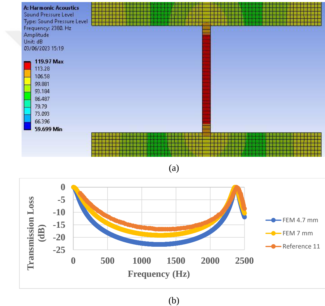
Figure 3.1. (a) Sound pressure level at the resonance frequency, (b) The resulting transmission loss graphs of the straight channel with length 60 mm for the widths of 4.7 mm and 7 mm via FEM, and reference article [11]. The width of the overall design domain is 129 mm.
