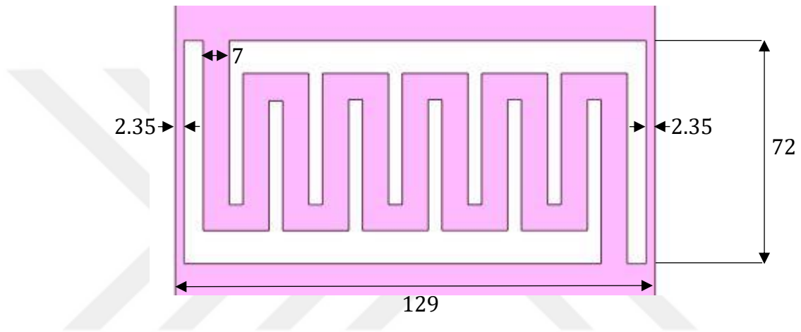
Figure 4.6. The design according to the given dimensions. The dimensions are in mm.
