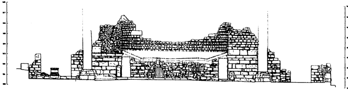
APHRODISIAS Temple of Aphrodisias, elevation with the temple of Apollo (1900) East Elevation of the temple of Aphrodisias 1900
