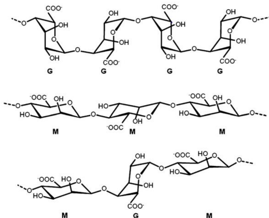
Figure 2.15. Alginate structure
