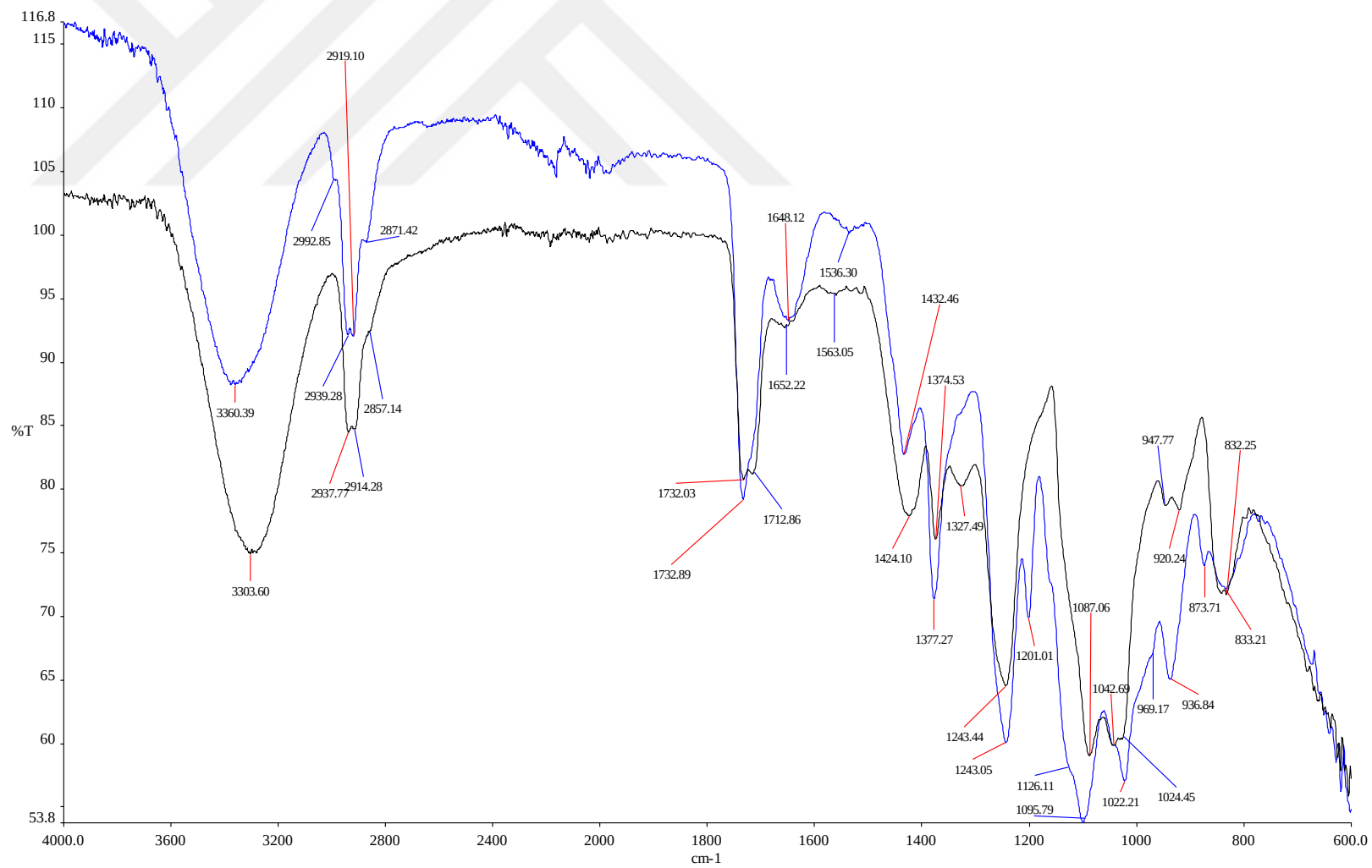
Figure 4.8. FTIR spectra of noncross-linked PAG-CSA hydrogel (black) and cross-linked PAG-CSA (blue) hydrogels
