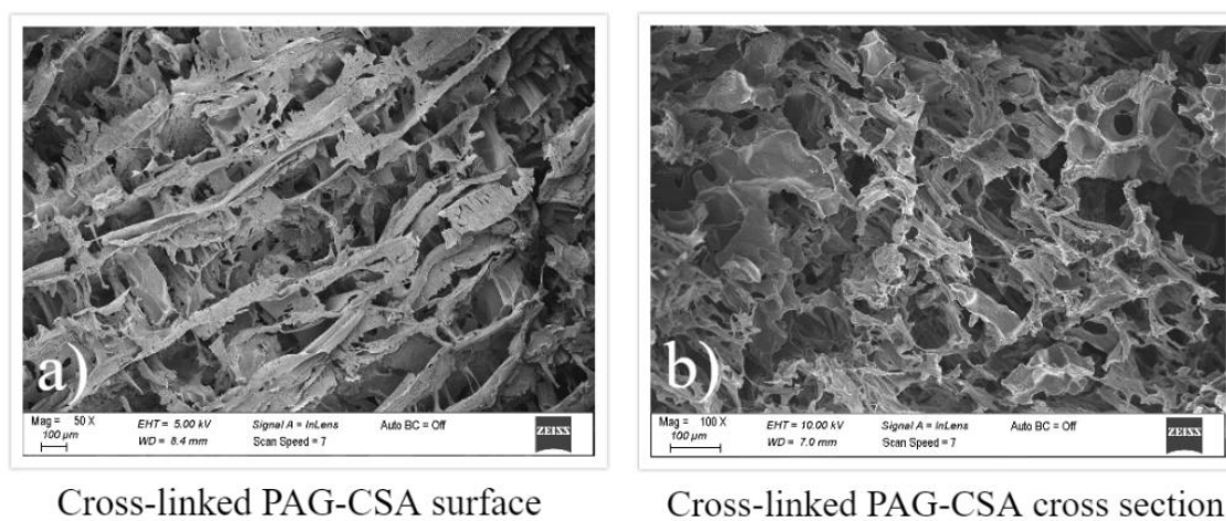
Figure 4.10. SEM images of cross-linked PAG-CSA hydrogel surface (a) and cross-linked PAG-CSA hydrogel cross section (b)
