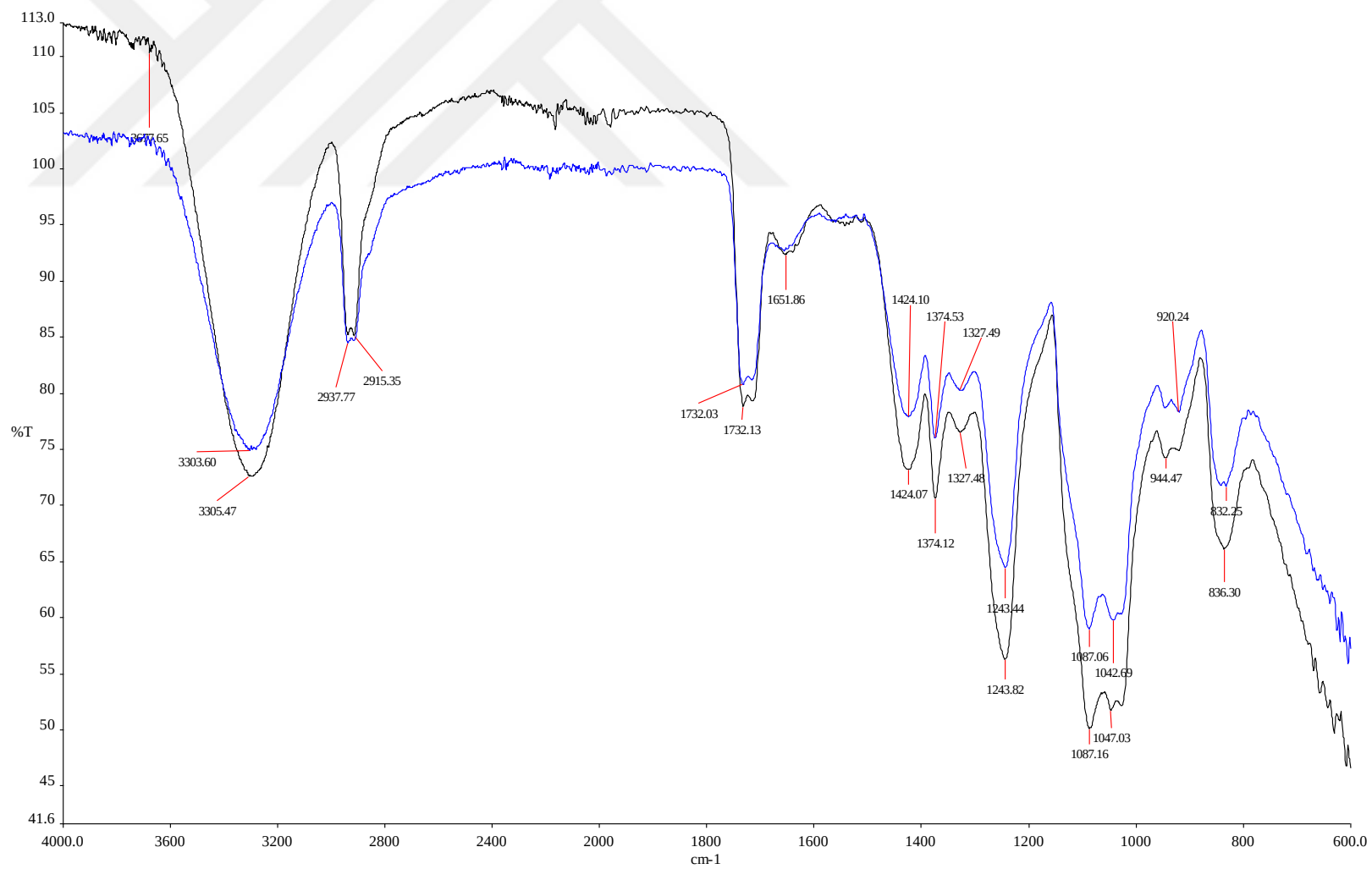
Figure 4.6. FTIR spectra of Noncross-linked PAG hydrogel (black) and noncross-linked PAG-CSA (blue) hydrogels.
