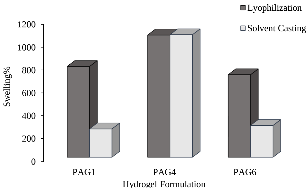
Figure 4.1. The swelling ratios of PAG hydrogels prepared via solvent casting and lyophilization methods (cross-linking time: 30 min)
