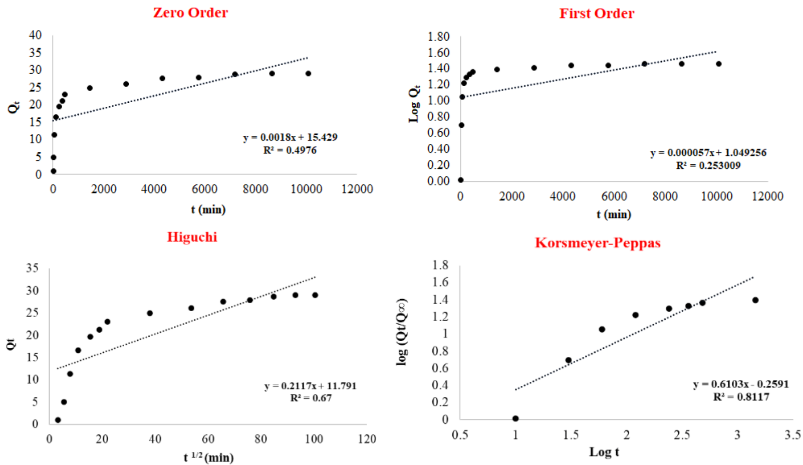
Figure 4.23. Graphs of release patterns of CSA-44 release from cross-linked PAG-CSA hydrogel
