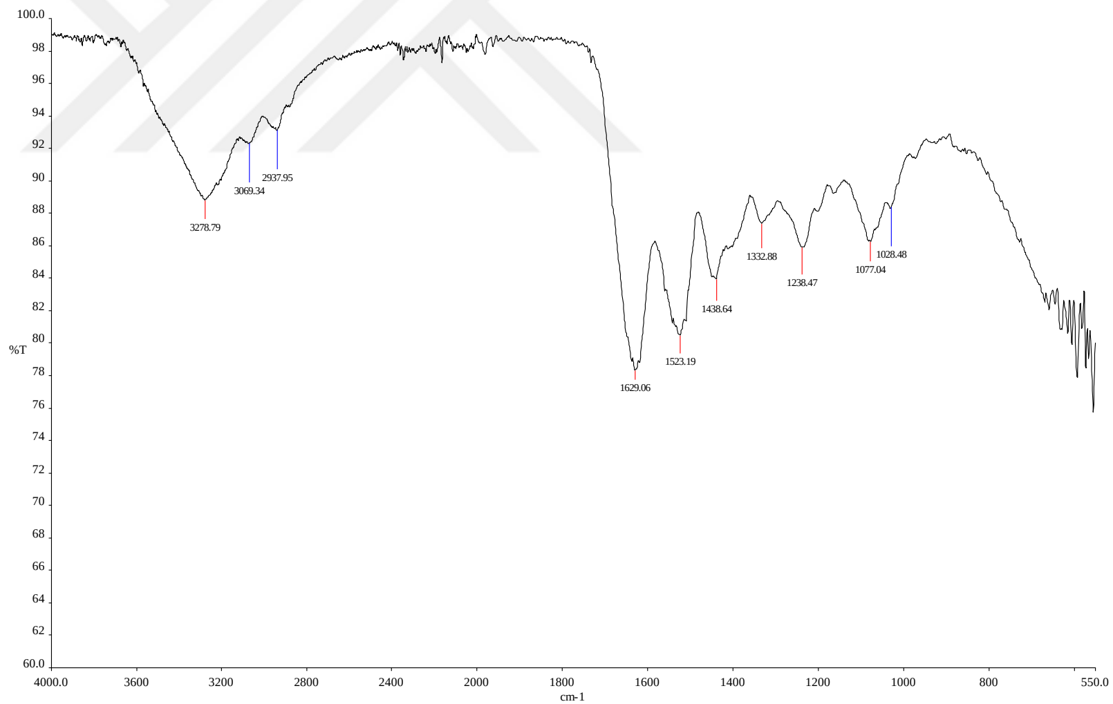
Figure 4.4. FTIR spectrum of gelatin
