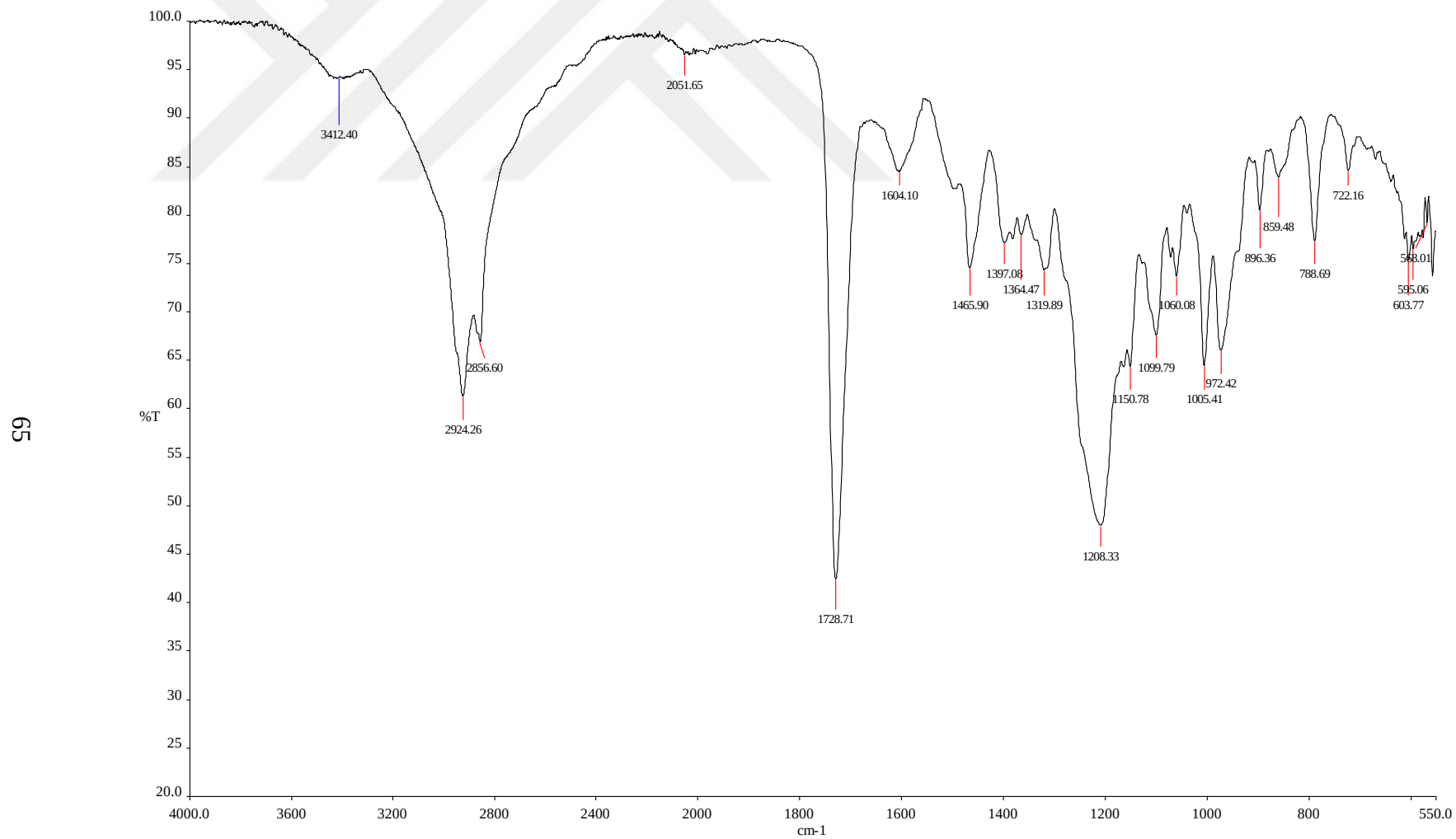
Figure 4.5. FTIR spectrum of CSA-44
