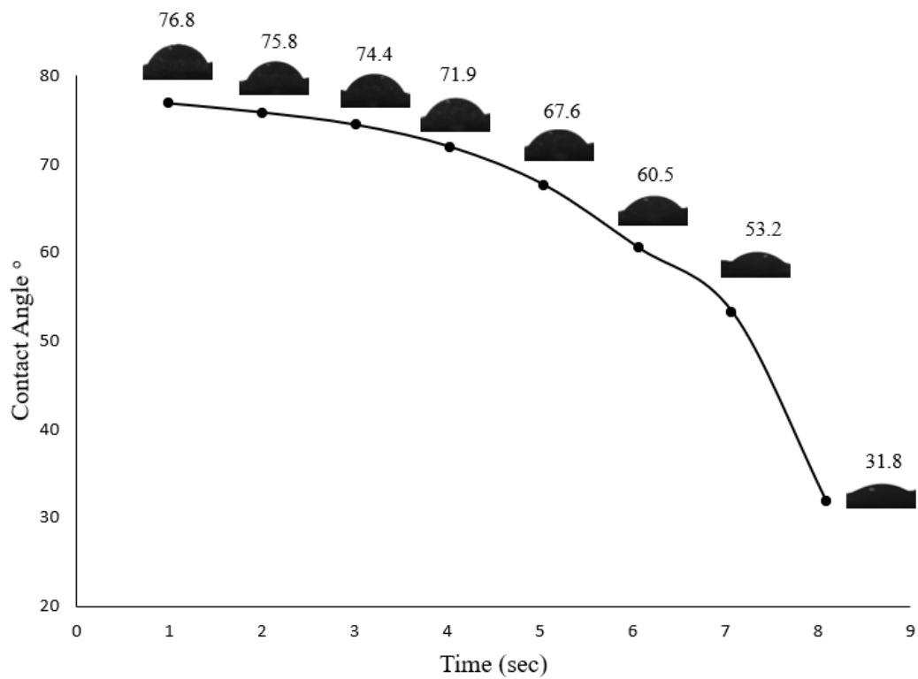
Figure 4.11. PAG-CSA the decrease of contact angle value within 8 seconds
