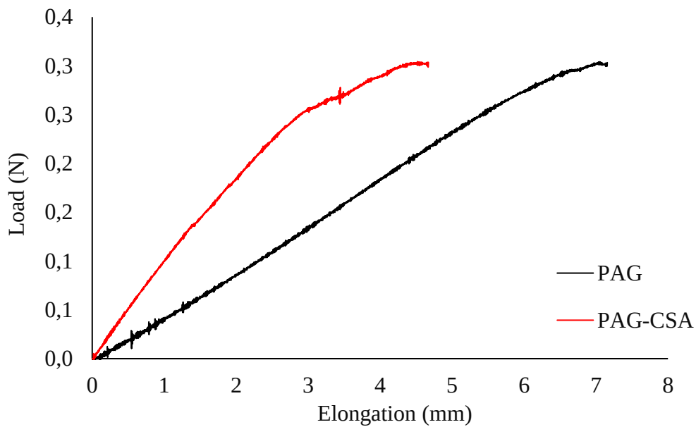
Figure 4.17. Elongation curve of PAG and PAG-CSA
