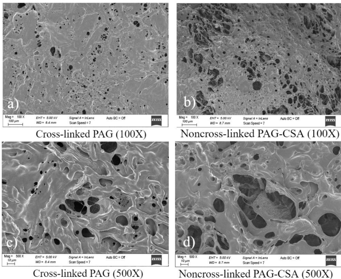
Figure 4.9. SEM images of cross-linked PAG (100X (a) & 500X (c)) and noncross-linked PAG-CSA (100X (b) & 500X (d)) hydrogels
