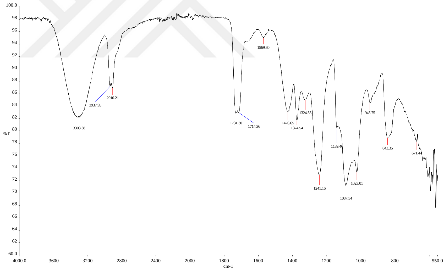
Figure 4.2. FTIR spectrum of PVA
