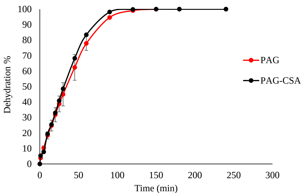
Figure 4.13. Dehydration (%) of PAG and PAG-CSA hydrogels
