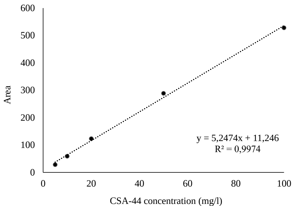
Figure 4.21. CSA-44 calibration graph
