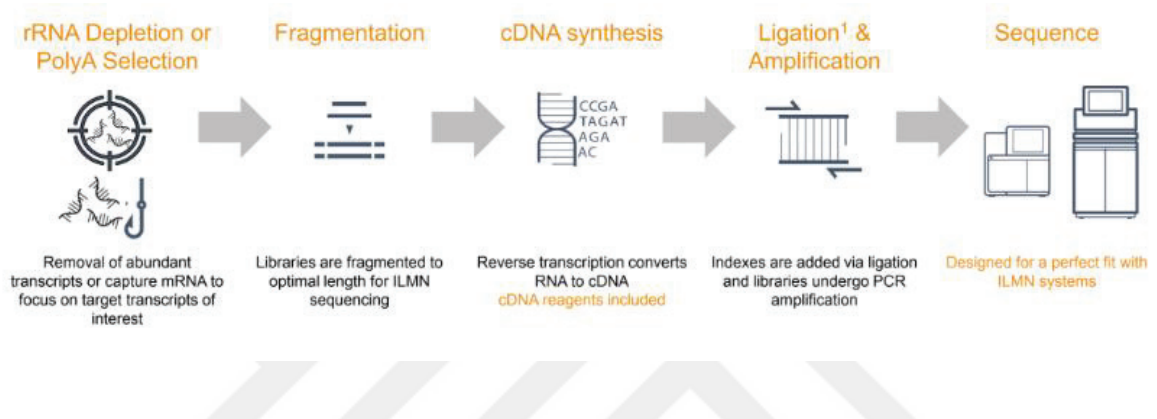
Figure 2.2. Schematic representation of the library preparation workflow (RefGEN Biotechnology, Turkey).
