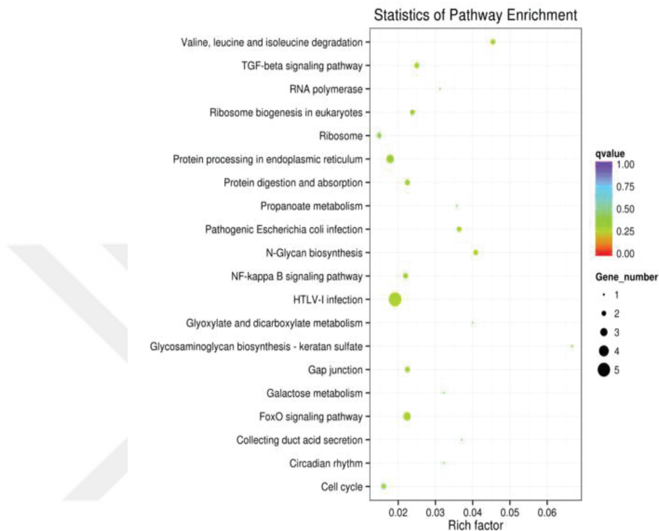
Figure 3.2. Gene ontology (GO) Pathway enrichment analysis.
