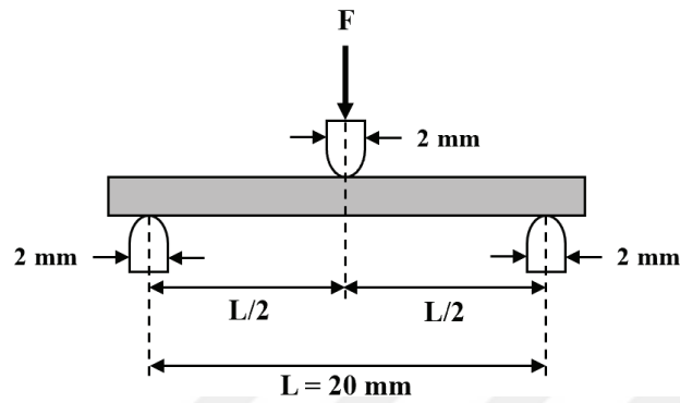
Figure 3.3 Schematic representation of the three-point bending test setup
