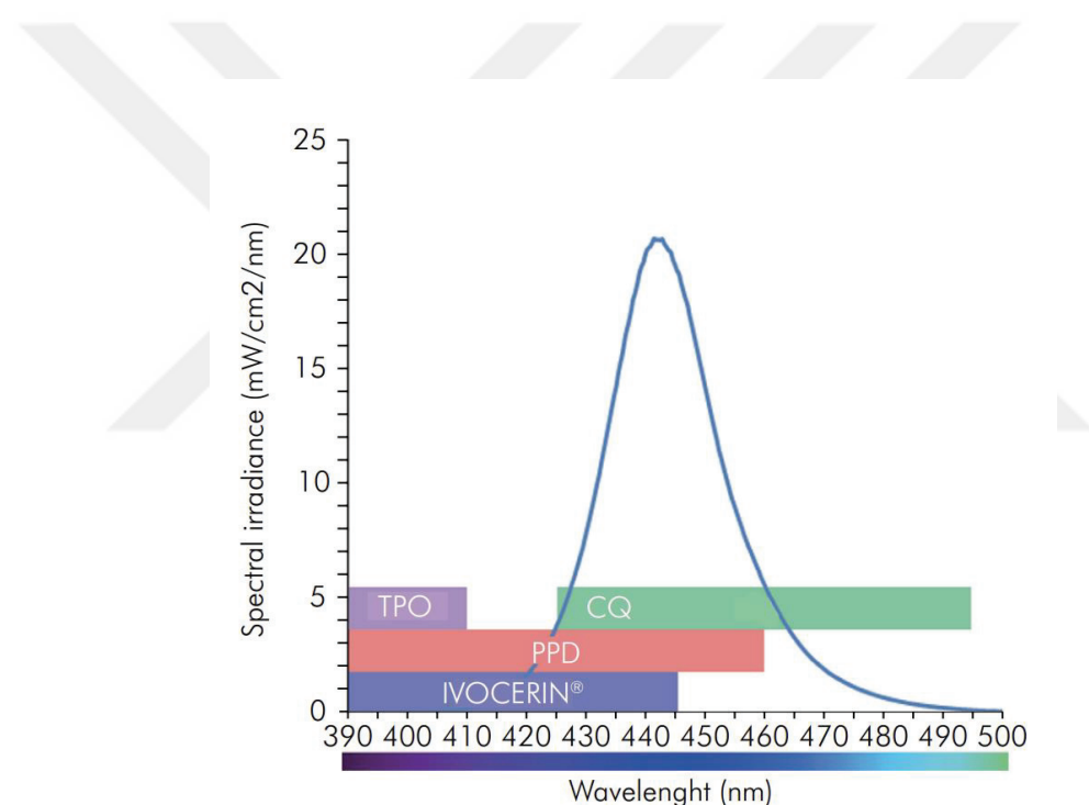
Figure 2.6 Absorption spectra of CQ, PPD, and TPO and emission spectrum of the blue LED (Source: Rueggeberg et al. 2017)
