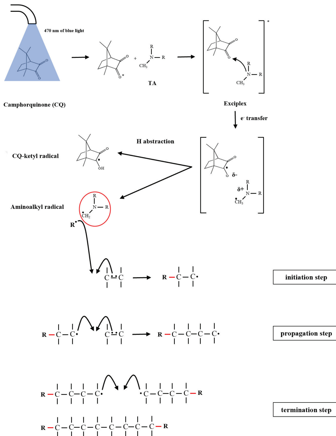
Figure 2.8 Photopolymerization of CQ (Source: Cosola et al. 2019)
