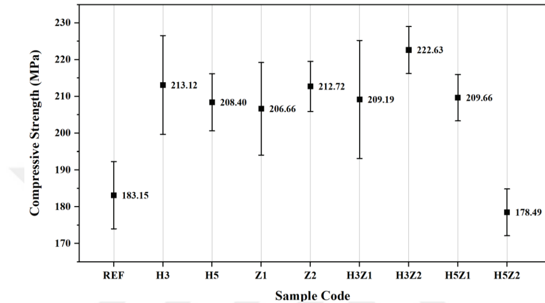
Figure 4.13 Compressive strength results of the dental composites with a standard deviation
