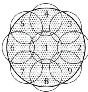
Figure 3.8 Top view of overlapping irradiation zones for the preparation of the water sorption specimens
