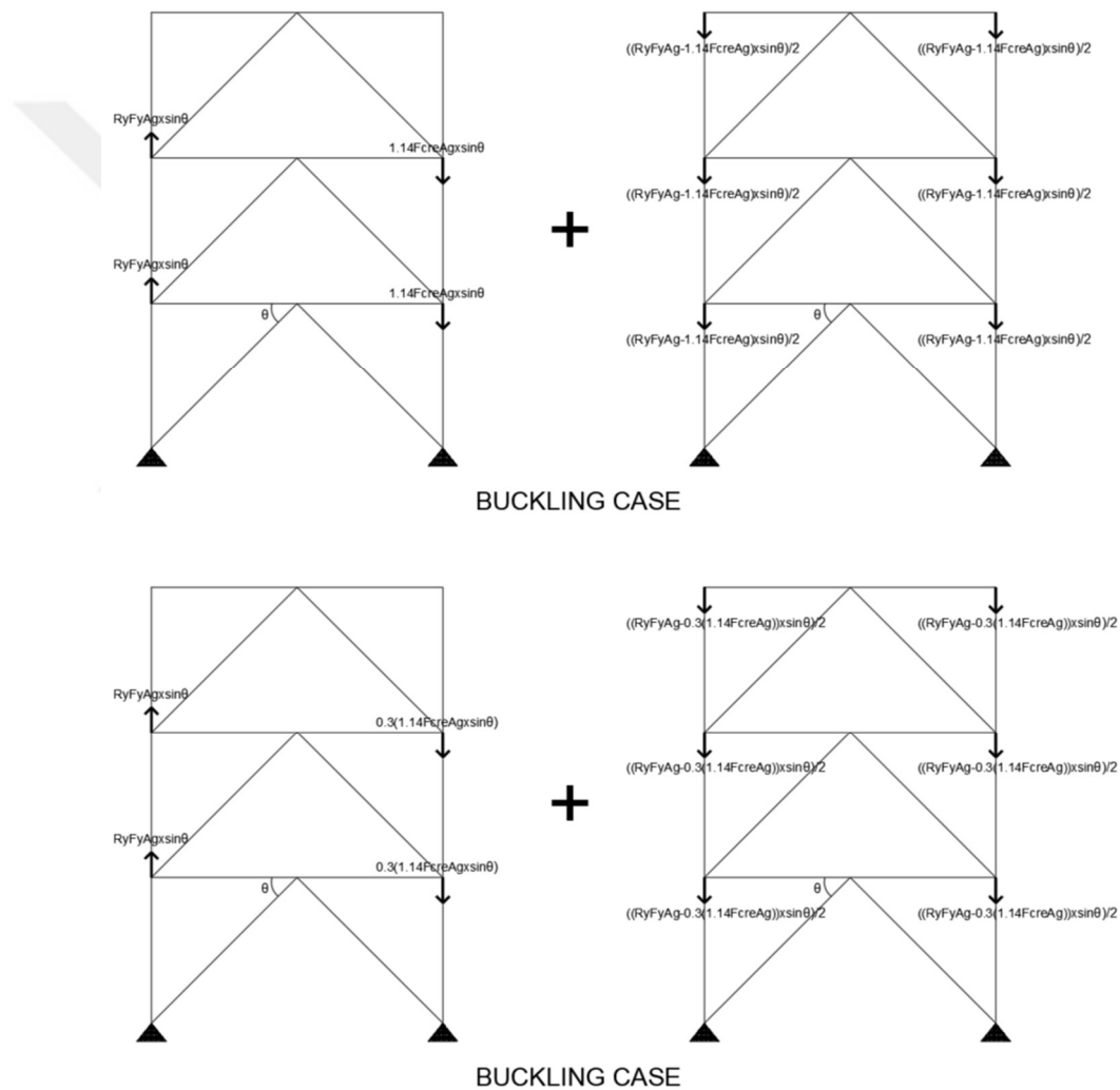
Figure 3.7. Acting forces on columns due to buckling and post-buckling mechanisms.
