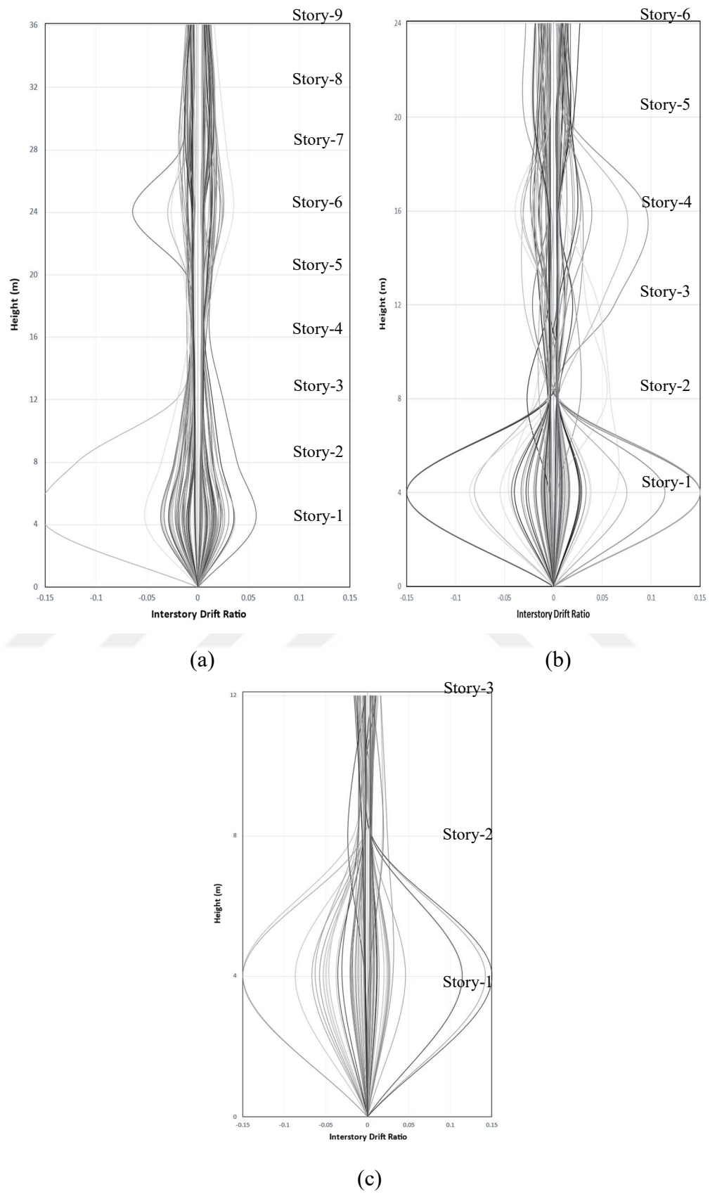
Figure 4.15. Intersory drift ratio distribution under MCE intensity for (a) building-3, (b) building-2, (c) building-1.
