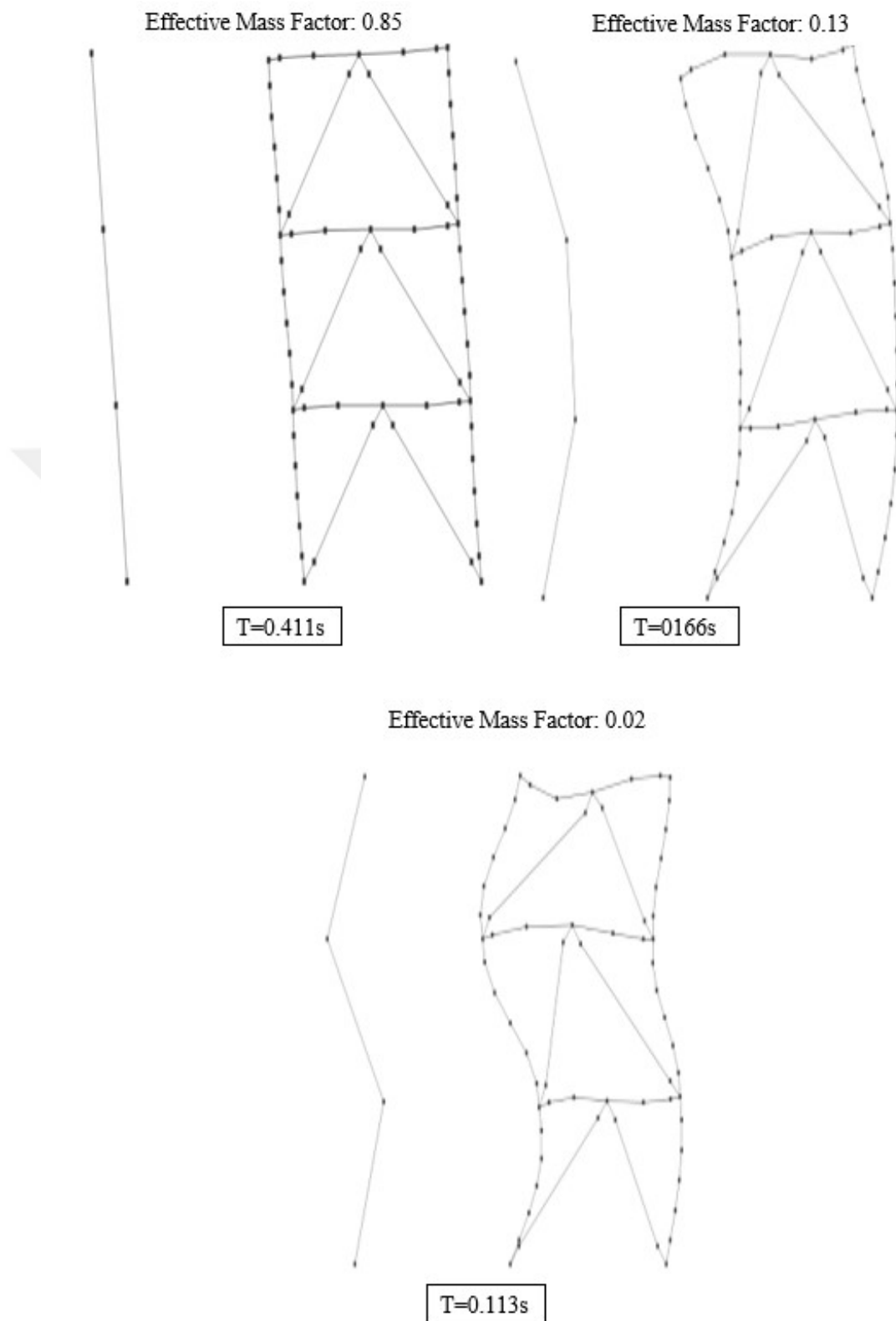
Figure 3.18. First three modes of building-1.
