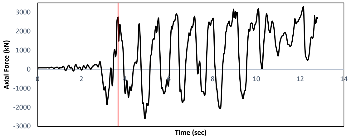
Figure 4.22. Axial forces in beam - time history.
