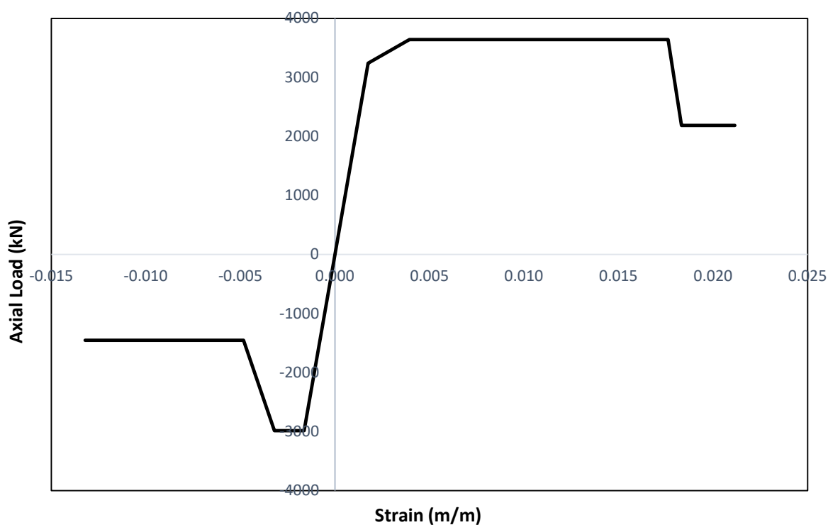
Figure 3.15. Sample brace backbone curve for HSS210X210X13 section.
