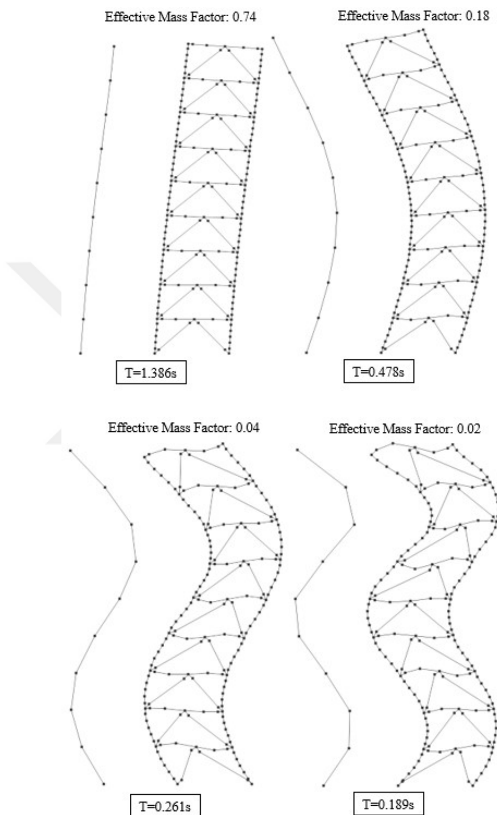
Figure 3.20. First four modes of building-3.
