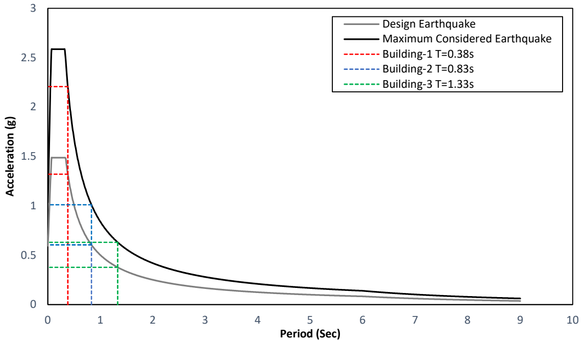
Figure 3.13. Design and maximum considered earthquake (DD-1) elastic response spectra.
