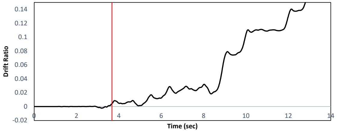
Figure 4.17. First story drift - time history.
