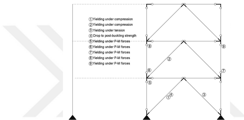
Figure 4.1. Hinge formation chronology for building-1.
