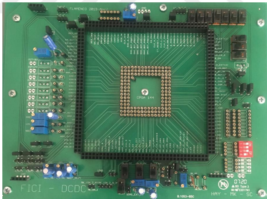
Figure 3.32. Charged balanced FICI system test PCB
