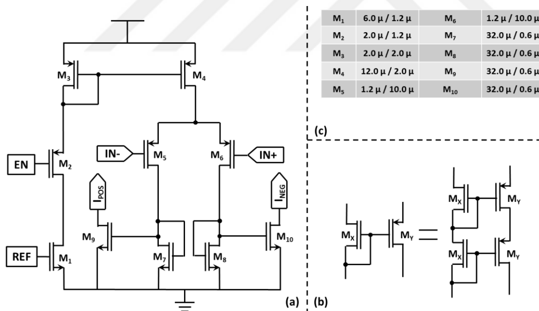
Figure 3.3. Schematic of the operational amplifier (a) current mirror structure (b) and sizes (c)
