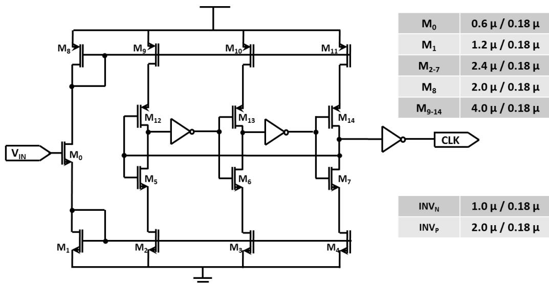
Figure 3.24. Schematic of the current starved voltage-controlled oscillator
