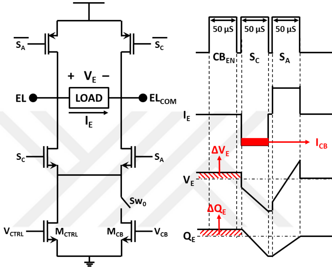
Figure 4.2. Modified CSS and charge unbalanced load characteristic
