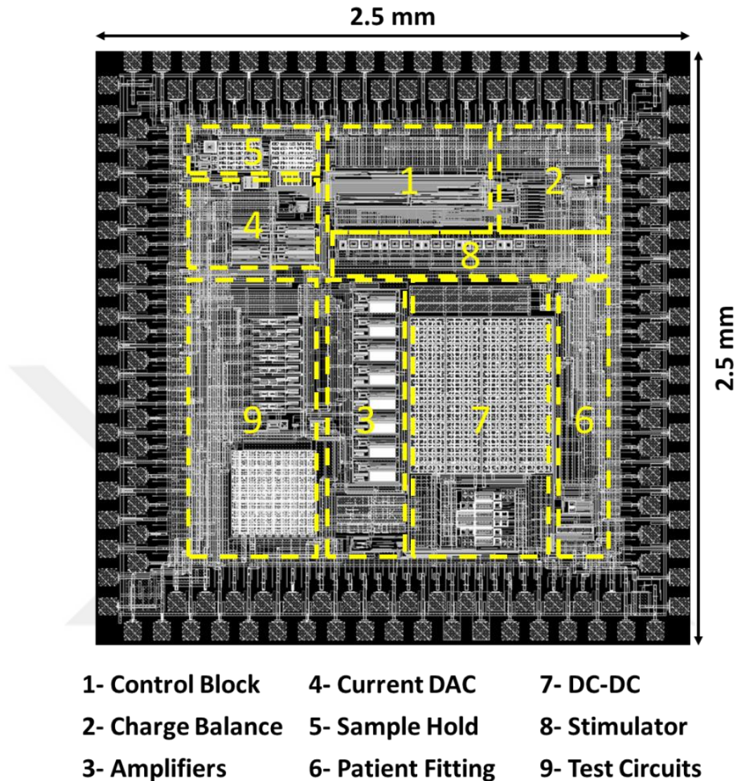
Figure 3.29. Layout of the designed FICI system
