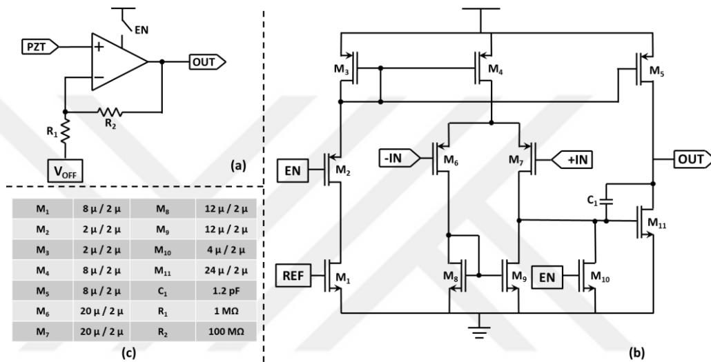
Figure 2.2. Input amplifier (a), schematic (b) and component parameters (c)
