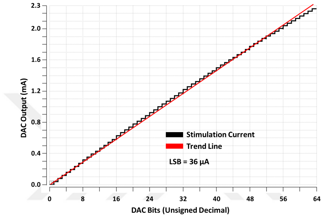
Figure 3.18. Patient fitting DAC characteristic
