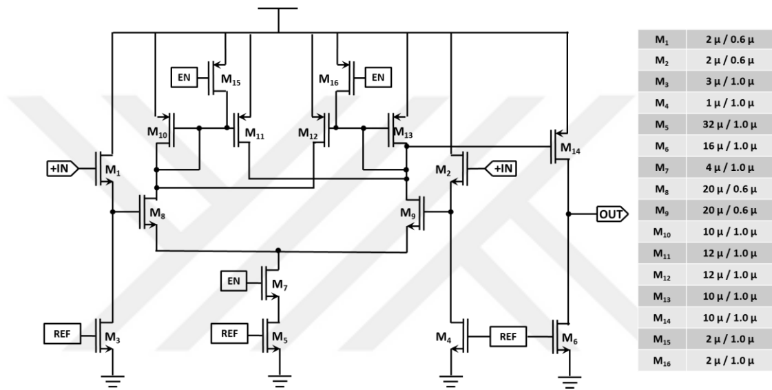
Figure 3.20. Charge balance window comparator schematic
