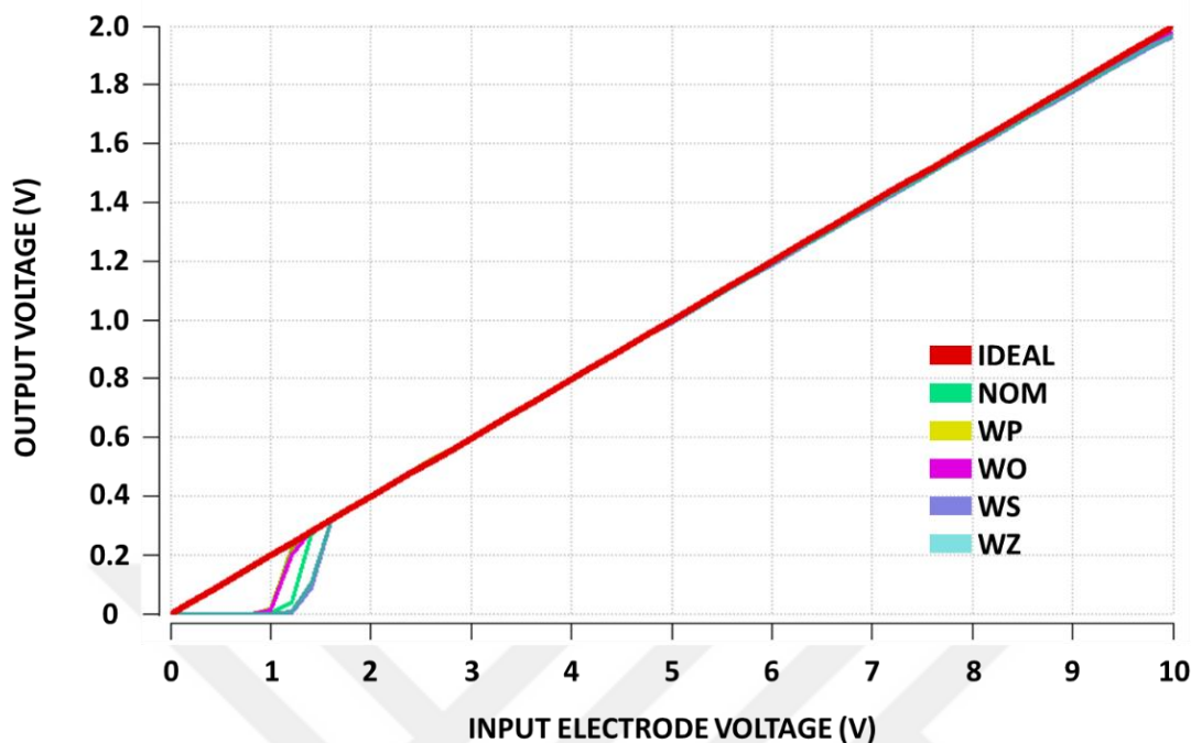
Figure 4.5. Corner simulation of the sensing part (Corners can be seen from Table 2.1.)
