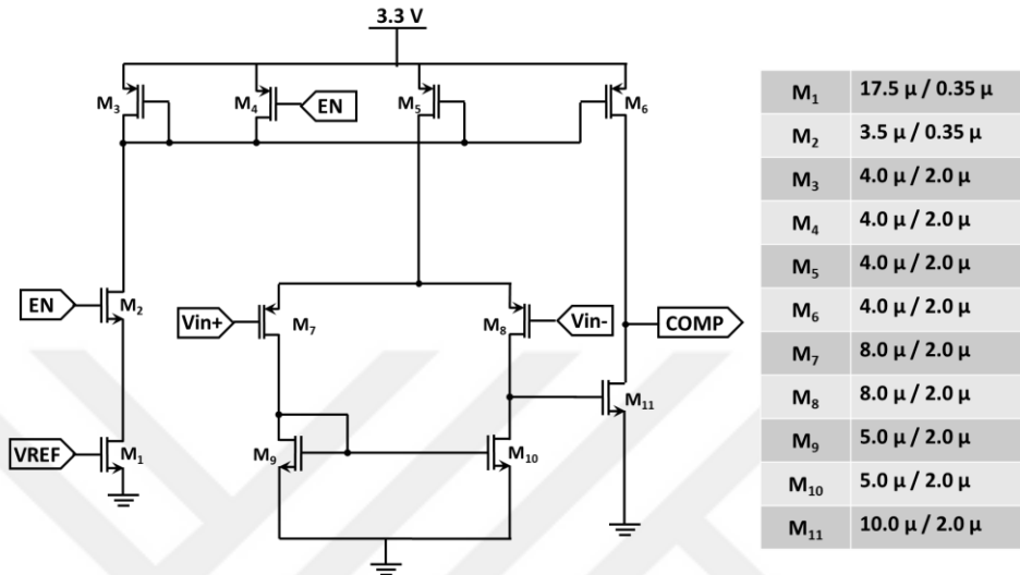
Figure 4.6. Schematic of the comparator
