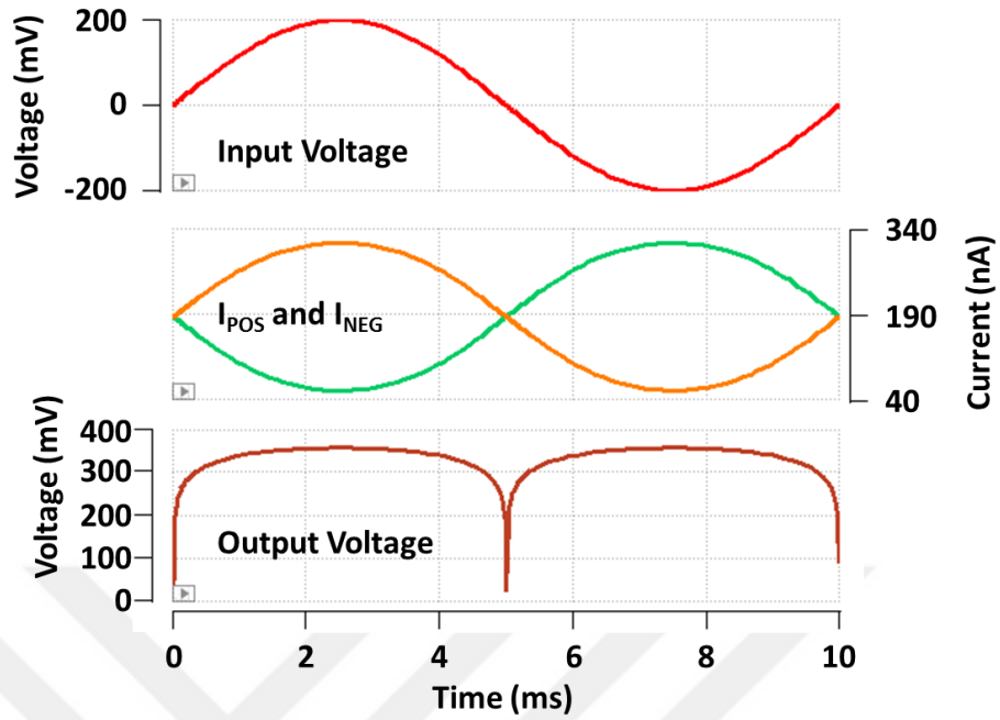
Figure 3.6. The amplifier and rectifier (diode load is connected to the rectifier) voltages when the input is sinusoidal wave with 200 mV PEAK voltage and 100 Hz frequency
