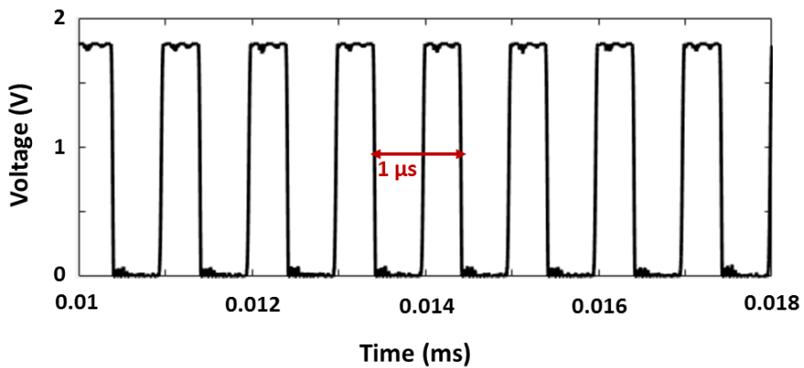
Figure 3.39. Oscillator circuit transient analysis
