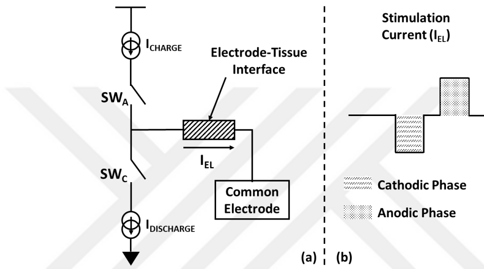
Figure 1.9. Simple CSS structure (a) and generated biphasic pulse waveform (b)
