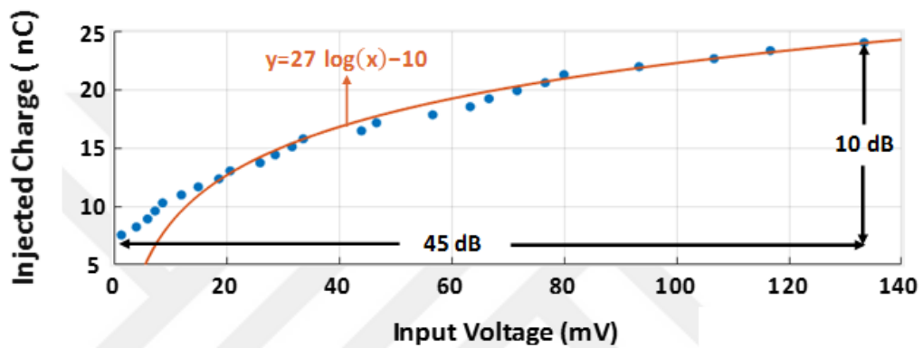
Figure 2.28. The injected charge amount respect to input voltage
