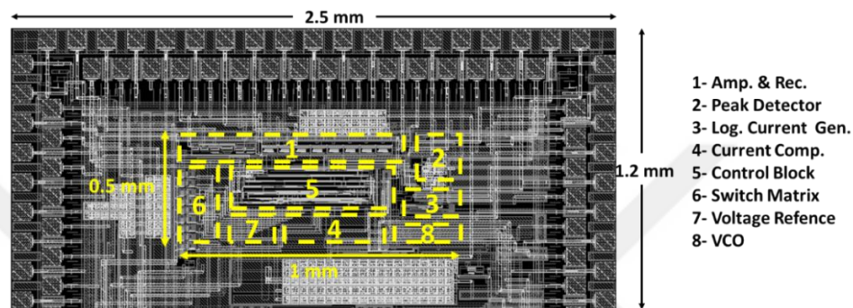
Figure 2.22. Layout of the FICI interface circuit
