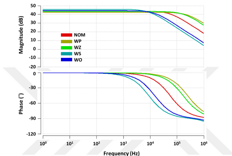
Figure 2.9. AC analysis of the rectifier comparator (Corners can be seen from Table 2.1.)
