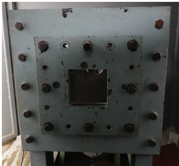
Figure 28 Specimen holder.
