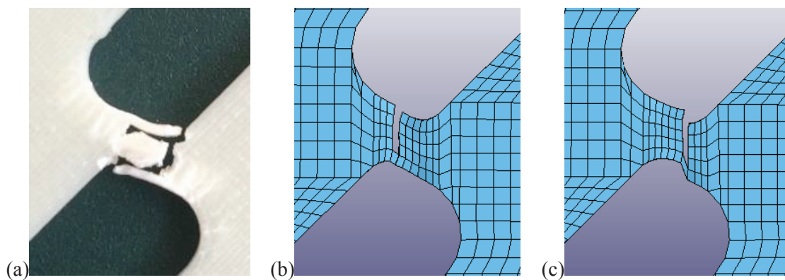
Figure 68 The state of failure of the shear 0° specimen in (a) experiment (b) single case optimization and (c) multi case optimization.
