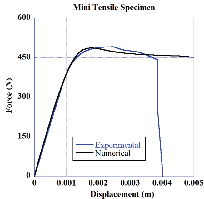
Figure 75 Experimental vs. single case optimization force–displacement curves of the mini tensile specimen.
