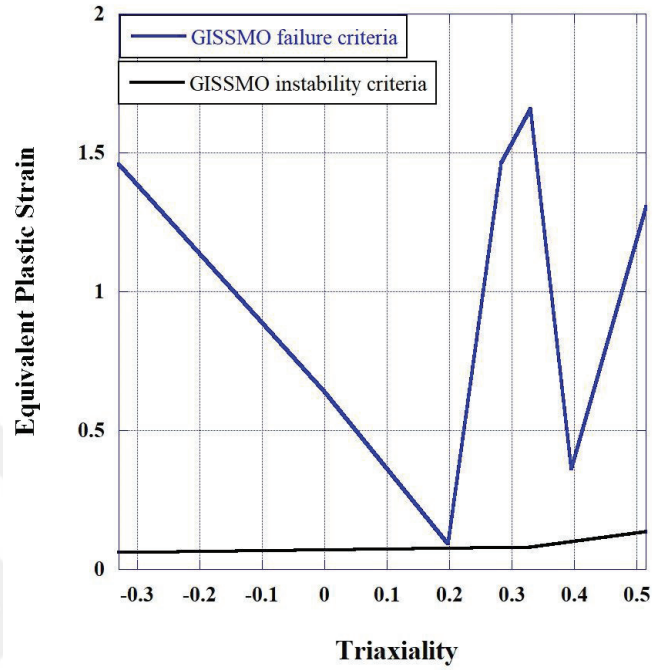
Figure 59 The GISSMO instability and failure criteria curves for all cases.
