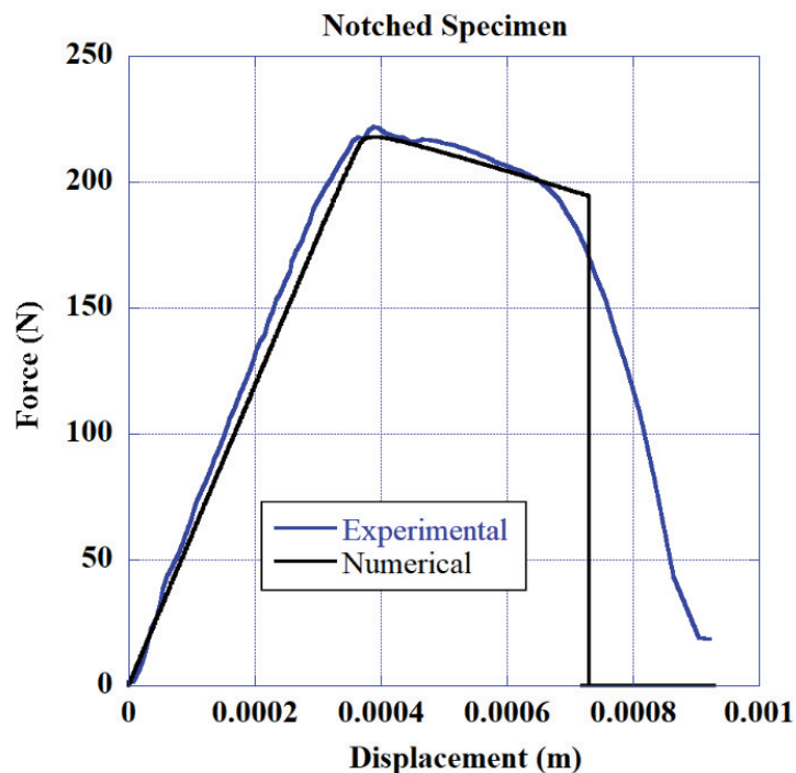
Figure 63 Experimental vs. single case optimization force–displacement curves of the notched specimen.
