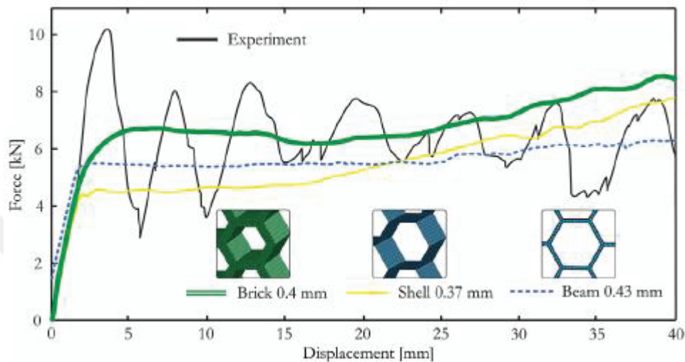
Figure 13. Force vs. displacement curves obtained from the experiments and numerical analyzes for three different element types (Source: Kucewicz et al. 2018).
