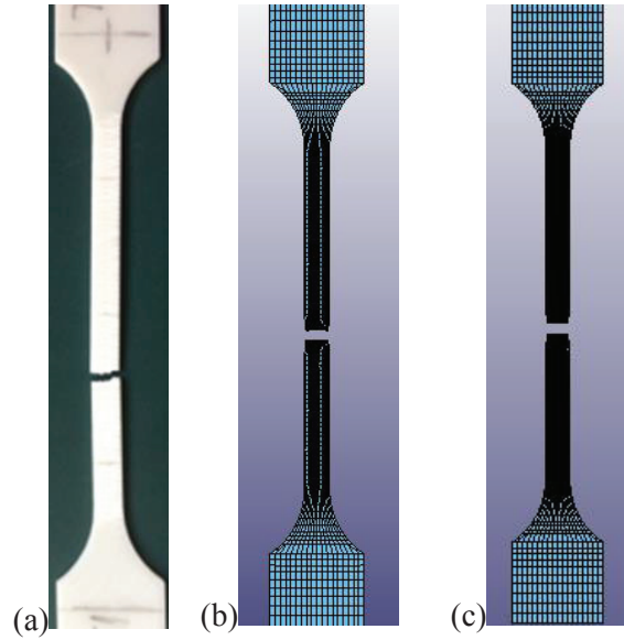
Figure 77 The state of failure of the mini tensile specimen in (a) experiment (b) single case optimization and (c) multi case optimization.
