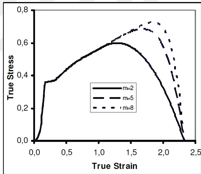
Figure 34 Effect of fading exponent (Source: Neukamm, Feucht, and Haufe 2009).
