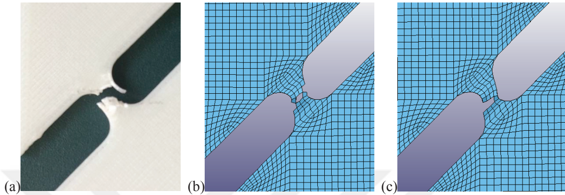
Figure 74 The state of failure of the shear 45° specimen in (a) experiment (b) single case optimization and (c) multi case optimization.
