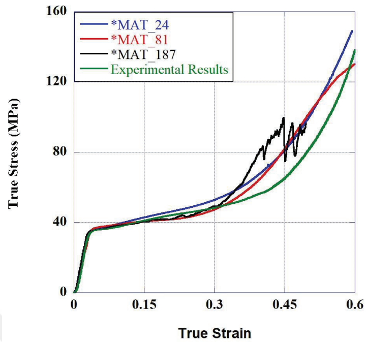
Figure 51 Comparison of material models for quasi-static compression test
