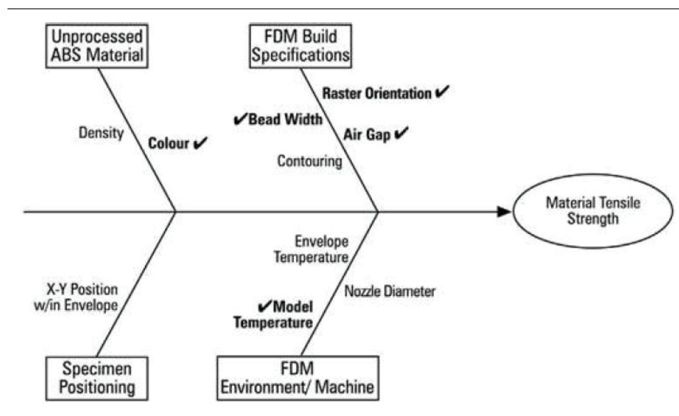
Figure 9. Fishbone diagram of potential parameters that effect tensile strength (Source: Ahn et al. 2002)
