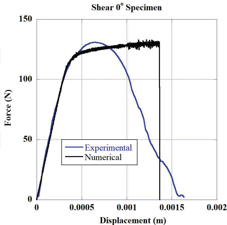
Figure 66 Experimental vs. single case optimization force–displacement curves of the shear 0° specimen.
