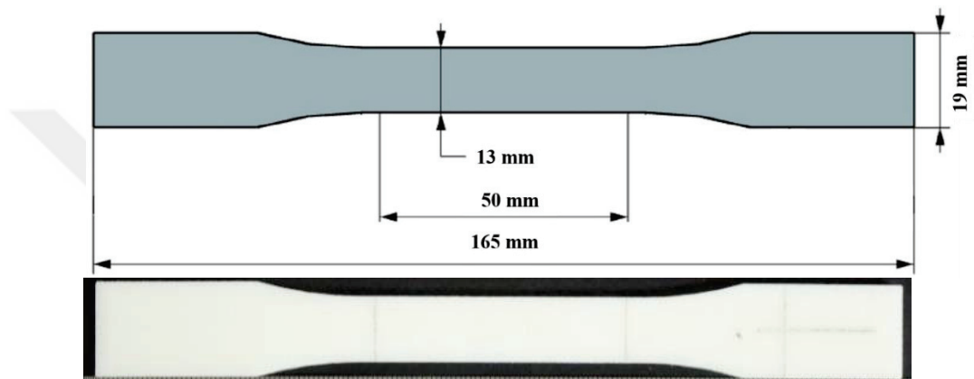
Figure 20 The dog-bone ABS specimen that is printed using FDM method according to ASTM D638-03 for quasi-static tensile testing.
