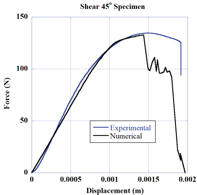
Figure 73 Experimental vs. multi case optimization force–displacement curves of the shear 45° specimen.
