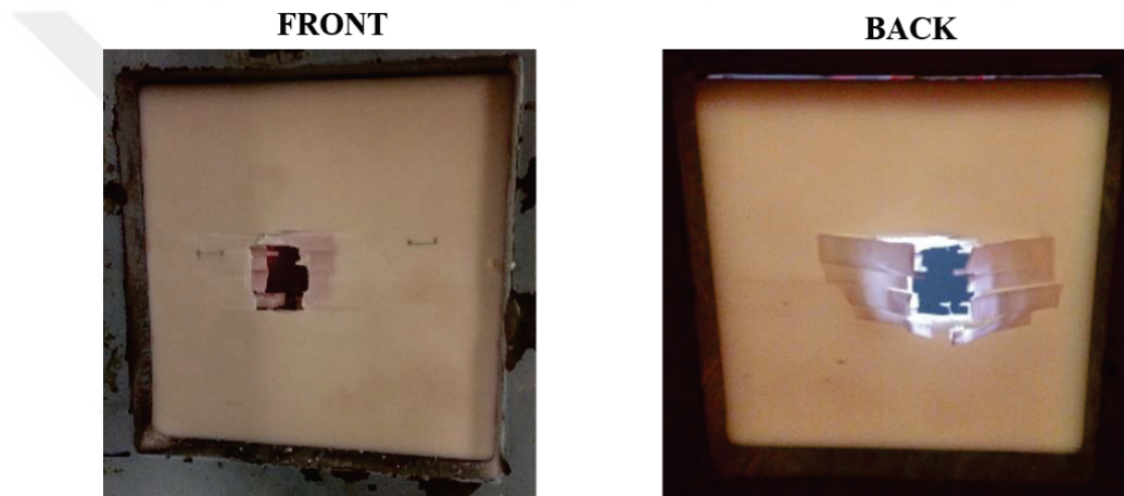
Figure 55 Front and back face of the deformed ABS plate.
