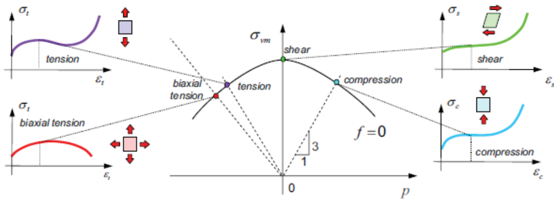
Figure 32 Von Mises stress as a function of pressure
