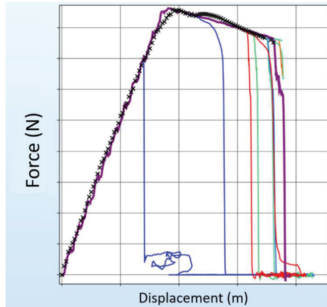
Figure 36 An example to a convergence process in LS-OPT
