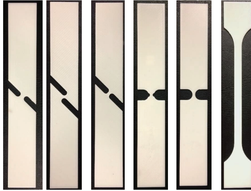
Figure 23 a) Shear60°, b) shear45°, c) shear 0°, d) double notched, e) notched, f) mini tensile ABS specimens that were printed using FDM method for GISSMO analyzes
