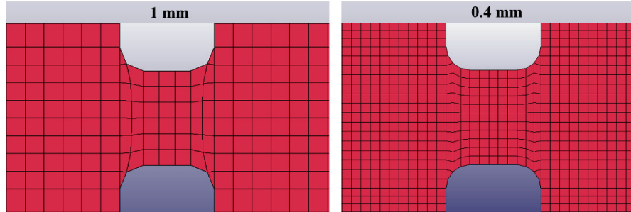
Figure 39 Custom tensile specimens meshed with 1 mm and 0.4 mm element size.
