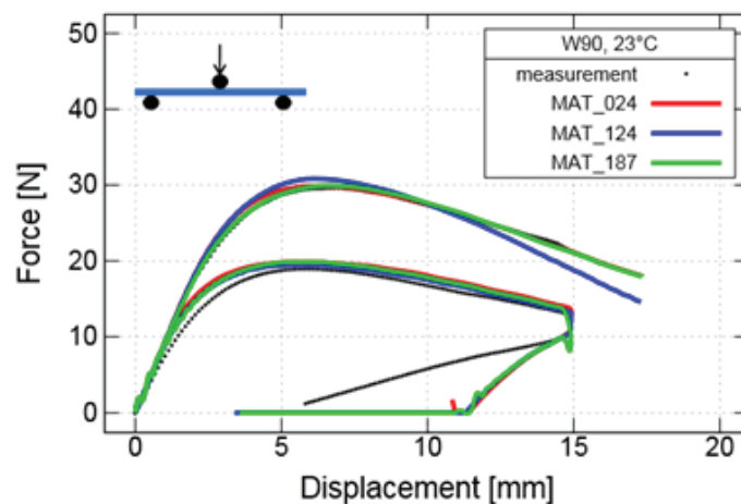
Figure 11. Force vs. displacement curves for the bending at quasi-static and high strain rates for the three material models (Source: P. Reithofer et al.2018).
