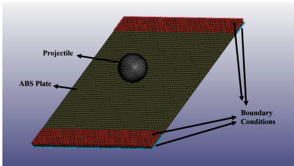
Figure 42 Gas gun model.
