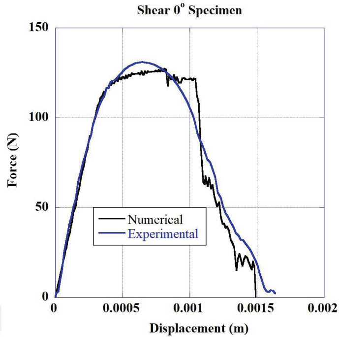
Figure 67 Experimental vs. multi case optimization force–displacement curves of the shear 0° specimen.
