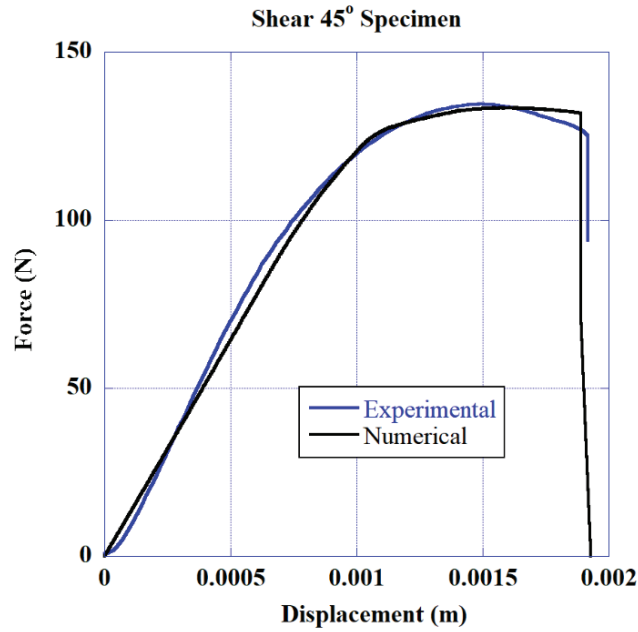
Figure 72 Experimental vs. single case optimization force–displacement curves of the shear 45° specimen.
