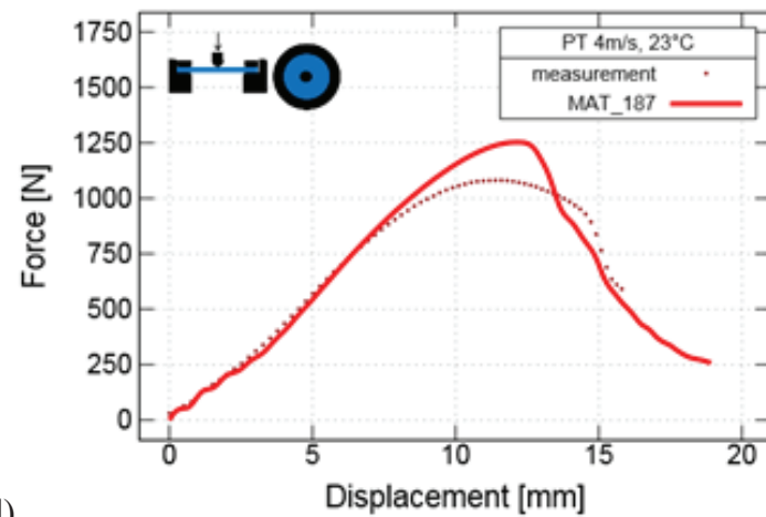
Figure 12. Comparison of test and simulation results for (a); tensile tests (b); dynamic bending tensile test and (c) dynamic puncture test (Source: P. Reithofer et al.2018).
