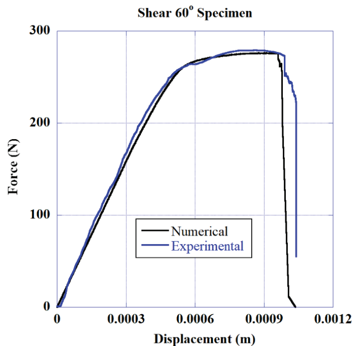
Figure 69 Experimental vs. single case optimization force–displacement curves of the shear 60° specimen.
