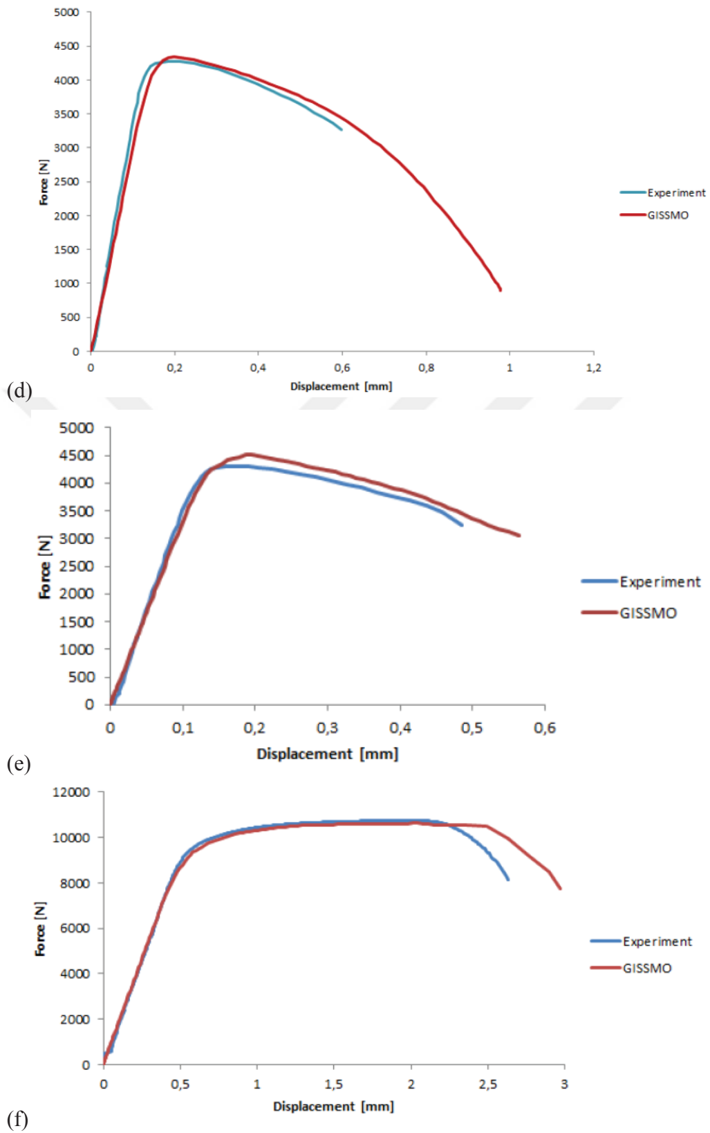
Figure 18. Force displacement curves for the (a) shear 0^\circ (b) shear 45^\circ (c) shear 60^\circ (d) notched (e) double notched (f) mini tensile specimens both experimental data and the GISSMO simulation (Source: D. Hörling et al.).
