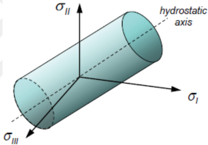
Figure 29 The von Mises yield surfaces in principal stress coordinates (Source:(Bertarelli 2016)).
