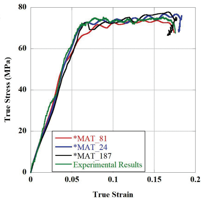
Figure 54 Comparison of material models for dynamic compression test.
