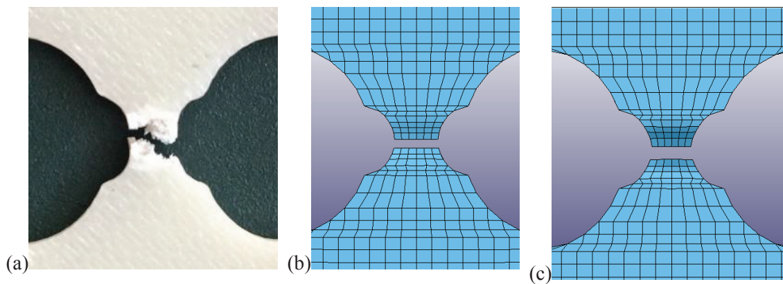
Figure 62 The state of failure of the double notched specimen in (a) experiment (b) single case optimization and (c) multi case optimization.
