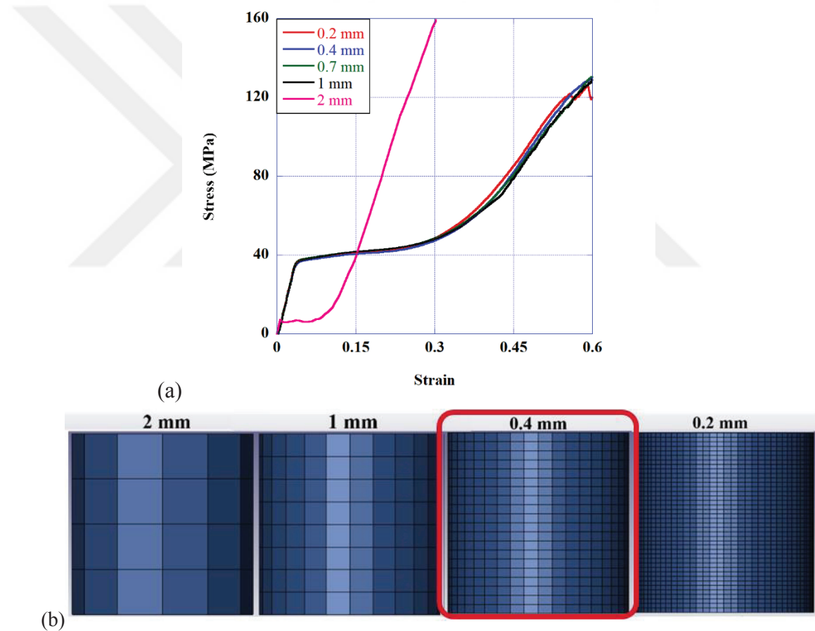
Figure 38 (a) Stress-strain curves for the compression with different element sizes (b) compression specimens meshed with 2, 1, 0.4 and 0.2 mm element size.
