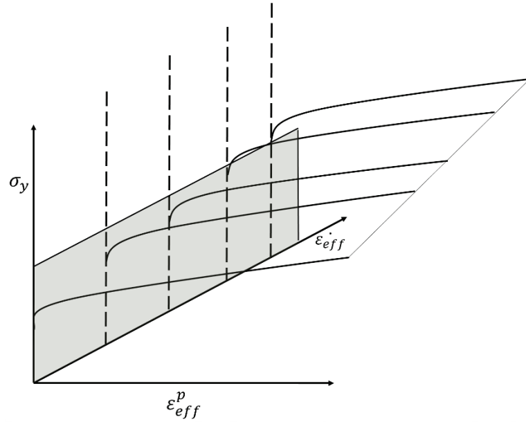
Figure 30 Table of curves defined to considerate strain rate effects.
