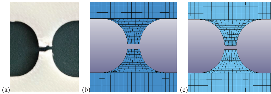
Figure 65 The state of failure of the notched specimen in (a) experiment (b) single case optimization and (c) multi case optimization.
