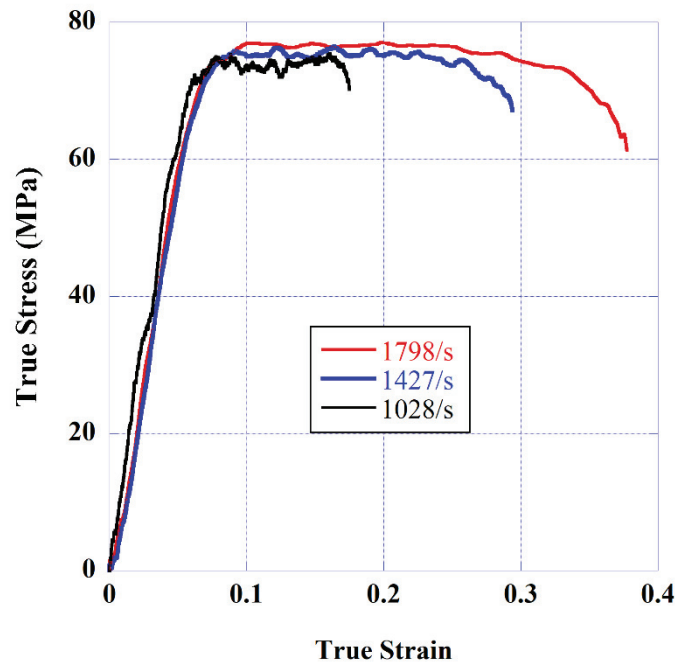
Figure 48 Comparison of compressive stress-strain curves obtained from SHPB at different strain rates
