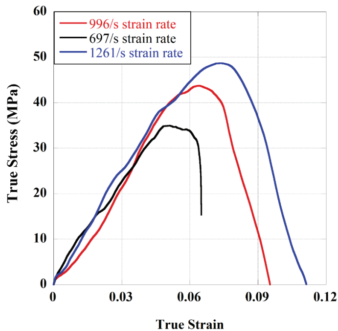
Figure 47 Comparison of tensile stress-strain curves obtained from SHTB at different strain rates
