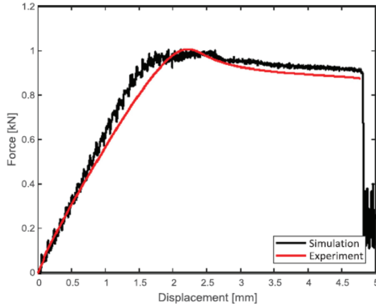
Figure 14. Numerical vs. experimental results of tensile test of ABS with using material model with damage (Source: Tabacu and Ducu 2018).
