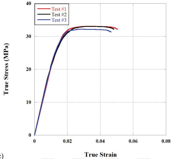
(c) Figure 43 Stress-strain curves of the FDM built ABS obtained from quasi-static tensile tests at (a) 10^{-3} \text{ s}^{-1} , (b) 10^{-2} \text{ s}^{-1} , and (c) 10^{-1} \text{ s}^{-1} strain rates.
