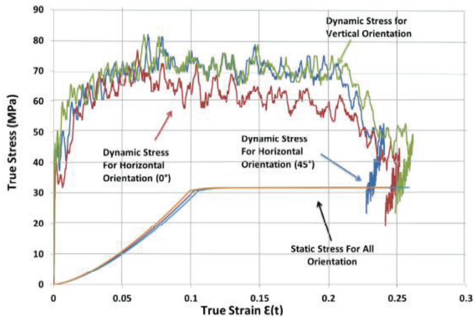
Figure 6. Stress strain curves at quasi-static and high strain rates for different building orientations of ABS specimens (Source: Jami, Masood, and Song 2013)
