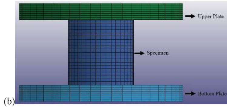
Figure 40 Quasi-static tensile (a) and compression (b) models.
