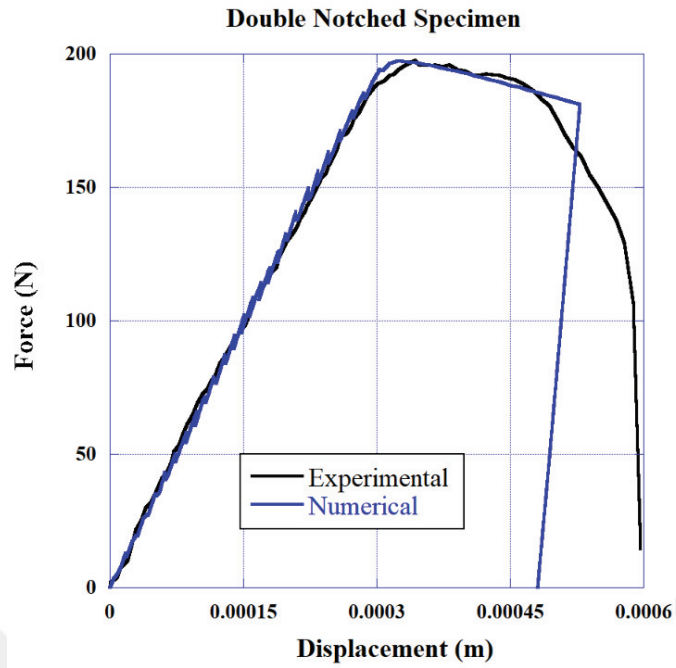
Figure 61 Experimental vs. multi case optimization force–displacement curves of the double notched specimen.
