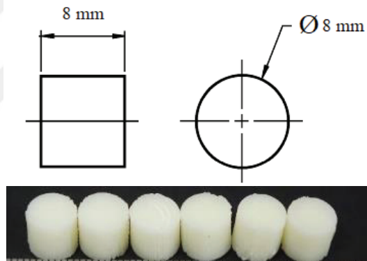
Figure 22 Cylindrical ABS specimen that is printed using FDM for quasi-static and dynamic compression testing.
