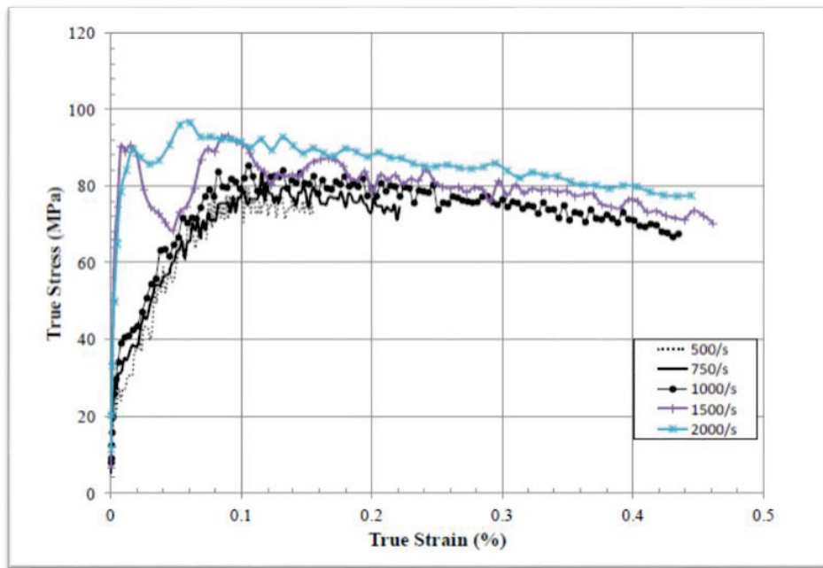
Figure 7. The Stress versus strain curve of the FDM built ABS under compressive load at different strain rates (Source: Peterson et. al. 2015)
