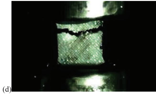
Figure 53 Failure states at STHB test, numerical and experimental comparison (a) *MAT_24 (b) *MAT_81 (c) *MAT_187 (d) experiment.
