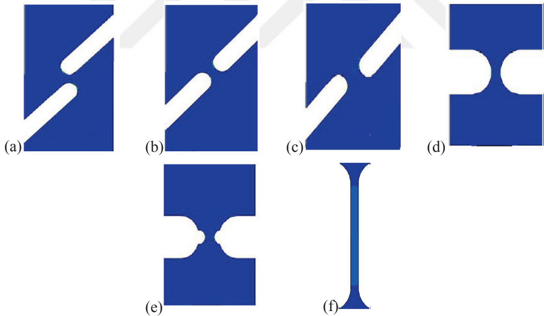
Figure 17 Produced (a) shear 0°, (b) shear 45°, (c) shear 60°, (d) notched, (e) double notched and (f) mini tensile test specimens (Source: D. Hörling et al.).
