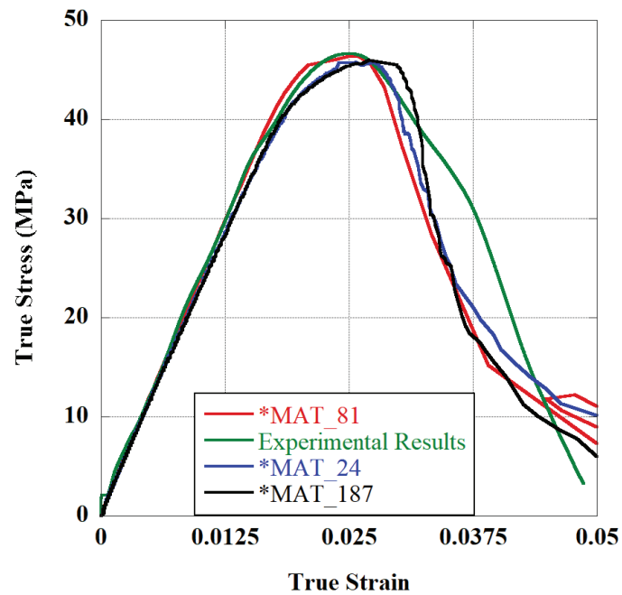
Figure 52 Comparison of material models for dynamic tensile test
