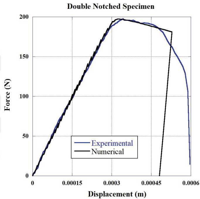
Figure 60 Experimental vs. single case optimization force-displacement curves of the double notched specimen.
