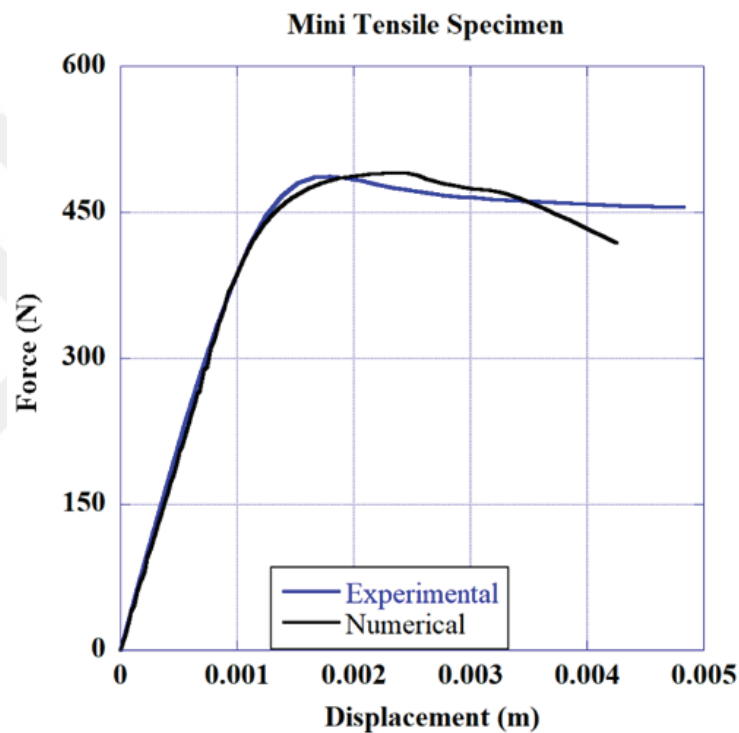
Figure 76 Experimental vs. multi case optimization force vs. displacement curves of the mini tensile specimen.
