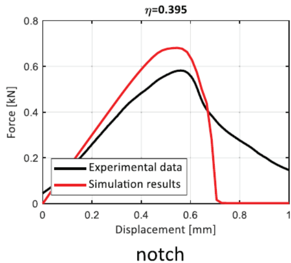
Figure 16. Force–displacement curves of experimental and numerical results (Source: S. Tabacu and C. Ducu. 2020).
