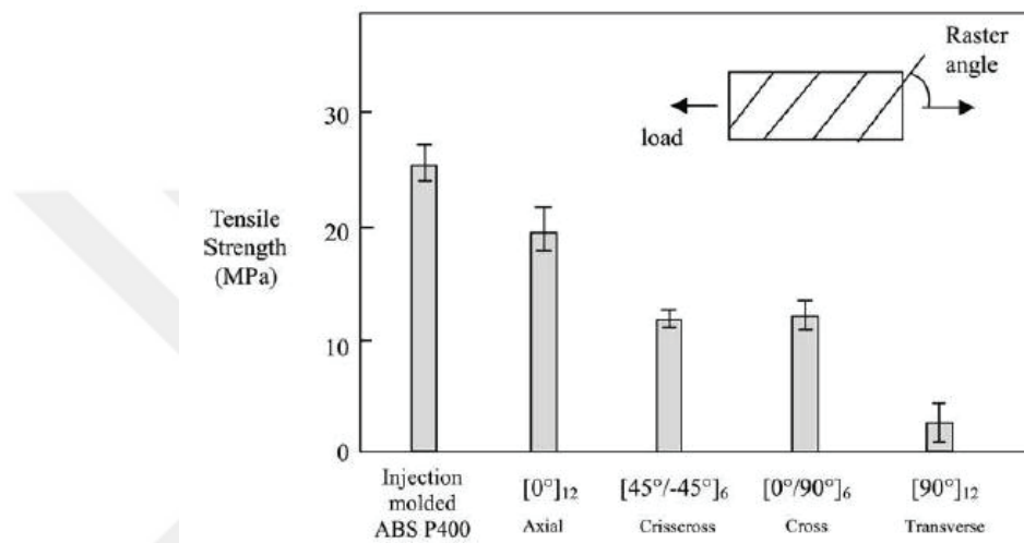
Figure 10 Tensile strength of the FDM produced ABS polymer with various raster angles (Source: Ahn et al. 2002).
