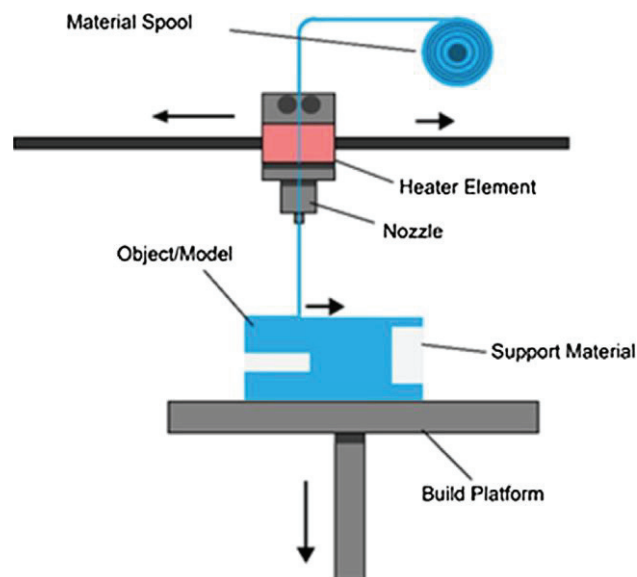
Figure 1. Fused Deposition Manufacturing setup (Source: Dizon et al. 2018).
