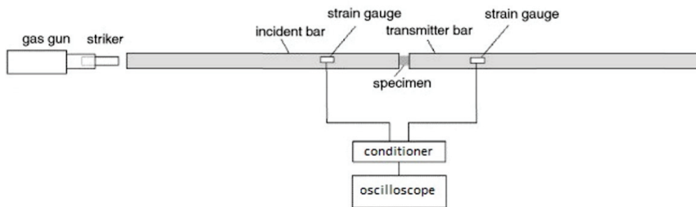
Figure 25 Split Hopkinson (a) tension (b) compression bar setup
