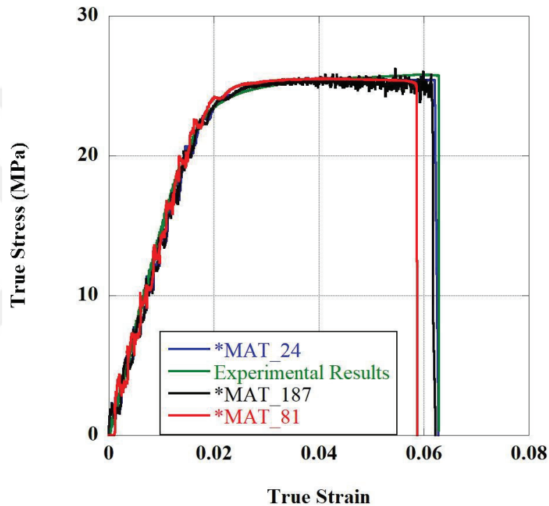
Figure 49 Comparison of material models for quasi-static tensile test
