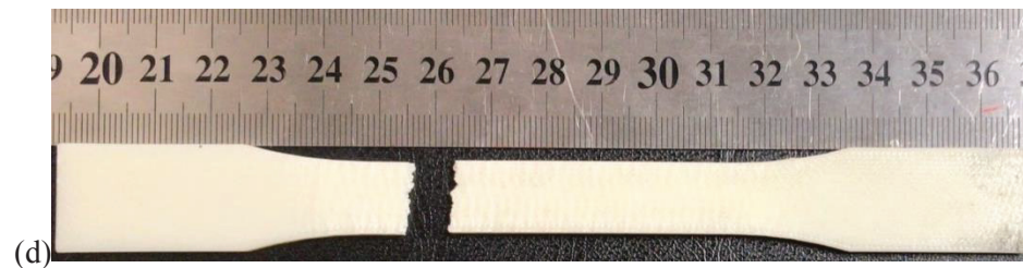
Figure 50 The D638 specimen at failure states (a) *MAT_24 (b) *MAT_81 (c) *MAT_187 (d) experiment.
