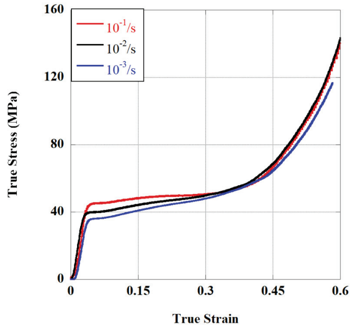
Figure 46 Comparison of compressive stress-strain curves at different strain rates
