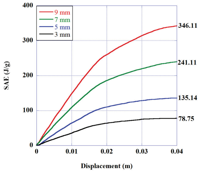
Figure 57 Comparison of SAE-Displacement Graphs for (a) MAT_24 and (b) MAT_187 material models for different thickness values.
