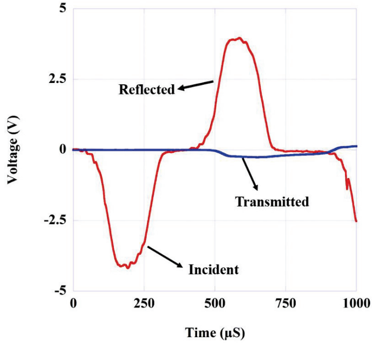
Figure 26 An example to a voltage versus time curve obtained from SHPB testing of FDM built ABS.
