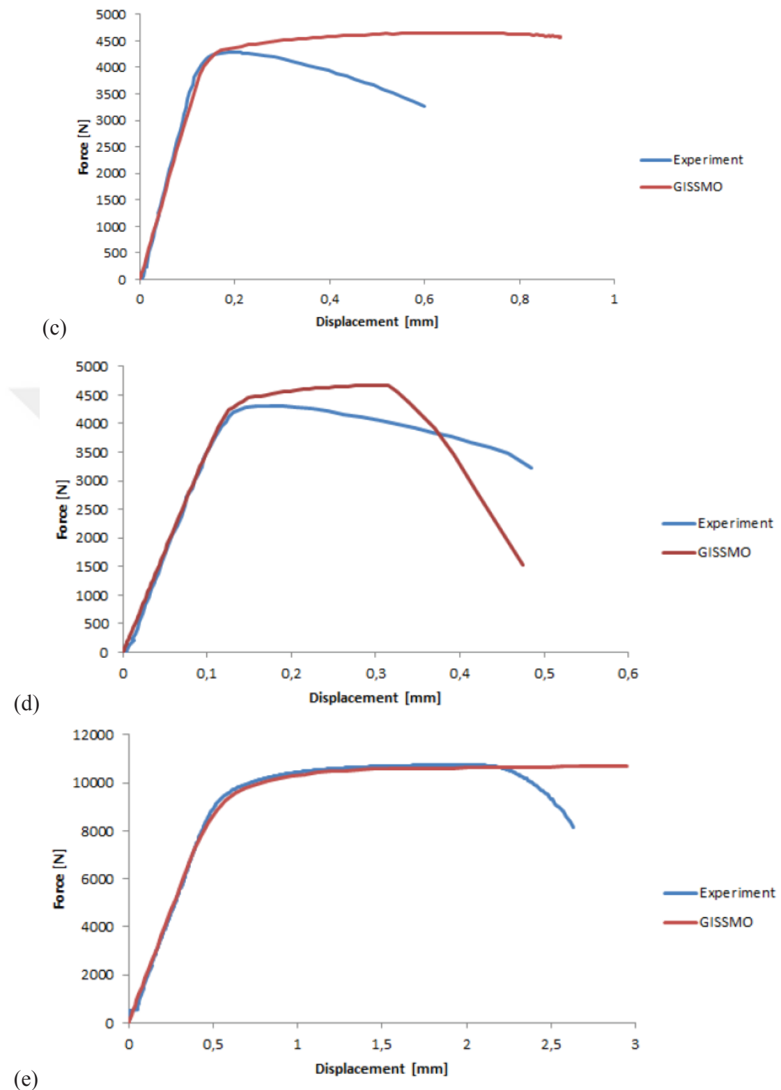
Figure 19. Force displacement curves for the (a) shear 0^\circ (b) shear 45^\circ (c) notched (d) double notched (e) mini tensile specimens both experimental data and the GISSMO simulation (Source: D. Hörling et al.).
