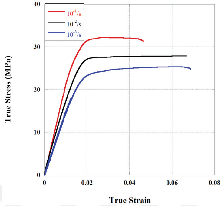
Figure 44 Comparison of tensile stress-strain curves at strain rates of 10^{-3} \text{ s}^{-1} , 10^{-2} \text{ s}^{-1} , and 10^{-1} \text{ s}^{-1} .
