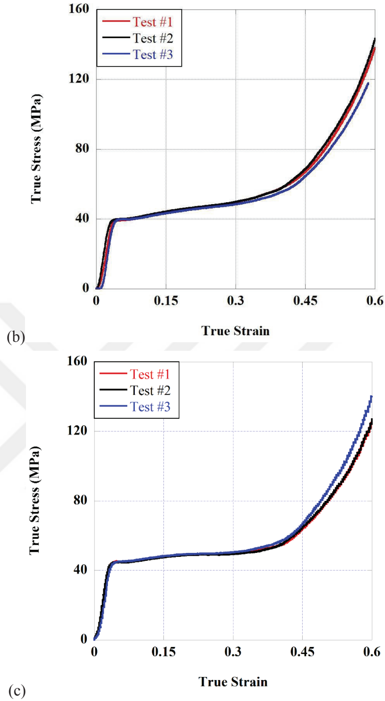
Figure 45. Stress-strain curves of FDM built ABS obtained from quasi-static compression tests at (a) 10^{-3} \text{ s}^{-1} , (b) 10^{-2} \text{ s}^{-1} , and (c) 10^{-1} \text{ s}^{-1} strain rates
