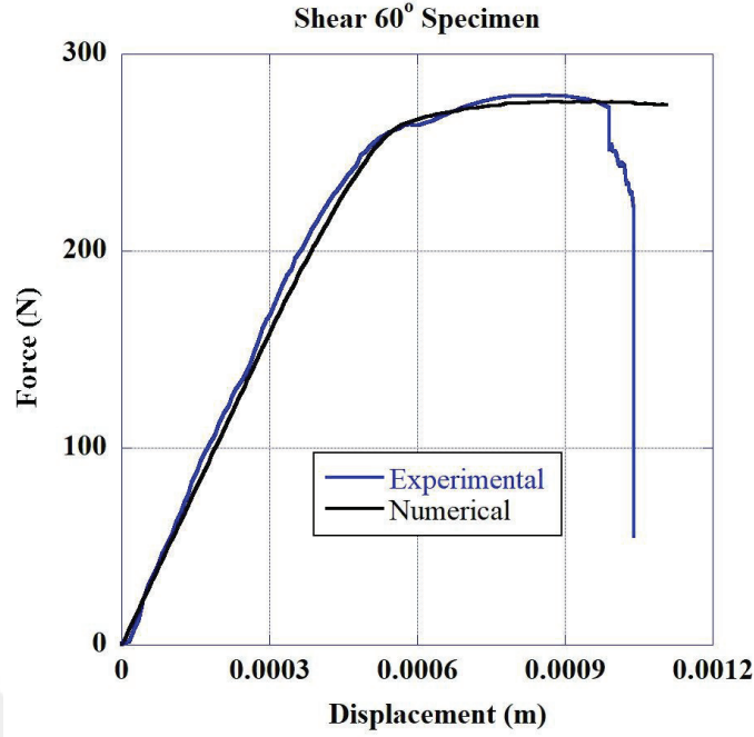
Figure 70 Experimental vs. multi case optimization force–displacement curves of the shear 60° specimen.
