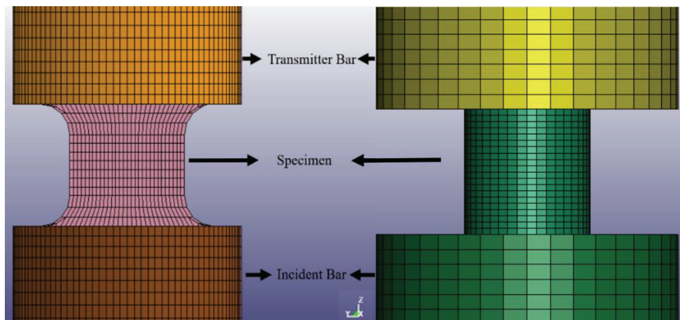
Figure 41 SHTB and SHPB models.
