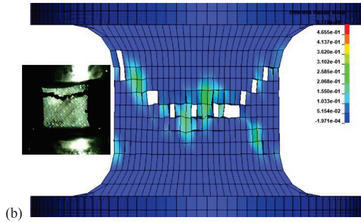
Figure 78 Comparison of experimental and numerical (a) true stress strain curves (b) appearance of failure for the SHTB test
