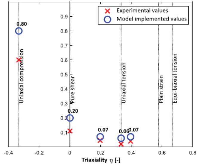
Figure 15. Model implemented and experimental equivalent plastic strain values (Source: S. Tabacu and C. Ducu. 2020).
