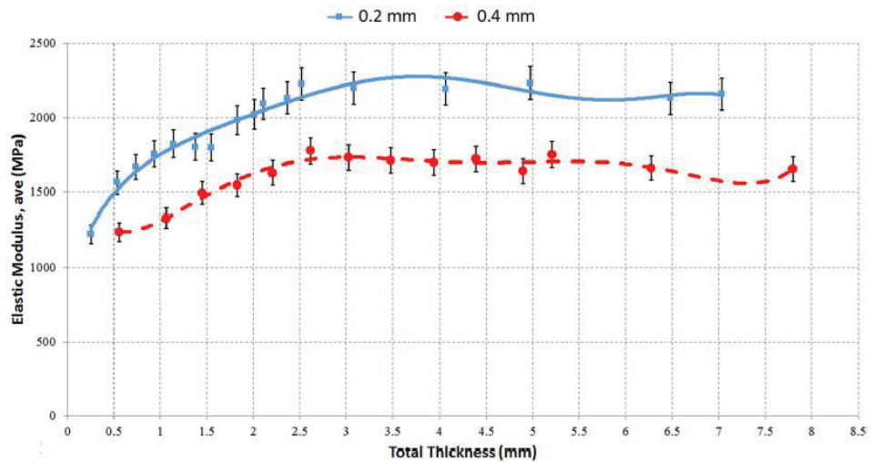
Figure 8 Comparison of elastic modulus for specimens produced with 0.2 mm and 0.4 mm layer thicknesses (Source: Rankouhi et al 2016).
