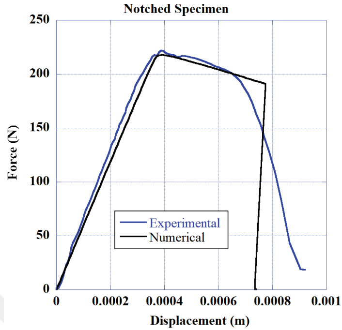
Figure 64 Experimental vs. multi case optimization force–displacement curves of the notched specimen.
