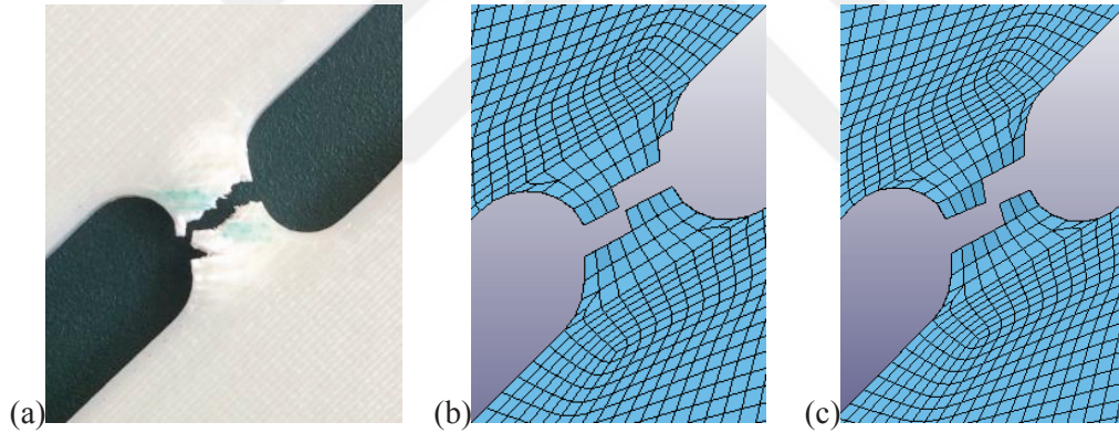
Figure 71 The state of failure of the shear 60° specimen in (a) experiment (b) single case optimization and (c) multi case optimization.
