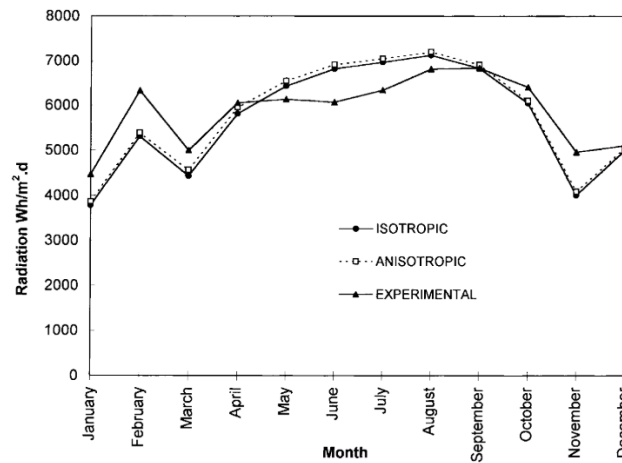
Figure 14. Monthly averages on 45° tilted surface [54].
