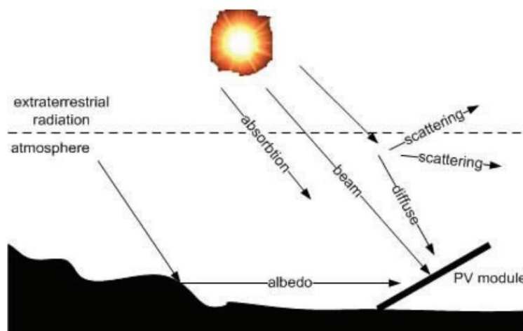
Figure 1. Solar energy components [4]
