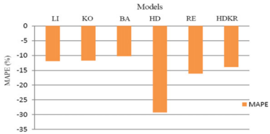
Figure 7. Mean Absolute Percentage Error (MAPE) for 6 models [47].
