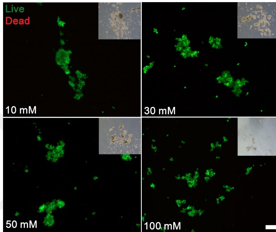
Figure 3.26. Cell viability images of H9c2 spheroids in varied Gx concentrations: 10, 30, 50 and 100 mM. Scale bar: 200 \mu m.
