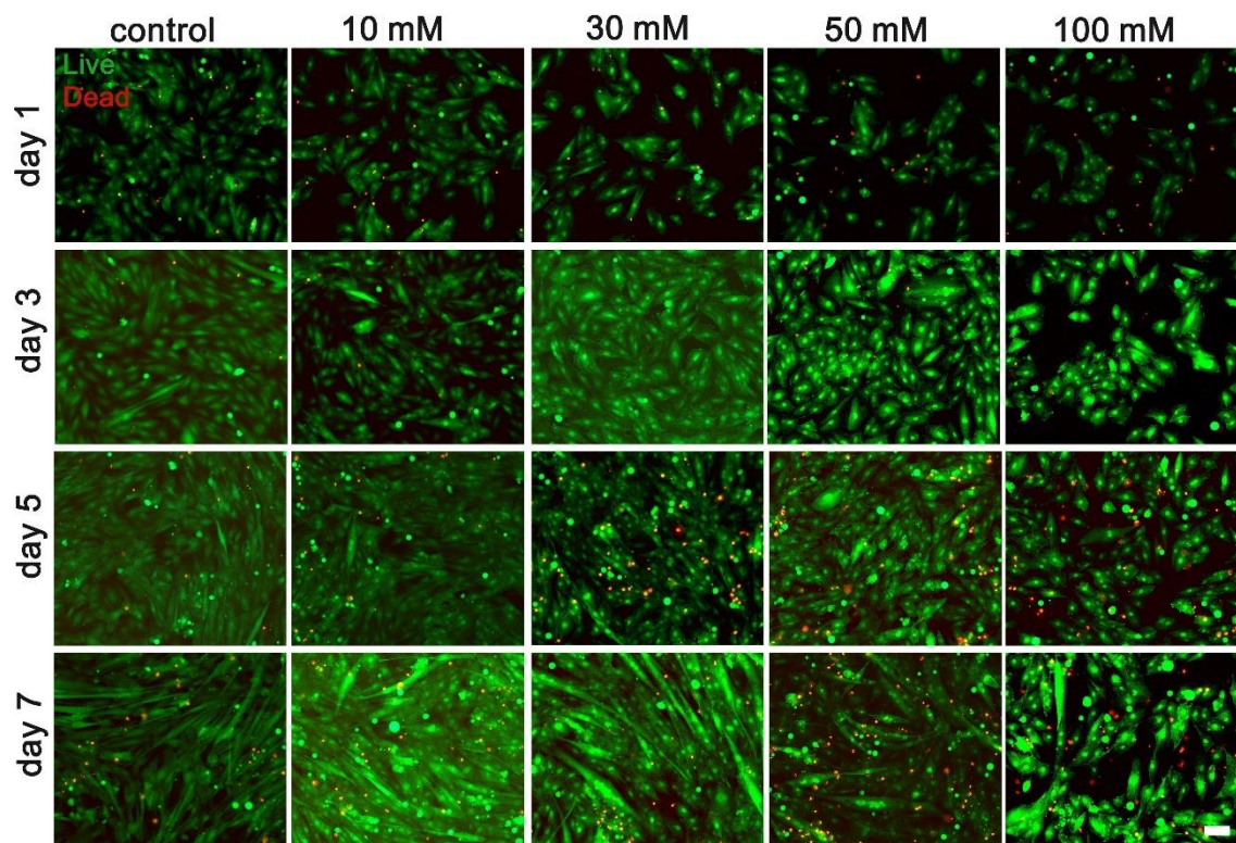
Figure 3.17. Cell viability images of H9c2 cells treated with Gx in varied concentrations (0/10/30/50/100 mM) in long-term culture (1/3/5/7 days). Scale bar: 100 \mu m.
