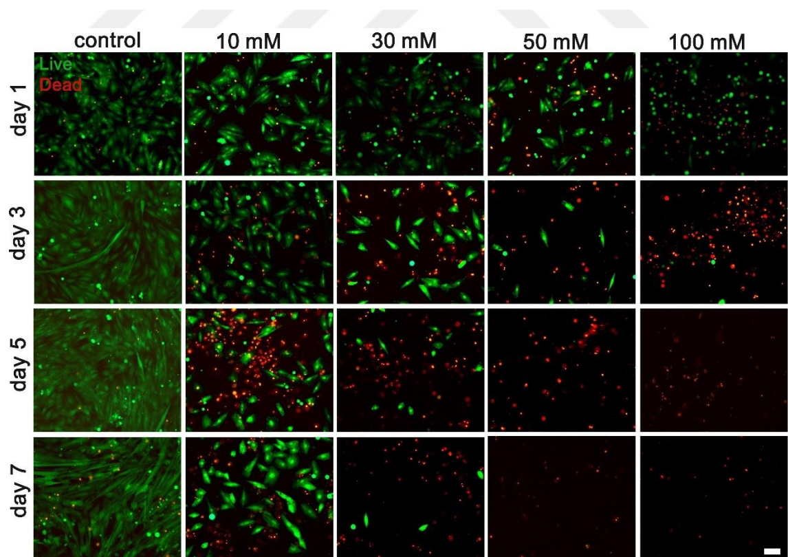
Figure 3.19. Cell viability images of H9c2 cells treated with Ox in varied concentrations (0/10/30/50/100 mM) in long-term culture (1/3/5/7 days). Scale bar: 100 \mu m.
