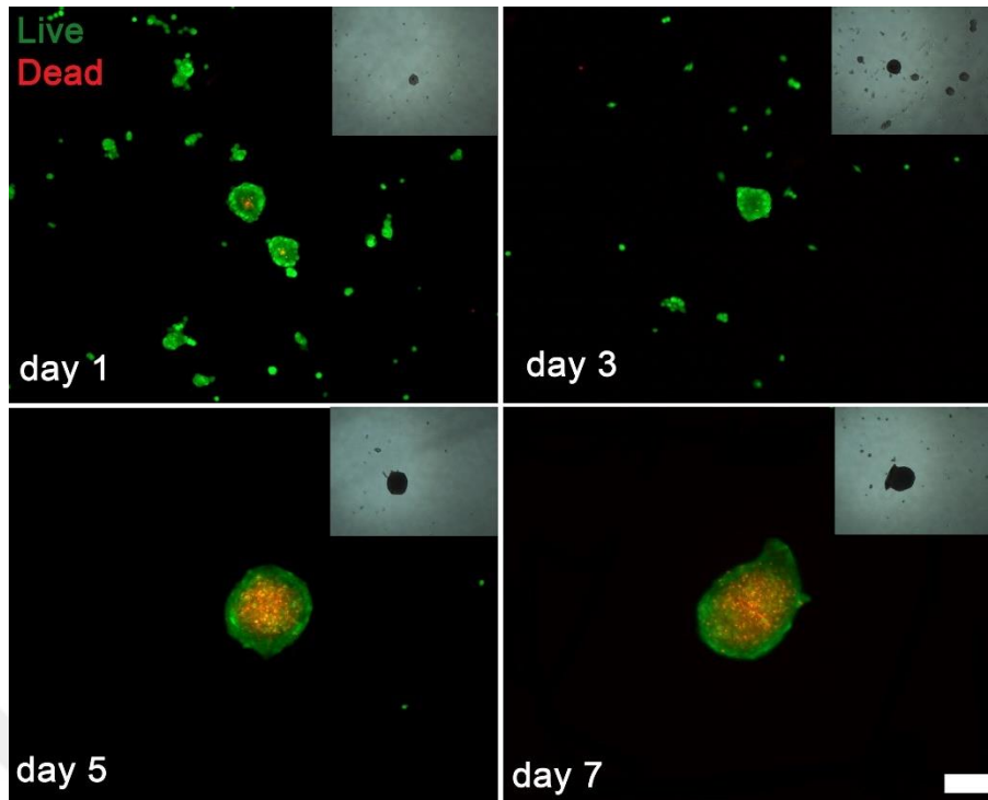
Figure 3.10. Cell viability images of NIH/3T3 spheroids for varied cell culture times on day 1, 3, 5,7 (green: live cells, red: dead cells). Scale bar: 200 \mu\text{m}
