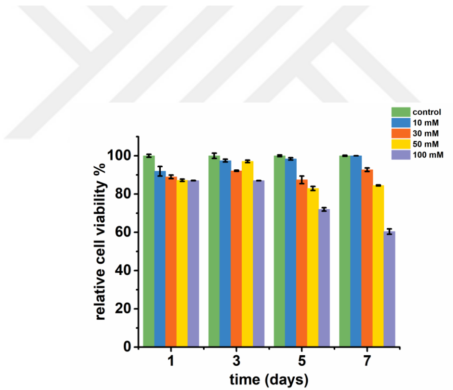
Figure 3.21. Relative cell viability % of H9c2 cells treated with Dx in varied concentrations (0/10/30/50/100 mM) in long-term culture (1/3/5/7 days).
