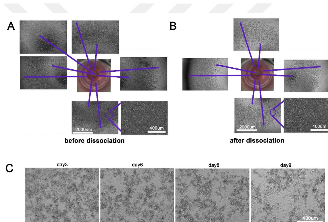
Figure 3.58. Light microscopy images of ring-shaped patterned WTC CMs. A) before disassociation, B) after disassociation, C) long-term cultured cellular structures.
