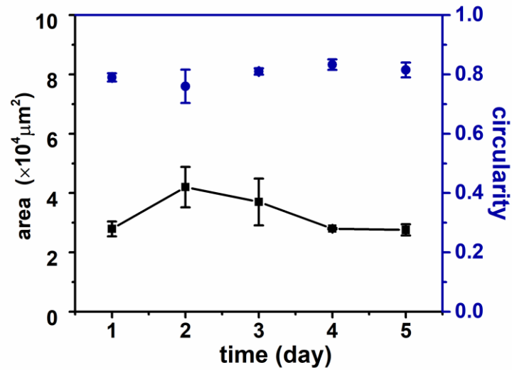
Figure 3.30. Representative spheroid area versus circularity for varied cell culture times on day 1, 2, 3, 4, 5.
