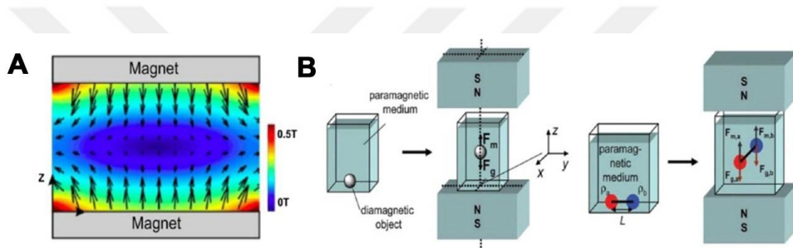
Figure 1.4. A) 3D magnetic field simulation in the X-Z plane, B) Schematic representation of basic MagLev setup showing the magnetic ( F_m ) and gravitational forces ( F_g ) that levitate the object 115 .
