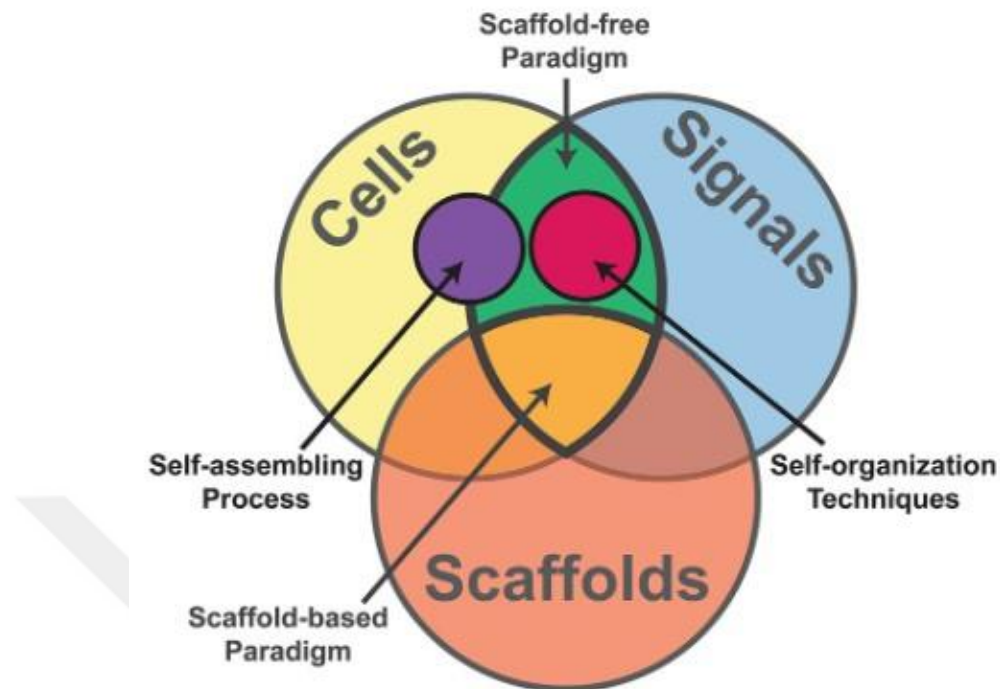
Figure 1.1. Traditional tissue engineering and, as a new approach, scaffold-free engineering with their components. 11
