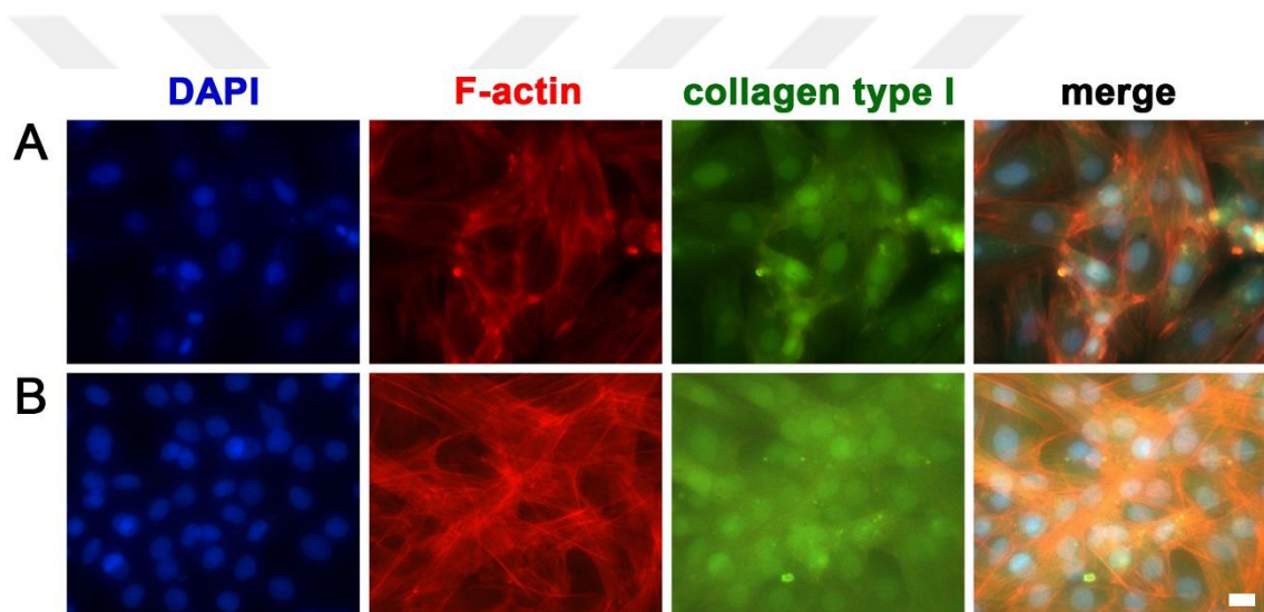
Figure 3.50. Immunofluorescent staining of patterned 3D cardiac structures. A) day 1, B) day 7. Scale bar: 20 \mu\text{m} .
