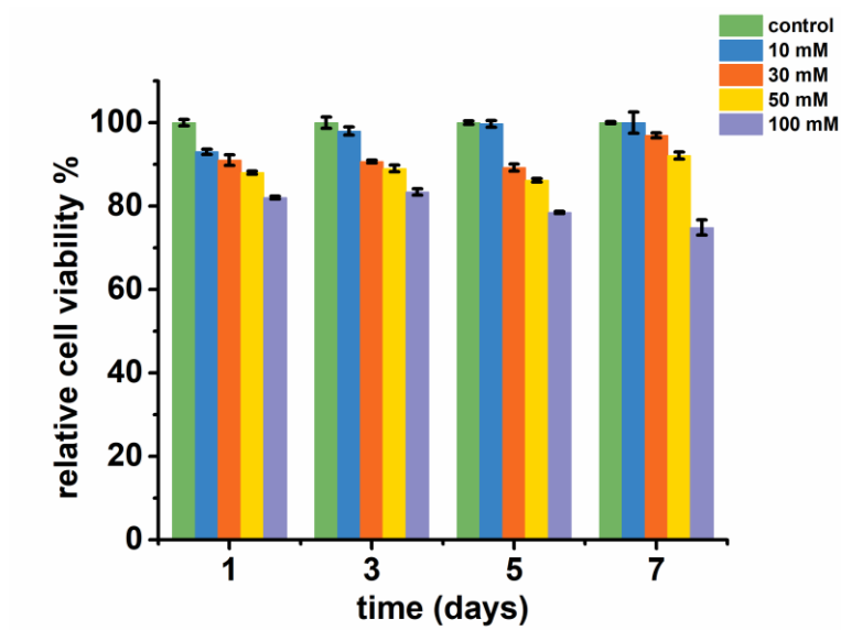
Figure 3.20. Relative cell viability % of H9c2 cells treated with Gx in varied concentrations (0/10/30/50/100 mM) in long-term culture (1/3/5/7 days).
