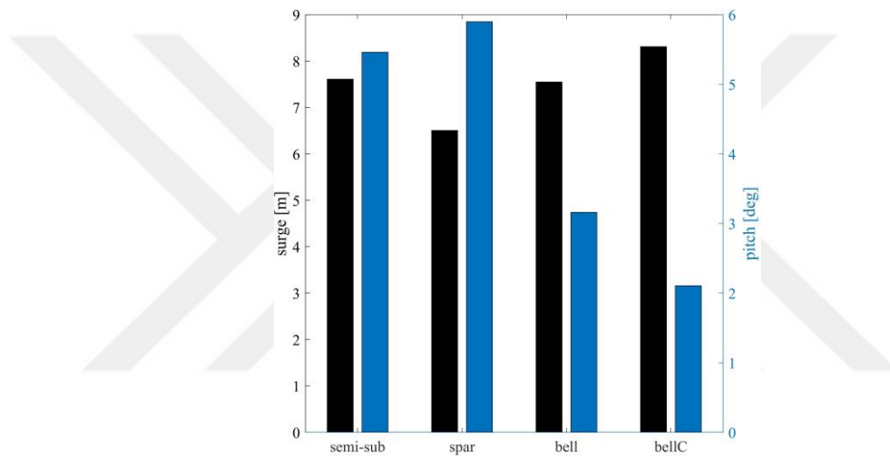
Figure 7.19: Platform responses to wind heeling moment (left y-axis is surge; right y-axis is pitch angle).
