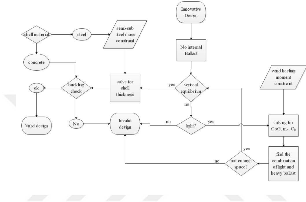
Figure 6.2: Flowchart explaining the procedure of a one-design point for the innovative geometry.
