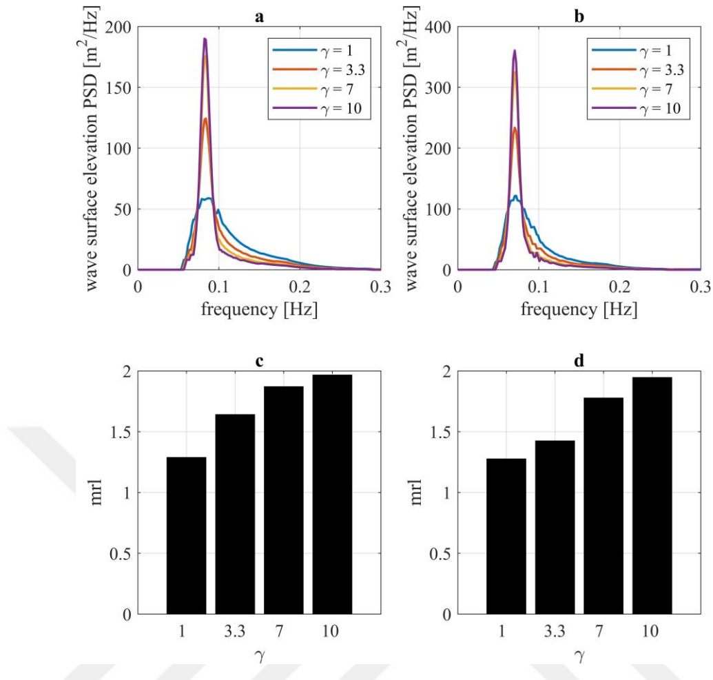
Figure 4.29: Power spectral density for the synthesized wave surface elevation and groupiness factor mrl of each spectrum shape (a and c for the moderate wave, b, and d for the extreme wave).
