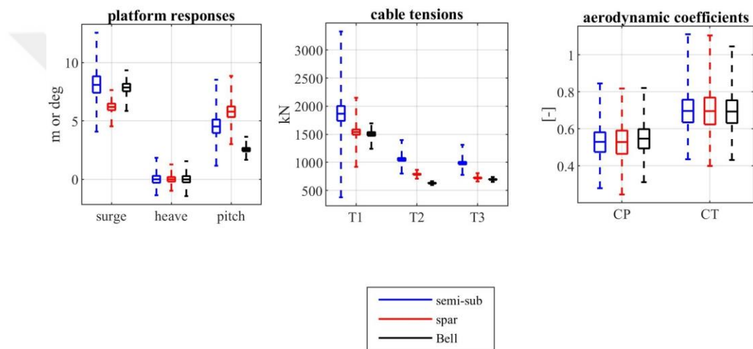
Figure 7.31: Whisper box, comparing responses, tensions, and aerodynamic coefficients for the designated platforms.
