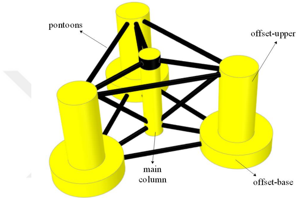
Figure 4.7: Perspective view of the OC5 DeepCwind floating platform geometry.
