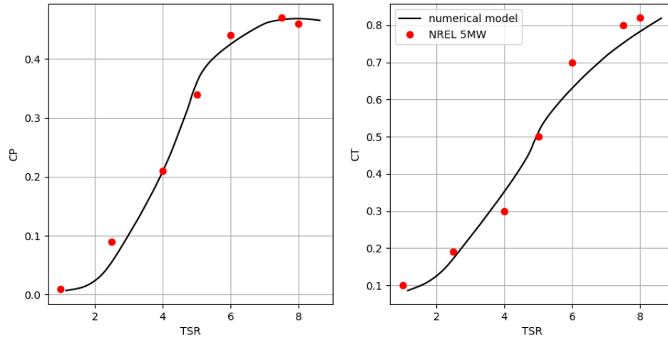
Figure 4.4: Power and thrust coefficient as a function of TSR.
