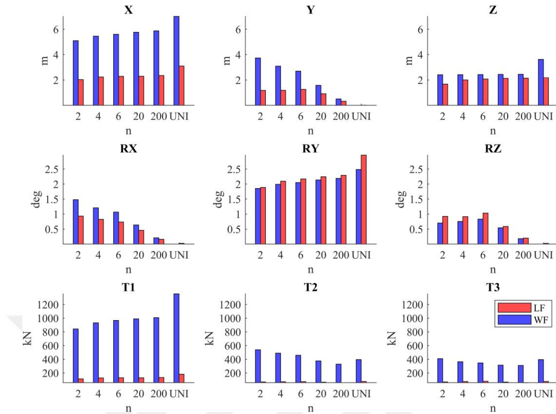
Figure 4.37: Structural motion and cable tensions showing the gradual change between a unidirectional and a multidirectional excitation (n=2,4,6,20, and 200).
