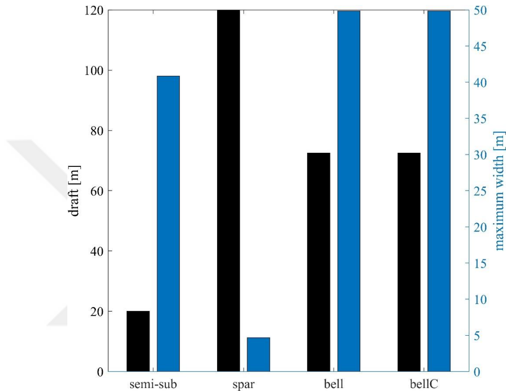
Figure 7.2: Geometric platform comparison. The left y-axis represents draft, and right y-axis is the width.
