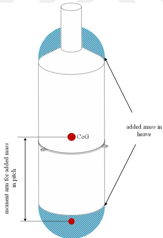
Figure 5.3: A simplified theoretical approach for calculating added mass in heave and pitch.
