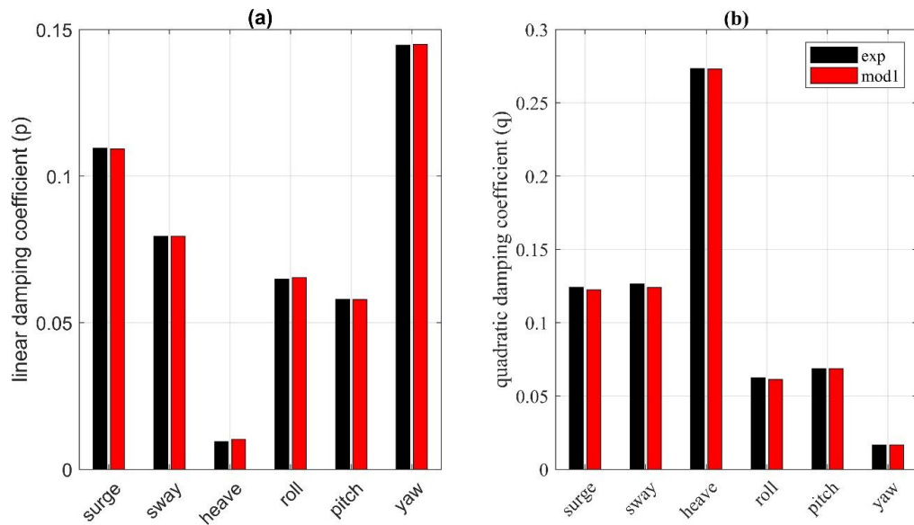
Figure 4.12: Linear and quadratic damping coefficients after calibration.
