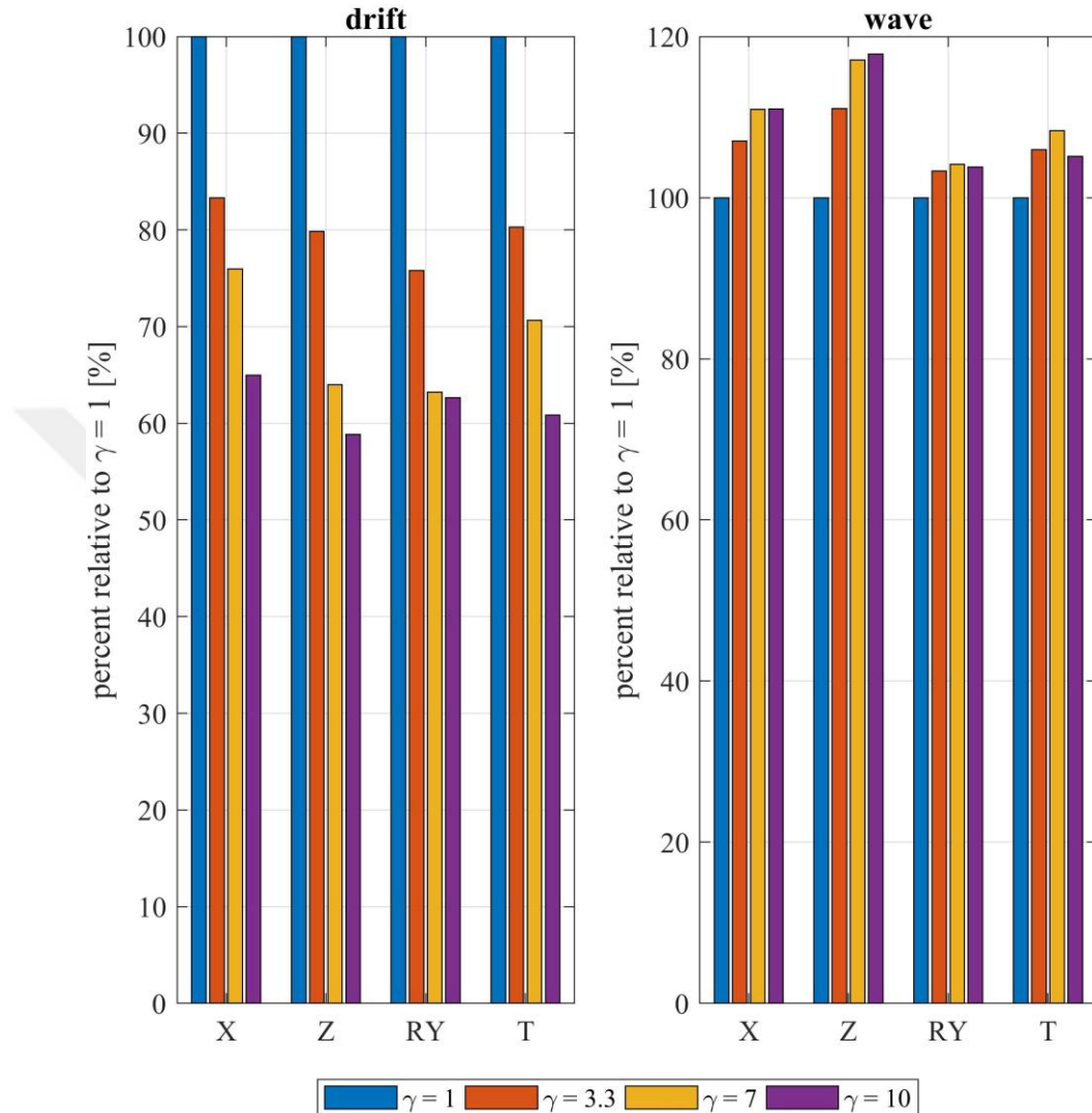
Figure 4.30: Percent change of drift and wave amplitudes in different spectral shape cases relative to the spectrum case with \gamma=1.0 (moderate case).
