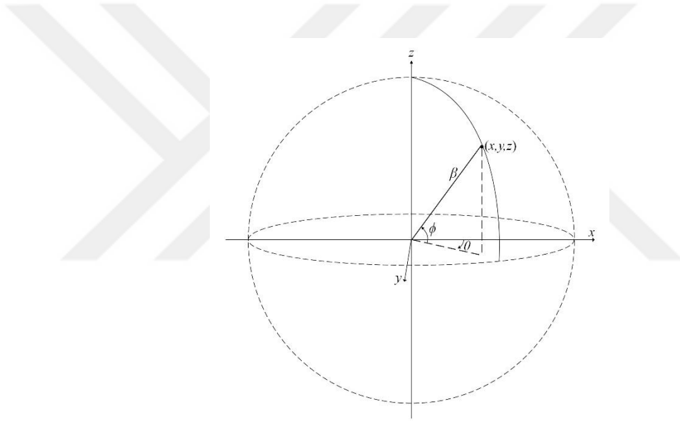
Figure A.5: Standard normal space sphere.
