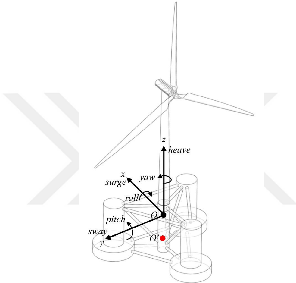
Figure 3.1: DoF conventions with the first convention of the origin point being deployed here.
