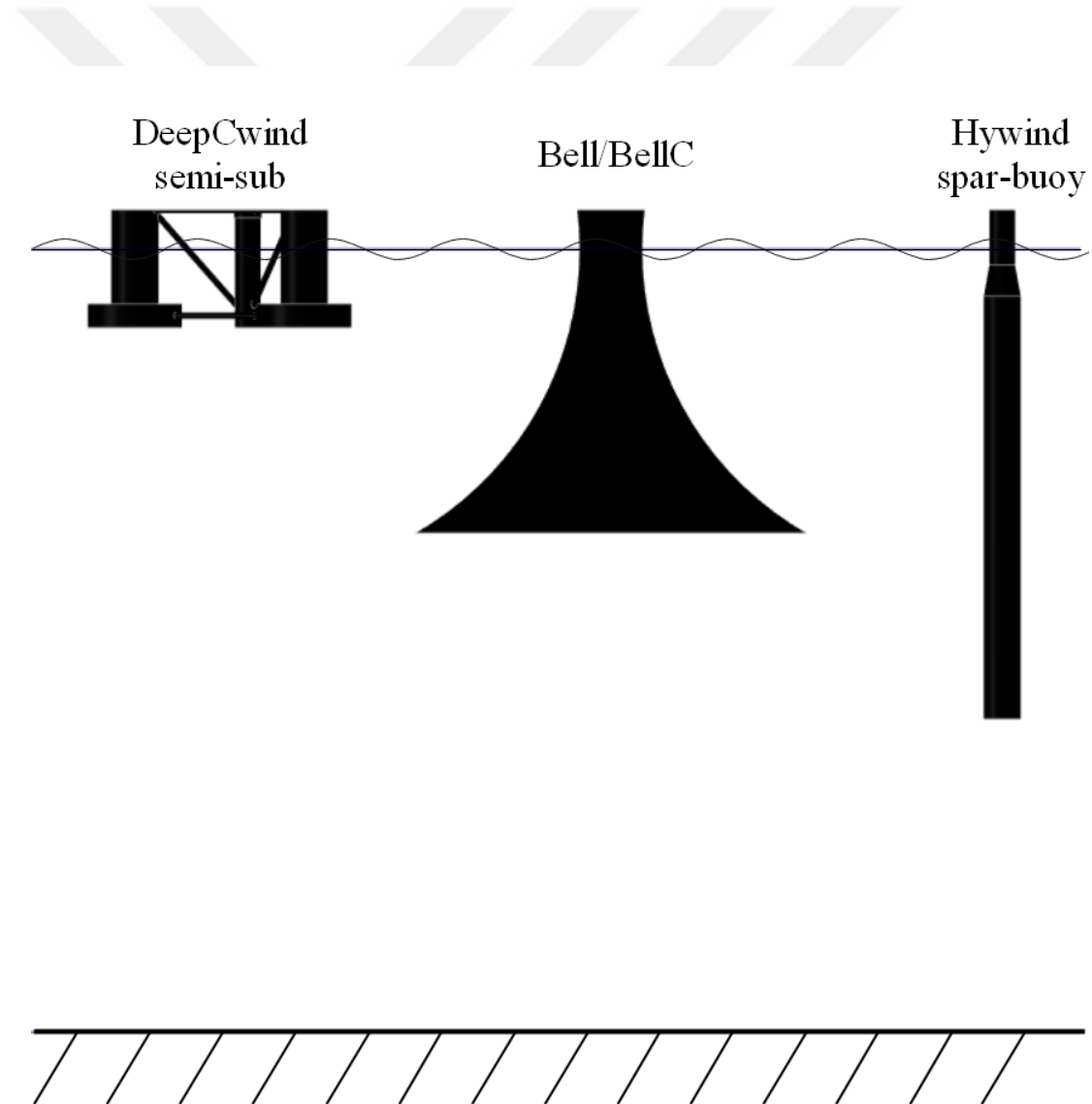
Figure 7.1: Configuration of platforms to be contrasted.
