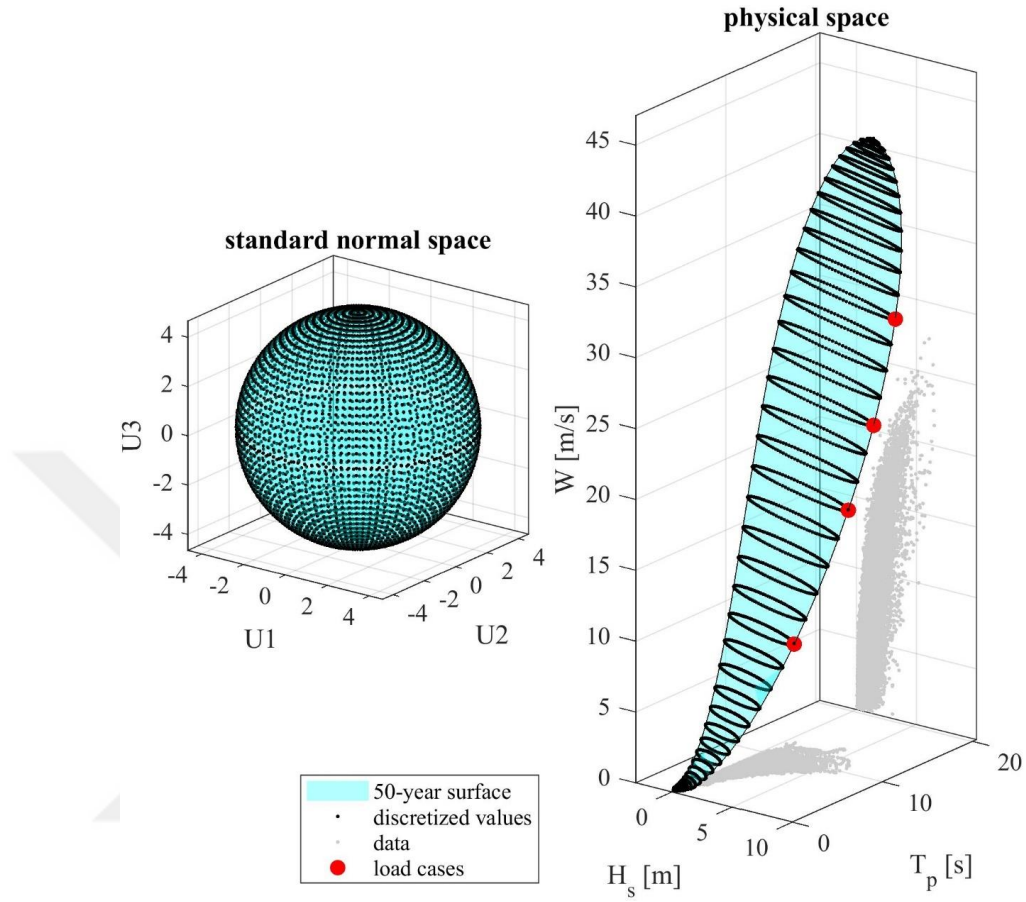
Figure 5.4: Transformation from the standard normal space to the physical space and the load cases' location at the 50-year contour surface.
