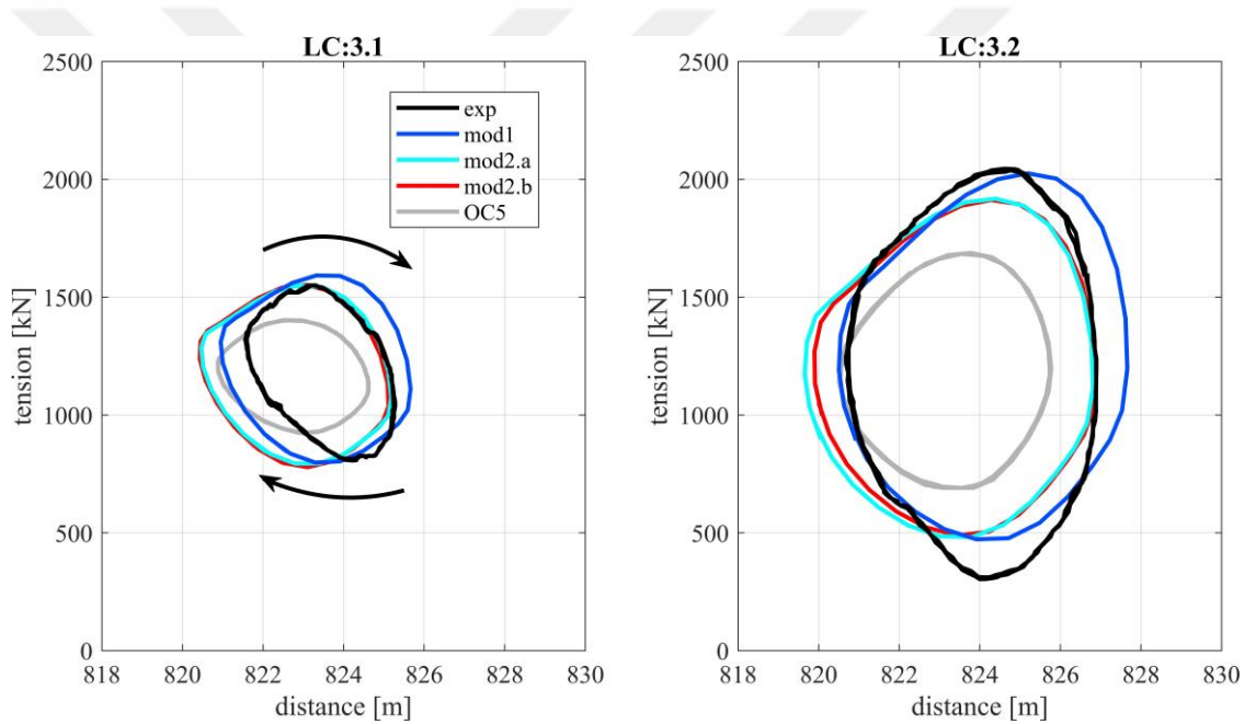
Figure 4.16: Motion-tension relation under moderate and extreme regular wave loading. The x-axis is the distance from anchor to fairlead.
