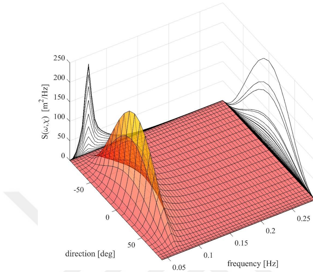
Figure 4.33: Multidirectional wave spectrum as a function of frequency and direction for a mean direction of 0^\circ and a spreading parameter of n = 2 .
