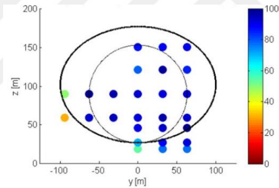
Figure 4.25: Wind velocity as a percentage of the maximum wind velocity.
