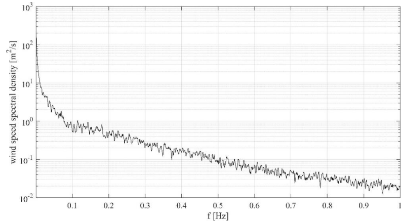
Figure 4.24: Wind energy spectrum.
