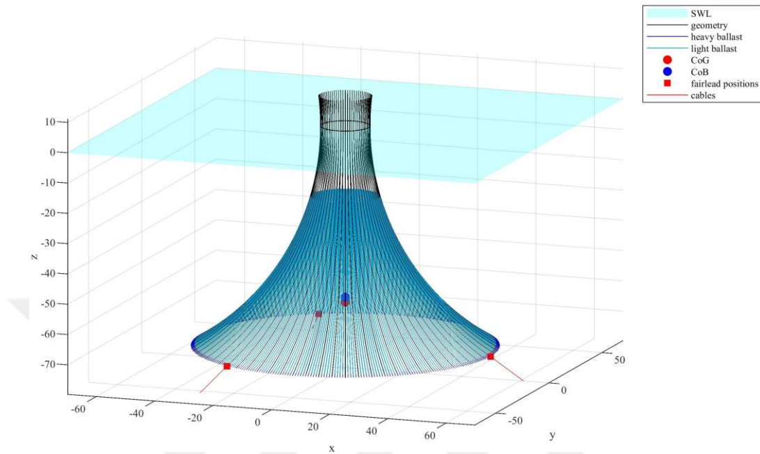
Figure 6.3: Innovative model geometric configuration.
