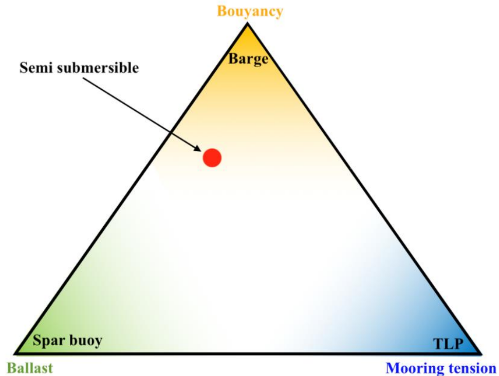
Figure 2.2: Stability triangle showing the representative platform for each method and a hybrid example.
