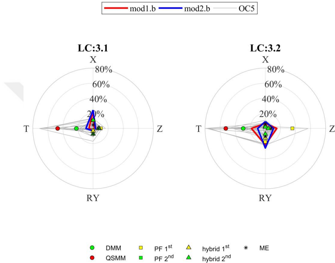
Figure 4.20: RAO response error assessment for regular wave cases in DoF 0 . The radii are the absolute percentage error (APE).
