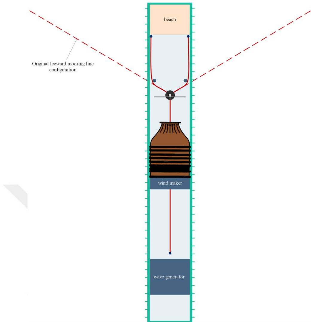
Figure 5.10: Top-view of the wave flume and the original and truncated configuration of the mooring system.
