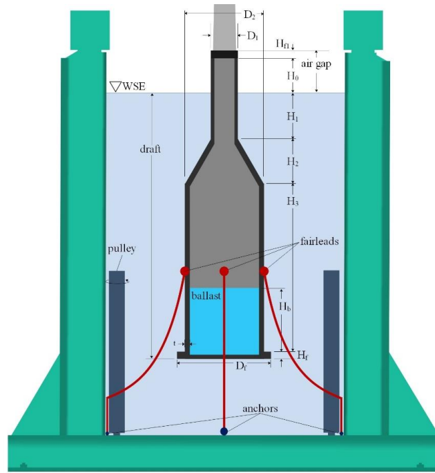
Figure 5.2: Schematic view of the spar-buoy design to be tested (dimensions not to scale).
