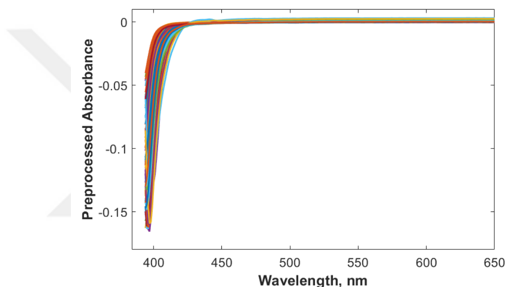
Figure 4.16. Preprocessed UV-Vis Spectra of light diesel samples.
