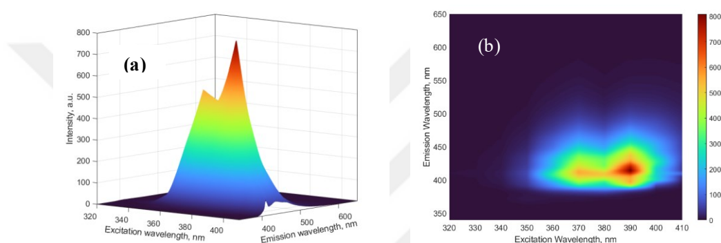
Figure 4.19. Total Fluorescence Spectra of light diesel sample with lowest API value (a) 3D topographical diagram (b) contour map.
