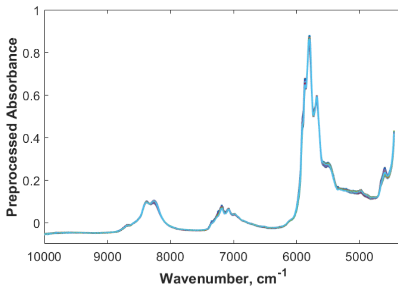
Figure 4.14. Preprocessed FT-NIR spectra of light diesel samples.
