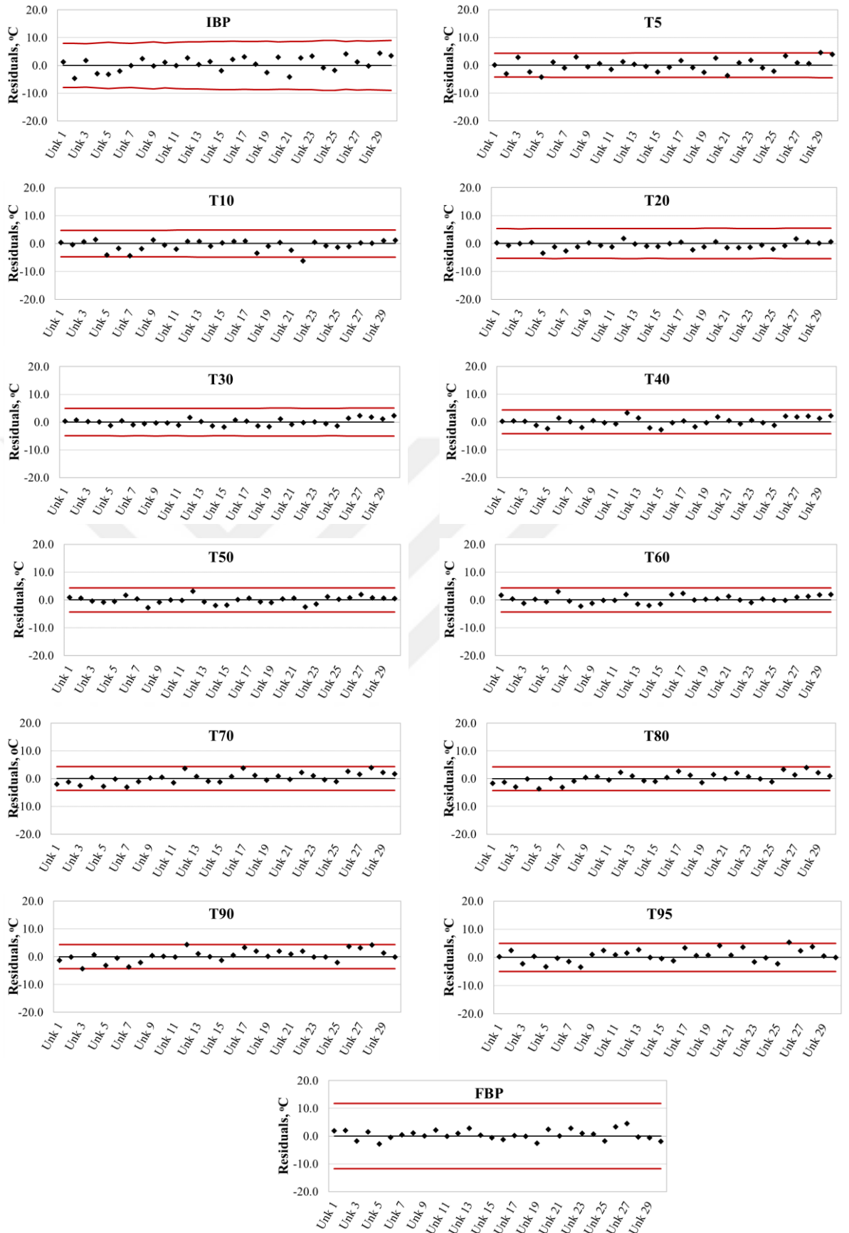
Figure 4.8. Residual graphs of 30 unknown samples from selected models for distillation points.
