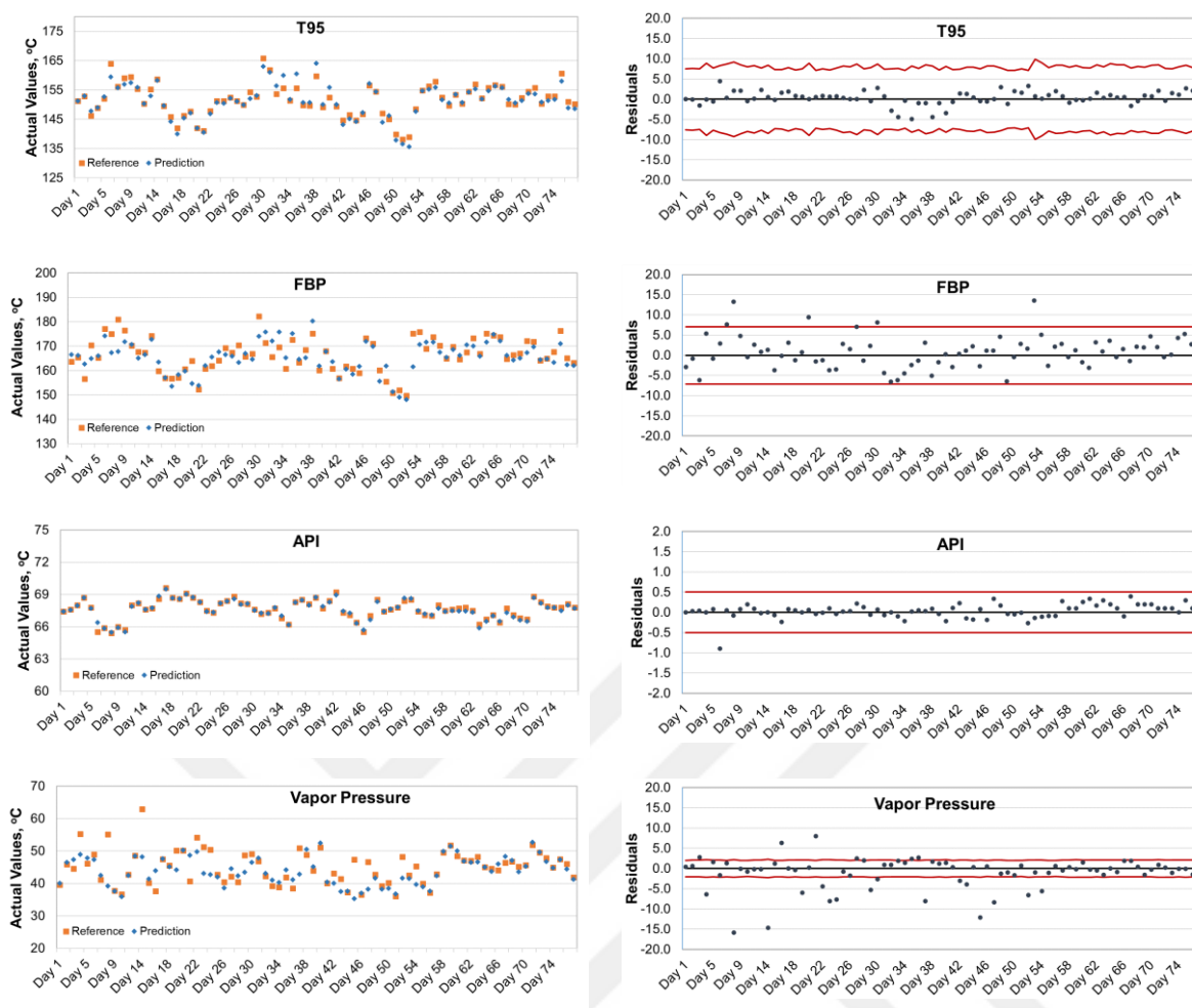
Figure 4.32. Model predictions of LSRN samples belongs to İzmir Refinery (cont'd).
