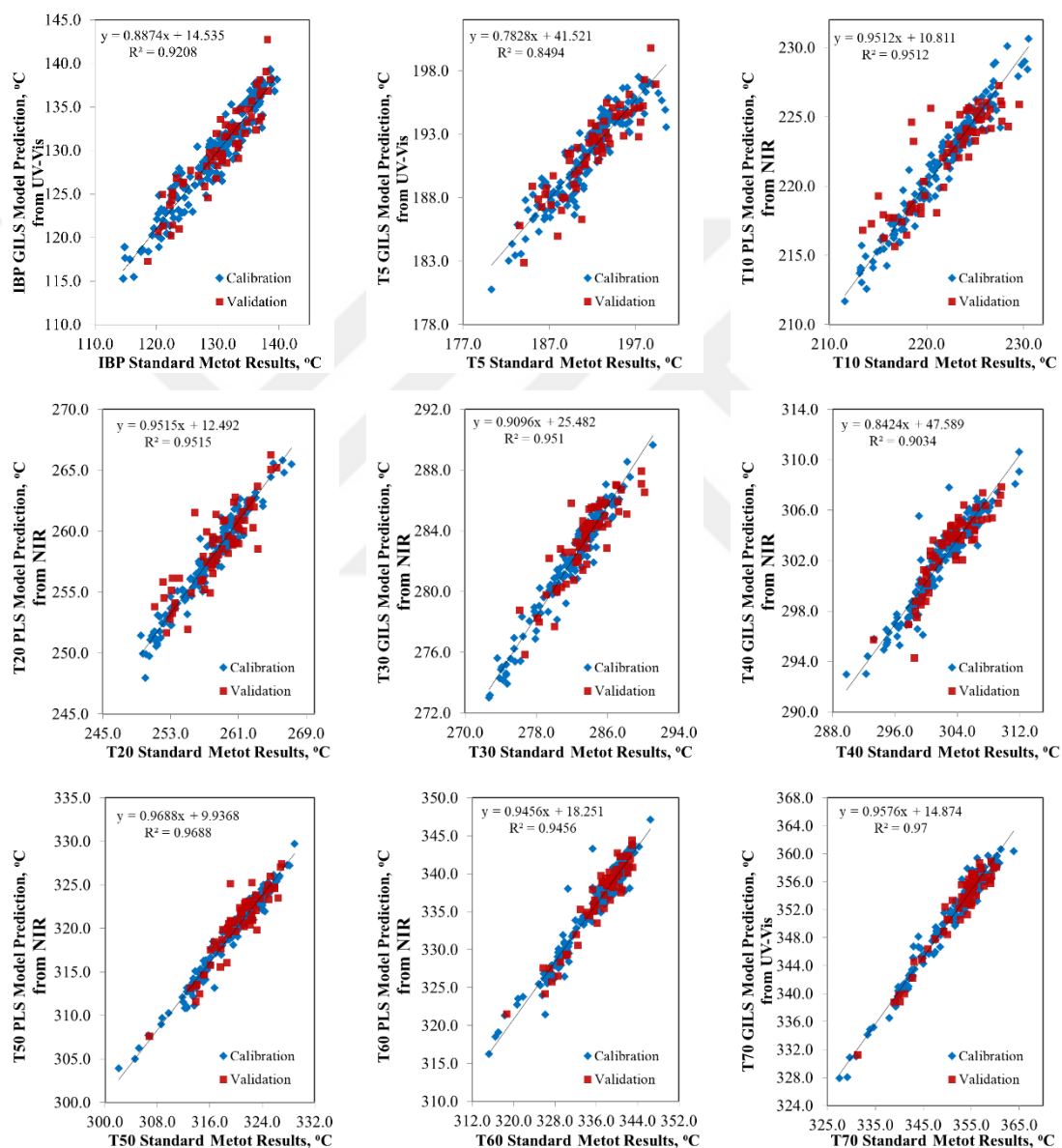
Figure 4.9. Standard analysis vs model prediction results obtained from three different spectroscopic analysis.
