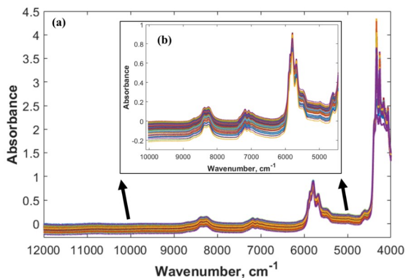
Figure 4.4. Raw FT-NIR Spectra of a total of 268 CDU heavy diesel samples (a) full range (b) narrowed range
