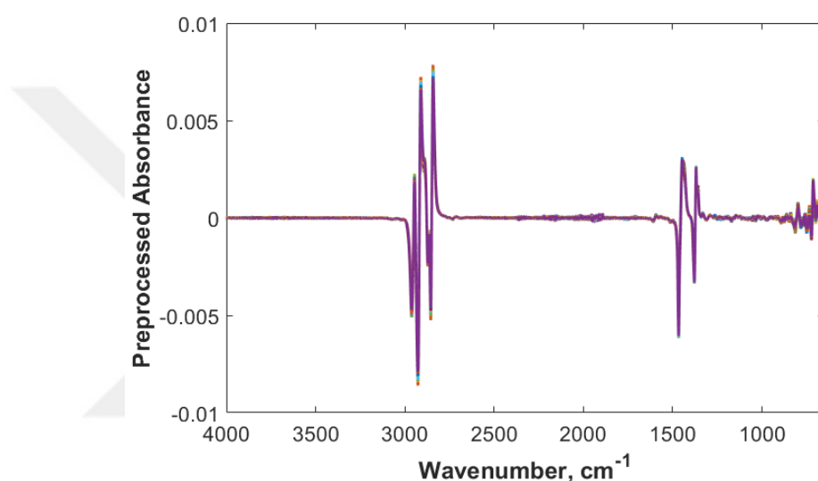
Figure 4.3. FTIR-ATR Spectra of heavy diesel samples treated by first derivative using first order polynomial and a window size of eleven followed by MSC.
