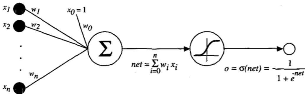
Figure 3.2: A sigmoid [1]
