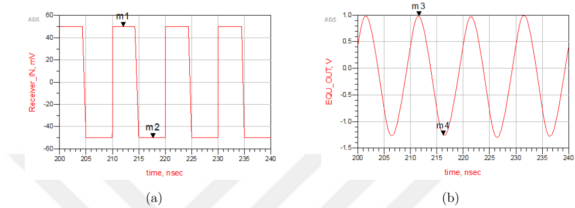
Figure 3.23. (a) Square wave input of the Discrete Receiver System at 100 MHz, (b) Output response of the Discrete Receiver System at 100 MHz.
