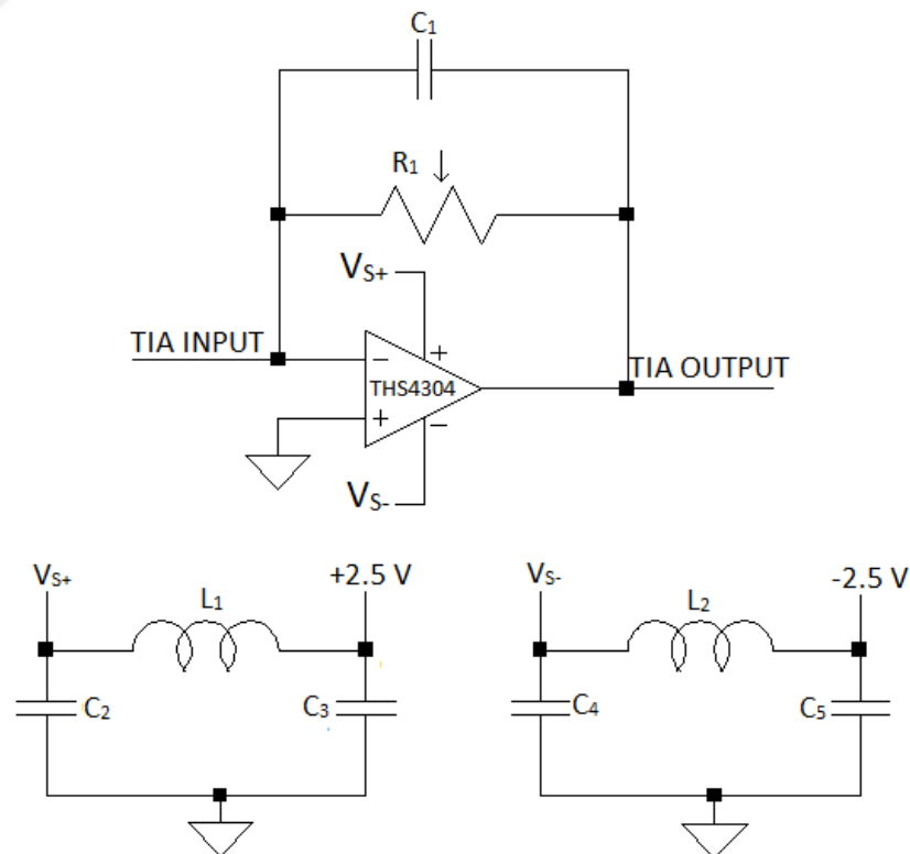
Figure 3.1. Circuit schematic of TIA.
