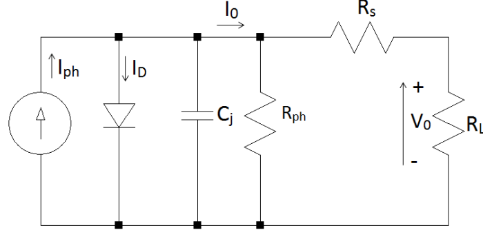
Figure 2.3. Equivalent circuit for a silicon photodiode [3].
