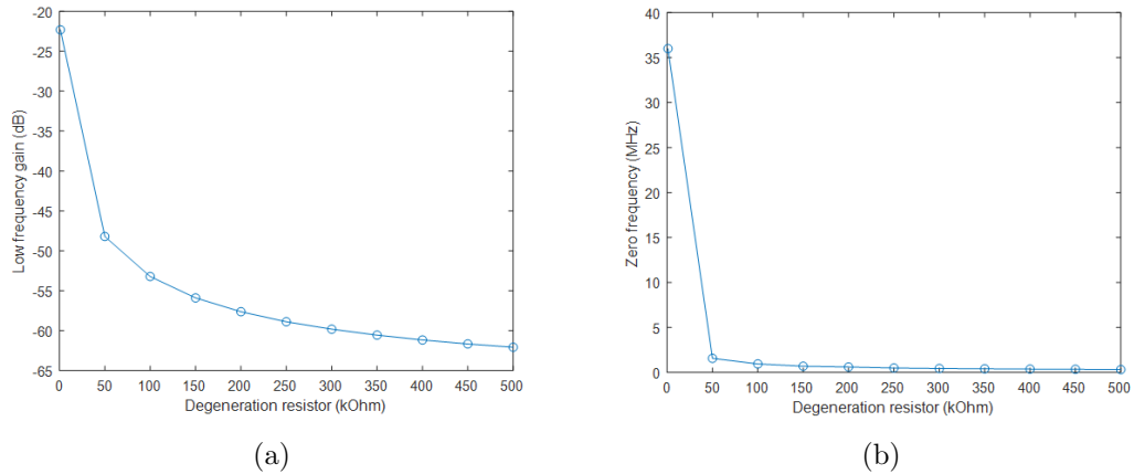
Figure 4.11. (a) Degeneration resistor versus low frequency gain, (b) Degeneration resistor versus zero frequency.
