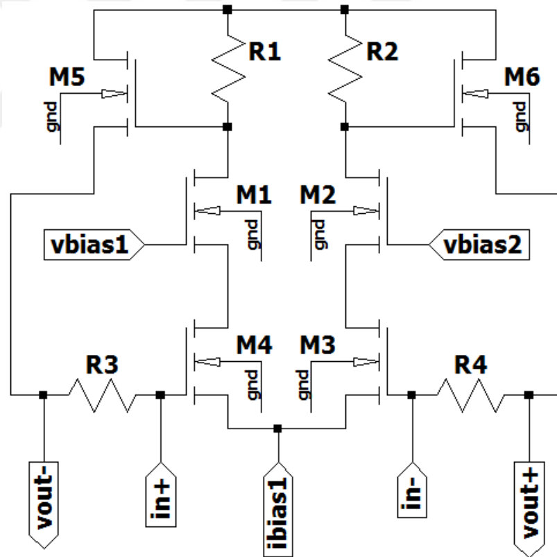
Figure 4.3. Schematic of CMOS TIA circuit.
