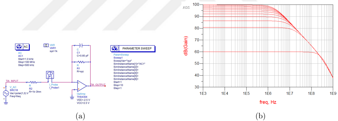
Figure 3.2. (a) Circuit schematic utilized for sweep analysis, (b) Effect of feedback resistance on 3-dB gain and 3-dB frequency.
