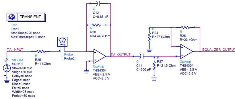
Figure 3.21. Circuit schematic of the Discrete Receiver System for transient simulation.
