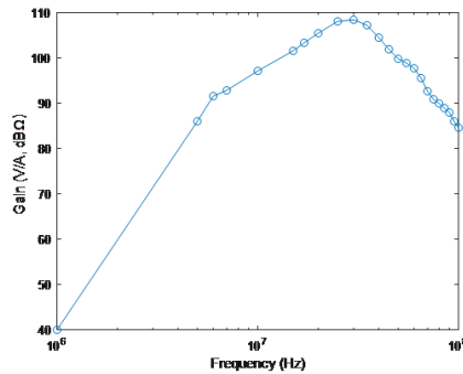
Figure 3.30. Frequency Response of the Discrete Receiver System.
