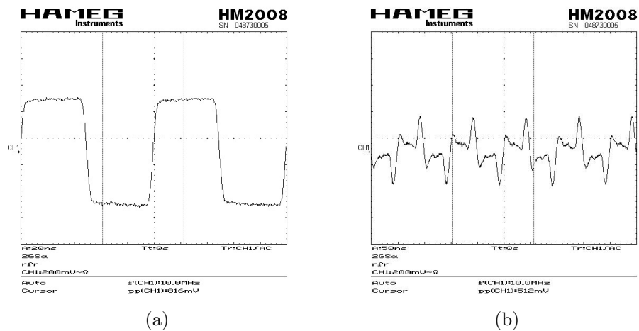
Figure 3.32. (a) Square wave input of the Discrete Receiver System at 10 MHz, (b) Output response of the Discrete Receiver System at 10 MHz.
