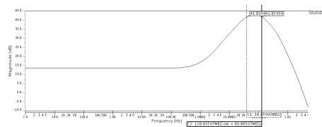
Figure 4.36. AC simulation result of the CMOS Receiver System using 2 pF photodiode junction capacitance.
