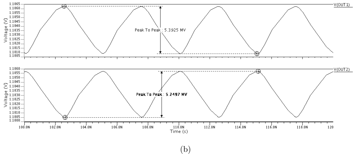
Figure 4.39. (a) Square wave input of the Integrated CMOS Receiver System at 200 MHz using 2 pF photodiode junction capacitance, (b) Square wave outputs of the Integrated CMOS Receiver System at 200 MHz using 2 pF photodiode junction capacitance.
