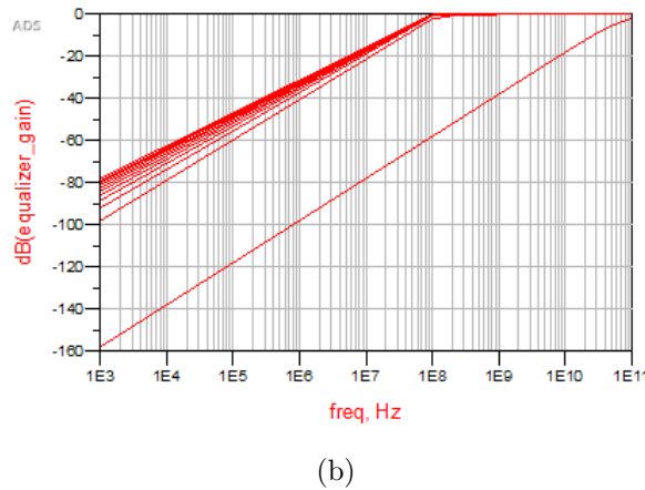
Figure 3.6. (a) Circuit schematic utilized for sweep analysis, (b) Effect of equalizer resistance on cutoff frequency.
