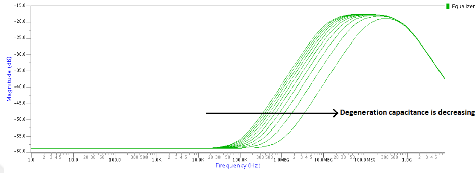
Figure 4.12. Effect of the degeneration capacitor on the first pole frequency and zero frequency.
