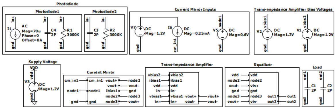
Figure 4.17. Schematic of receiver circuit.
