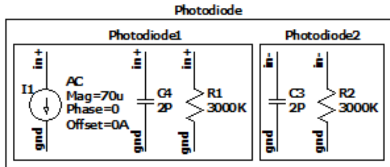
Figure 4.2. Schematic of the equivalents for two types of photodiodes used for simulation.
