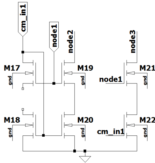
Figure 4.9. Schematic of low voltage current mirror.
