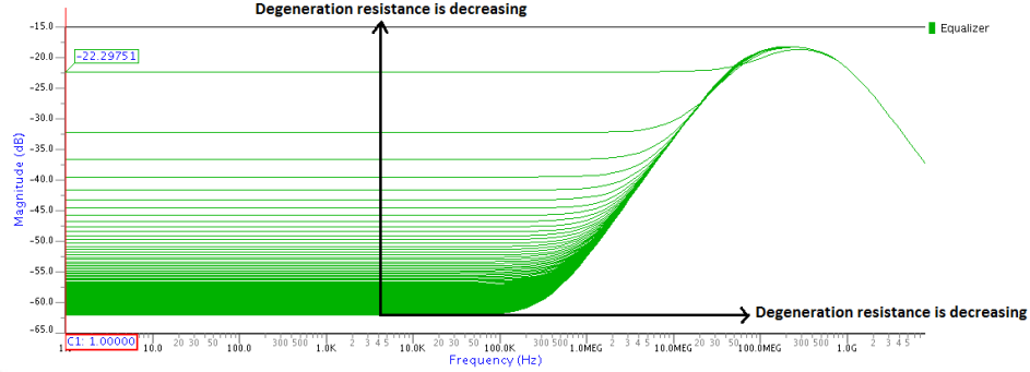
Figure 4.10. Effect of degeneration resistor on low frequency gain and zero frequency.
