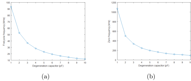
Figure 4.13. (a) Degeneration capacitor versus first pole frequency, (b) Degeneration capacitor versus zero frequency.
