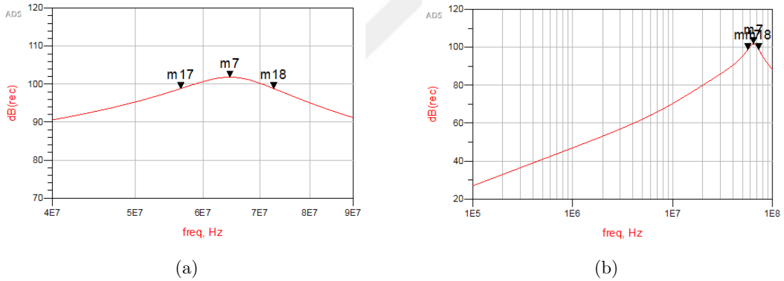
Figure 3.18. (a) Frequency response of the Discrete Receiver System (zoomed in), (b) Frequency response of the Discrete Receiver System (fully viewed).
