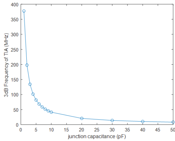
Figure 4.6. Junction capacitance of photodiode versus 3-dB frequency of TIA.
