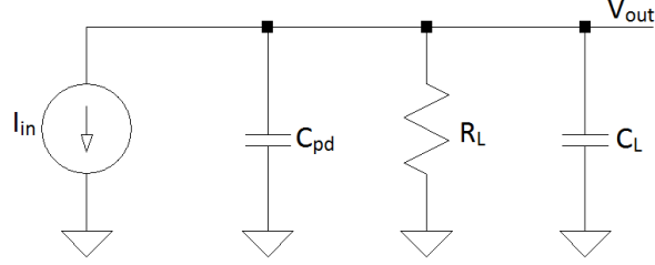
Figure 2.11. Single resistor trans-impedance circuitry in which photodiode model is used [5].
