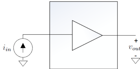
Figure 2.9. Trans-impedance amplifier.
