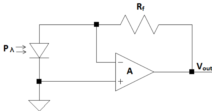
Figure 2.6. Circuit for zero bias operation [4]
