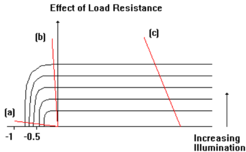
Figure 2.8. Load resistance effect on current/voltage characteristics [4].
