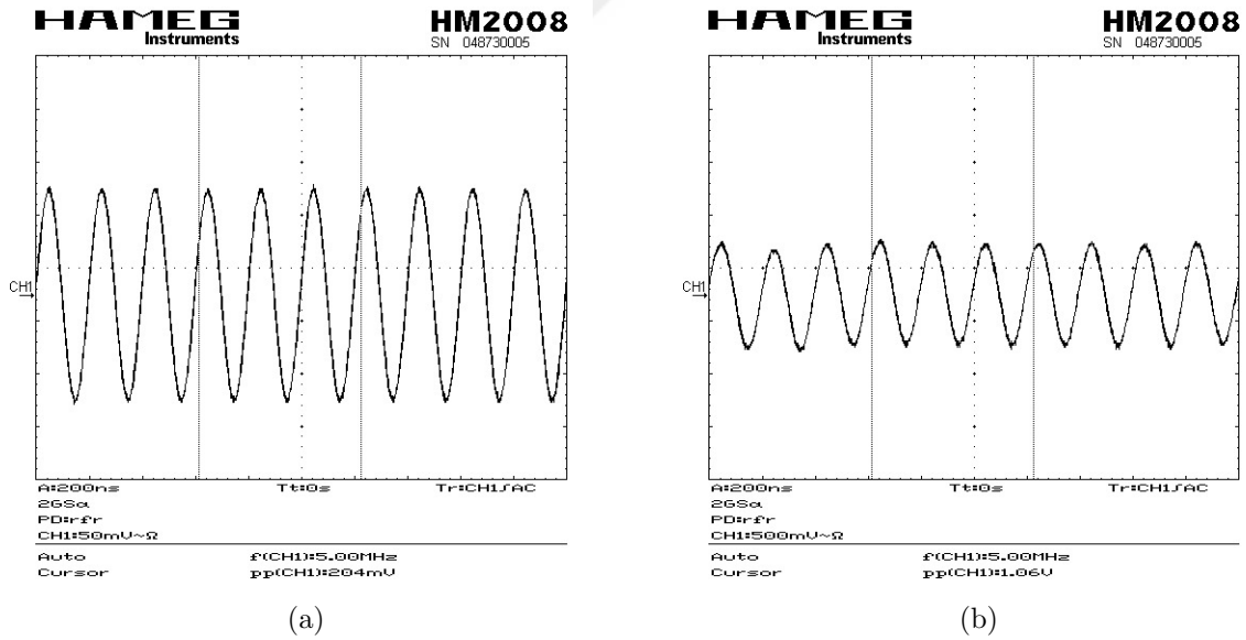
Figure 3.27. (a) Sinusoidal input of the TIA at 5 MHz, (b) Sinusoidal output of the TIA at 5 MHz.
