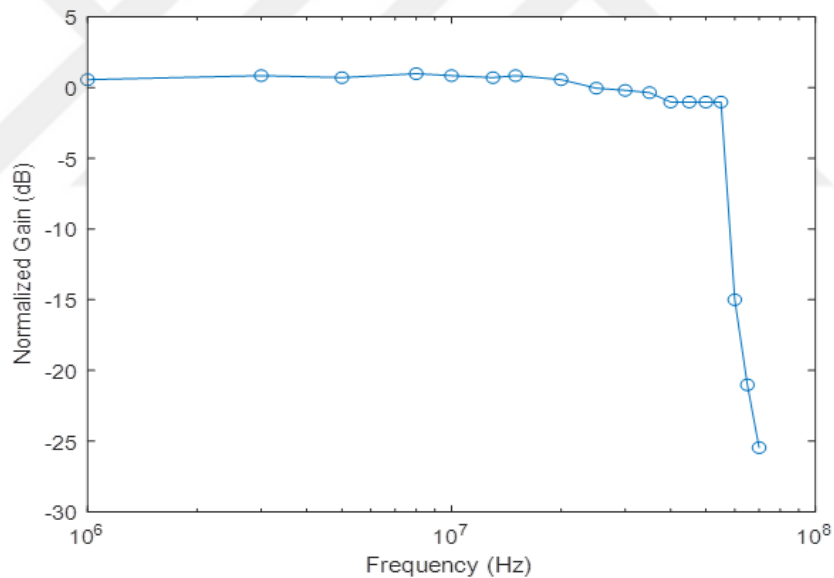
Figure 3.34. Frequency response of the Discrete Receiver System with visible light communication.
