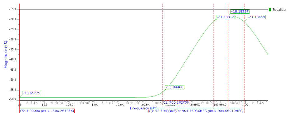
Figure 4.27. AC simulation result of the Equalizer.
