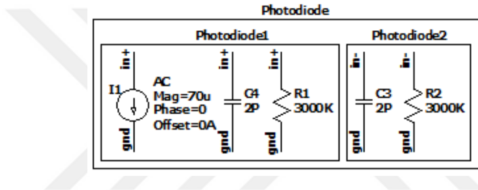
Figure 4.19. Photodiode Testbench.
