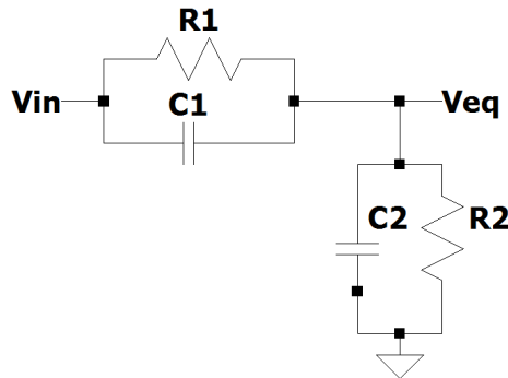
Figure 2.16. Passive CTLE circuit [7].
