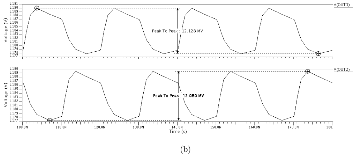
Figure 4.38. (a) Square wave input of the Integrated CMOS Receiver System at 50 MHz using 2 pF photodiode junction capacitance, (b) Square wave outputs of the Integrated CMOS Receiver System at 50 MHz using 2 pF photodiode junction capacitance.
