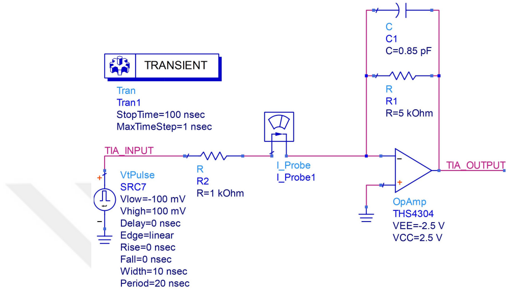
Figure 3.13. Circuit Schematic of the TIA for Transient simulation.
