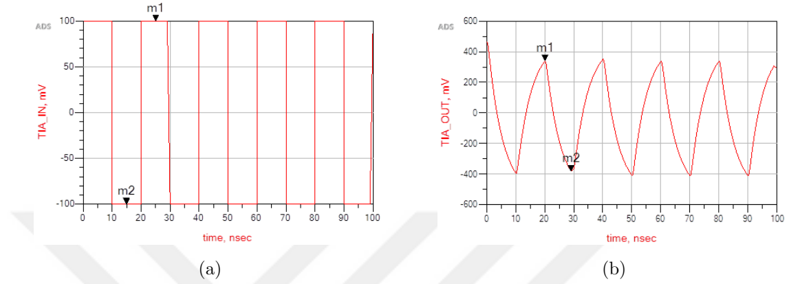
Figure 3.15. (a) Square wave input at 50 MHz, (b) Output response of the TIA at 50 MHz.
