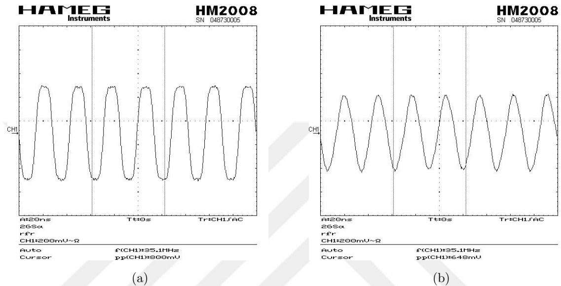
Figure 3.33. (a) Square wave input of the Discrete Receiver System at 35 MHz, (b) Output response of the Discrete Receiver System at 35 MHz.
