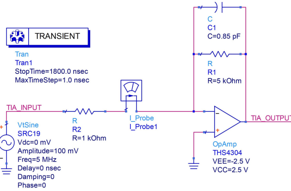
Figure 3.11. Circuit Schematic of the TIA for transient simulation.
