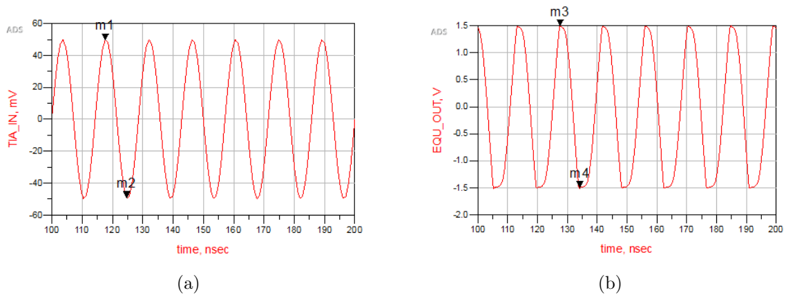
Figure 3.20. (a) Sinusoidal input of the Discrete Receiver System at 70 MHz, (b) Sinusoidal output of the Discrete Receiver System at 70 MHz.
