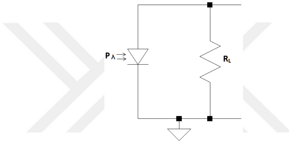
Figure 2.5. Circuit for photovoltaic operation [4].
