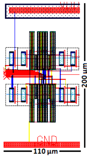
Figure 4.7. Layout of trans-impedance amplifier.
