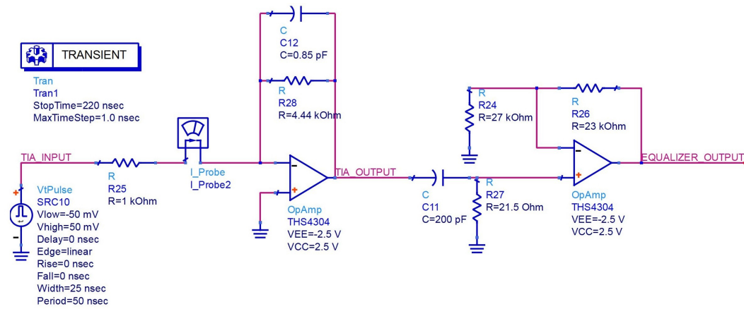
Figure 3.19. Circuit schematic of the Discrete Receiver System for transient simulation.
