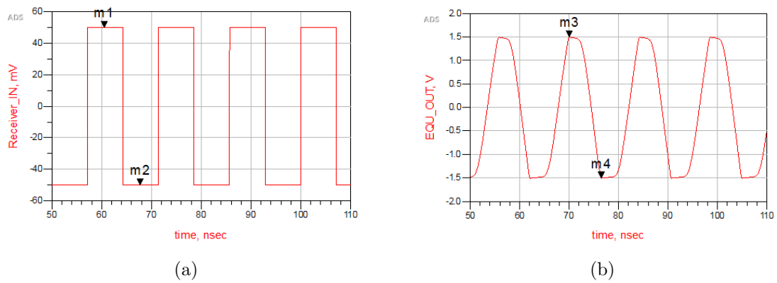
Figure 3.22. (a) Square wave input of the Discrete Receiver System at 70 MHz, (b) Output response of the Discrete Receiver System at 70 MHz.
