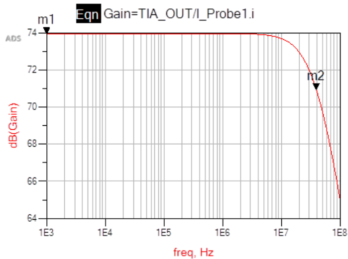
Figure 3.10. Frequency Response of the TIA.
