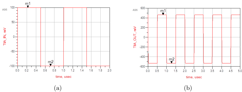
Figure 3.14. (a) Square wave input at 1 MHz, (b) Output response of the TIA at 1 MHz.
