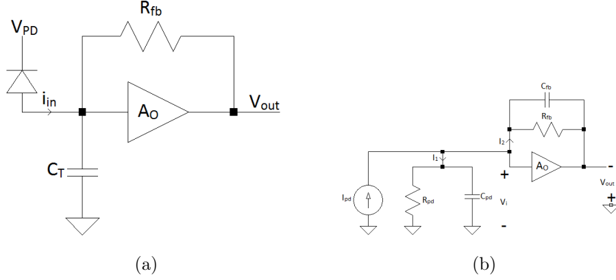
Figure 2.14. (a) Basic circuit of shunt feedback TIA, (b) TIA circuitry with photodiode model [5], [6].
