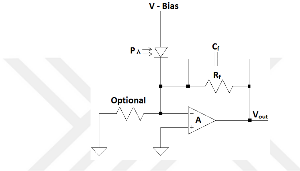
Figure 2.7. Circuit for photoconductive operation [4]
