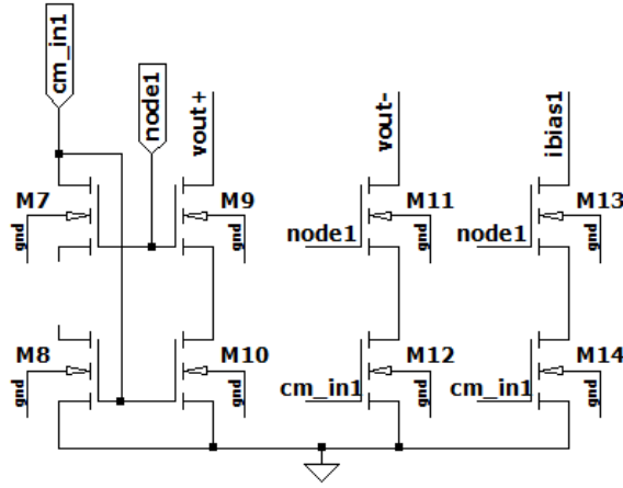
Figure 4.5. Schematic of low voltage current mirror.
