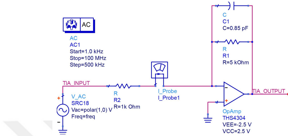
Figure 3.9. Circuit schematic of the TIA for AC simulation.
