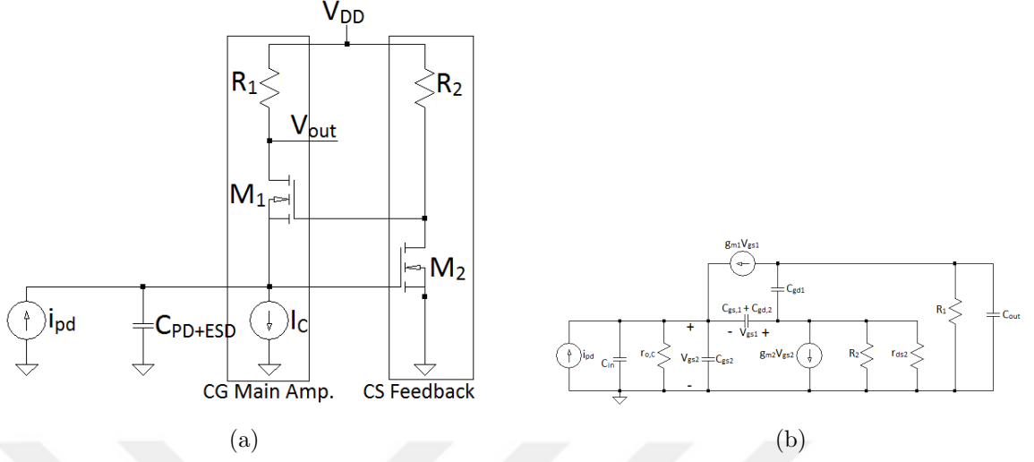
Figure 2.13. (a) Regulated cascode TIA circuitry, (b) Small-signal model of regulated cascode TIA [5].
