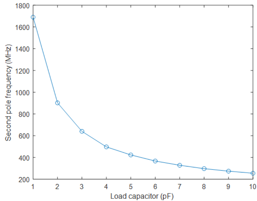
Figure 4.15. Load capacitance versus second pole frequency.
