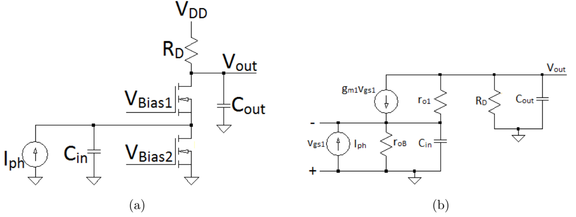
Figure 2.12. (a) CG-TIA circuitry, (b) Small-signal model of CG-TIA [5], [6].
