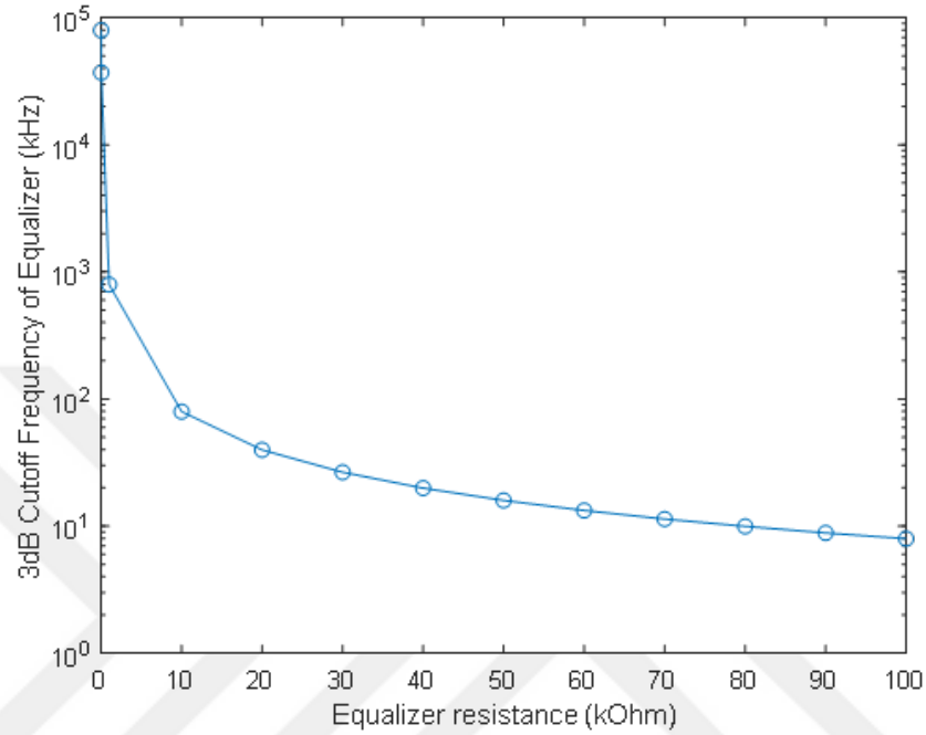
Figure 3.7. Equalizer resistance versus 3-dB Cutoff frequency.
