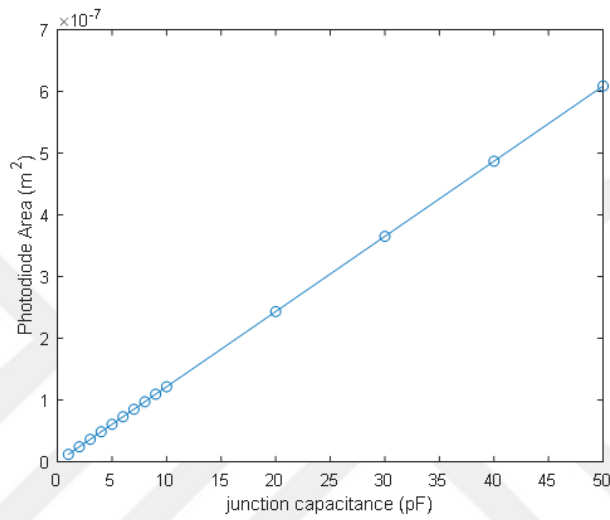
Figure 4.1. Photodiode junction capacitance versus photodiode area.
