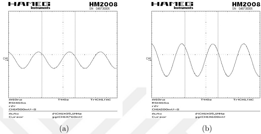
Figure 3.31. (a) Sinusoidal input of the Discrete Receiver System at 35 MHz, (b) Sinusoidal output of the Discrete Receiver System at 35 MHz.
