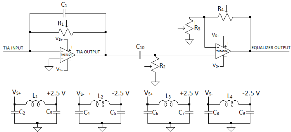
Figure 3.5. Circuit schematic of the Discrete Receiver System.
