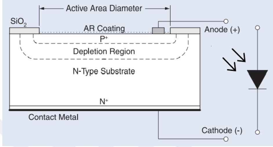
Figure 2.4. Planar diffused silicon photodiode [3].
