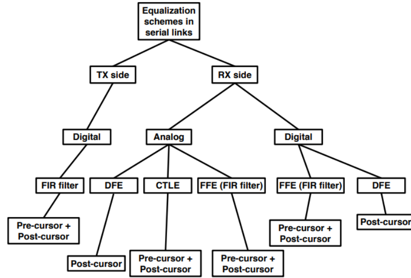
Figure 2.15. Equalizer methods utilized in high speed links [2]
