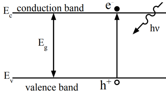
Figure 2.1. Energy diagram [1].
