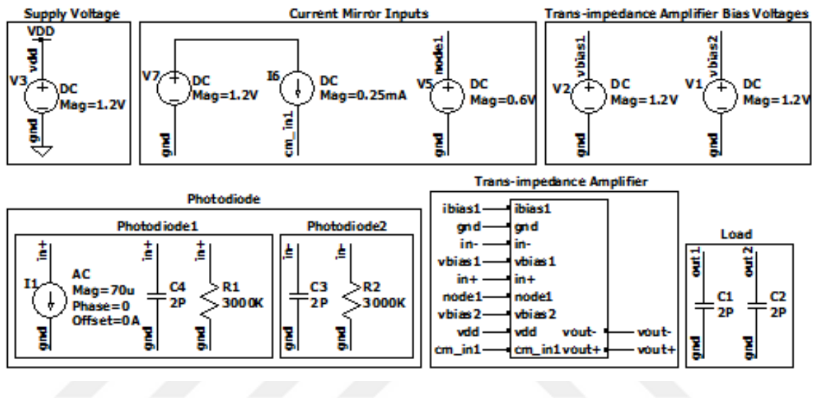
Figure 4.26. Test bench of the Equalizer for the AC simulation
