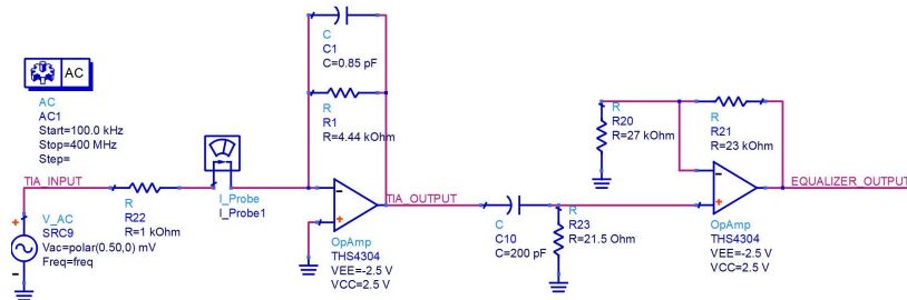
Figure 3.17. Circuit Schematic of the Discrete Receiver System for AC simulation.
