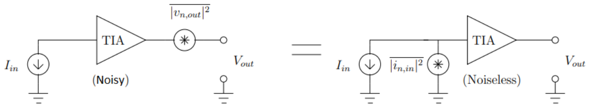
Figure 2.10. Input referred noise current.
