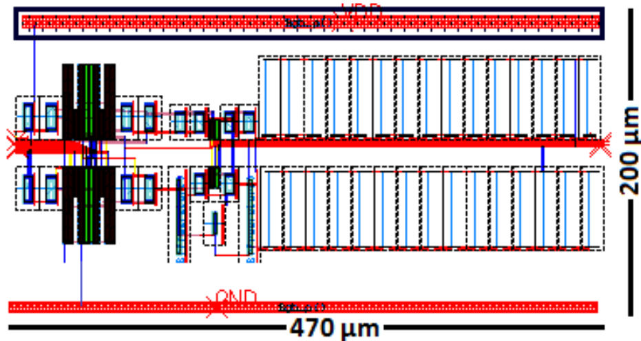
Figure 4.18. Layout of receiver circuit.
