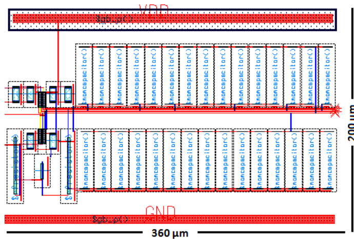
Figure 4.16. Layout of Equalizer circuit.
