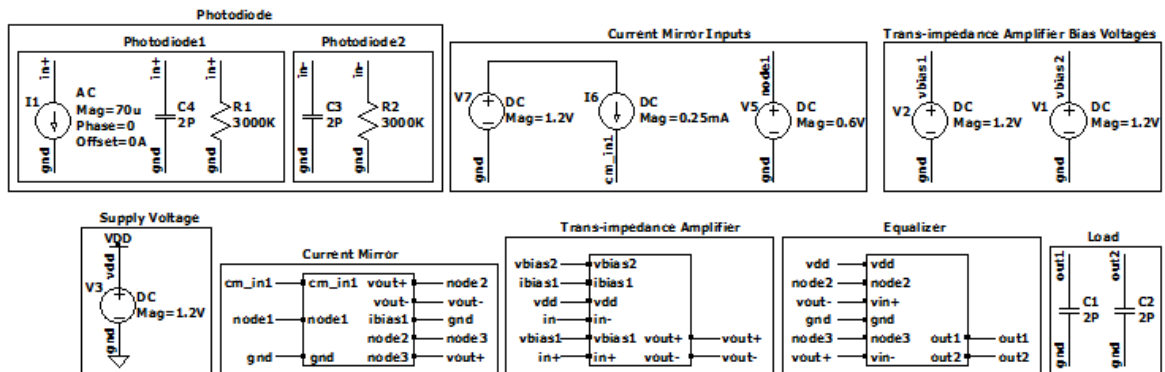
Figure 4.31. Schematic of receiver circuit.
