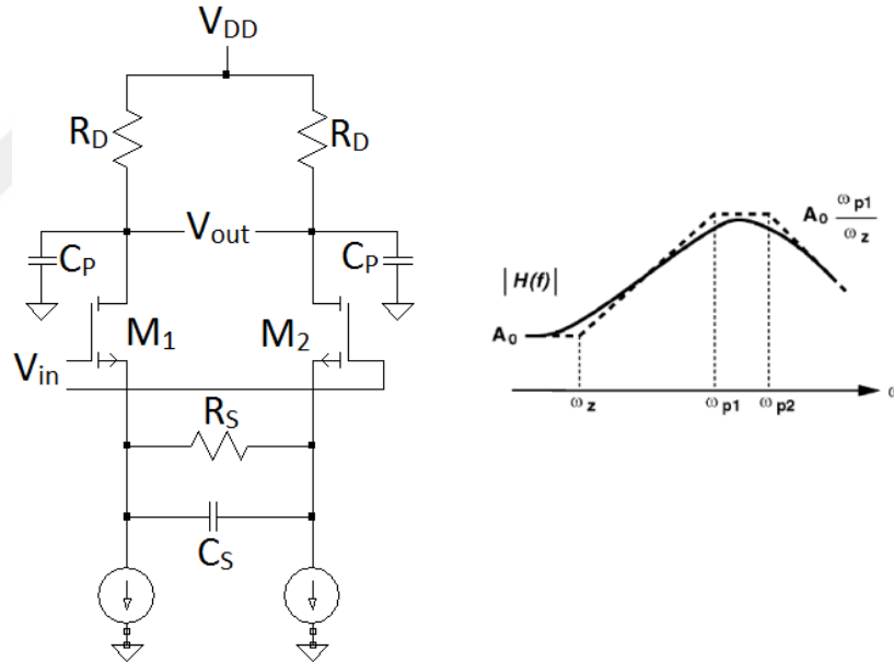
Figure 2.17. Active CTLE circuit [8].
