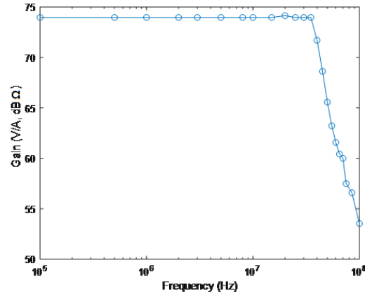
Figure 3.26. Frequency Response of the TIA.
