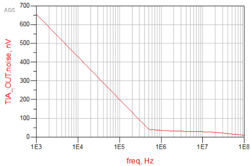
Figure 3.16. The output noise density of the discrete TIA.
