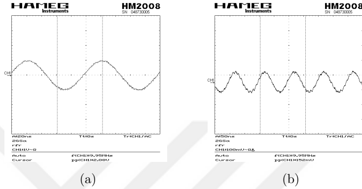
Figure 3.35. (a) Sinusoidal input of the Discrete Receiver System with visible light communication at 10 MHz, (b) Sinusoidal output of the Discrete Receiver System with visible light communication at 10 MHz.
