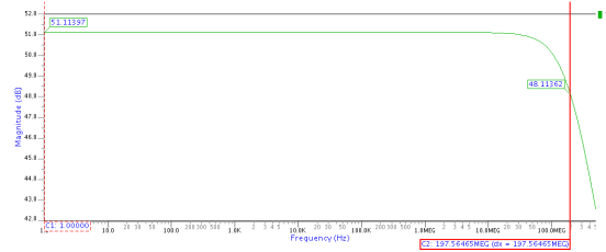
Figure 4.21. AC simulation result of the TIA obtained using 2 pF photodiode junction capacitance.
