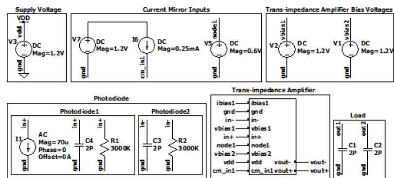
Figure 4.20. Test bench of the TIA for the AC simulation.
