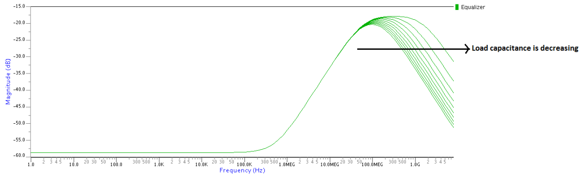
Figure 4.14. Effect of the load capacitor on the second pole frequency.
