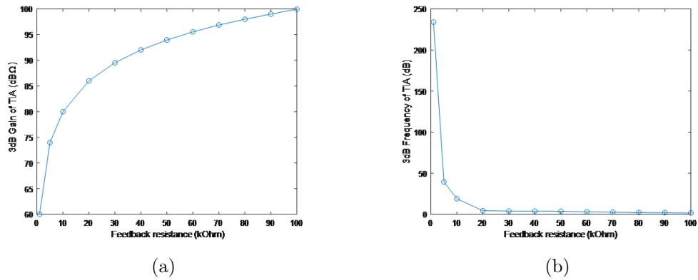
Figure 3.3. (a) Feedback resistance versus 3-dB gain, (b) Feedback resistance versus 3-dB frequency.
