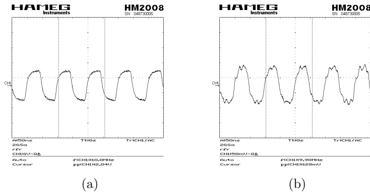
Figure 3.36. (a) Square wave input of the Discrete Receiver System with visible light communication at 10 MHz, (b) Output response of the Discrete Receiver System with visible light communication at 10 MHz.
