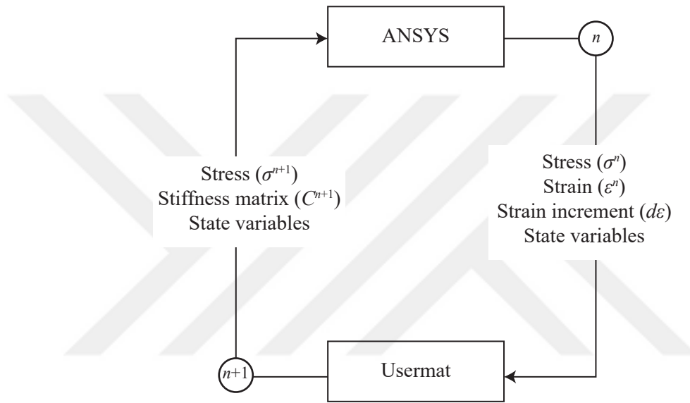
Figure 5.12: ANSYS-Usermat working scheme
