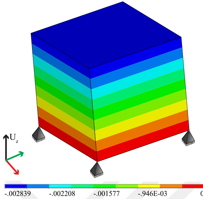
Figure 5.8: Displacement at the end of the first cycle, \Delta q = 237 \text{ kPa}
