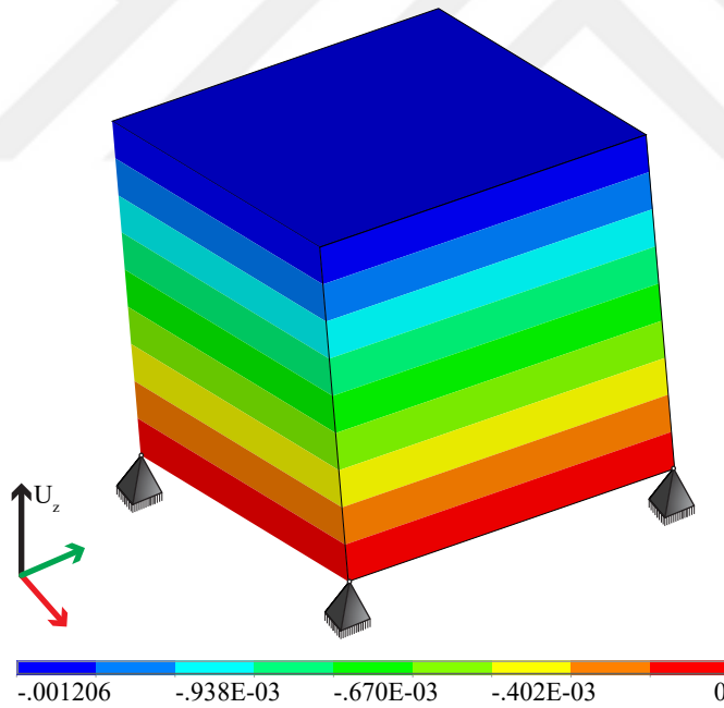
Figure 5.9: Displacement at the end of the first cycle, \Delta q = 153 \text{ kPa}
