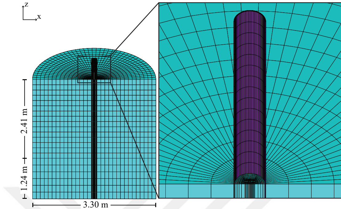
Figure 5.19: 3D meshed model of design
