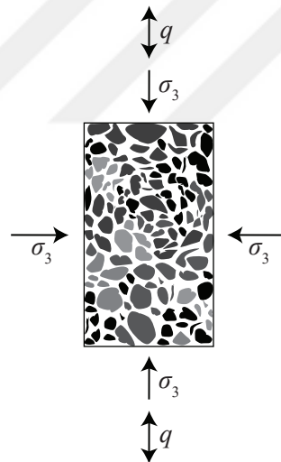
Figure 5.6: Cyclic triaxial test scheme
