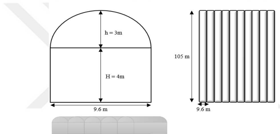
Figure 3.8. Dimensions And Schematic View of The Sample Greenhouse Design
