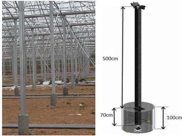
Figure 3.3. Columns of Sample Greenhouse Design (Courtesy of Emre İçöz)
