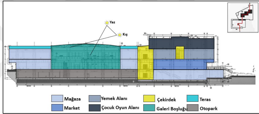
Şekil 5. 63 Mall of Mitrovica kesiti (ODA Architects, 2022)
