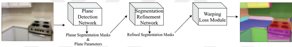
Figure 1.6.: An illustration of PlaneRCNN architecture. This deep learning framework for piecewise plane segmentation is composed of three components. A plane detection network takes a single RGB image and produces segmentation masks, plane parameters, and a depth map for an entire image. Segmentation refinement network takes estimated instance segmentation masks and refines them by joint optimization. Refined segmentation masks are given to the warping loss module, which aims at enforcing the consistency of reconstructed planes with a neighbor view of the corresponding scene.
