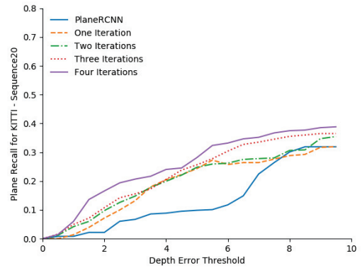
(f) Plane Recall for Sequence 20
