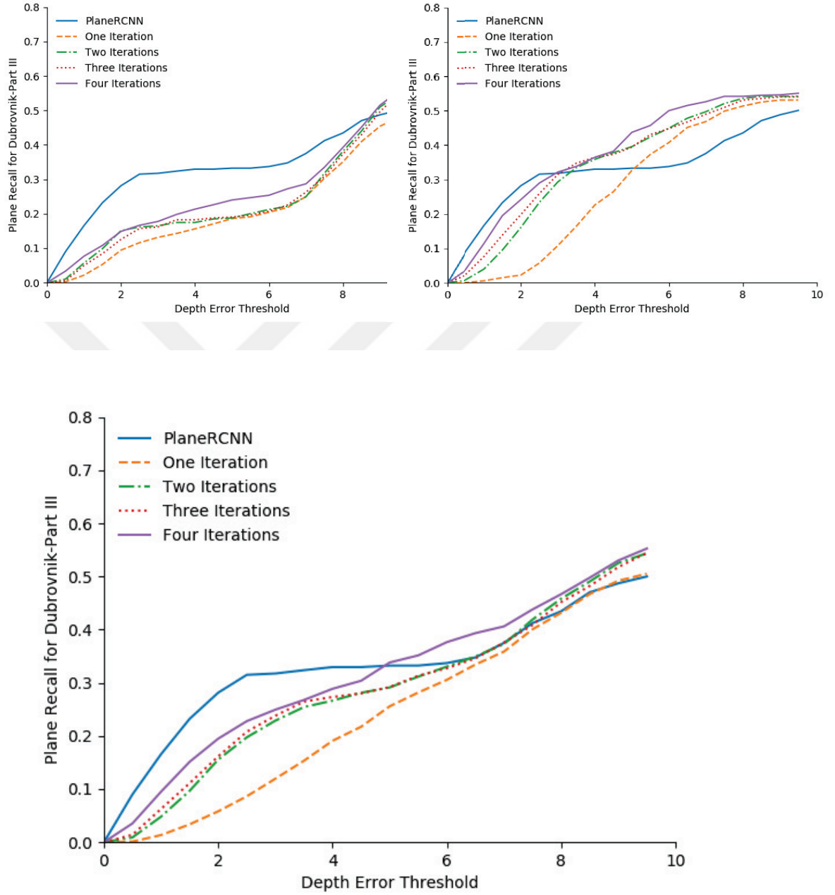
Figure 2.11.: Plane recall for the Part III of Dubrovnik dataset. In the upper row, plane recall for the Part III is illustrated under training of Part II and part I respectively from left to right. Average plane recall for the Part III is shown in the lower row as the number of training iterations is increased.
