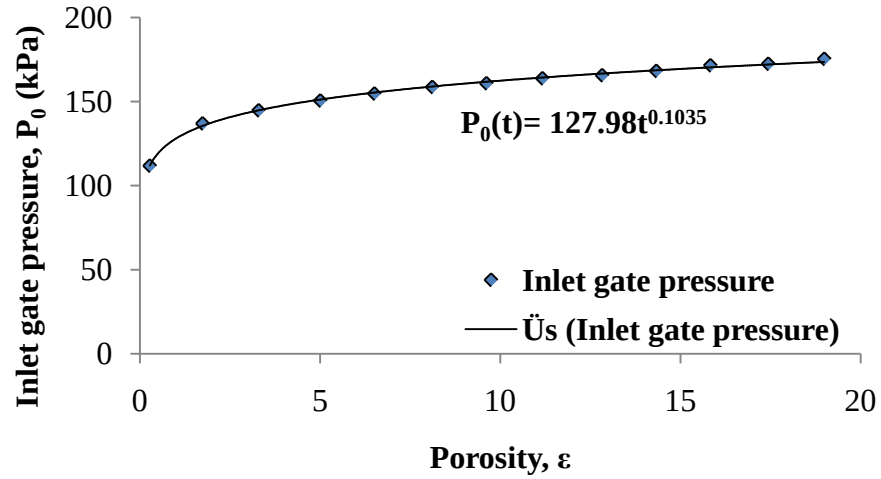
Figure 4.16. Inlet gate pressure distribution obtained from the analytical solution results of Pham and Trochu [1]
