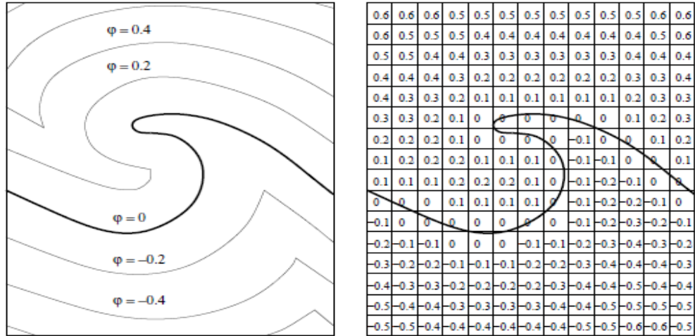
Figure 3.1. Interface definition with level set method (Left: level set contours, Right: level set function values) [54]
