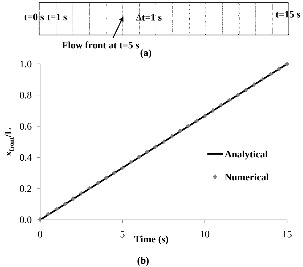
Figure 4.2. a) Flow front positions obtained via COMSOL Multiphysics® ( \Delta t=1\text{ s} ), b) flow front positions of analytical and numerical solutions for during 1-D particle-filled impregnation
