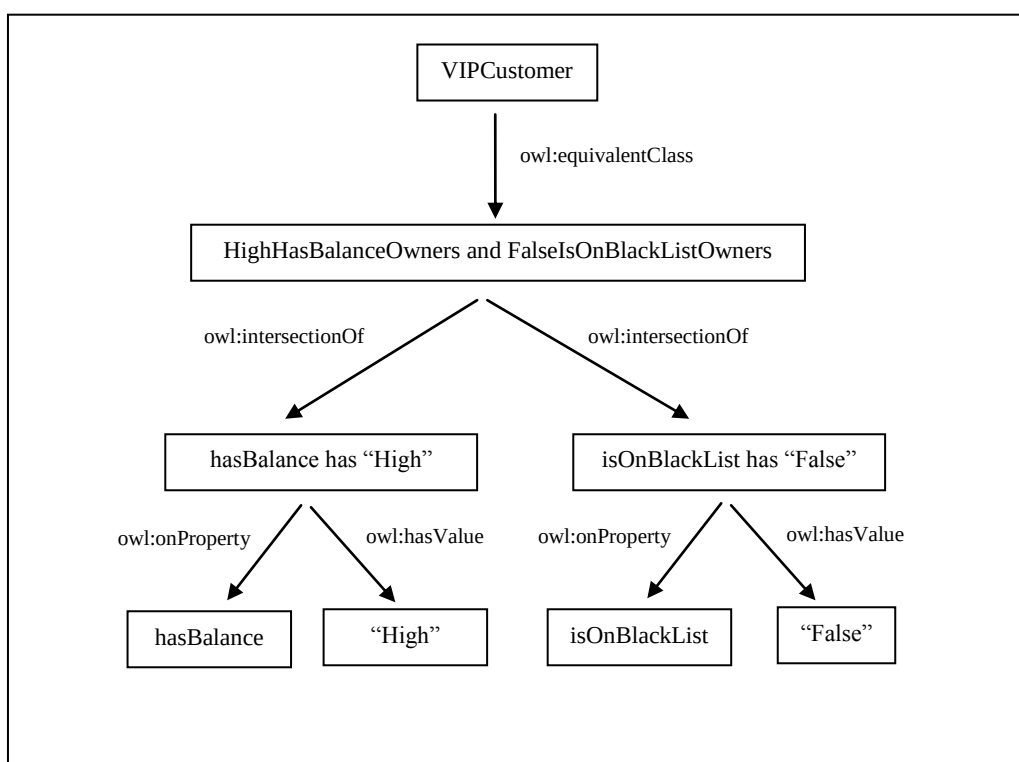
Figure 5.8 RDF-Graph representation of VIPCustomer class.
