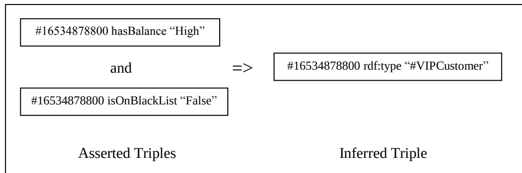
Figure 5.30 Inference rule for VIPCustomer class.
