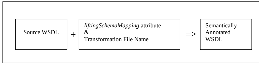
Figure 5.10 Semantic annotation for a source system.
