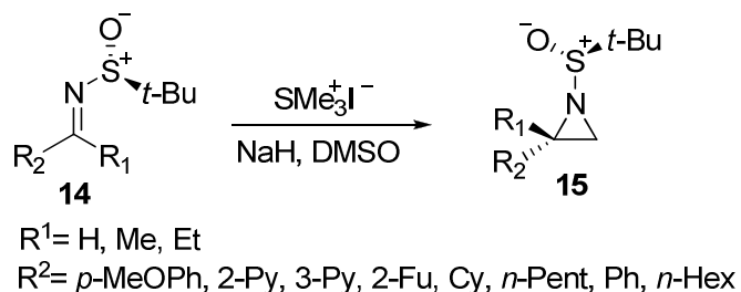
Scheme 5. Ylide-mediated aziridination.
