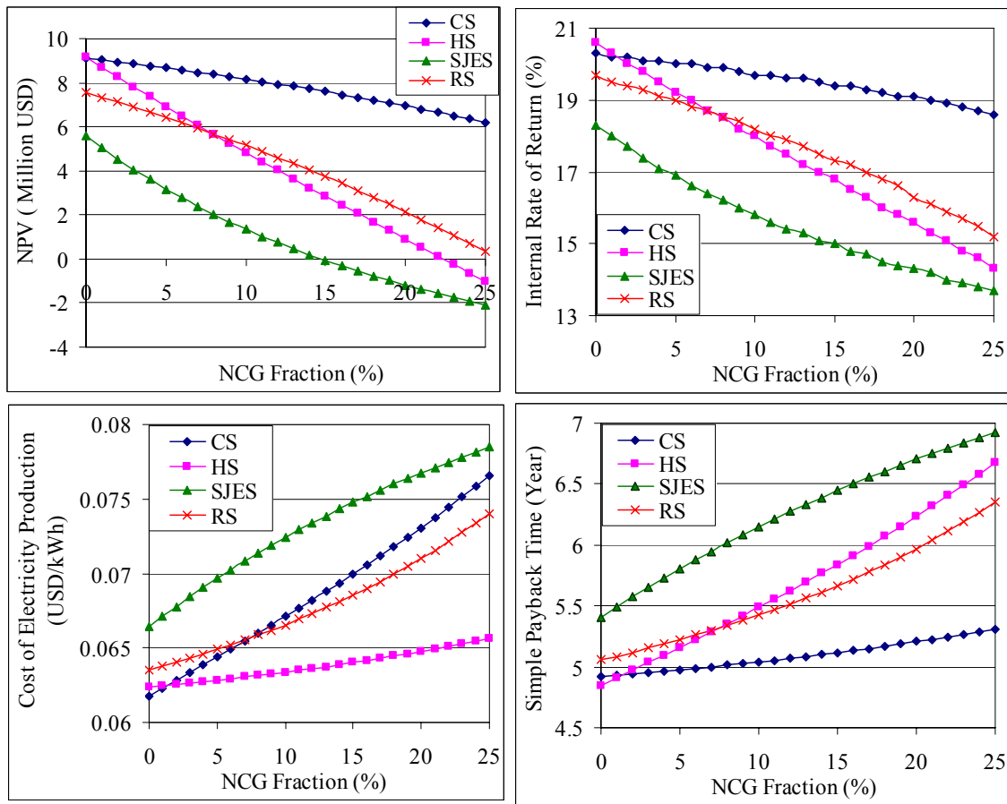
Figure 6.39. Comparison of the NCG removal system for double-flash design with optimum separator pressures.
