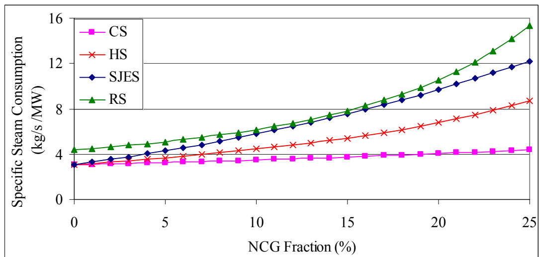
Figure 6.8. Specific steam consumption for various NCG fractions.
