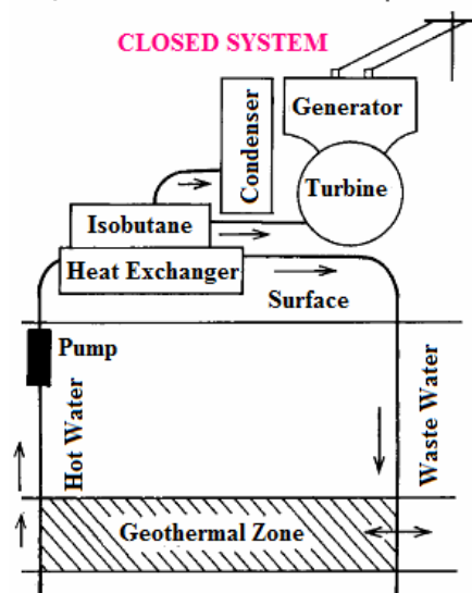
Figure 2.2. Basic GPP types. (Source: Gupta and Roy, 2007)
