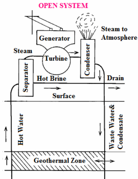
Flashed-Steam GPPs
