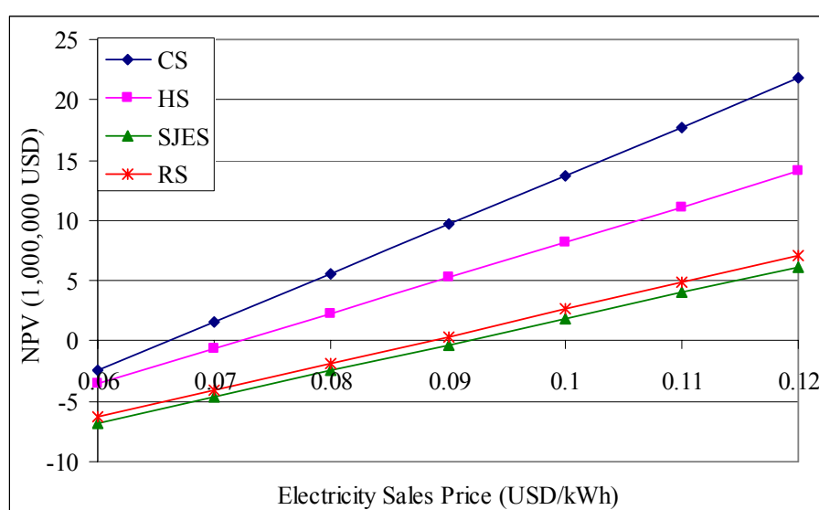
Figure 6.25. NPV of NCG removal systems vs. electricity sales price.
