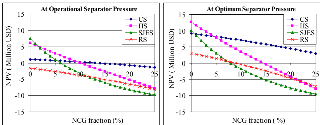
Figure 6.34. Simulation results for separator pressure.
