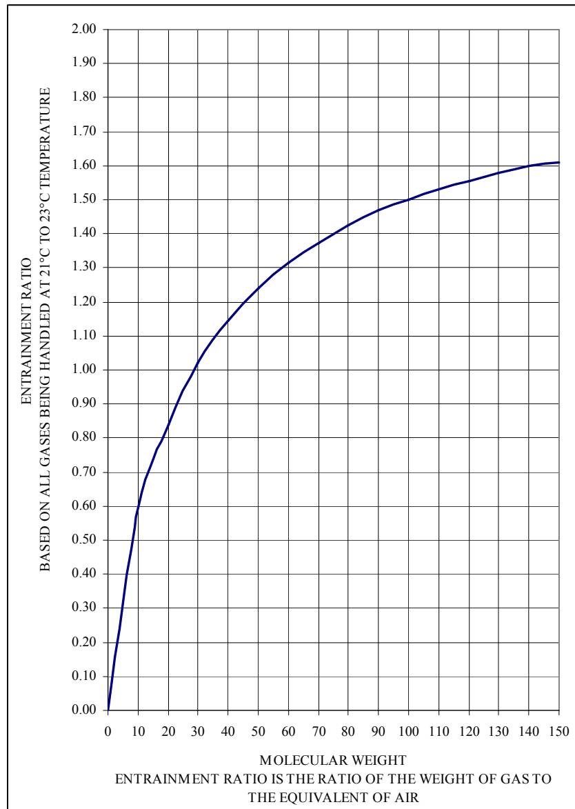
Figure 4.13. Entrainment ratio curve. (Source: Geothermal Institute, 1996b)
