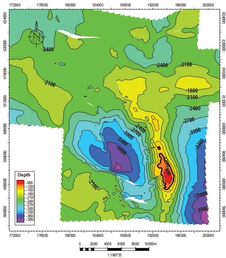
Figure 4.7: Map view (left) and vertically exxagerated (3x) 3D perspective view of top Zechstein, indicating the rise of the salt layer.
