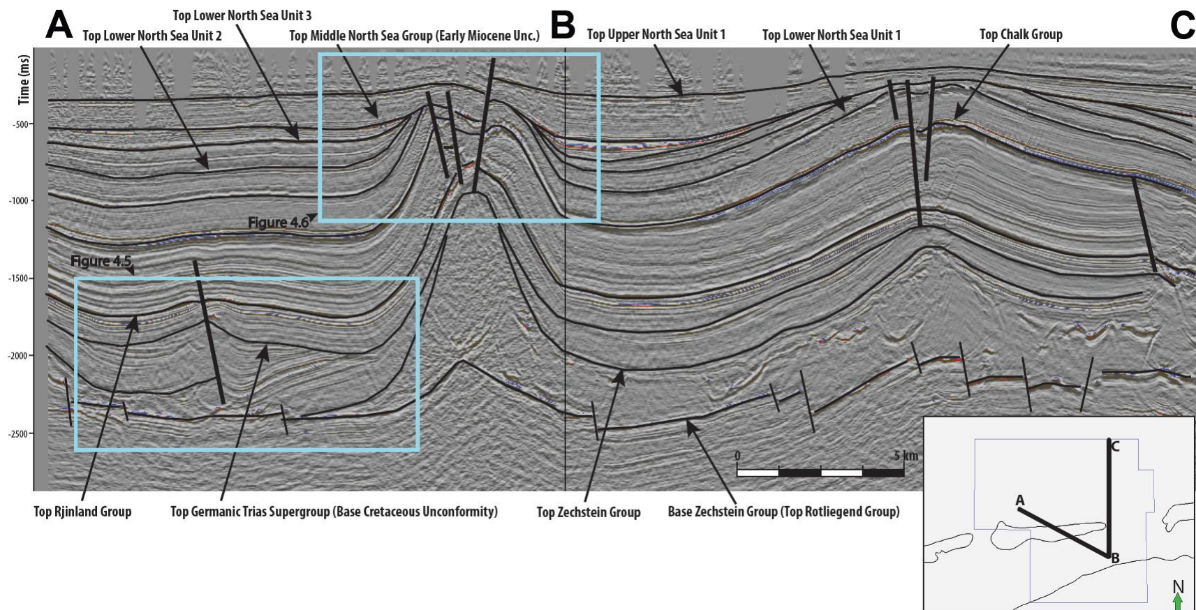
Figure 4.3: Interpreted and vertically (x5) exaggerated composite (arbitrary) seismic section in time domain.
