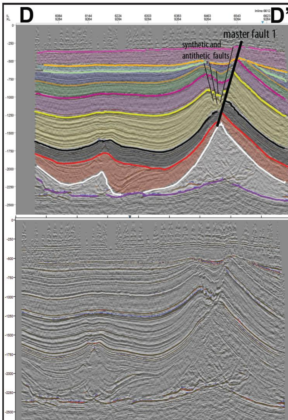
Figure B.4: Interpreted (top) and uninterpreted (bottom) seismic section D-D'. See Figure 4.11 for its location.
