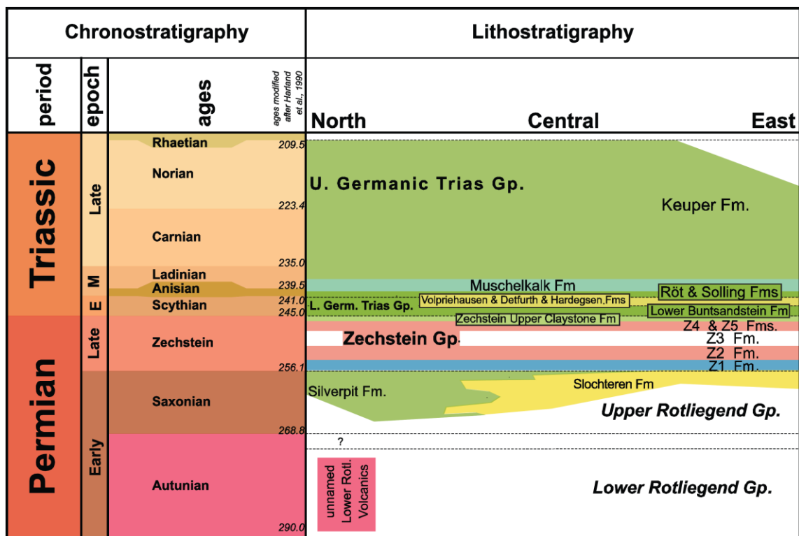
Figure 2.8: Generalized Permian and Triassic lithostratigraphy in the Netherlands (adopted from Geluk, 2007b; Herengreen & Wong, 2007; Wong et al, 2007).
