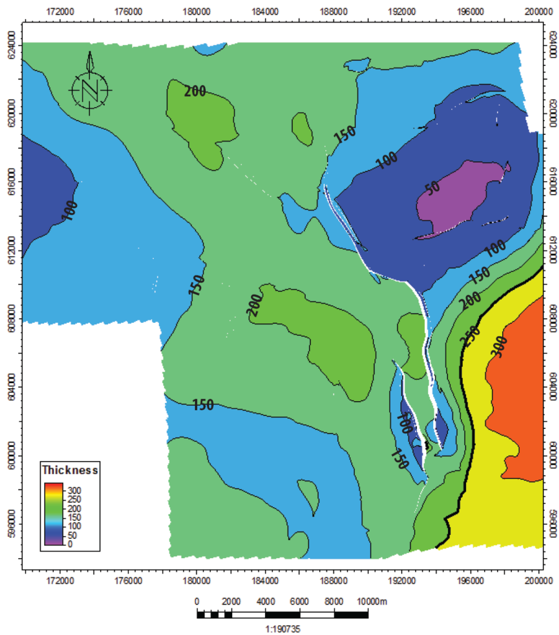
Figure A.7: Isopach map of Upper North Sea Group.
