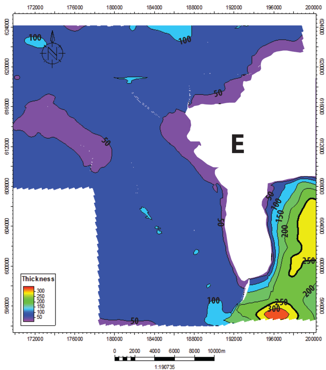
Figure A.6: Isopach map of Middle North Sea Group. E: eroded areas.
