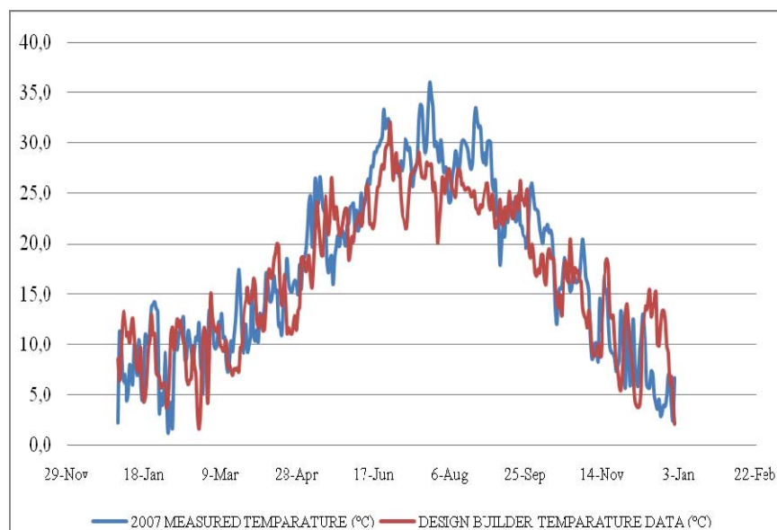
Figure 3.12. Comparison of Outside Temperatures.
