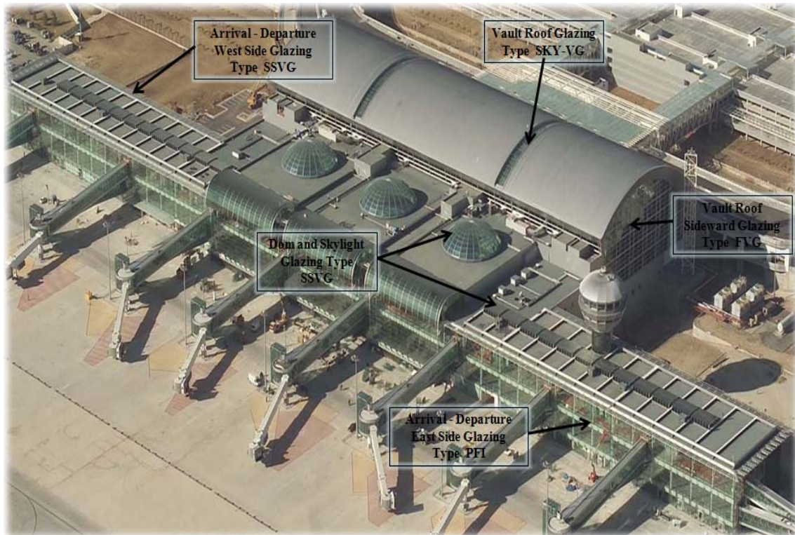
Figure 2.4. Glazing Types.
