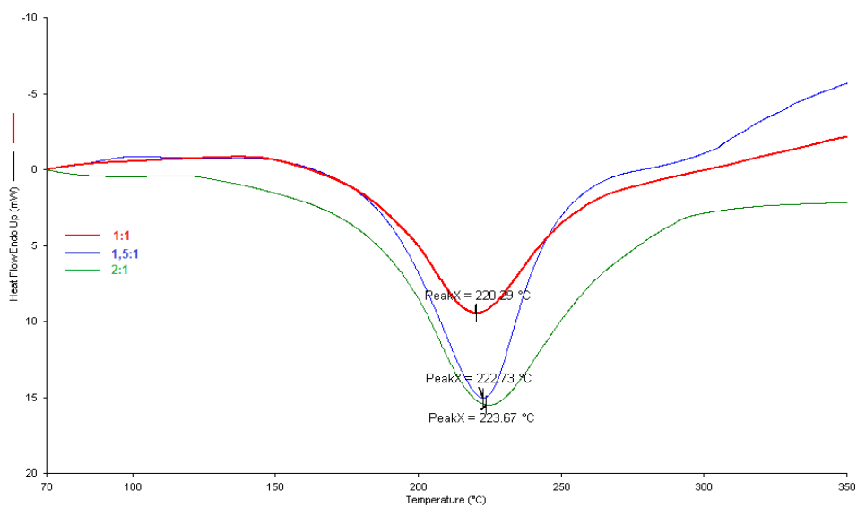
Figure 3.17 DSC thermograms of BMI/ADM prepolymers (BMI/ADM 1:1 mole ratio; BMI/ADM 1.5:1 mole ratio; BMI/ADM 2:1 mole ratio)
