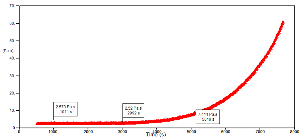
Figure 3.26 Viscosity-time plot at 120°C for BMI/ADM mole ratio of 1:1
