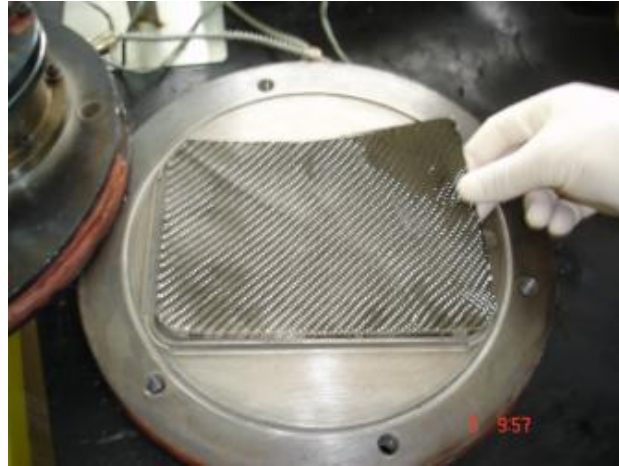
Figure 2.9 Placing carbon fabric layers in the lower mold cavity
