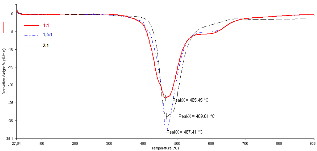
Figure 3.25 T_{d_{max}} results of BMI/ADS resins
