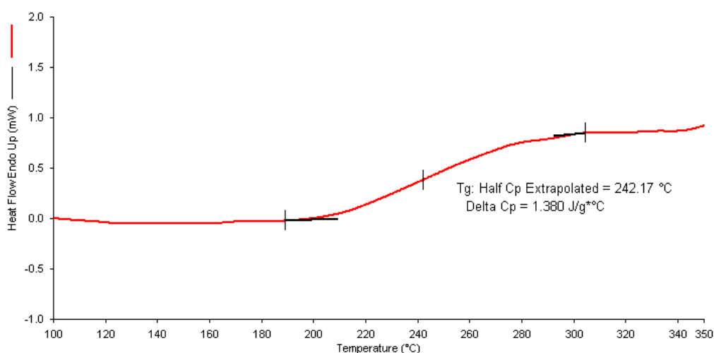
Figure 3.31 Glass transition temperature of composite 1
