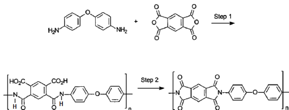
Figure 1.2 Reaction route for the synthesis Kapton™ polyimide [5].
