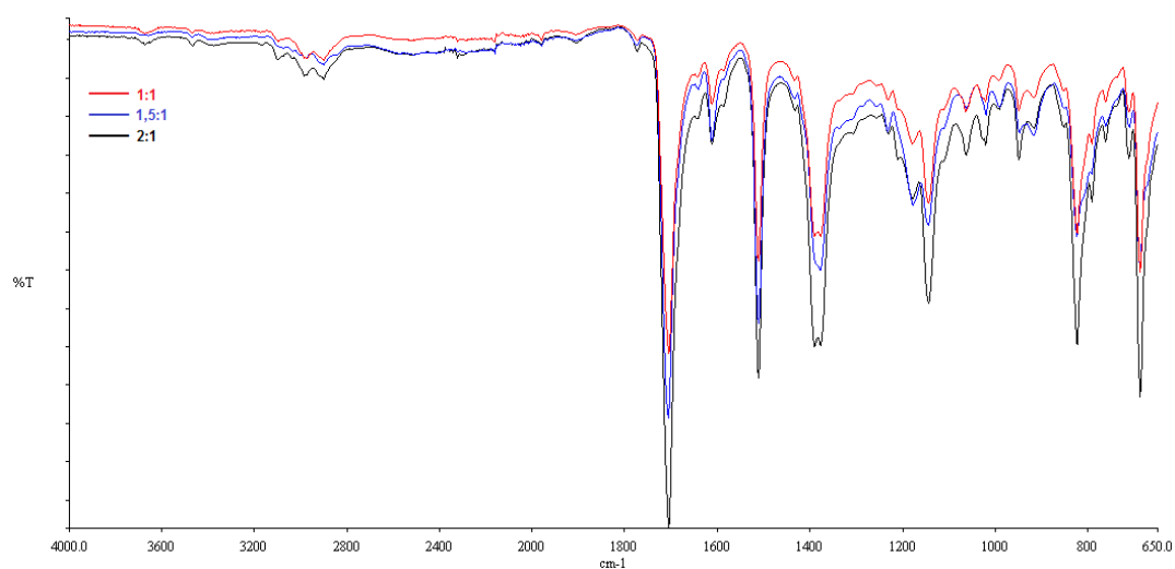
Figure 3.14.a FTIR spectra of BMI/ADM resins ( BMI/ ADM 1:1 mole ratio; BMI/ ADM 1.5:1 mole ratio; BMI/ ADM 2:1 mole ratio)
