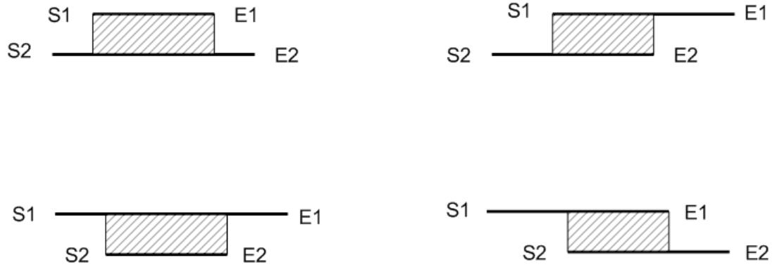
Figure 6.2: Overlapping conditions for two time intervals and their overlapping regions.
