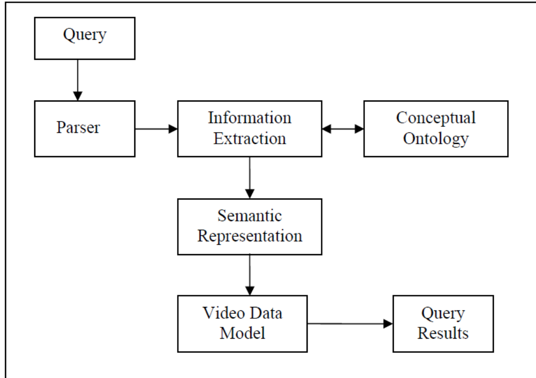
Figure 3.4: The main structure of the natural language interface of the video data model
