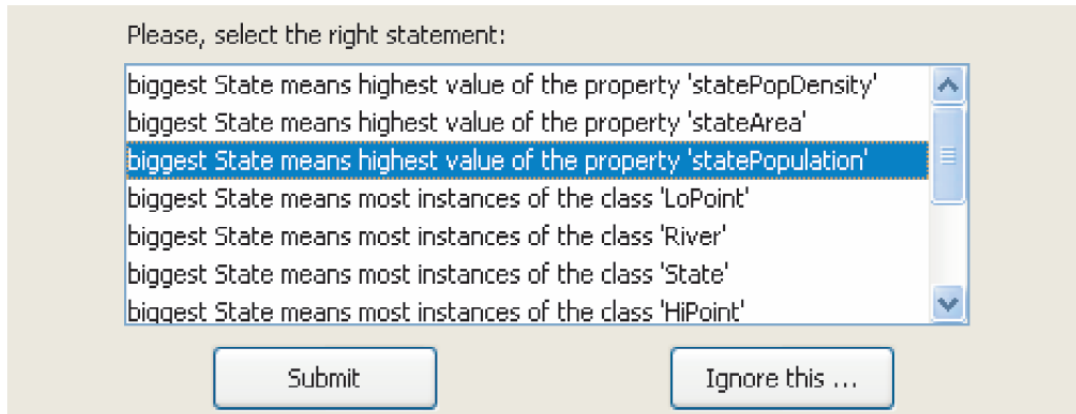
Figure 3.2: Querix Clarification Dialog
