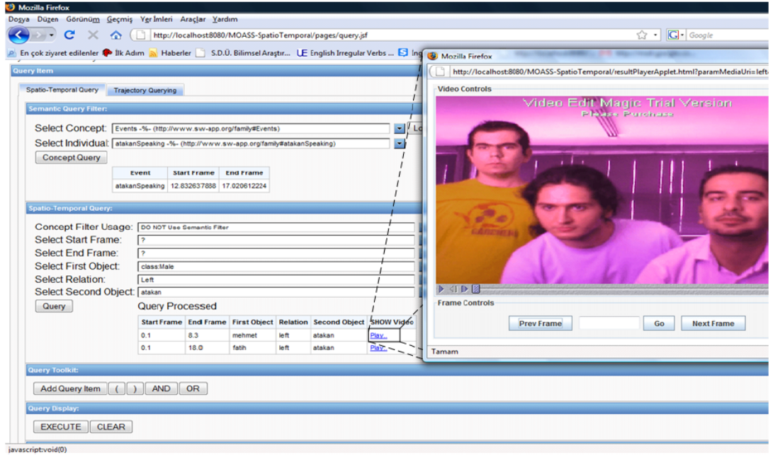
Figure 3.5: Simple Spatial Query Screen of OntoVMS
