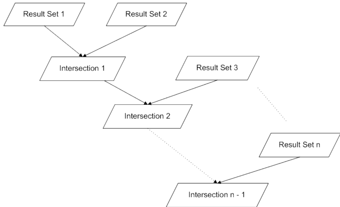
Figure 6.1: The intersection of the execution results of concept queries.
