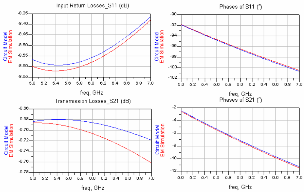
Figure 3-49: EM Simulation and Circuit Model Results of L=500\mu\text{m} , W=20\mu\text{m} , W_t=30\mu\text{m} and N=16
