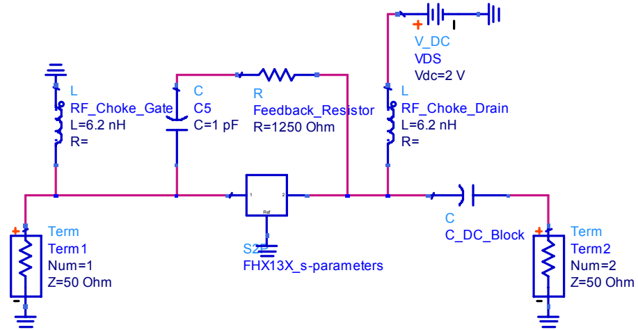
Figure 4-17: Schematic of FHX13X with Bias and Stability Circuits
