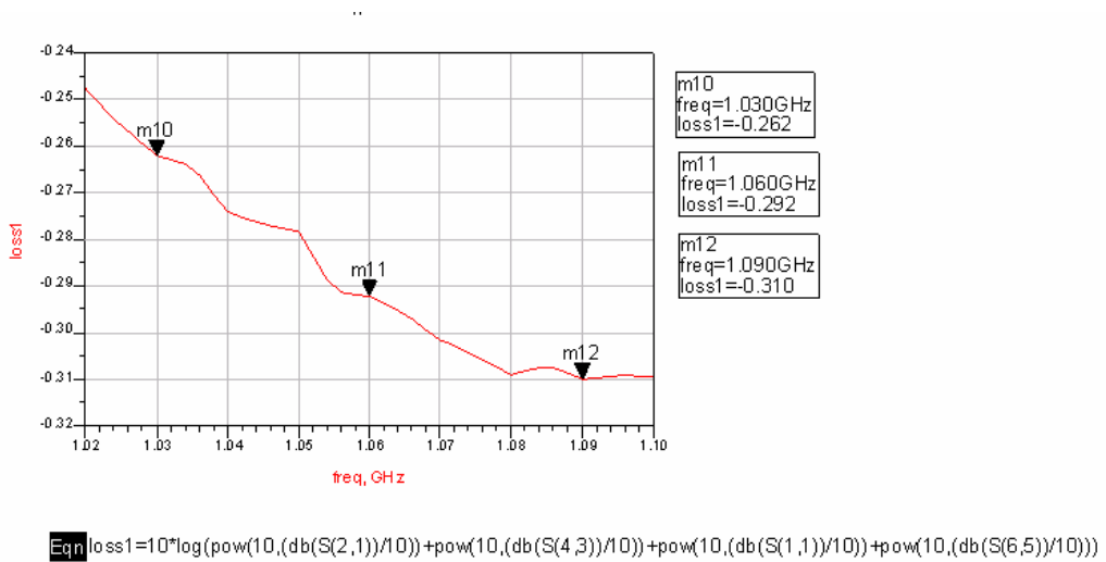
Figure 3-10: Total Loss of Dual Transmission Line Branch-Line Coupler
