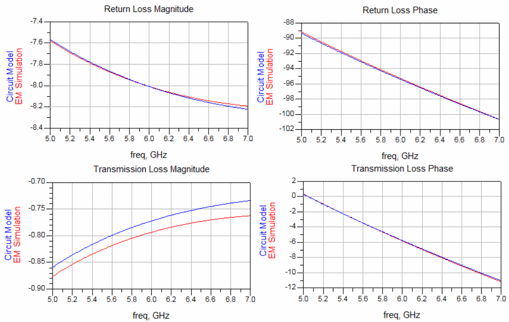
Figure 4-10: EM Simulation and Circuit Model Results of L=500\mu\text{m} , W=30\mu\text{m} , W_t=30\mu\text{m} and N=12
