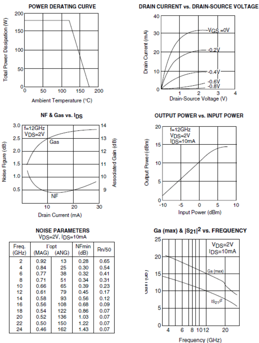
Figure B-2: FHX13X Characteristic Curves
