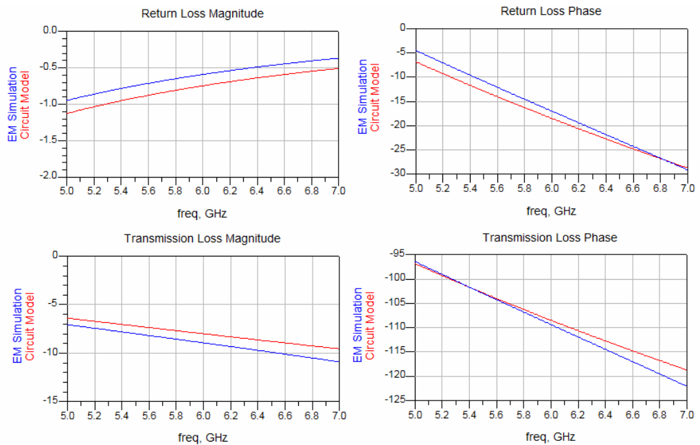
Figure 4-8: EM and Circuit Model Simulation Results of Spiral Inductor with Dimensions 1000x900 \mu\text{m}
