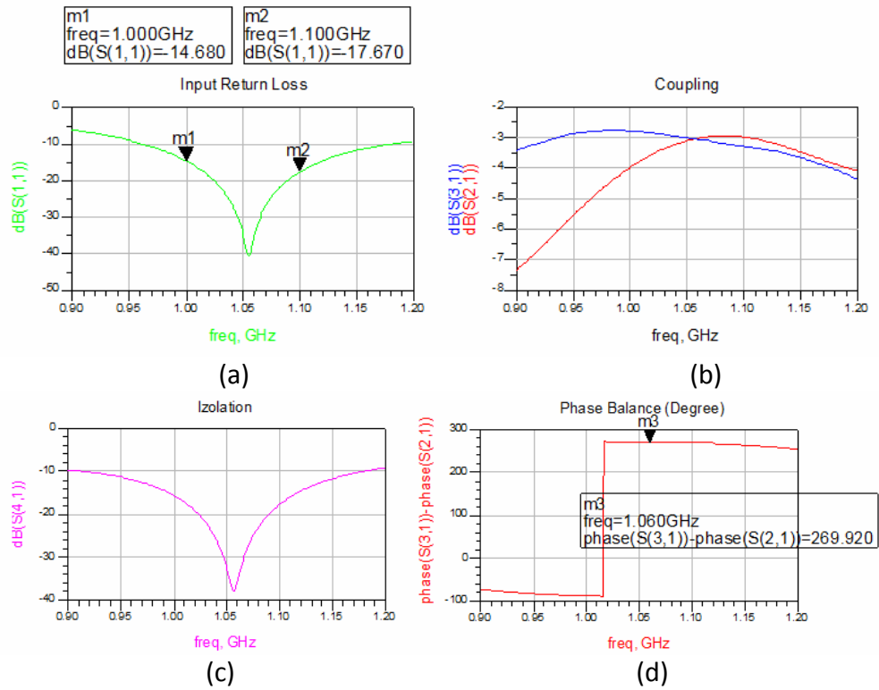
Figure 3-15: EM Simulation Results of Branch-Line Coupler with Shunt Connected Capacitors, (a) Input Reflection (b) Direct and Coupled Port Transmission (c) Isolation (d) Phase Difference of the Output Ports
