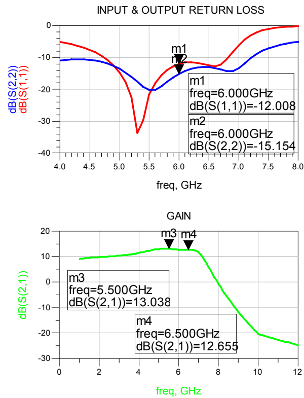
Figure 4-14: Simulation Results of TGF2021-01 I/O Match with IDCs and SIs
