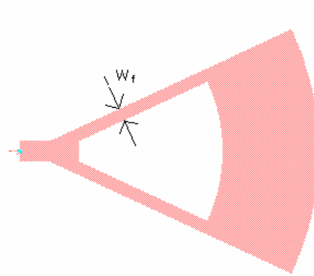
Figure 3-36: Layout of Radial Stub with Radial Slot with W_f Feed-line Width
