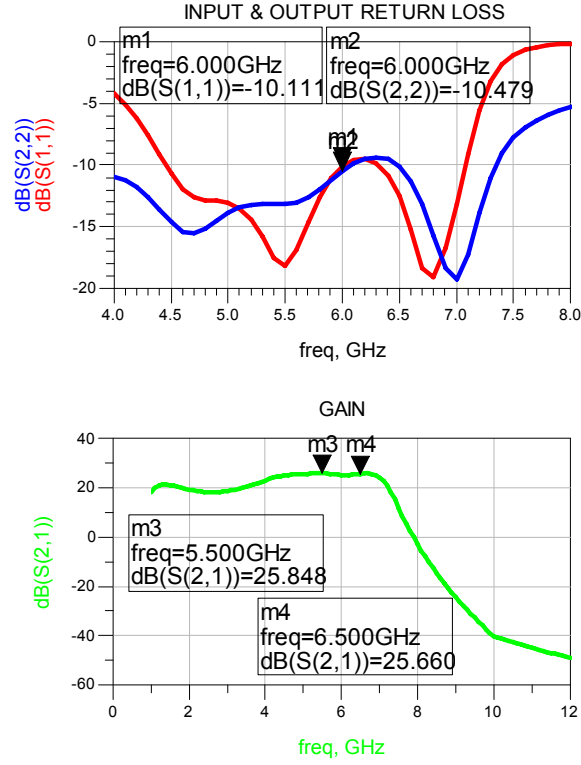
Figure 4-15: Simulation Results of Two Cascaded TGF2021-01 Amplifier
