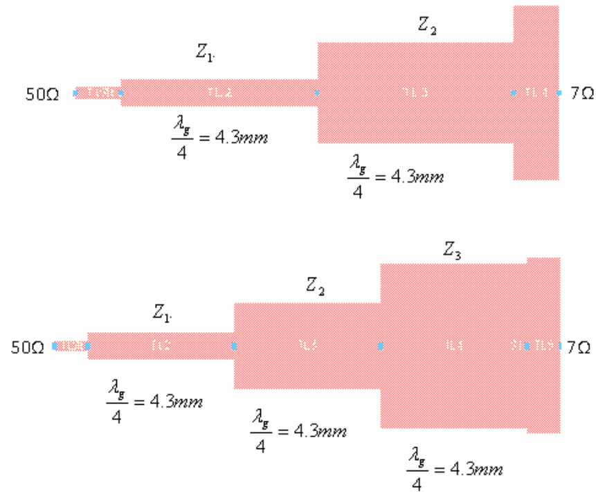
Figure 3-58: Layout of 2 and 3 Stage Matching Sections
