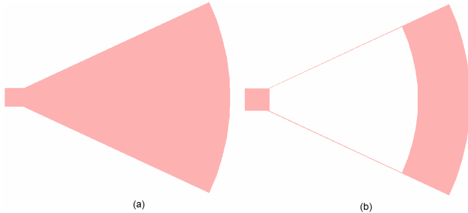
Figure 4-12: Layouts of Radial Stub on Alumina (a) Before and (b) After Miniaturization
