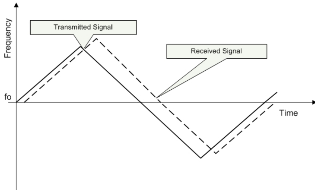
Figure 2-6: Triangular frequency modulation for transmitted and received signals with Doppler shift
