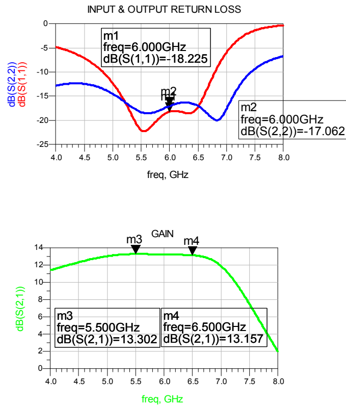
Figure 4-5: Simulation Results of Ideal Component Match of TGF2021-01
