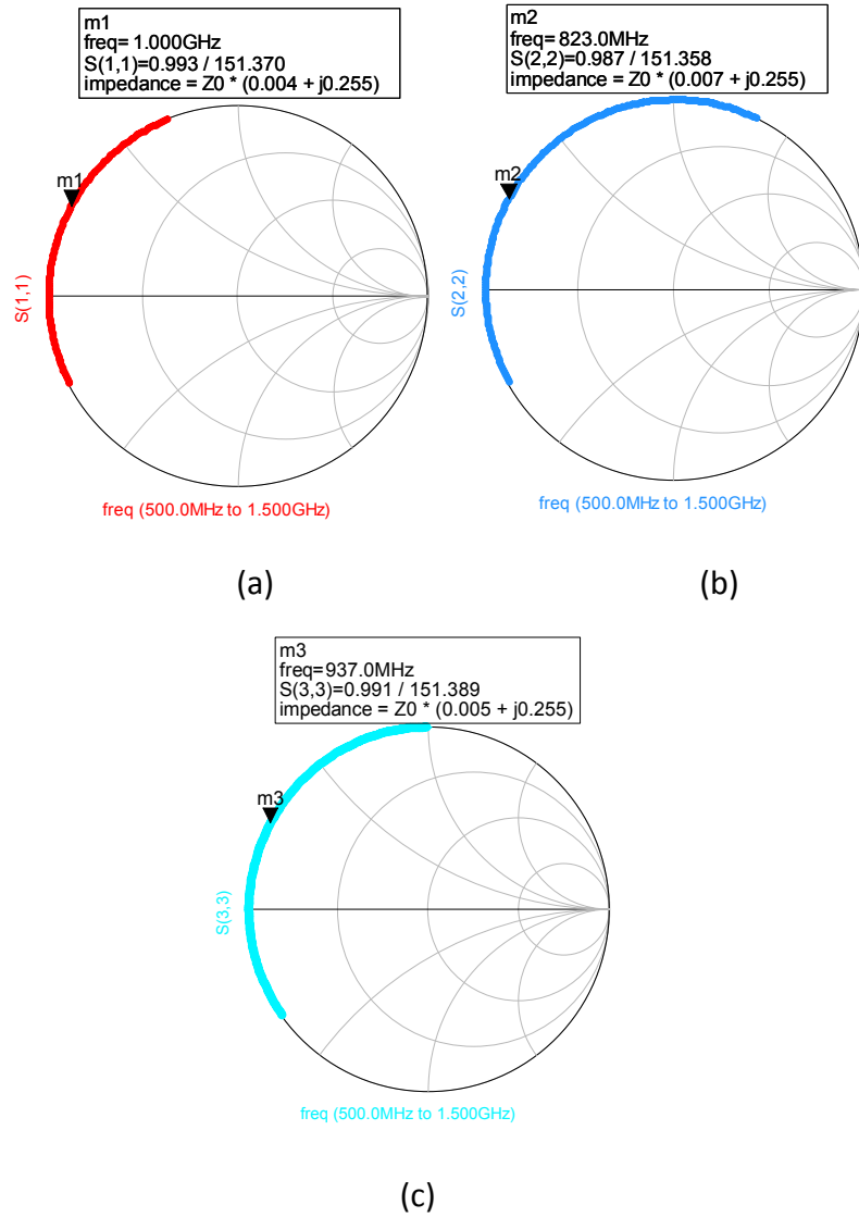
Figure 3-40: Measurement Results (a) Reference Short Point, (b) 0.3mm, (c) 1mm Feedline Width
