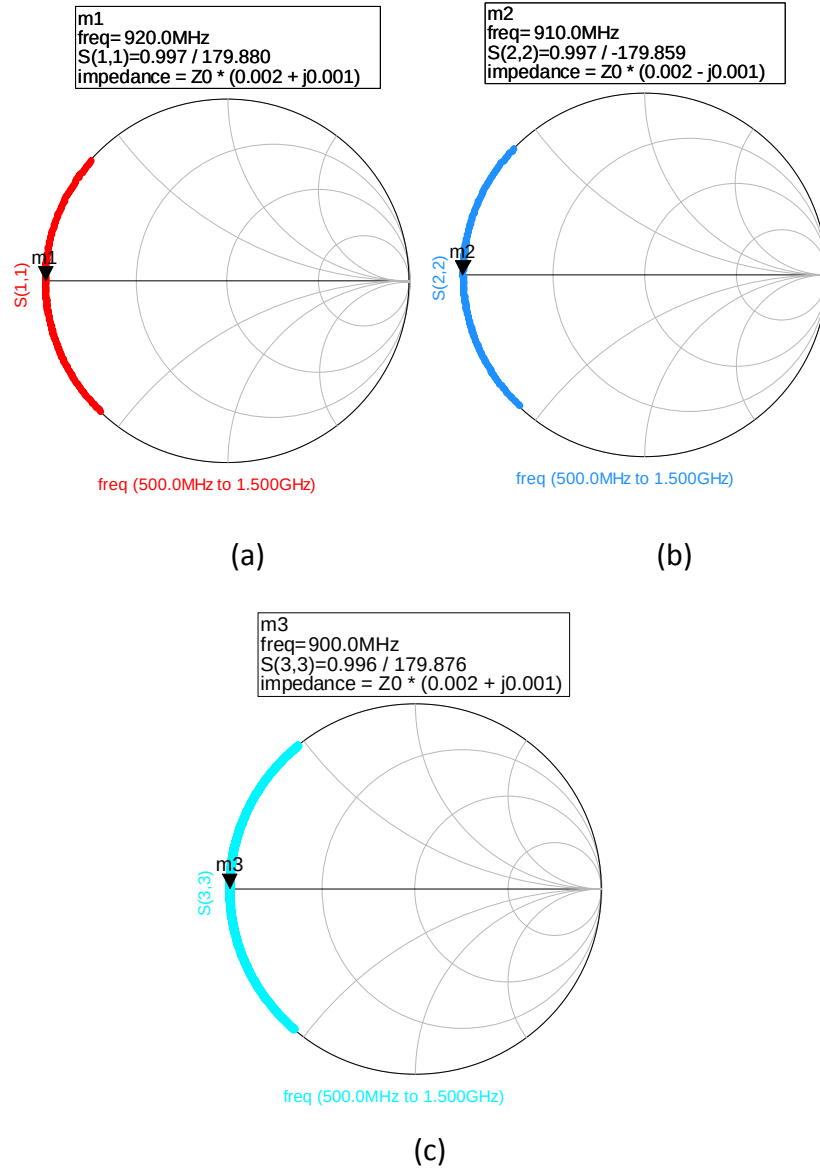
Figure 3-31: EM Simulation Results of 40° Radial Stub with slot length (a) 10mm, (b) 11mm, (c) 13mm
