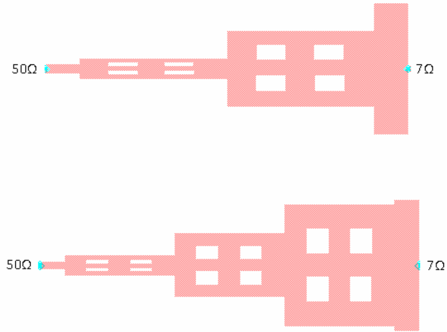
Figure 3-59: Layout of Matching Sections with Sierpinski Square for Iteration Order-1
