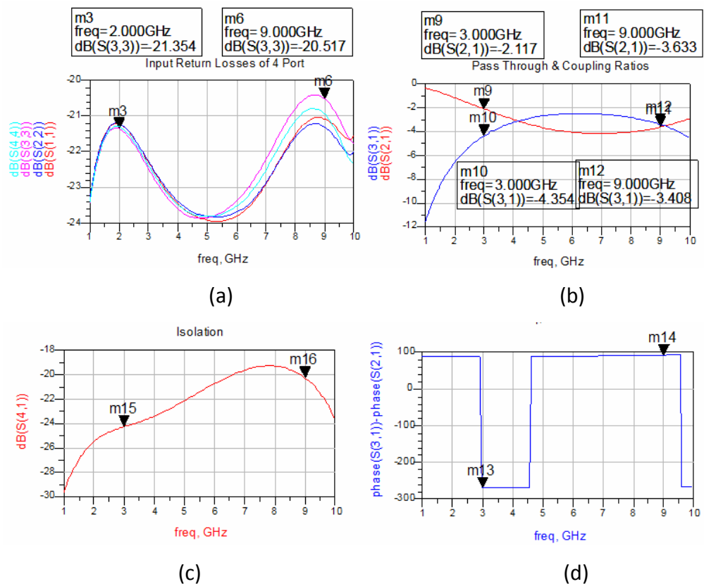
Figure 3-19: EM Simulation Results of 3 dB Directional Coupler, (a) Input Reflection (b) Direct and Coupled Port Transmission (c) Isolation (d) Phase Difference of the Output Ports
