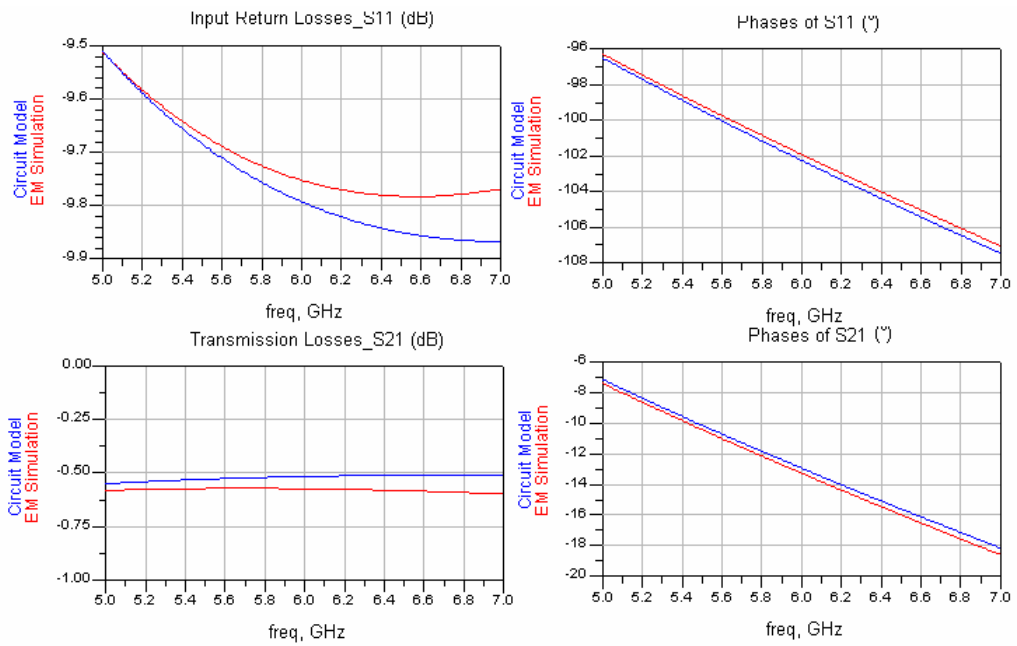
Figure 3-46: EM Simulation and Circuit Model Results of L=1000\mu\text{m} , W=20\mu\text{m} , W_t=30\mu\text{m} and N=8
