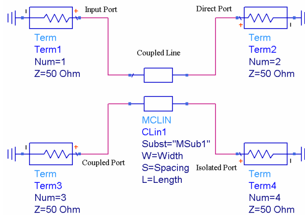
Figure 3-2: Schematic of a Coupled Line Coupler
