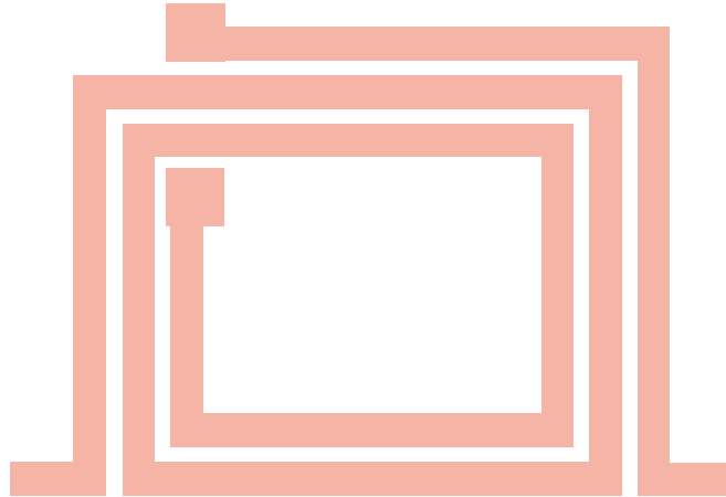
Figure 4-7: Layout of 2 \frac{3}{4} Turn Spiral Inductor
