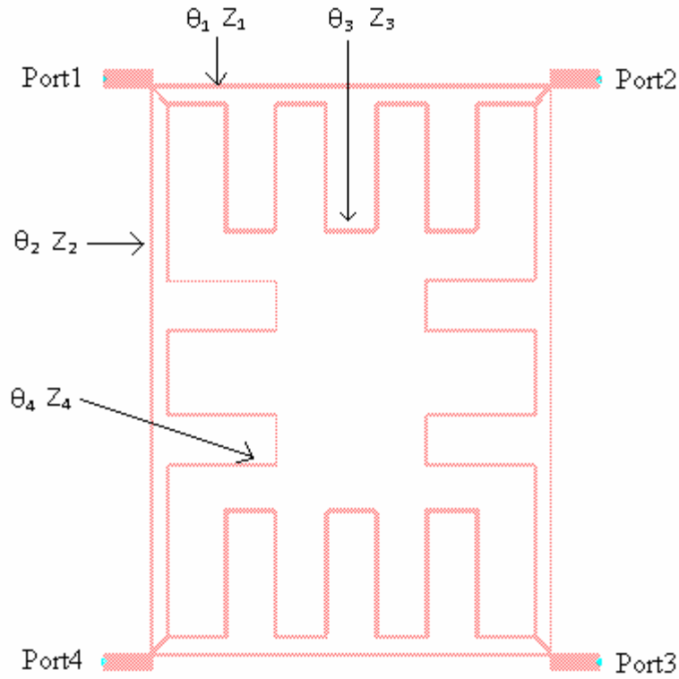
Figure 3-7: Layout of Branch-Line Coupler with Dual Transmission Lines
