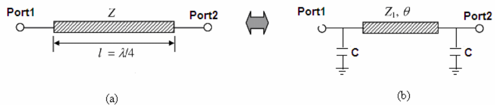
Figure 3-12: (a) Quarter Wavelength Transmission Line (b) Reduced Size Equivalent
