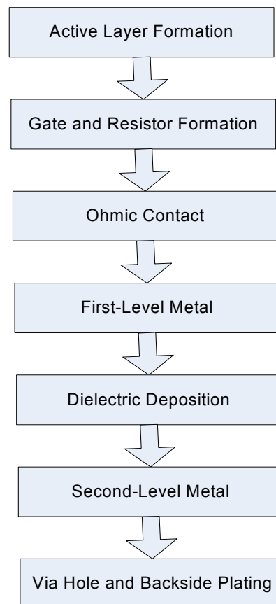
Figure 1-1: Typical MMIC fabrication process
