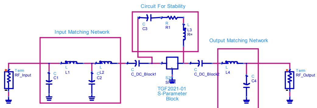
Figure 4-4: TGF2021-01 Input & Output Match with Ideal Components
