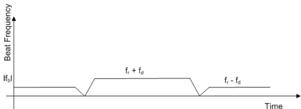
Figure 2-7: The beat frequency of triangular modulated signal with Doppler shift
