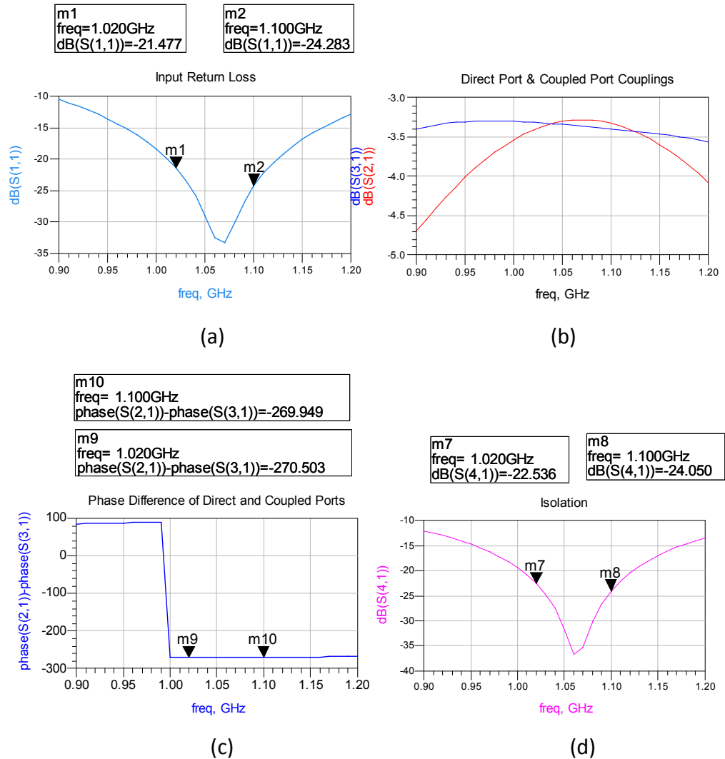
Figure 3-5: Simulation Results of Branch-Line Coupler at Center Frequency 1060MHz (a) Input Reflection (b) Direct and Coupled Port Transmission (c) Phase Difference of the Output Ports (d) Isolation
