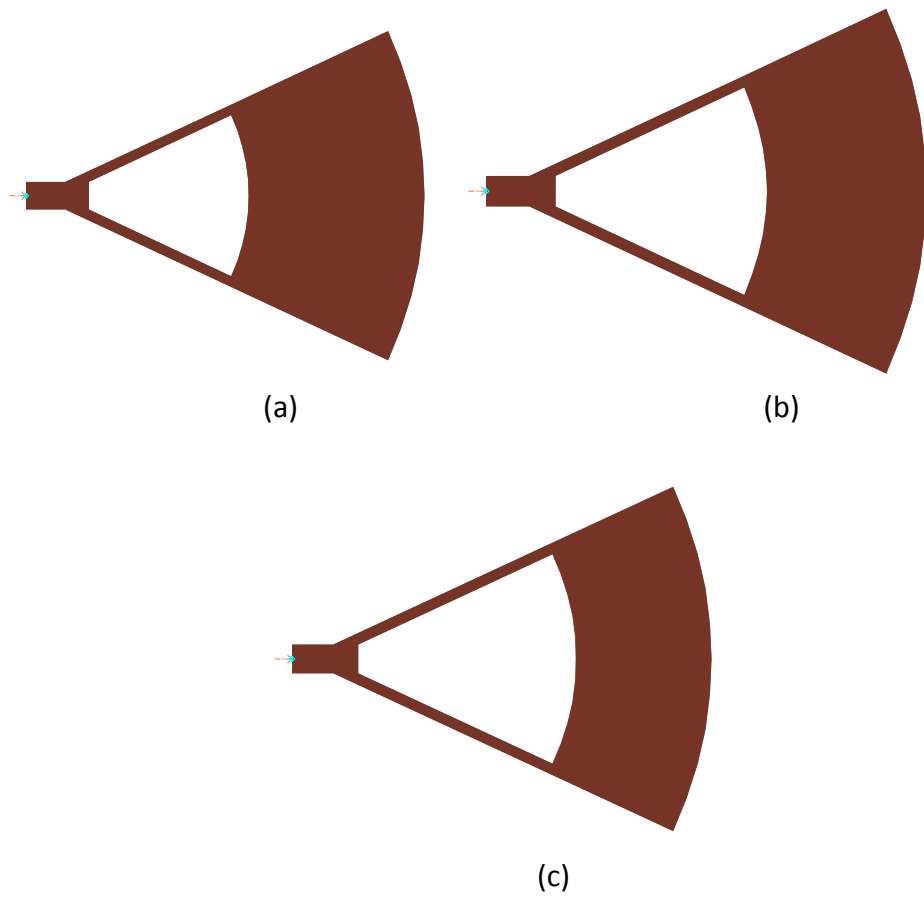
Figure 3-32: Layouts of 50° Radial Stub with Radial Slot Length (a) 10mm, (b) 12mm, (c) 13mm
