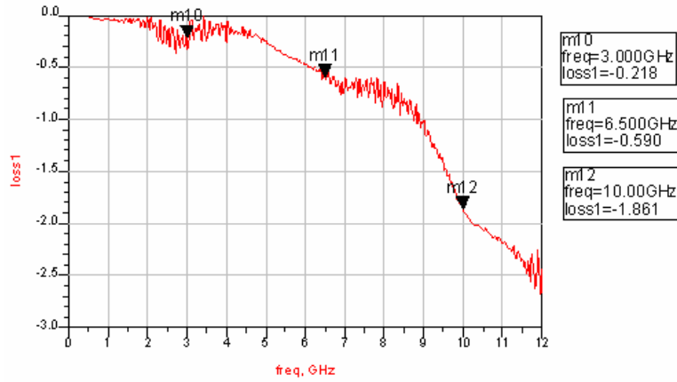
Figure 3-22: Total Loss Calculation of Measured Performance
