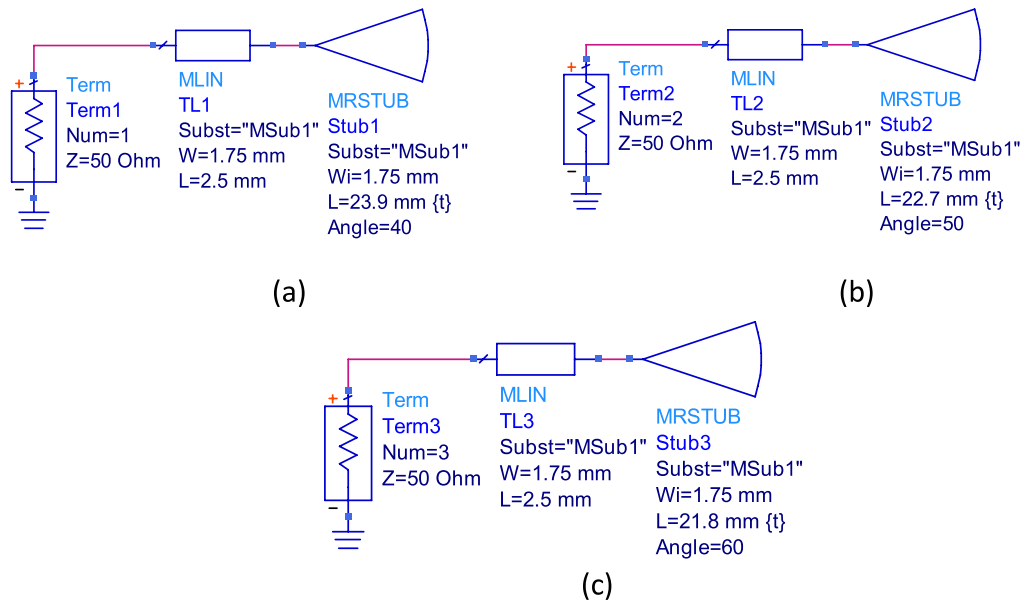
Figure 3-28: ADS Schematic of (a) 40°, (b) 50°, (c) 60° Radial Stubs @ 1 GHz
