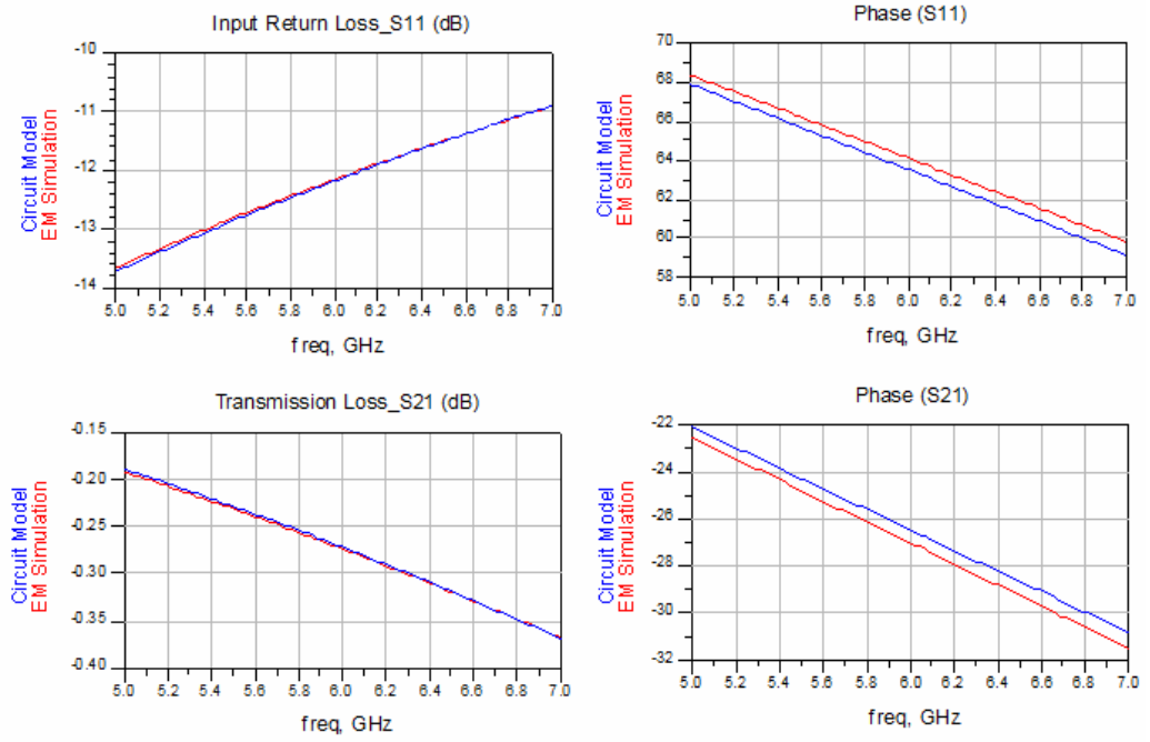
Figure 3-55: EM and Circuit Model Simulation Results of Spiral Inductor with Dimensions 400x400 \mu\text{m}
