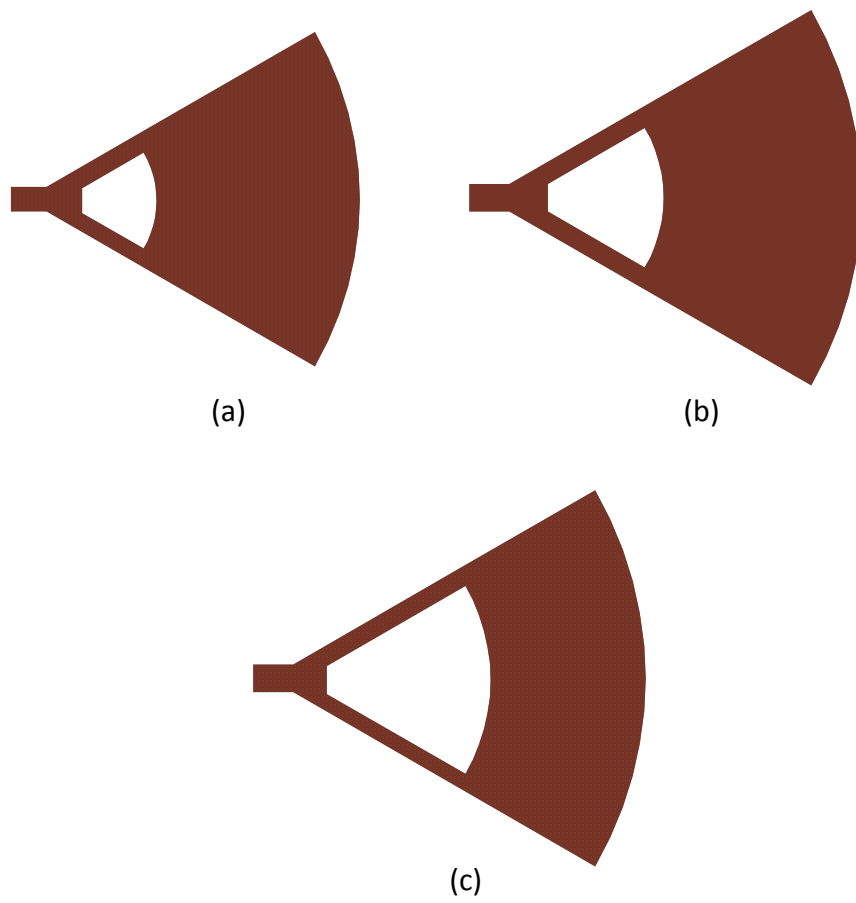
Figure 3-34: Layouts of 60° Radial Stub with Radial Slot Length (a) 5mm, (b) 7mm, (c) 10mm
