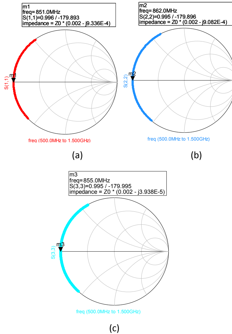
Figure 3-33: EM Simulation Results of 50° Radial Stub with slot length (a) 10mm, (b) 12mm, (c) 13mm
