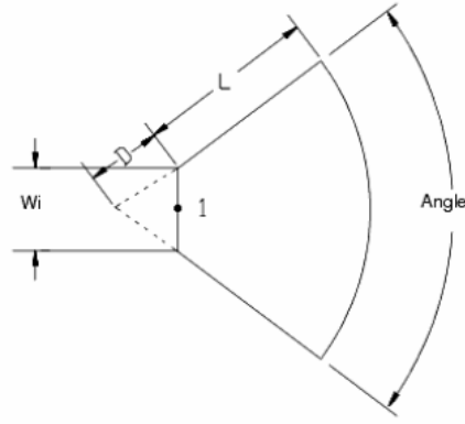
Figure 3-27: Geometry of Radial Stub
