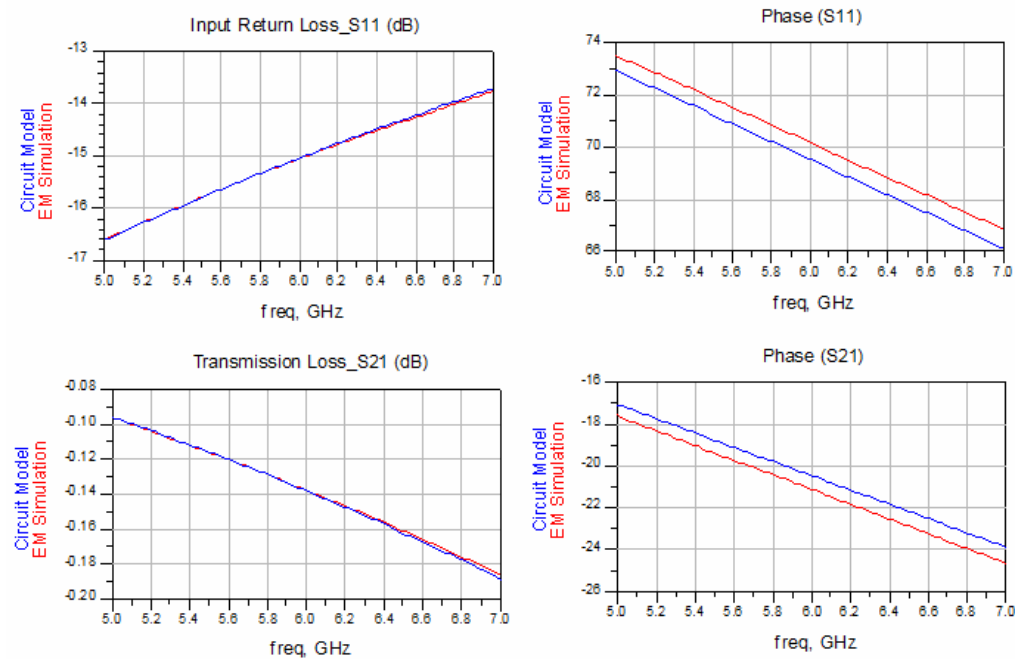
Figure 3-54: EM and Circuit Model Simulation Results of Spiral Inductor with Dimensions 400x320 \mu\text{m}
