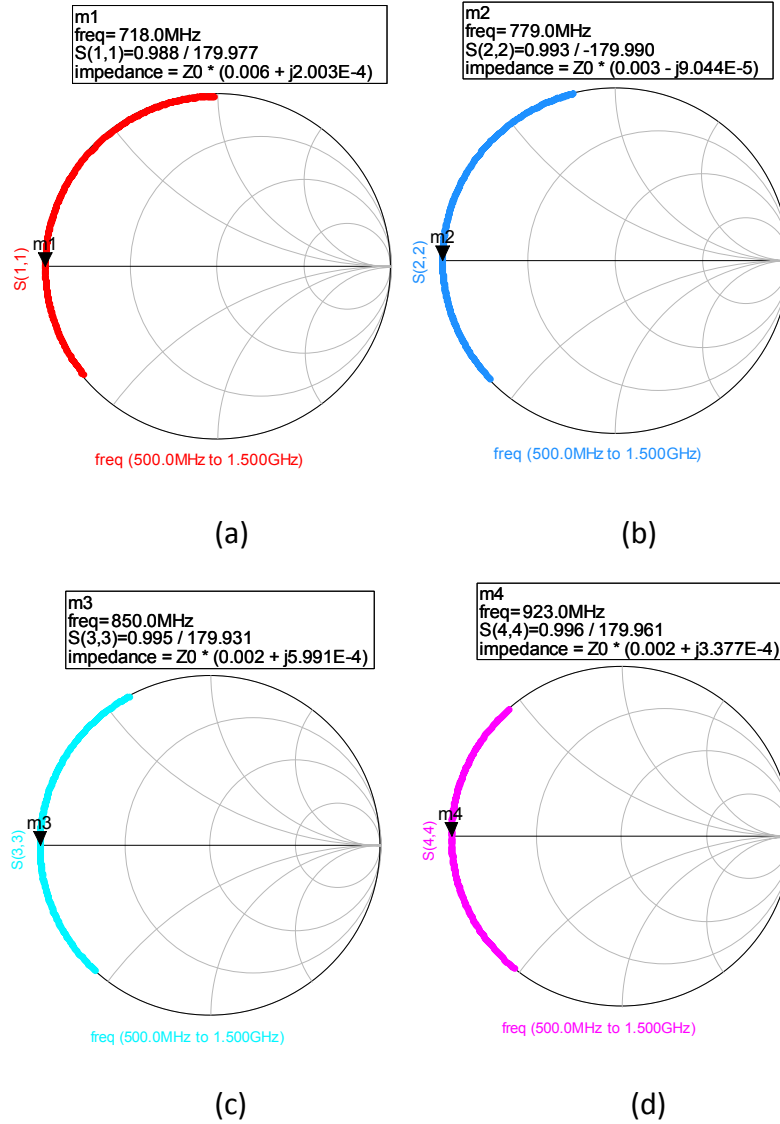
Figure 3-38: EM Simulation Results of 50° Miniaturized Radial Stub for Feedline Widths (a) 0.125mm, (b) 0.3mm, (c) 0.6mm, (d) 1mm
