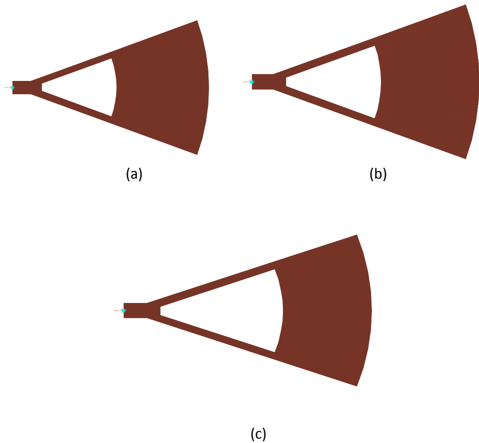
Figure 3-30: Layouts of 40° Radial Stub with Radial Slot Length (a) 10mm, (b) 11mm, (c) 13mm
