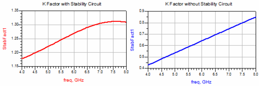
Figure 4-6: Stability Factor-K with and without Stability Circuit
