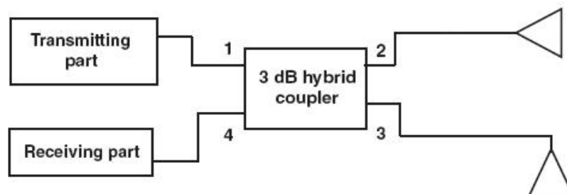
Figure 2-3: Front-end structure of FMCW radar with dual-polarized antenna
