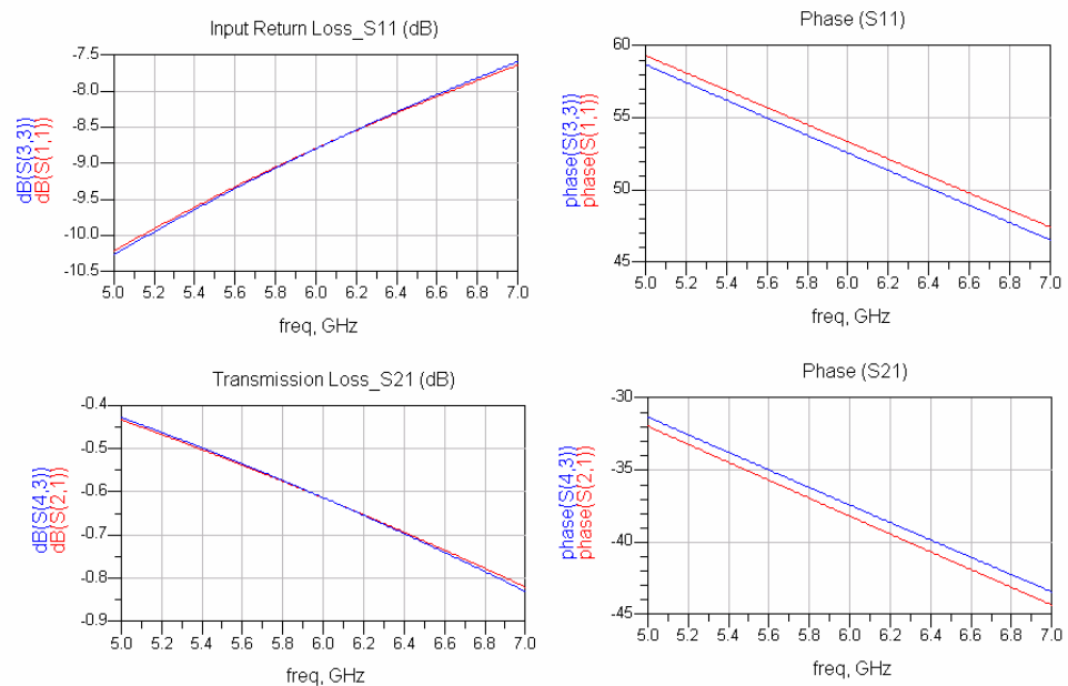
Figure 4-25: EM and Circuit Model Simulation Results of Spiral Inductor with Dimensions 510x510 \mu\text{m} and 1 \frac{3}{4} Turn
