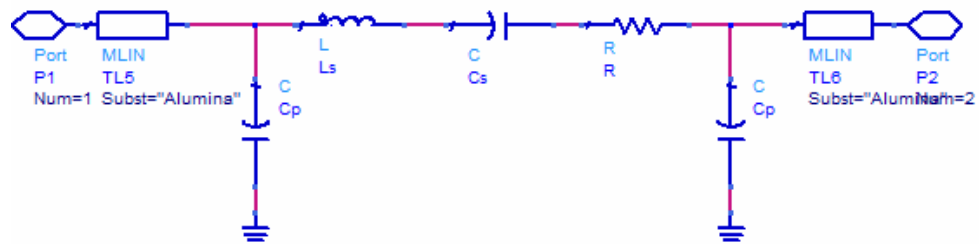
Figure 3-44: Lumped Element Equivalent Circuit of Interdigital Capacitor
