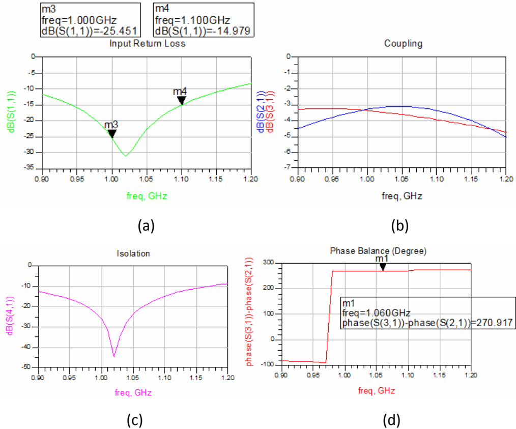
Figure 3-8: EM Simulation Results of Dual Transmission Line Branch-Line Coupler (a) Input Reflection (b) Direct and Coupled Port Transmission (c) Isolation (d) Phase Difference of the Output Ports
