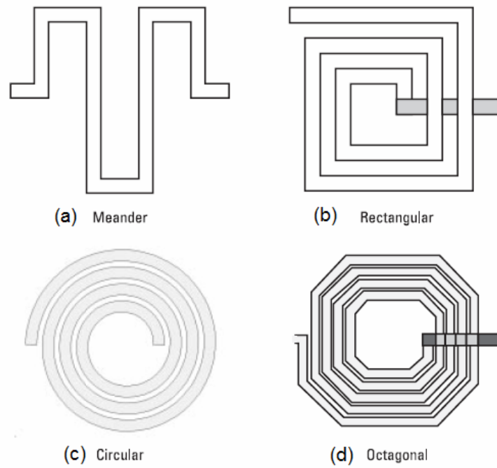
Figure 3-50: Two dimensional Inductor Types, (a) Meander, (b) Rectangular, (c) Circular, (d) Octagonal
