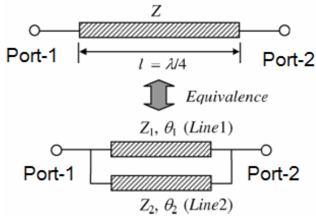
Figure 3-6: Dual Transmission Line Equivalent of Quarter Wavelength Transmission Line
