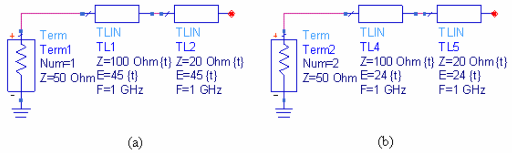
Figure 3-24: ADS Schematics of Proposed Method for Miniaturization of Quarter Wavelength Stubs
