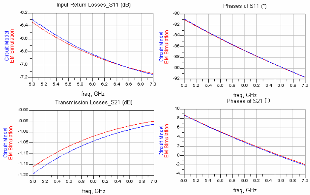
Figure 3-47: EM Simulation and Circuit Model Results of L=500\mu\text{m} , W=50\mu\text{m} , W_t=30\mu\text{m} and N=8
