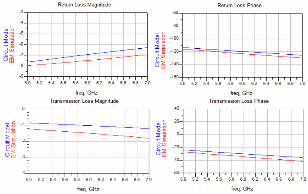
Figure 4-11: EM Simulation and Circuit Model Results of L=500um, W=30um, Wt=30um and N=12
