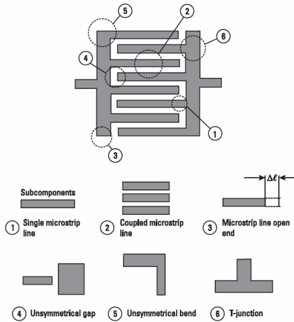
Figure 3-43: Interdigital Capacitor and its Subcomponents
