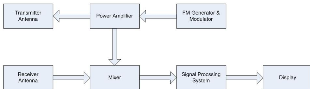
Figure 2-1: Basic block diagram of FMCW radar with two antennas
