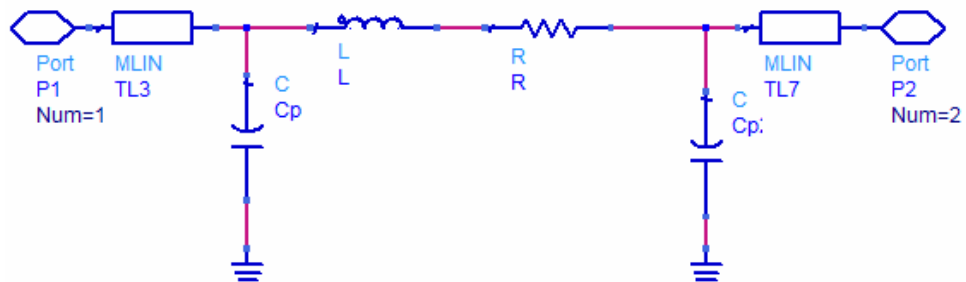
Figure 3-52: Equivalent Circuit for Rectangular Spiral Inductor
