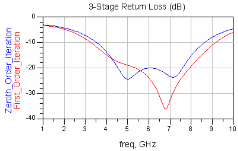
Figure 3-61: EM Simulation Result of 3-stage Matching Section Design
