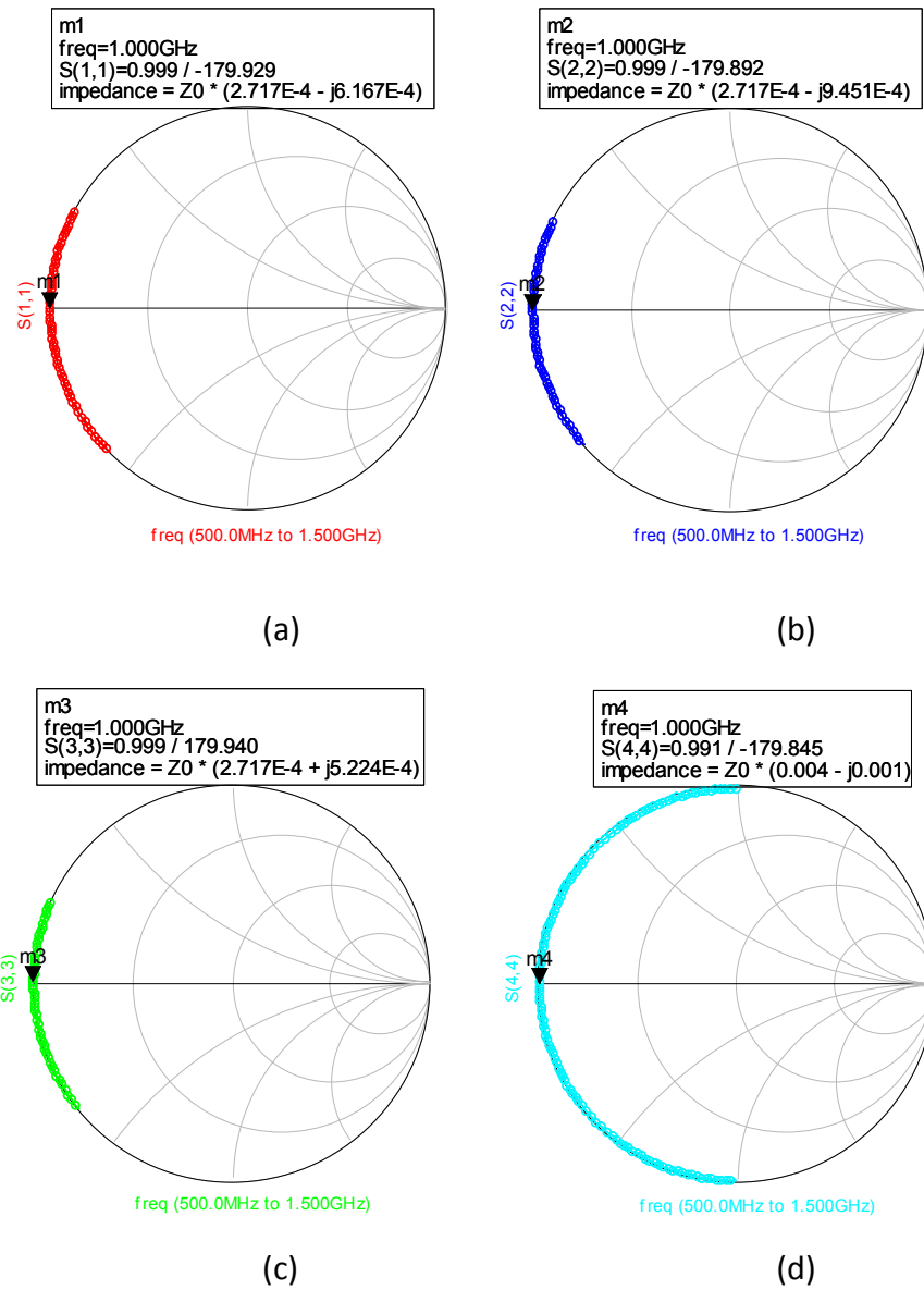
Figure 3-29: Simulation Results of (a) 40°, (b) 50°, (c) 60° Radial Stubs, (d) Quarter Wavelength Stub
