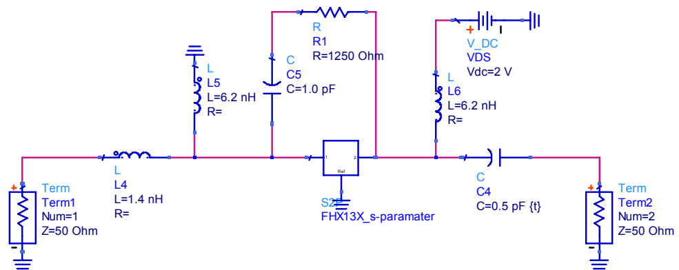
Figure 4-22: Final Schematic of FHX13X LNA Circuit
