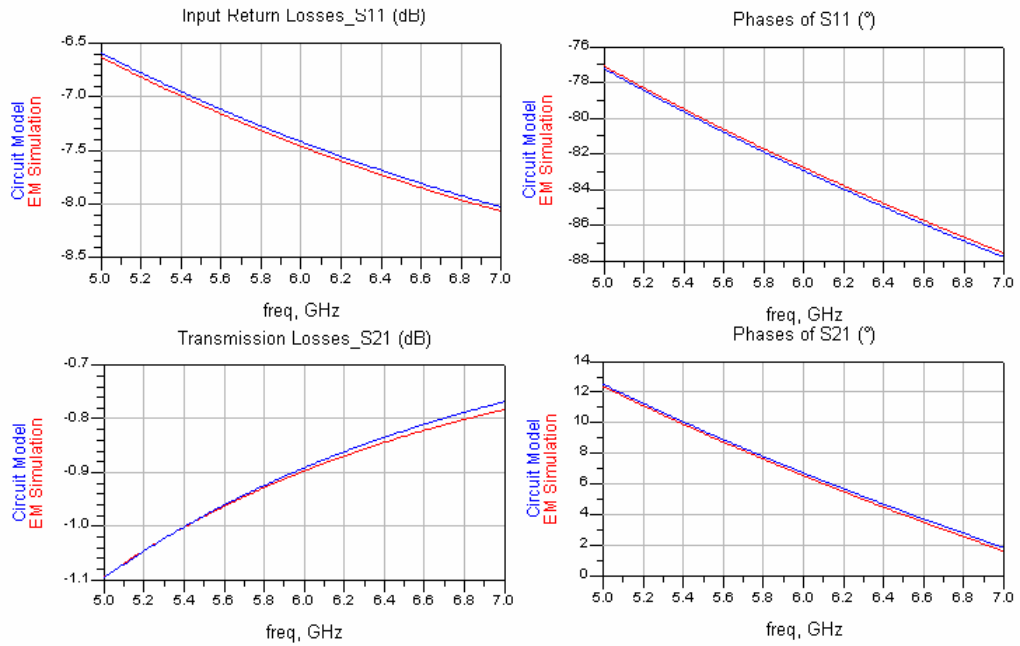
Figure 3-48: EM Simulation and Circuit Model Results of L=500\mu\text{m} , W=20\mu\text{m} , W_t=50\mu\text{m} and N=8
