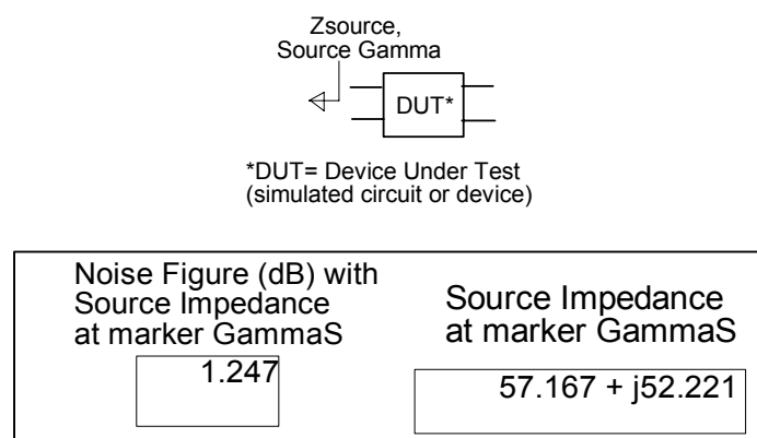
Figure 4-19: The Noise Figure and Source Impedance at Marker GammaS
