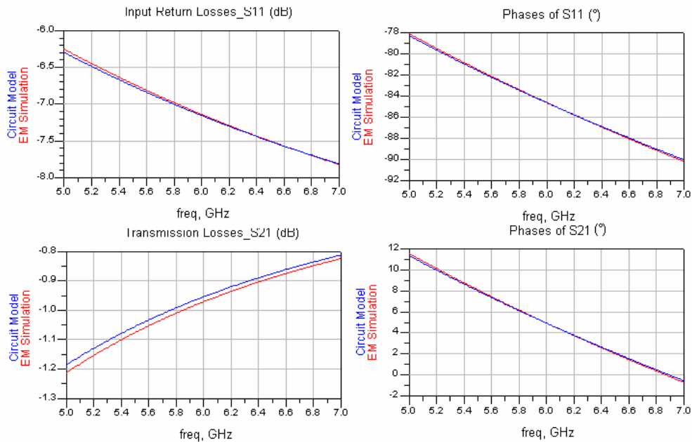
Figure 3-45: EM Simulation and Circuit Model Results of L=500\mu\text{m} , W=20\mu\text{m} , W_t=30\mu\text{m} and N=8
