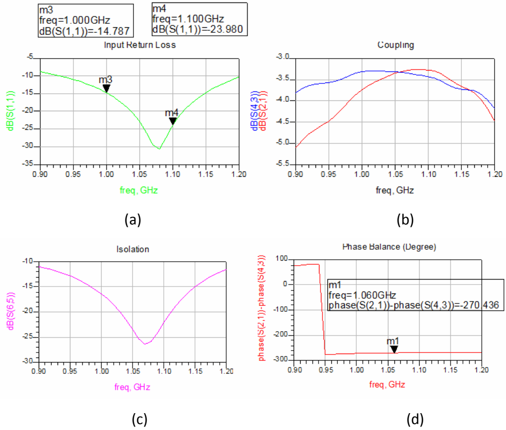
Figure 3-9: Measurement Results of Dual Transmission Line Branch-Line Coupler (a) Input Reflection (b) Direct and Coupled Port Transmission (c) Isolation (d) Phase Difference of the Output Ports
