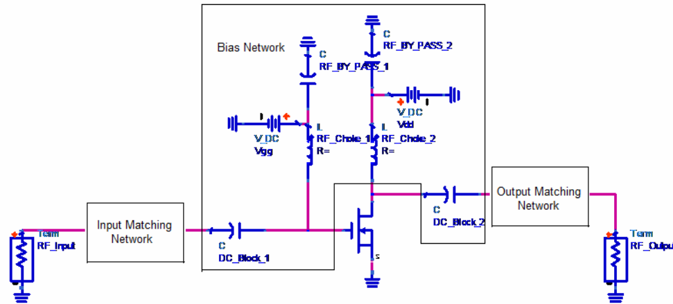
Figure 4-2: A Typical Single Stage Amplifier Schematic
