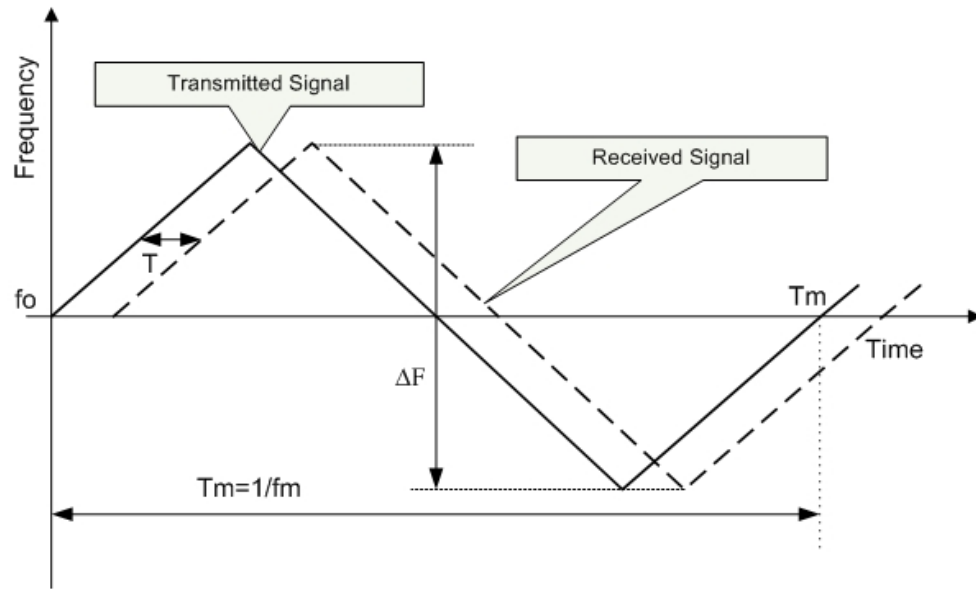
Figure 2-4: Triangular frequency modulation for transmitted and received signals
