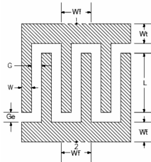
Figure 3-42: Layout of a Typical Microstrip Interdigital Capacitor
