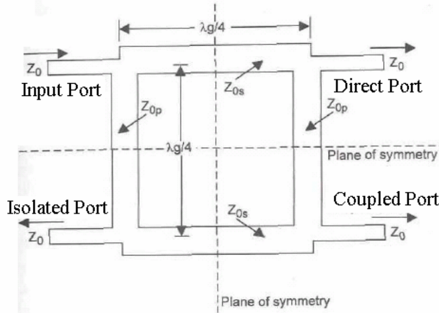
Figure 3-3: Layout of a Branch-Line Coupler
