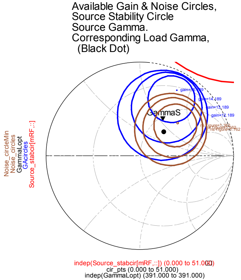
Figure 4-20: Gain, Stability and Noise Circles of FHX13X on Smith Chart
