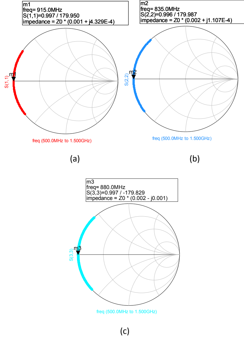
Figure 3-35: EM Simulation Results of 60° Radial Stub with slot length (a) 5mm, (b) 7mm, (c) 10mm
