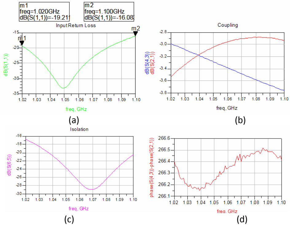
Figure 3-16: Measurement Results of Branch-Line Coupler with Shunt Connected Capacitors, (a) Input Reflection (b) Direct and Coupled Port Transmission (c) Isolation (d) Phase Difference of the Output Ports
