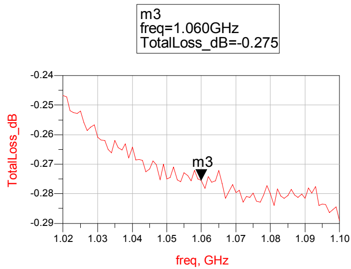
Figure 3-17: Total Loss of Branch-Line Coupler with Shunt Connected Capacitors
