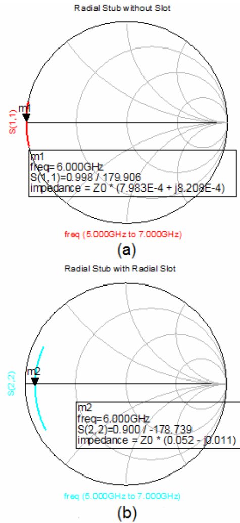
Figure 4-13: The Simulation Results of Radial Stub on Alumina (a) Before and (b) After Miniaturization
