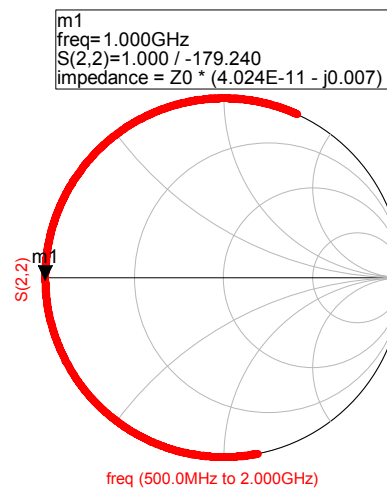
Figure 3-26: Simulation Result of Proposed Method in Figure 3-24-(b) on Smith Chart
