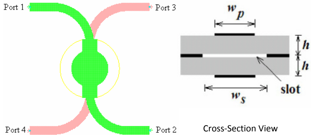
Figure 3-18: Simulated Layout of Aperture Coupled Directional Coupler
