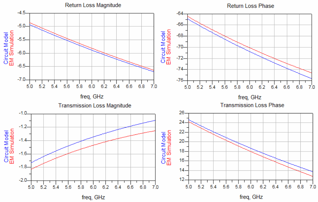
Figure 4-9: EM Simulation and Circuit Model Results of L=350\mu\text{m} , W=30\mu\text{m} , W_t=30\mu\text{m} and N=8
