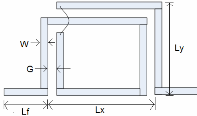
Figure 3-51: Layout of 1 \frac{3}{4} Turn Rectangular Inductor
