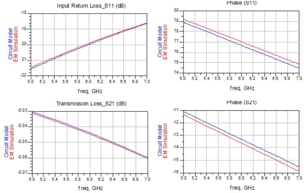
Figure 3-53: EM and Circuit Model Simulation Results of Spiral Inductor with Dimensions 250x300 \mu\text{m}
