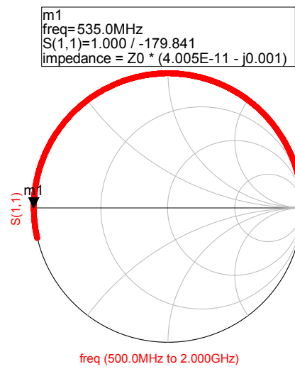
Figure 3-25: Simulation Result of Proposed Method in Figure 3-24-(a) on Smith Chart
