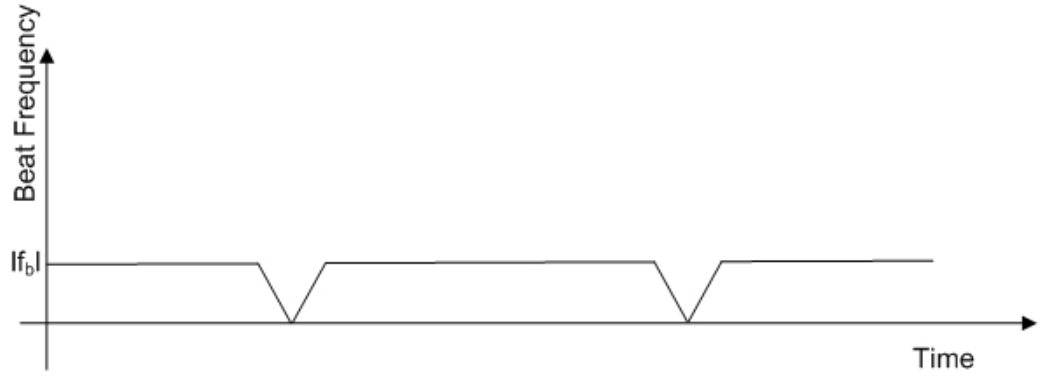
Figure 2-5: The beat frequency of triangular modulated signal
