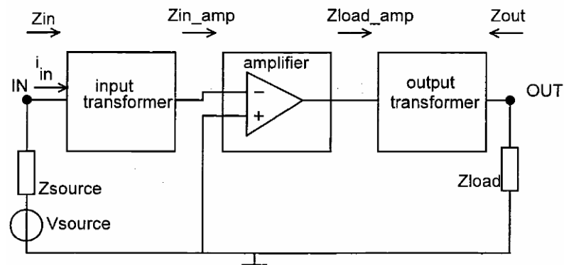
Figure 4-16: LNA with Input and Output Transformers
