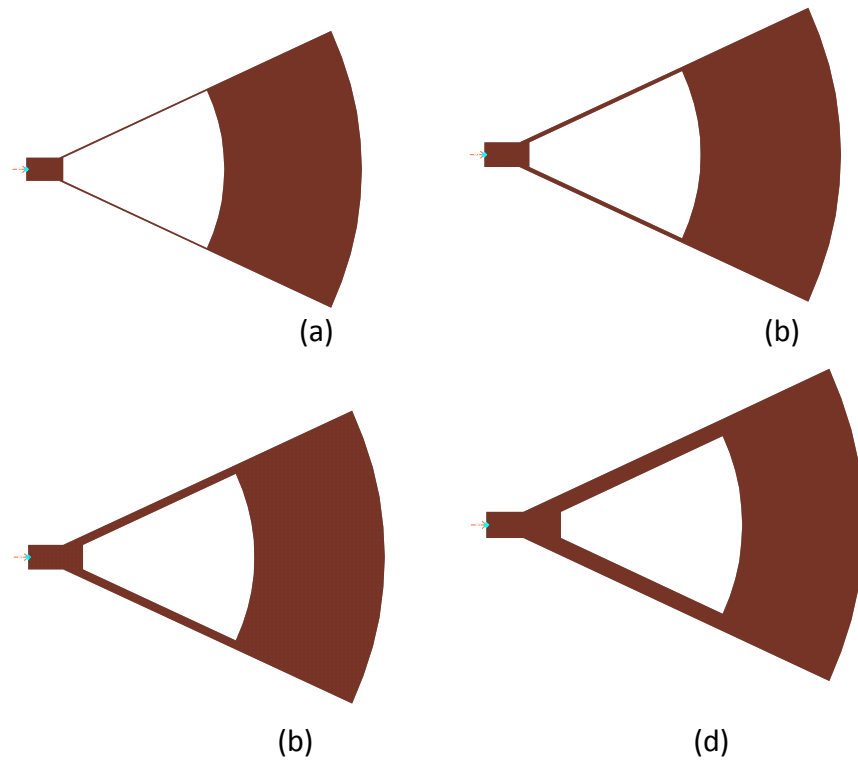
Figure 3-37: Layouts of 50° Miniaturized Radial Stub for Feedline Widths (a) 0.125mm, (b) 0.3mm, (c) 0.6mm, (d) 1mm
