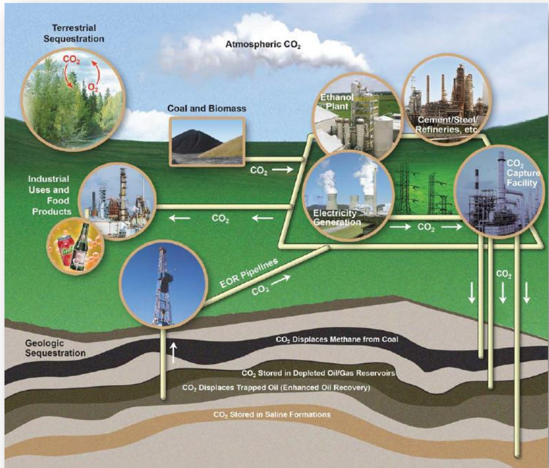
Figure 4: Schematic diagram of possible CCS systems (10)
