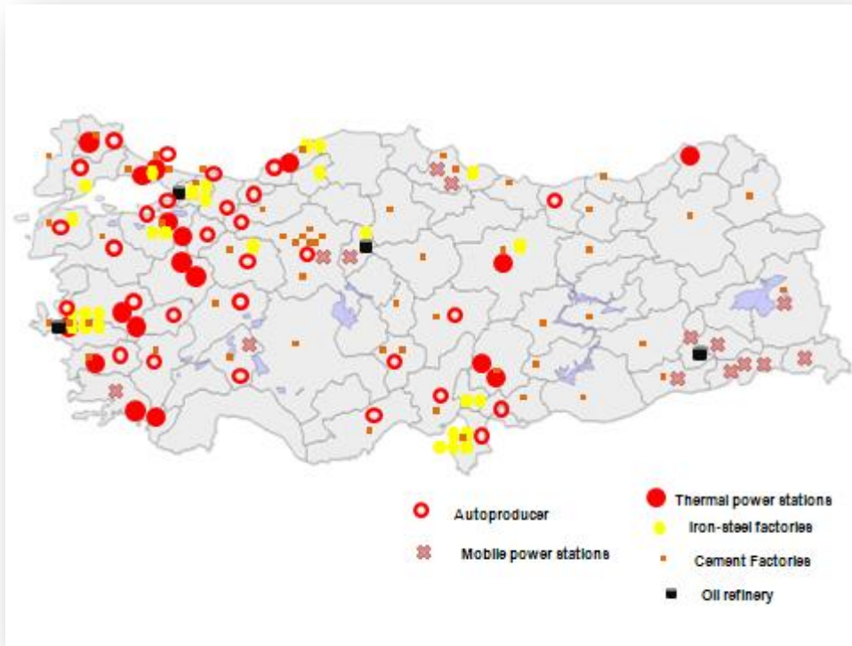
Figure 26: CO 2 Sources
