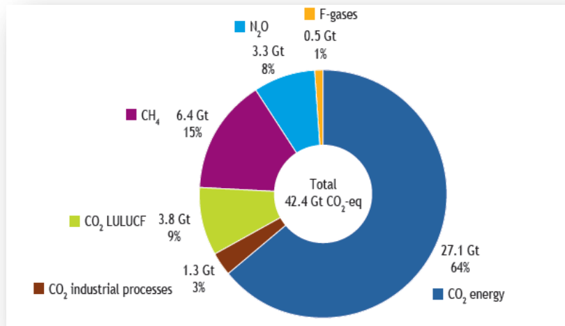
Figure 10: World anthropogenic greenhouse-gas emissions by source, 2005[3]
