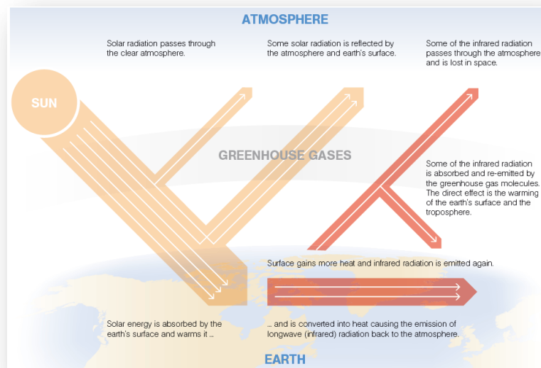
Figure 22: The green house effect [23]
