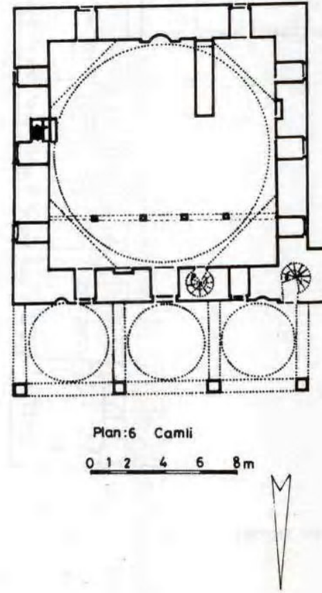
Plan 2.37. İncesu Merzifonlu Kara Mustafa Paşa
