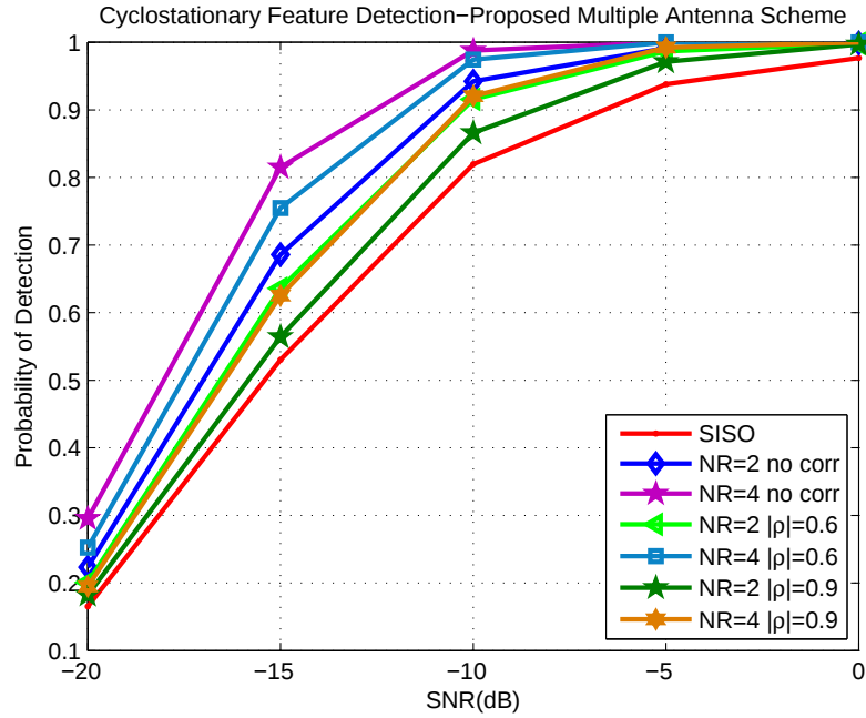
Figure 4.26. P_d vs. SNR for P_f = 0.01 -BPSK systems
