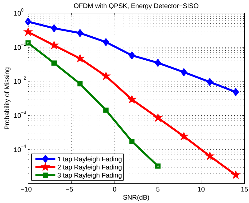
Figure 3.15. P_m vs. SNR for SISO -OFDM with QPSK
