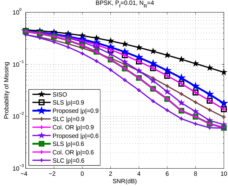
Figure 4.18. P_m vs. SNR for BPSK correlated SIMO systems
