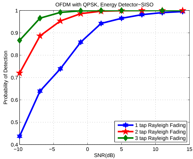
Figure 3.16. P_d vs. SNR for SISO-OFDM with QPSK
