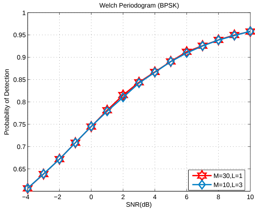
Figure 3.8. P_d vs. SNR using Welch Periodogram with different M,L values - BPSK
