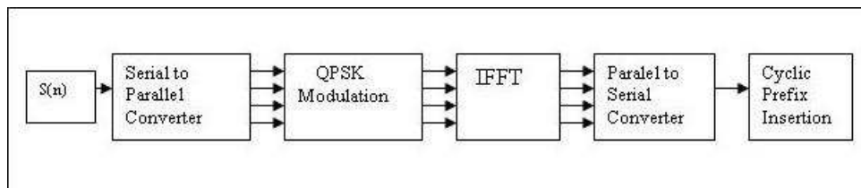
Figure 2.3. OFDM transmitter
