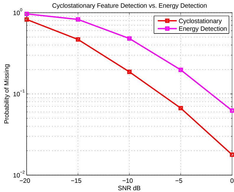
Figure 3.23. Probability of Missing, Cyc. Feature Detection vs. Energy Detection
