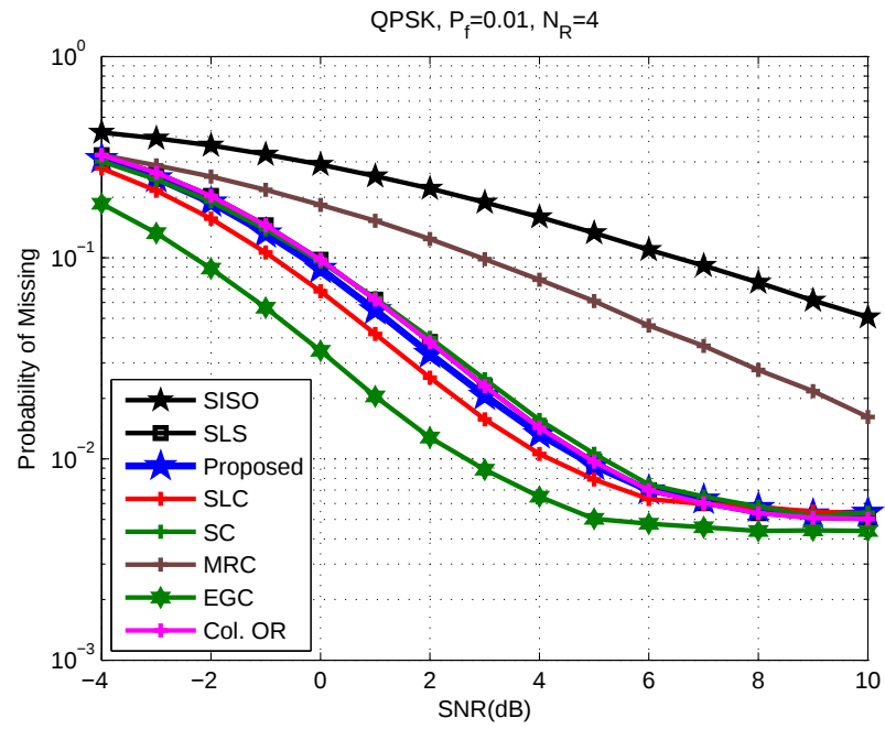
Figure 4.12. P_m vs. SNR for QPSK SIMO systems
