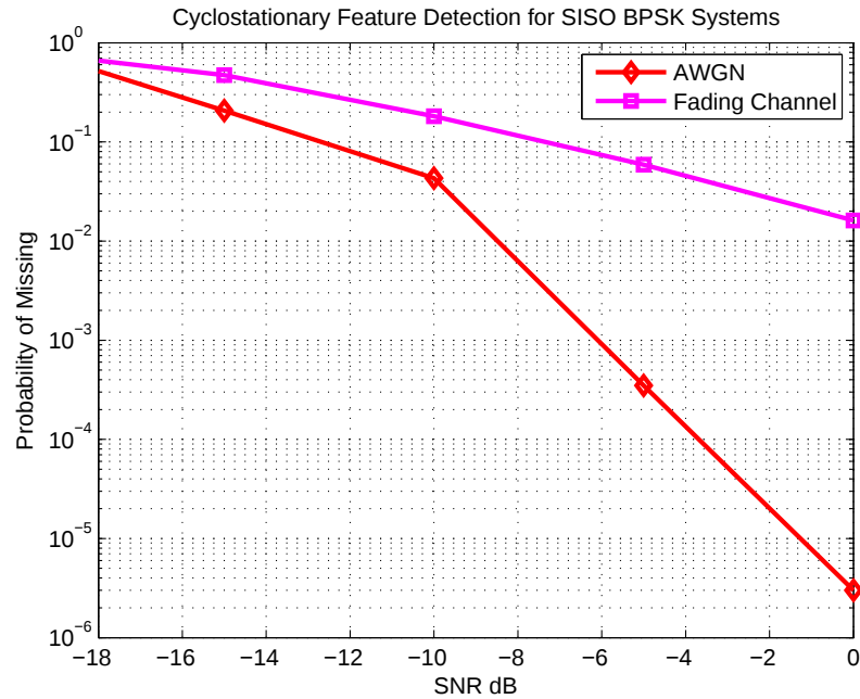
Figure 3.20. P_m under P_f = 0.01 for SISO-BPSK
