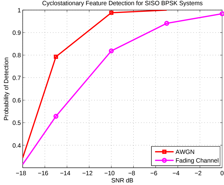
Figure 3.21. P_d under P_f = 0.01 for BPSK modulated symbols
