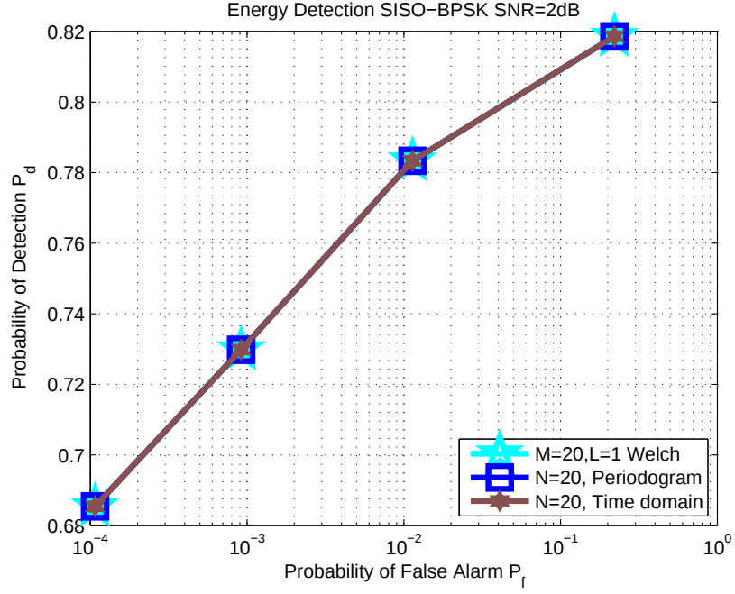
Figure 3.7. Probability of Detection vs. Probability of False alarm - BPSK
