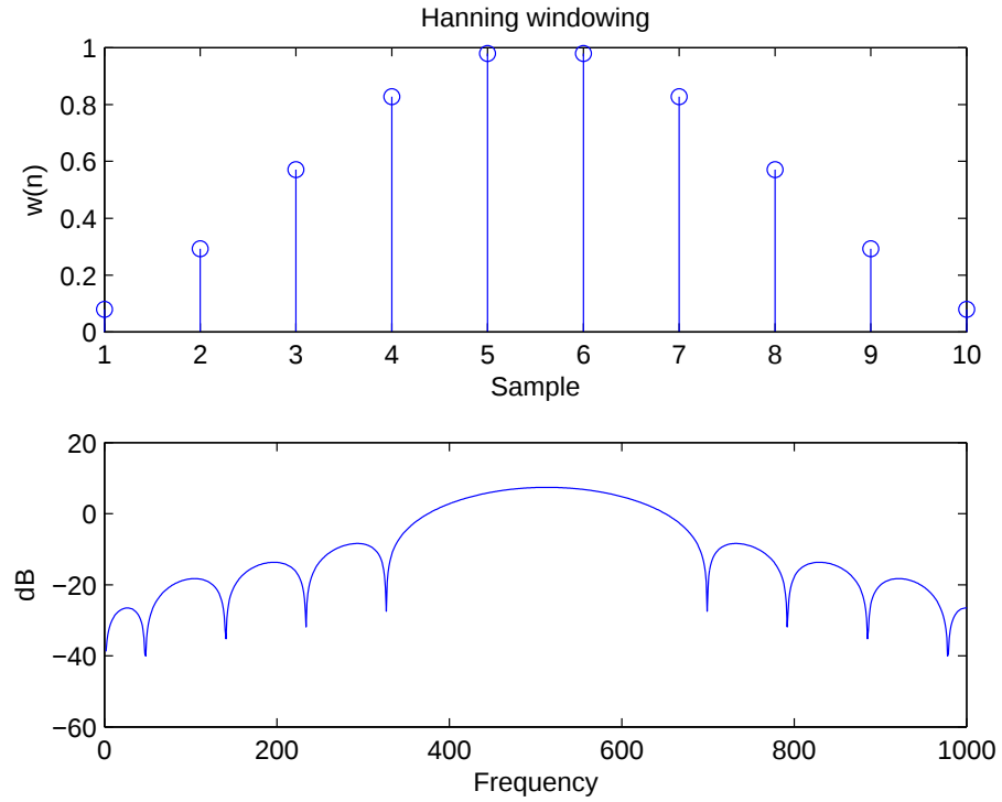
Figure 3.17. Hanning window.
