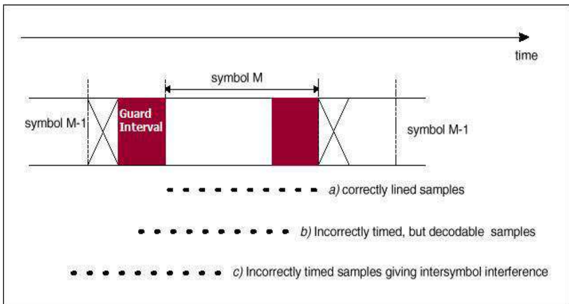
Figure 2.4. Cyclic Prefix Insertion
