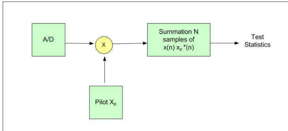
Figure 3.3. Pilot Detection via Matched Filtering
