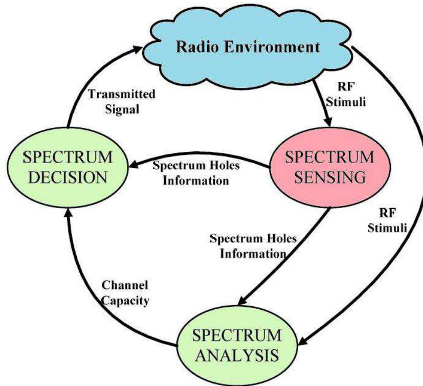
Figure 2.8. Cognitive Cycle
