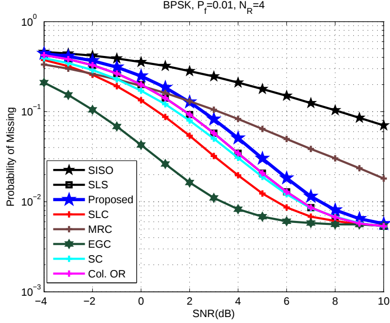
Figure 4.9. P_m vs. SNR for BPSK SIMO systems
