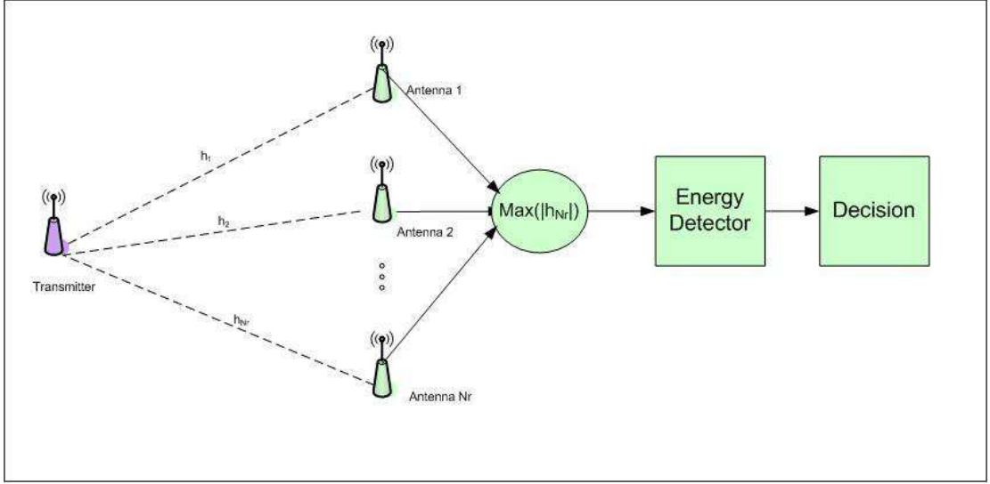
Figure 4.1. Selection Combining with Channel State Information
