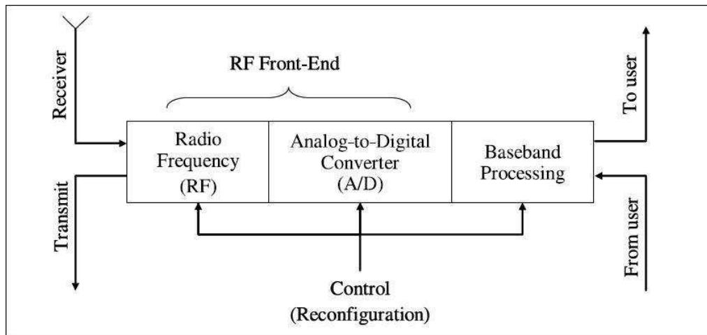
Figure 2.6. Cognitive Radio Transceiver
