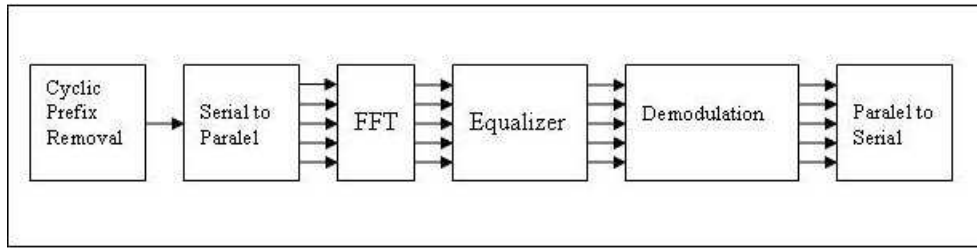
Figure 2.5. OFDM receiver
