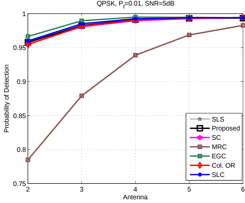
Figure 4.14. P_d vs. Antenna Number for QPSK SIMO systems
