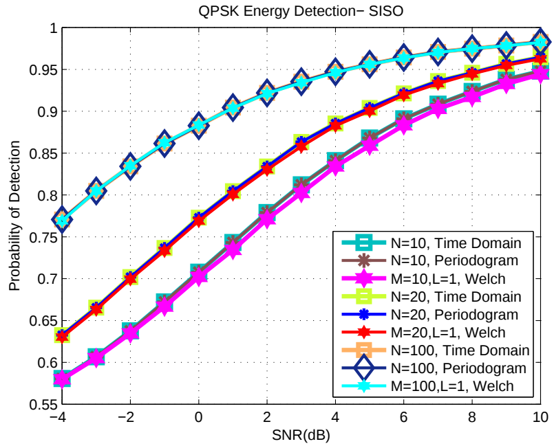
Figure 3.13. P_d vs. SNR for SISO-QPSK using different energy detection algorithms
