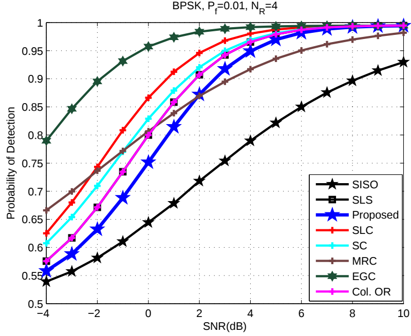
Figure 4.10. P_d vs. SNR for BPSK SIMO systems
