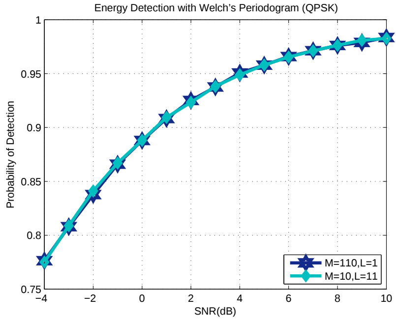
Figure 3.12. P_d of Welch Periodogram using different M,L values -QPSK
