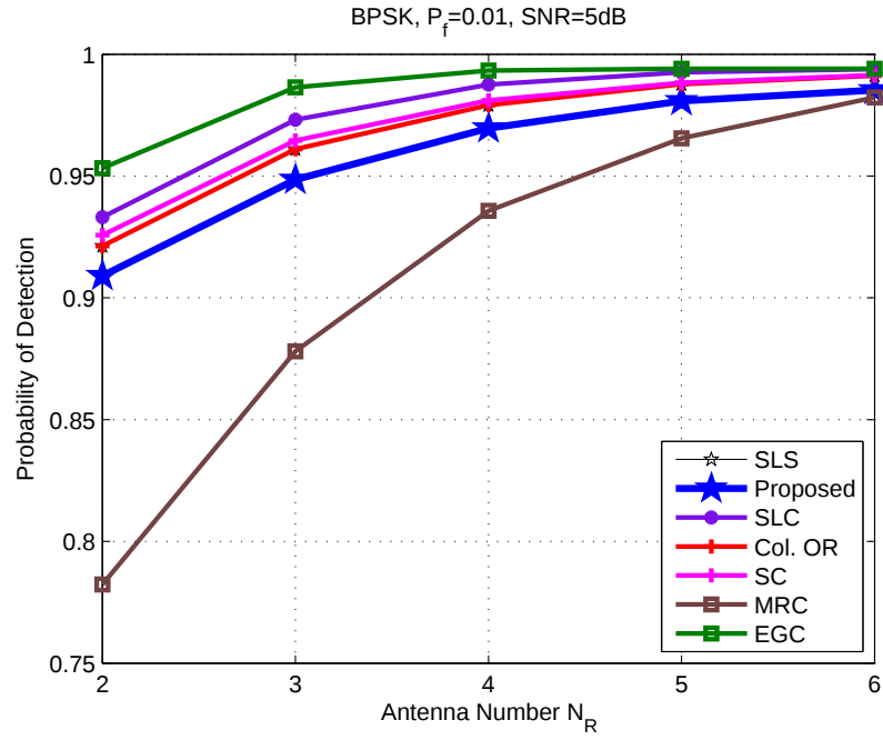
Figure 4.11. P_d vs. Antenna Number for BPSK SIMO systems
