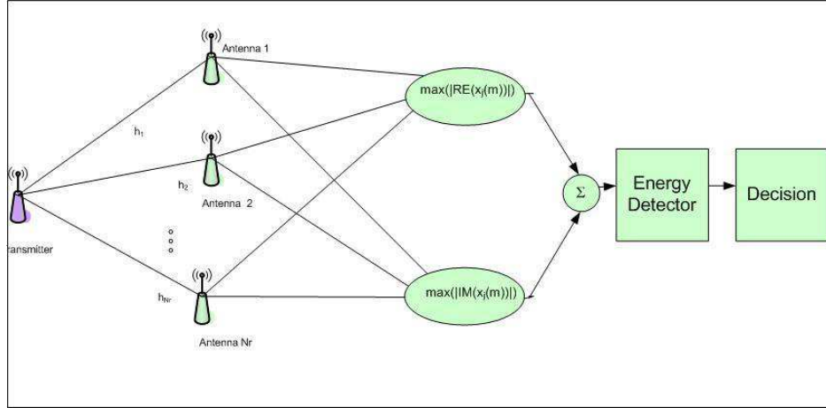
Figure 4.8. Proposed Maximum Selection
