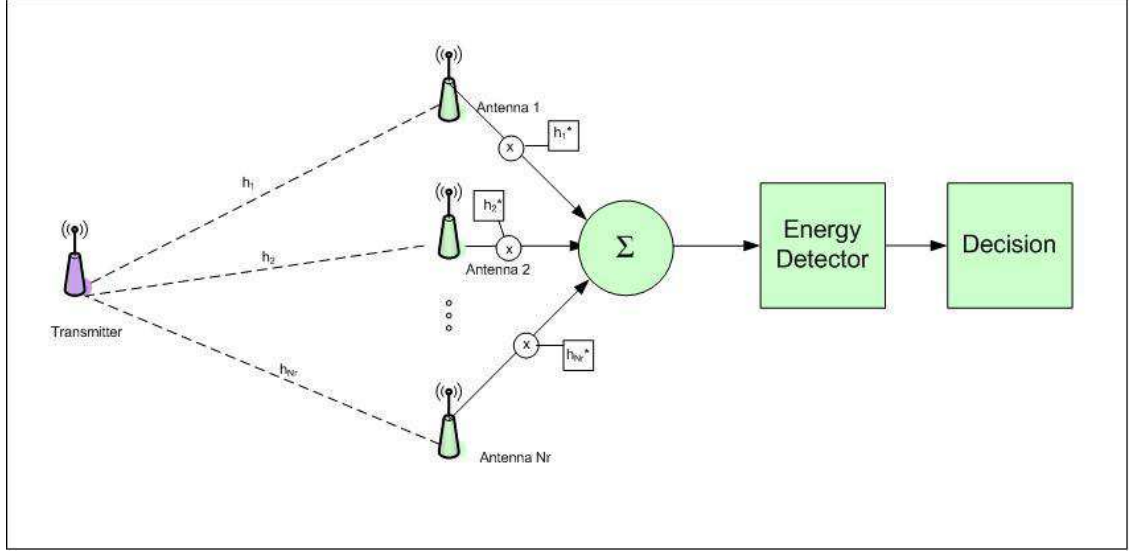
Figure 4.2. Maximum Ratio Combining
