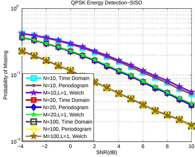
Figure 3.14. P_m vs. SNR for SISO-QPSK using different energy detection algorithms
