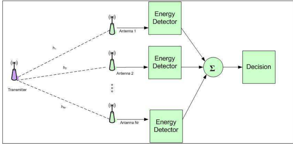
Figure 4.4. Square Law Combining
