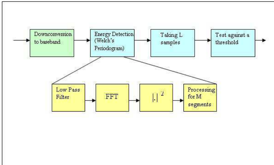
Figure 3.5. Energy Detection with Welch's Periodogram
