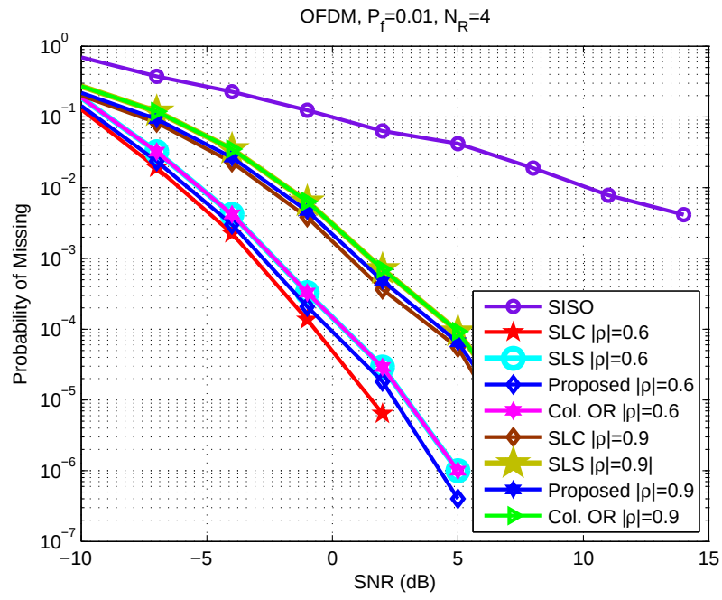
Figure 4.23. P_m vs. SNR for OFDM correlated SIMO systems
