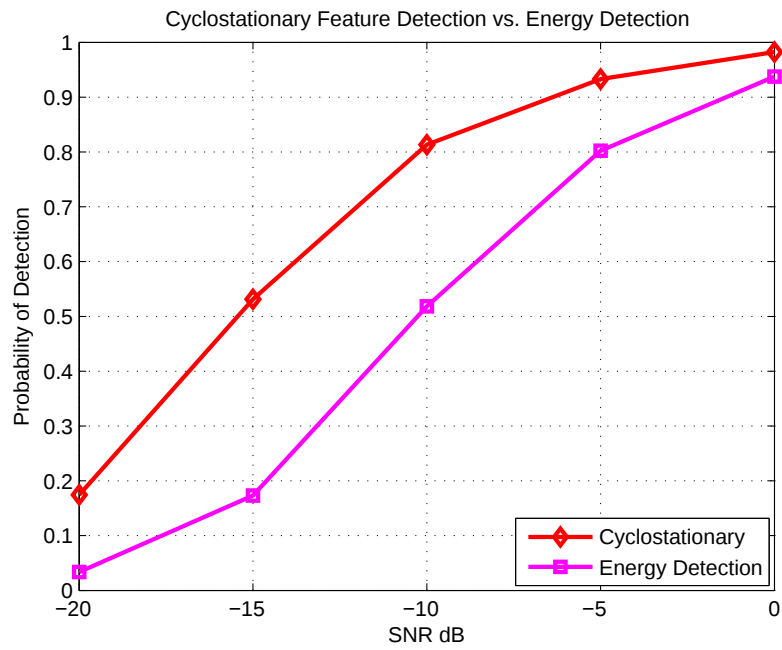
Figure 3.22. Probability of Detection, Cyc. Feature Detection vs. Energy Detection
