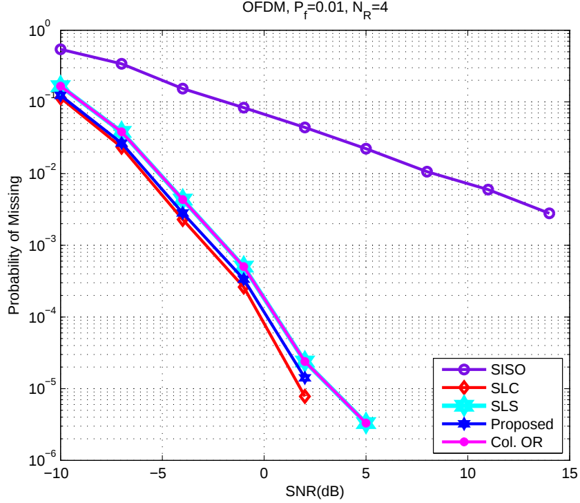
Figure 4.15. P_m vs. SNR for OFDM SIMO systems
