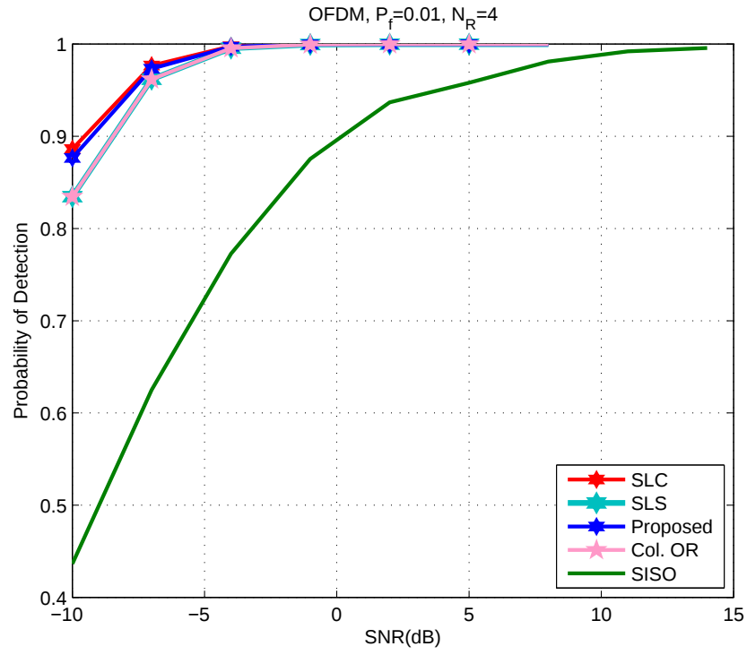
Figure 4.16. P_d vs. SNR for OFDM SIMO systems with QPSK
