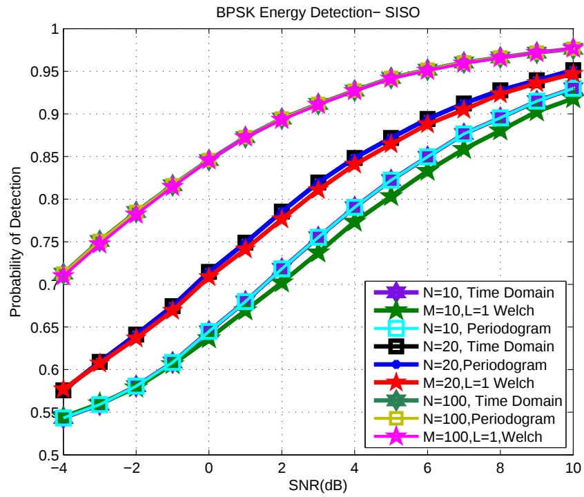
Figure 3.9. P_d vs. SNR for SISO-BPSK using different energy detection algorithms
