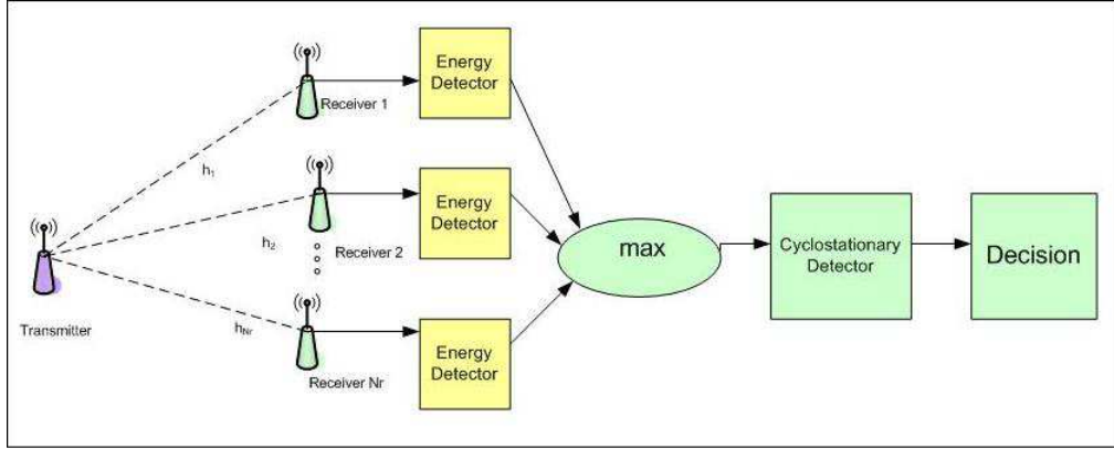
Figure 4.25. Proposed Scheme
