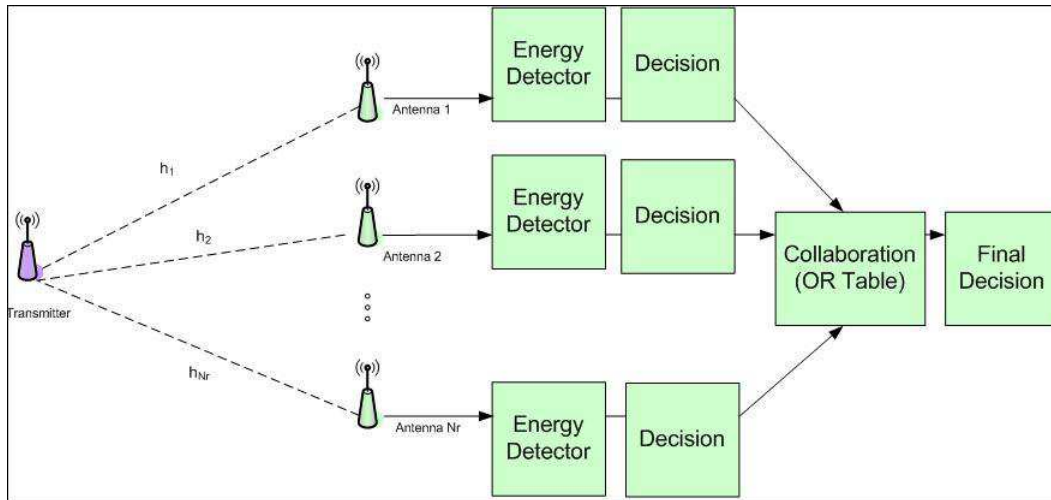
Figure 4.6. Collaborative Spectrum Sensing
