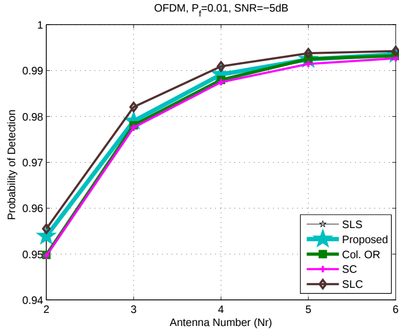
Figure 4.17. P_d vs. Antenna Number for OFDM SIMO systems
