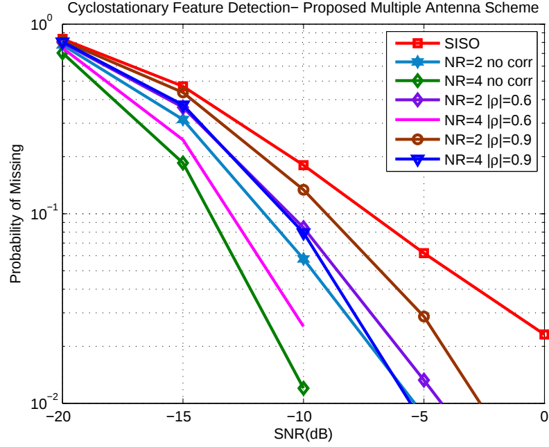
Figure 4.27. P_m vs. SNR for P_f = 0.01 -BPSK systems
