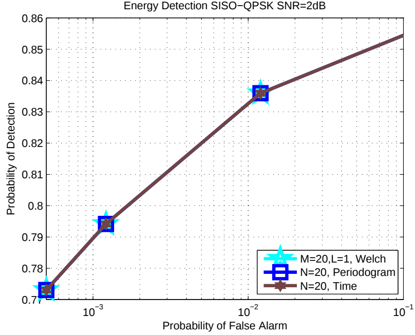
Figure 3.11. Probability of Detection vs. Probability of False alarm - QPSK
