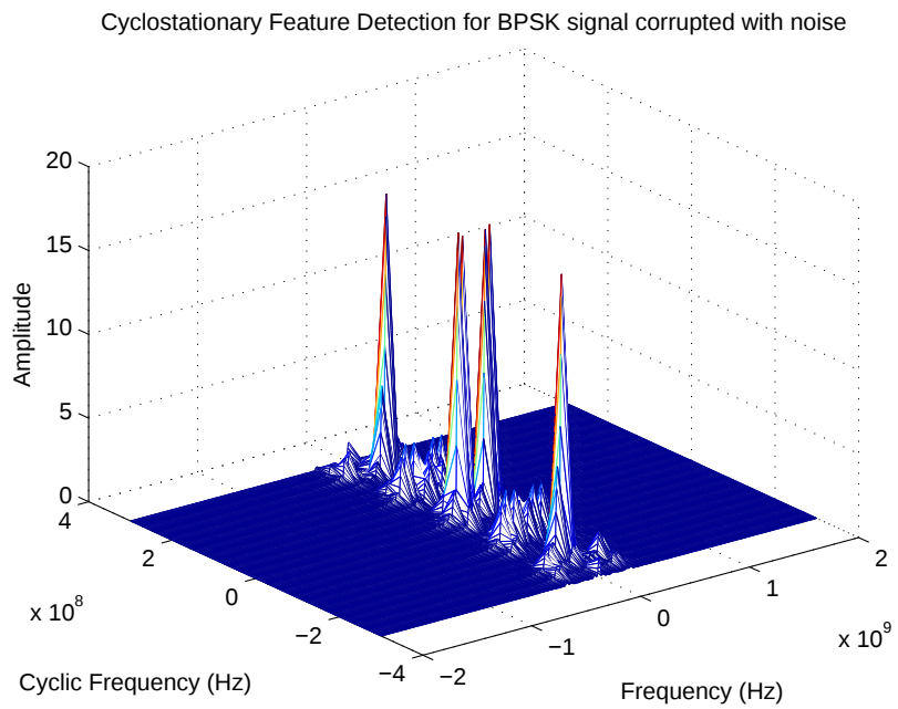
Figure 3.18. Cyclic Spectrum of BPSK signal with AWGN Noise
