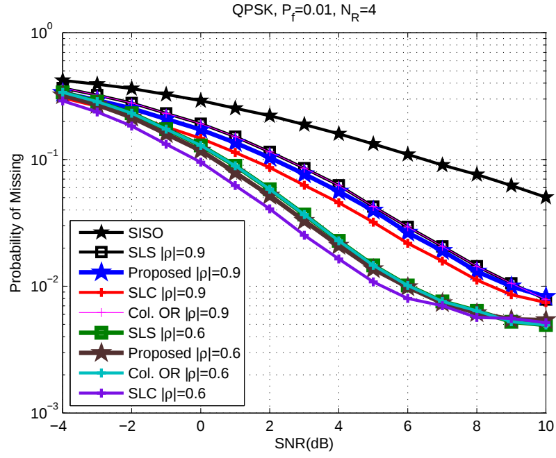
Figure 4.20. P_m vs. SNR for QPSK correlated SIMO systems
