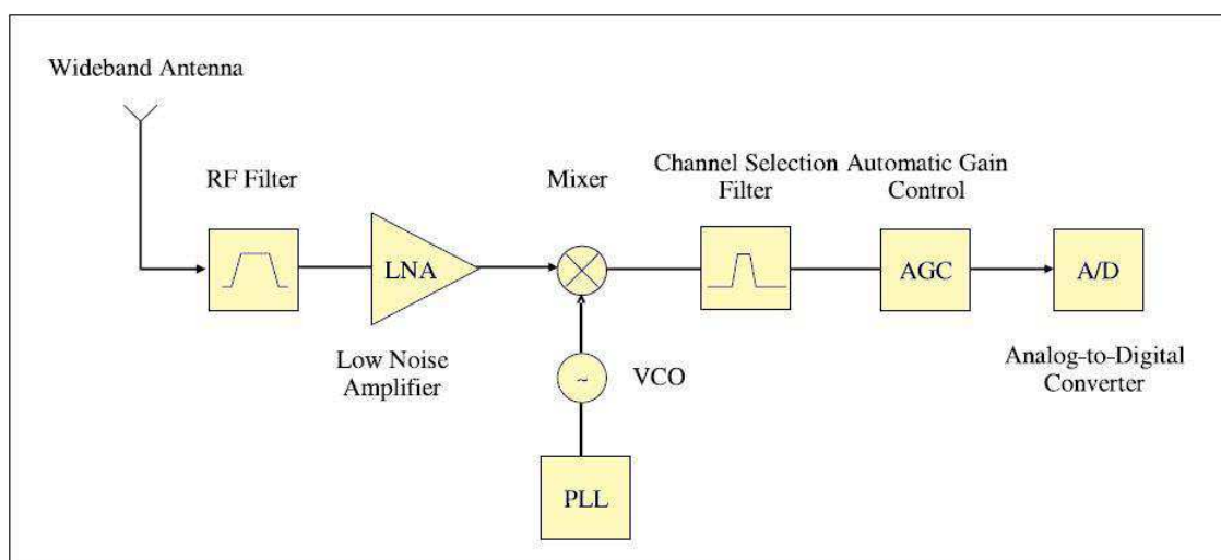
Figure 2.7. Wideband RF/ Analog Front-end
