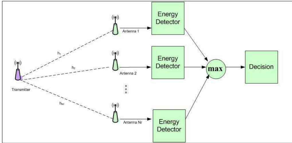
Figure 4.5. Square Law Selection
