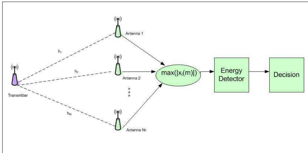
Figure 4.7. Proposed Maximum Selection
