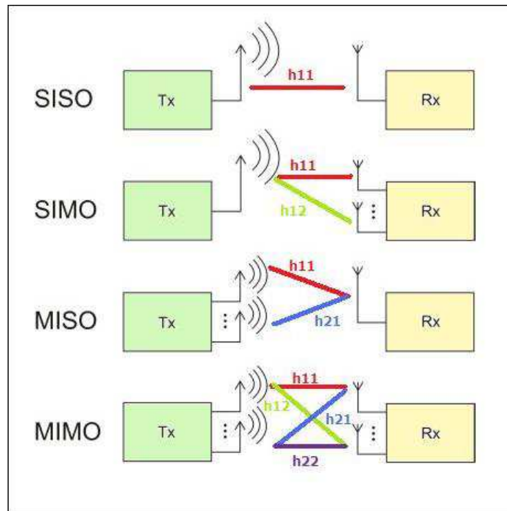
Figure 2.2. Multiple Antenna Techniques
