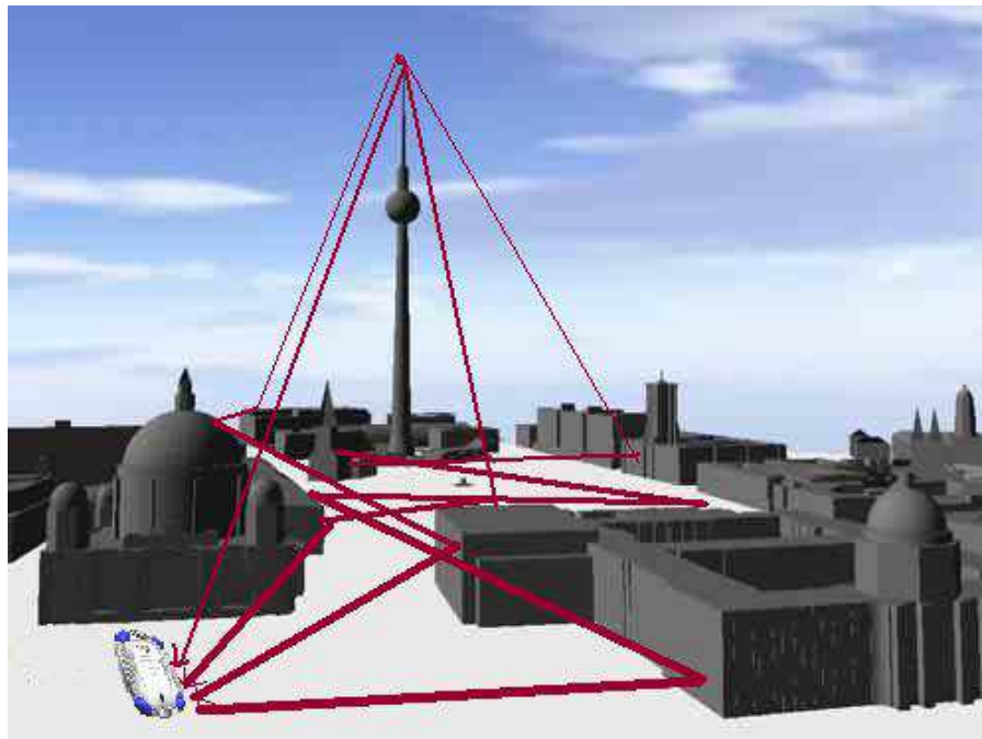
Figure 2.1. Multipath Propagation
