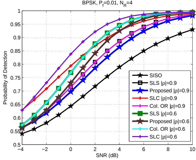
Figure 4.19. P_d vs. SNR for BPSK correlated SIMO systems
