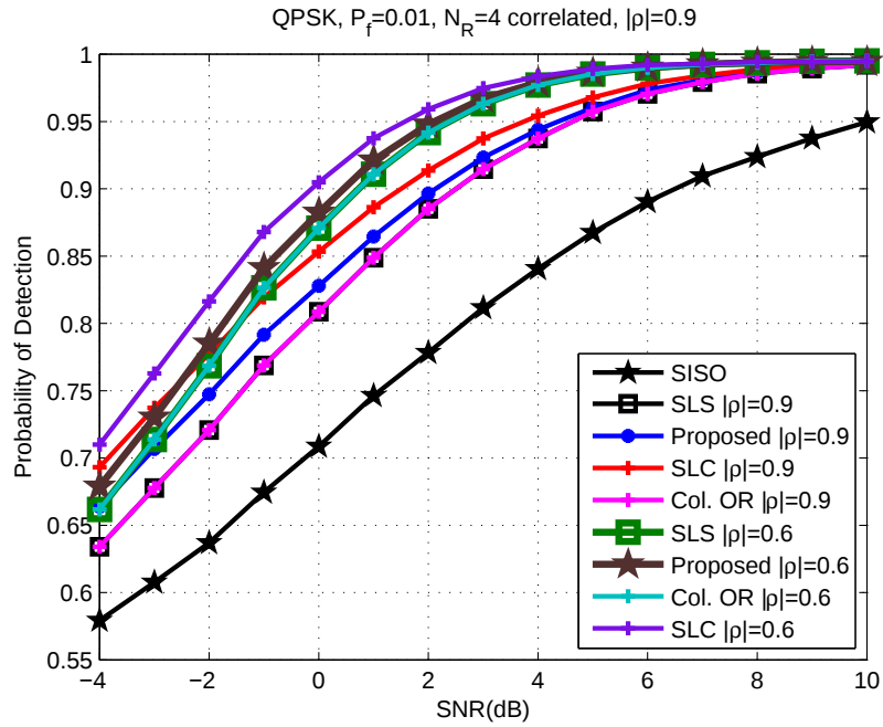
Figure 4.21. P_d vs. SNR for QPSK correlated SIMO systems
