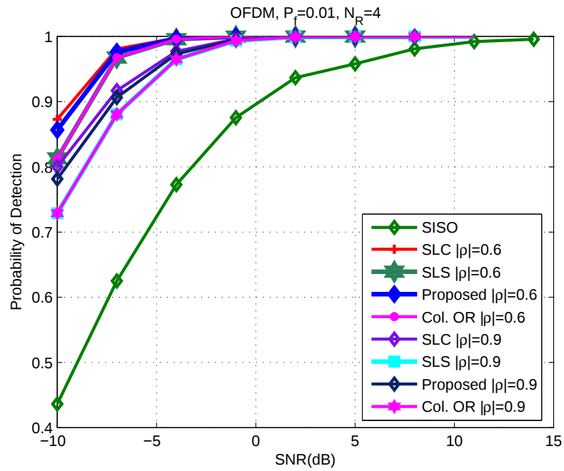
Figure 4.24. P_d vs. SNR for OFDM correlated SIMO systems
