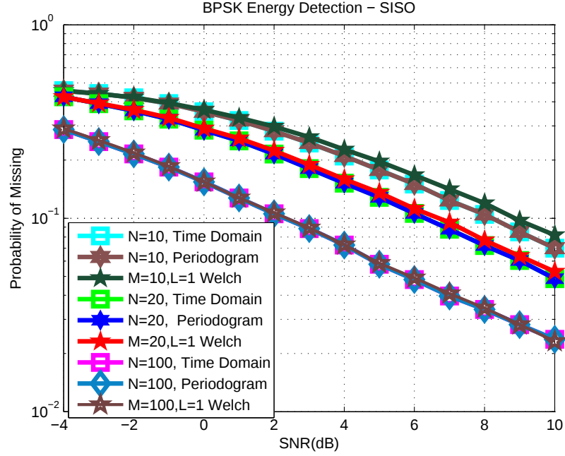
Figure 3.10. P_m vs. SNR for SISO-BPSK using different energy detection algorithms
