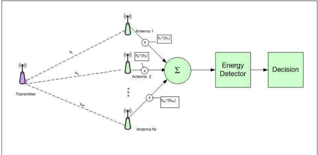
Figure 4.3. Equal Gain Combining
