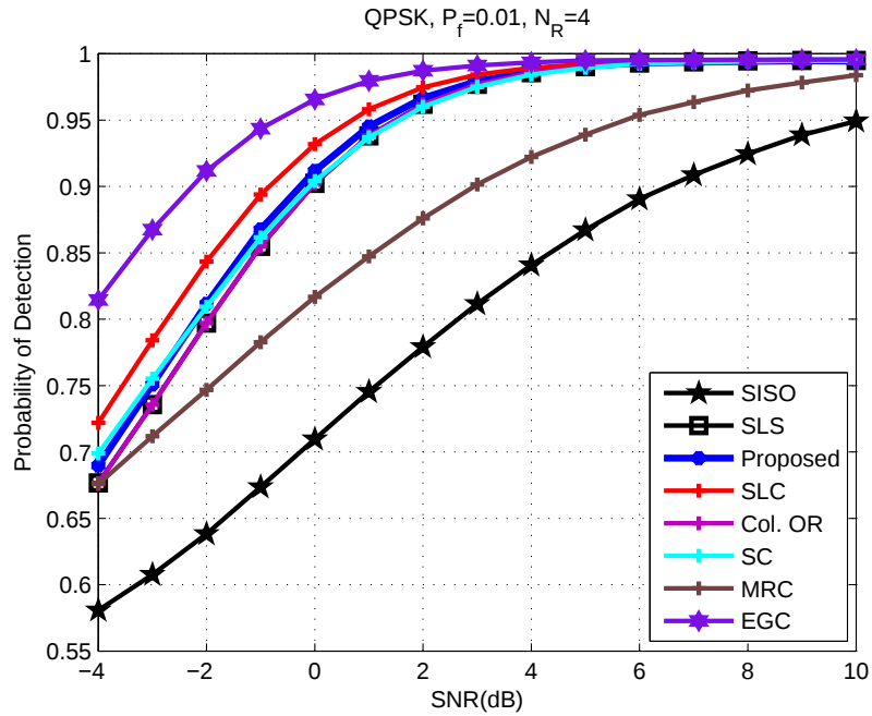
Figure 4.13. P_d vs. SNR for QPSK SIMO systems
