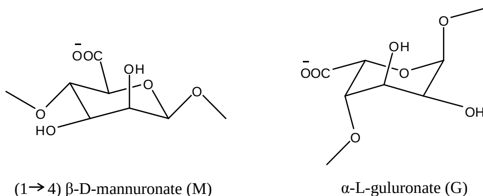
Figure 6 The chemical structures of β-D-mannuronic acid and α-L-guluronic acid units of alginate.
