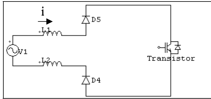
Figure 4.2 Equivalent circuit when switching transistor on and mains supply's voltage phase is between 0 and 180^\circ .
