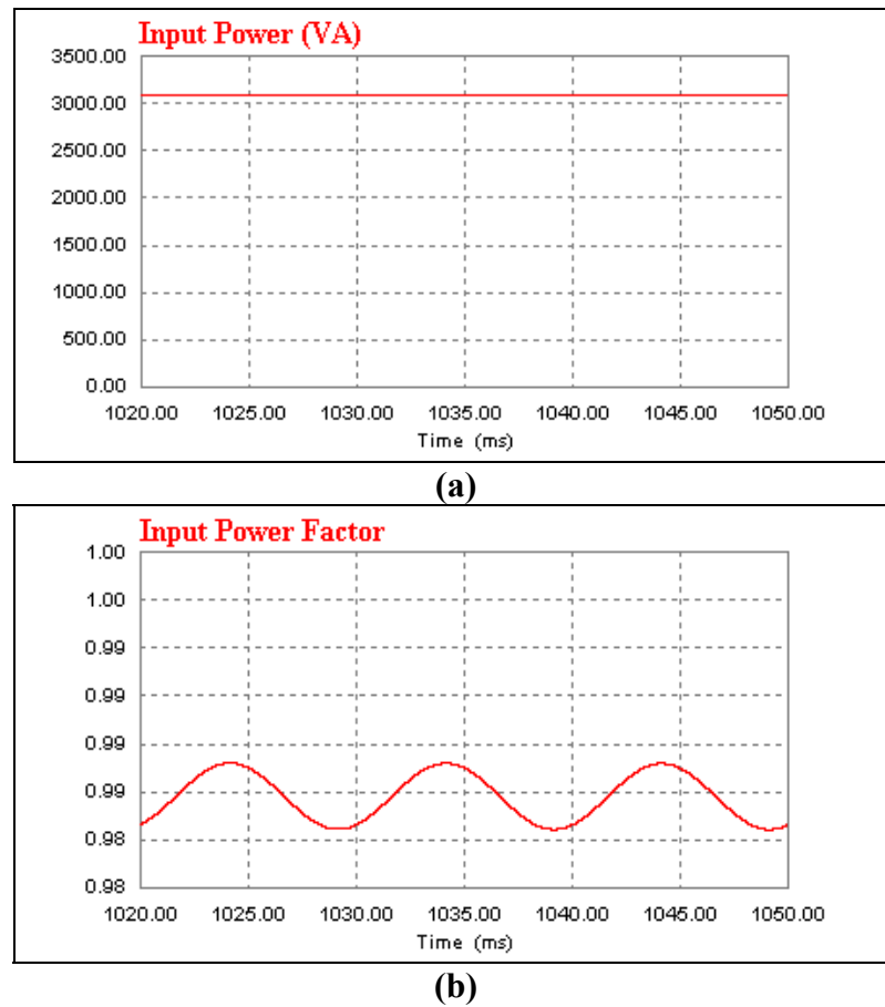
Figure D.1 Classical unity power factor rectifier's input power and power factor at purely resistive 3 kW load, (a) its input power, (b) its power factor graph.
