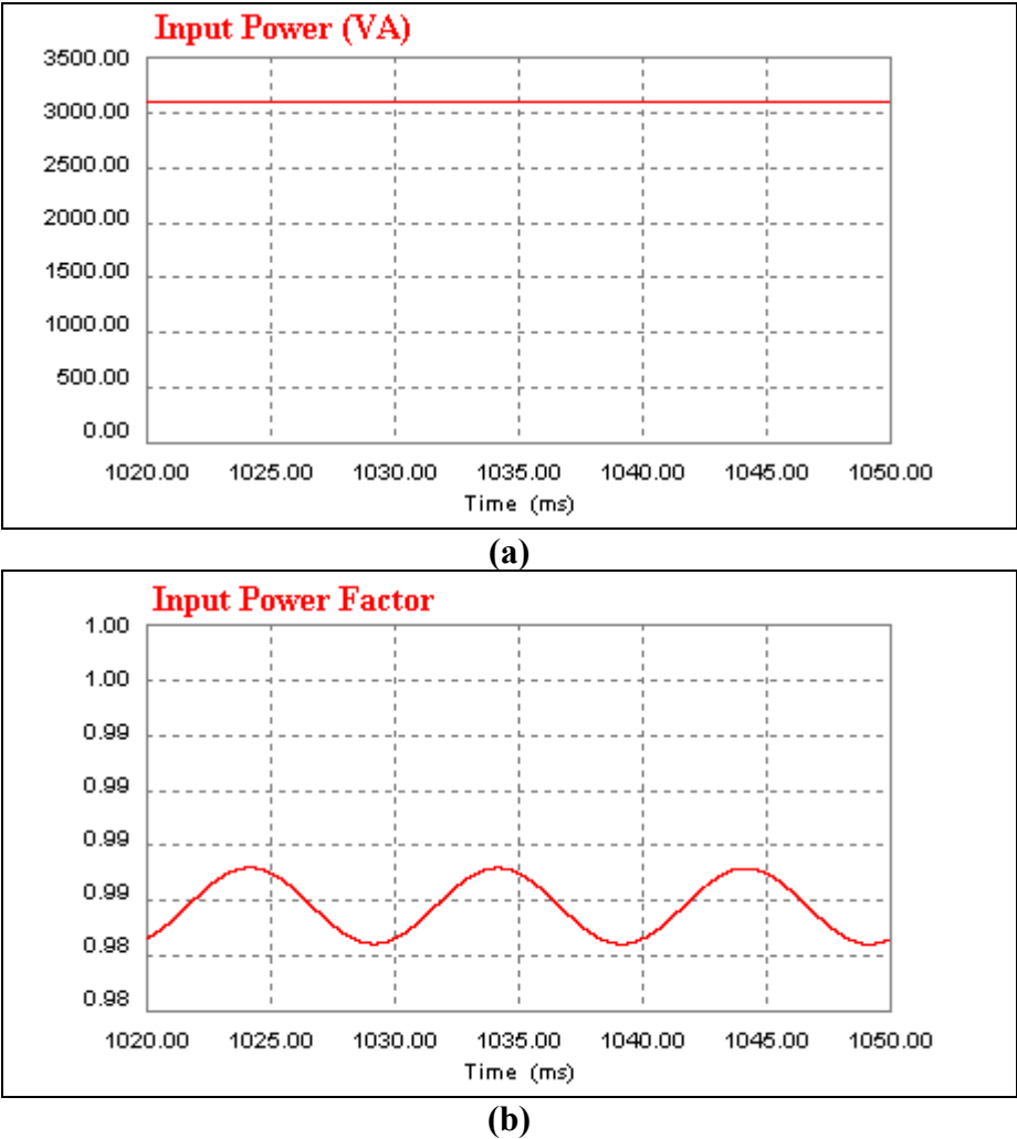
Figure D.20 Classical unity power factor rectifier's input power and power factor at inductive-resistive 3 kW load (10 \mu H), (a) its input power, (b) its power factor.
