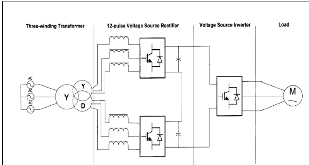
Figure 2.12 Main circuit of the voltage source converter drive system.
