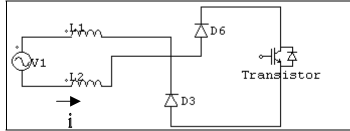
Figure 4.4 Equivalent circuit when mains supply's voltage phase is between 180^\circ and 360^\circ , switching transistor is on.
