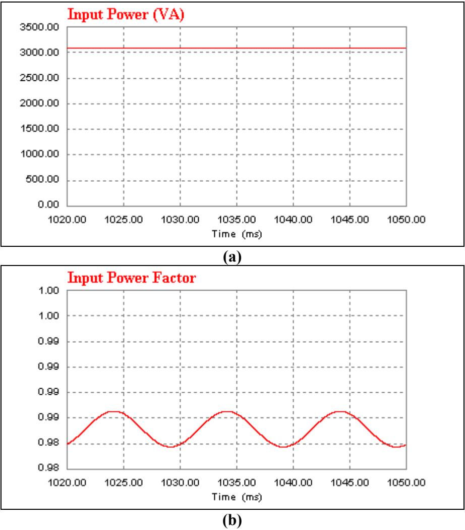
Figure D.23 Proposed rectifier's input power and power factor at inductive-resistive 3 kW load (100 \mu H), (a) its input power, (b) its power factor.
