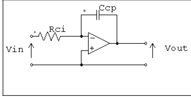
Figure 7.13 An integrator.
