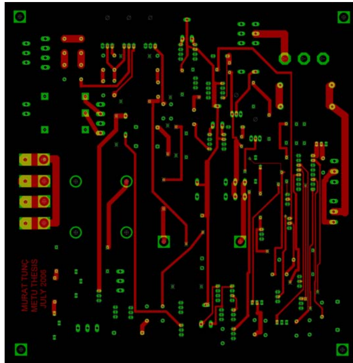
Figure E.2 Classical unity power factor rectifier and proposed rectifier's printed circuit board's top layer.
