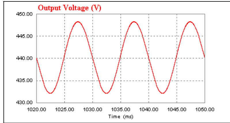
Figure 6.21 Proposed rectifier's output voltage waveform with 3 kW inductive-resistive load (100 \mu H) at steady state.
