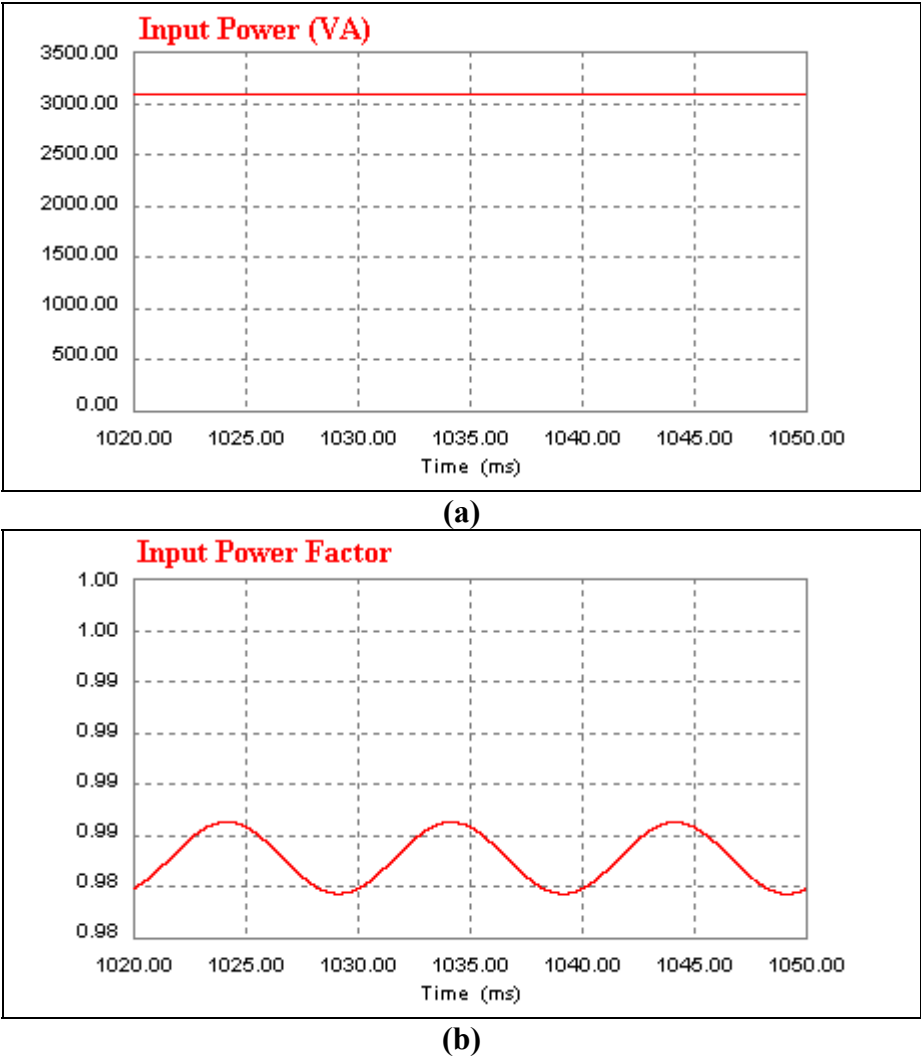
Figure D.30 Proposed rectifier's input power and power factor at inductive-resistive 3 kW load (10 uH), (a) its input power, (b) its power factor.
