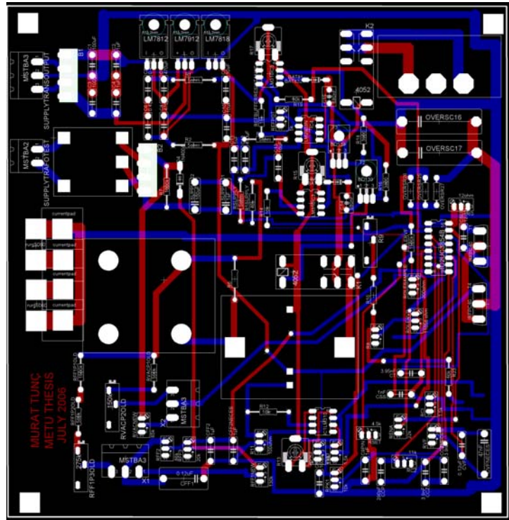
Figure E.1 Classical unity power factor rectifier and proposed rectifier's printed circuit board.
