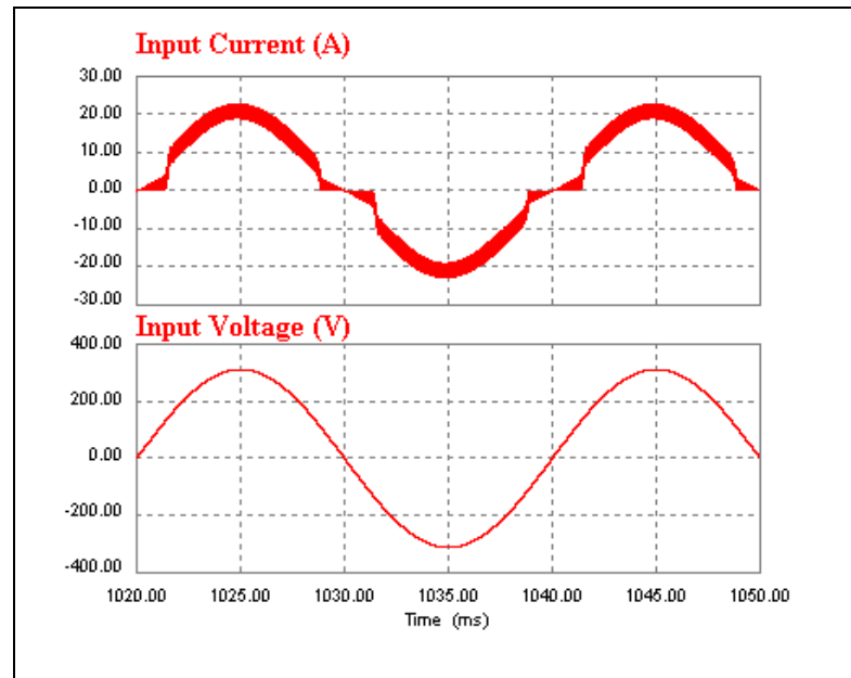
Figure 6.22 Proposed rectifier's input voltage and current waveform with 3 kW inductive-resistive load (10 \mu\text{H} ) at steady state.
