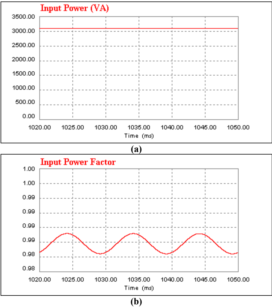
Figure D.14 Classical unity power factor rectifier's input power and power factor at inductive-resistive 3 kW load (100 \mu H), (a) its input power, (b) its power factor.
