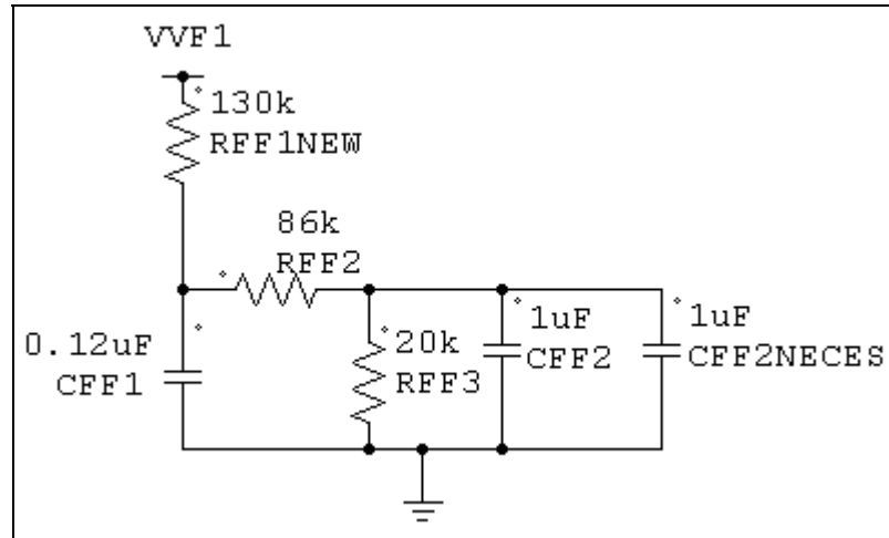
Figure 7.11 Low pass filter in proposed rectifier circuit.
