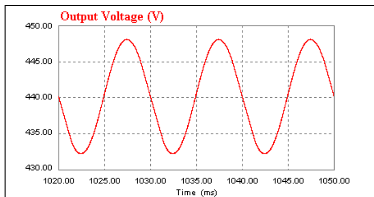
Figure 6.17 Classical unity power rectifier's output voltage waveform with 3 kW inductive-resistive load (100 \mu\text{H} ) at steady state.
