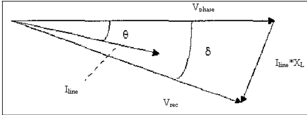
Figure 2.13 Phasor diagram of front-end voltage source converter.
