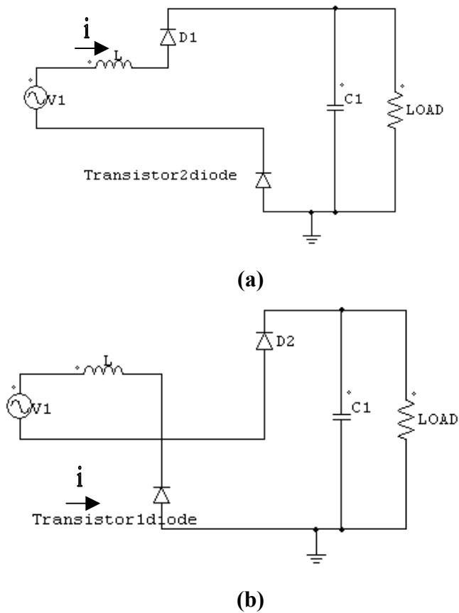
Figure 4.11 Low conduction loss AC/DC UPF rectifier's equivalent circuit when the switching transistor is off (a) mains supply's voltage phase is between 0 and 180^\circ , (b) mains supply's voltage phase is between 180 and 360^\circ .
