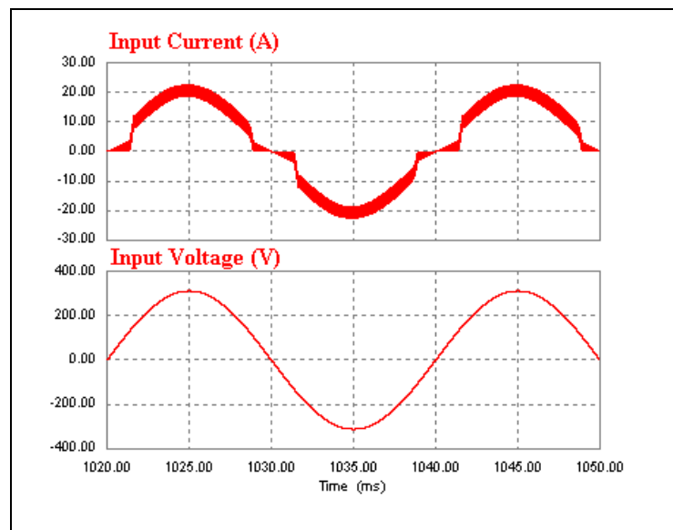
Figure 6.16 Classical unity power rectifier's input voltage and current waveform with 3 kW inductive-resistive load (100 \mu\text{H} ) at steady state.
