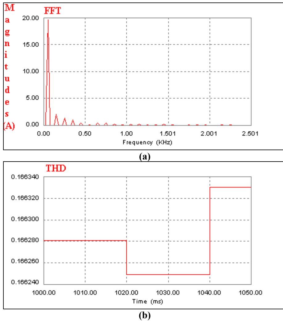
Figure D.35 The classical unity power factor rectifier's input current FFT and THD graph obtained with 3 kW purely resistive load by taking reference voltage from a transformer connected to mains supply, (a) its FFT waveform (b) its THD graph.
