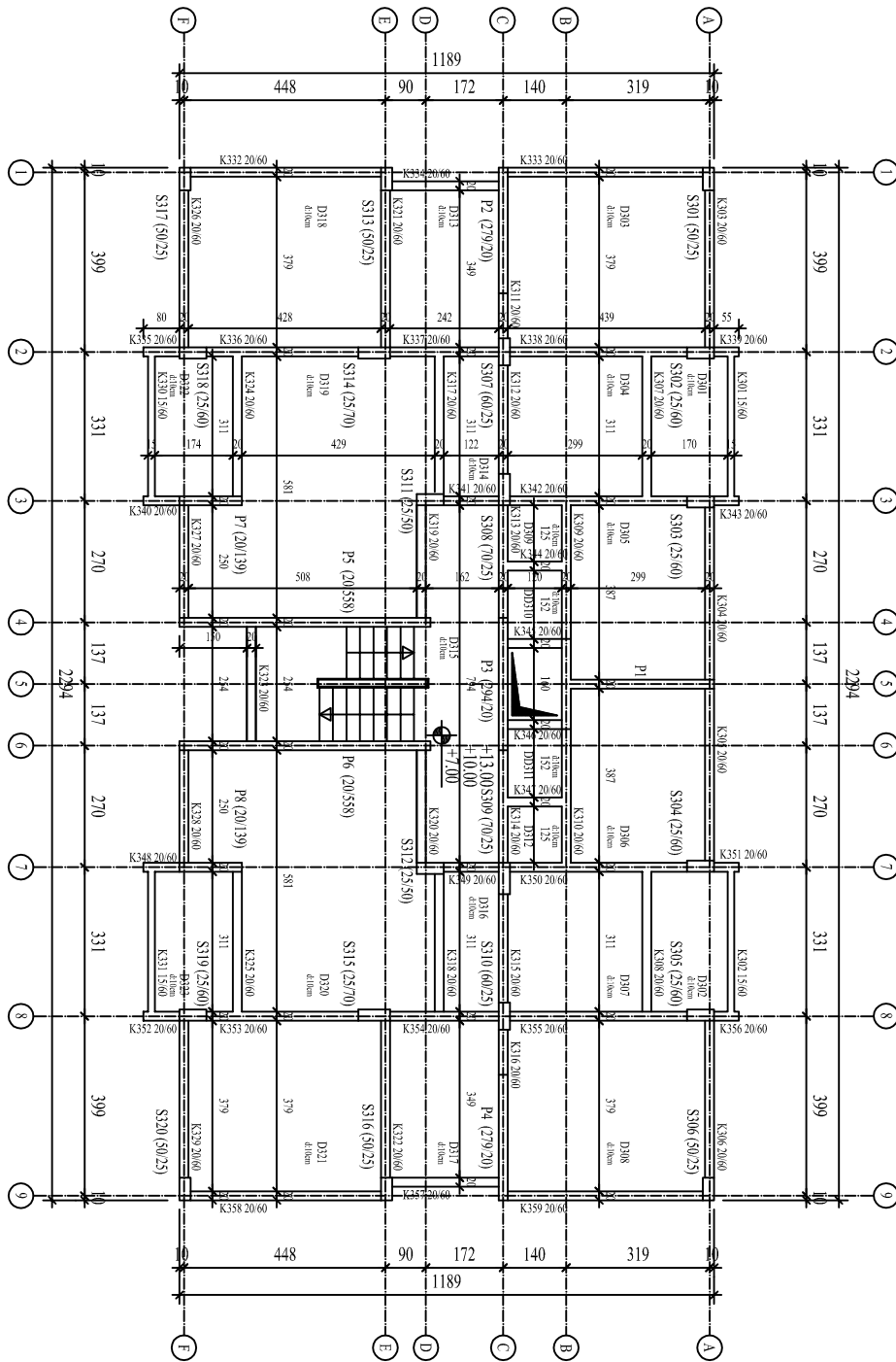
Figure B.3 The structural project of 1 st , 2 nd , and 3 rd floor ceilings
