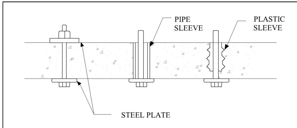
Figure 2.3 Bolted connections [6]
