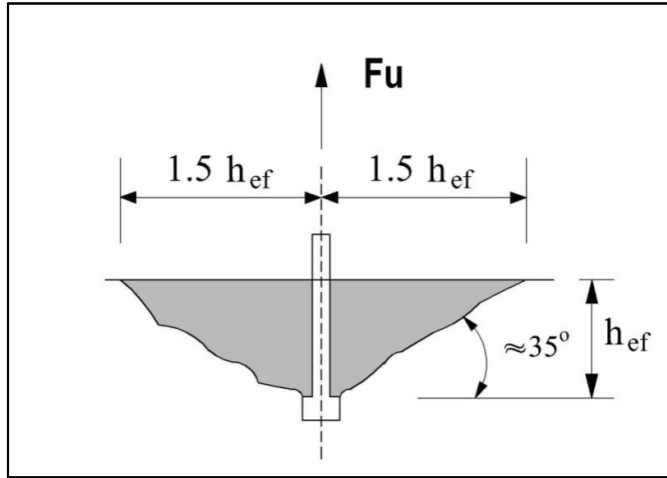
Figure 2.17 Concrete cone failure [17]
