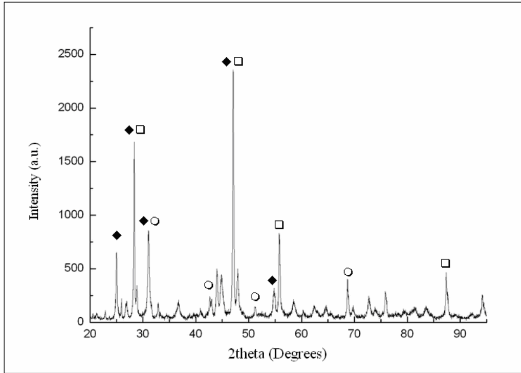
◆: Bastnasite □: CaF 2 ○: BaSO 4 Figure 3.2. XRD pattern of bastnasite preconcentrate
