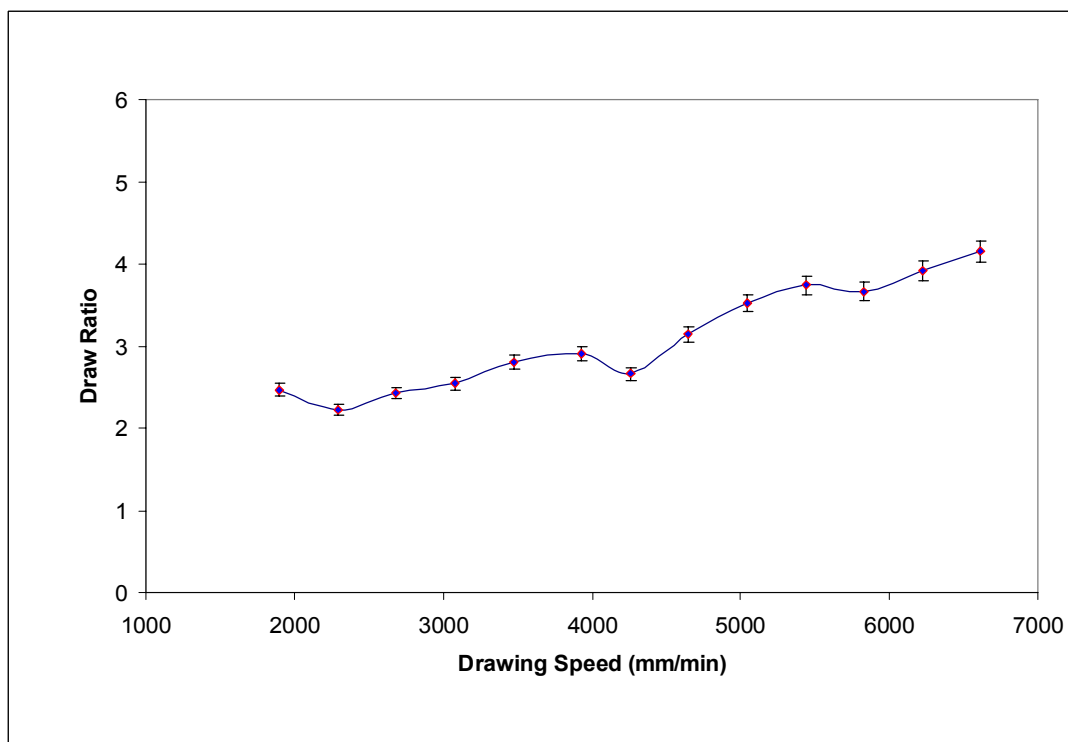
Figure A.3. Effect of drawing speed on draw ratio of PET/HDPE sample processed at 180 rpm and drawn at room temperature ( \sim 20^{\circ}\text{C} )
