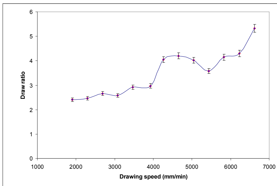
Figure A.2. Effect of drawing speed on draw ratio of PET/HDPE sample processed at 120 rpm and drawn at room temperature ( \sim 20^{\circ}\text{C} )
