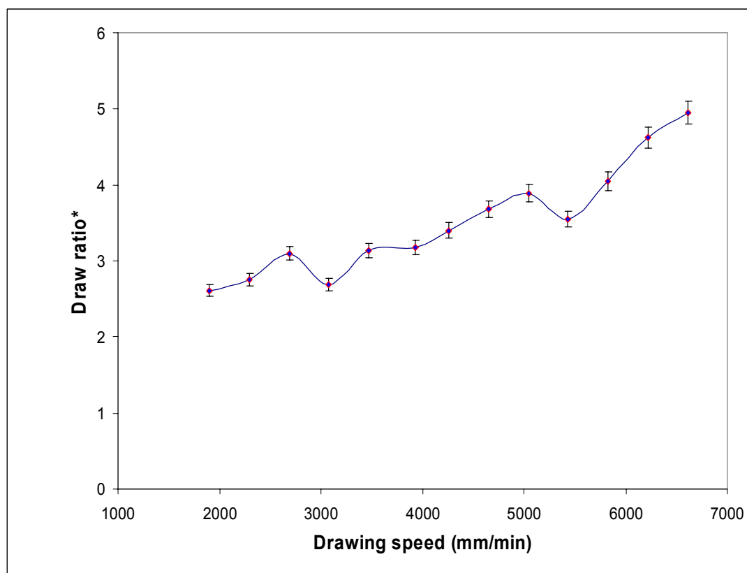
Figure A.1. Effect of drawing speed on draw ratio of PET/HDPE sample processed at 60 rpm and drawn at room temperature ( \sim 20^{\circ}\text{C} )
