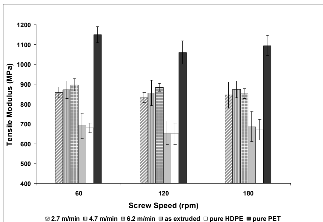
Figure 4.16 Tensile modulus versus screw speed
