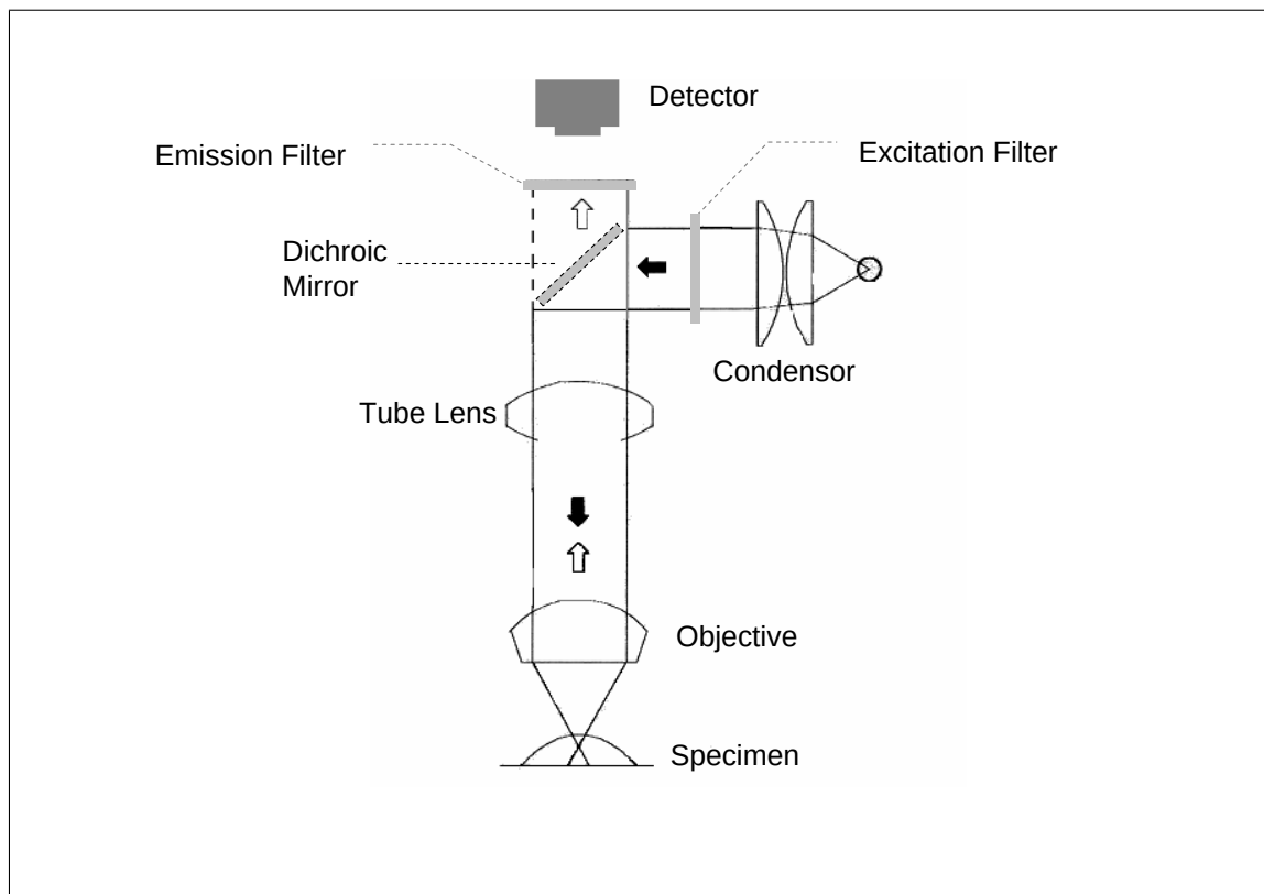
Figure B.1 Epifluorescence microscope and its main components
