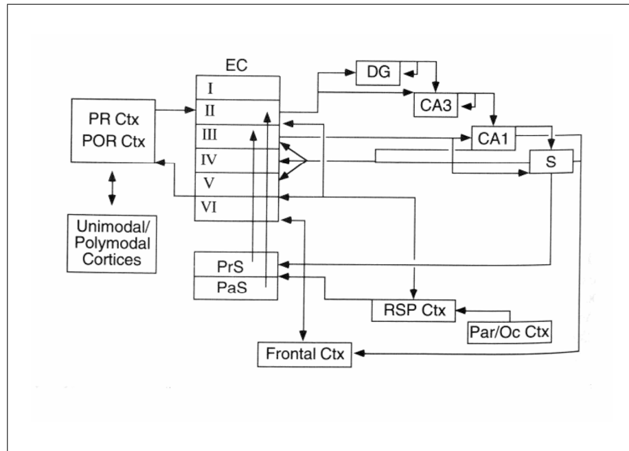
Figure 2.3 Intrinsic connections and extrinsic inputs of the hippocampal formation. The diagram emphasizes the serial and parallel aspects of the intrinsic hippocampal circuitry. DG, dentate gyrus; EC, entorhinal cortex; PR, perirhinal; POR, postrhinal; PrS, presubiculum; PaS, parasubiculum; Par/Oc Ctx, parietal occipital cortices; RSP Ctx, retrosplenial complex (adapted from Johnston et.al. 1998) [12].
