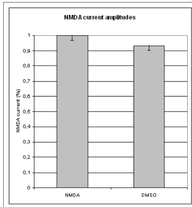
Figure 4.8 Change in NMDA current after DMSO application.
