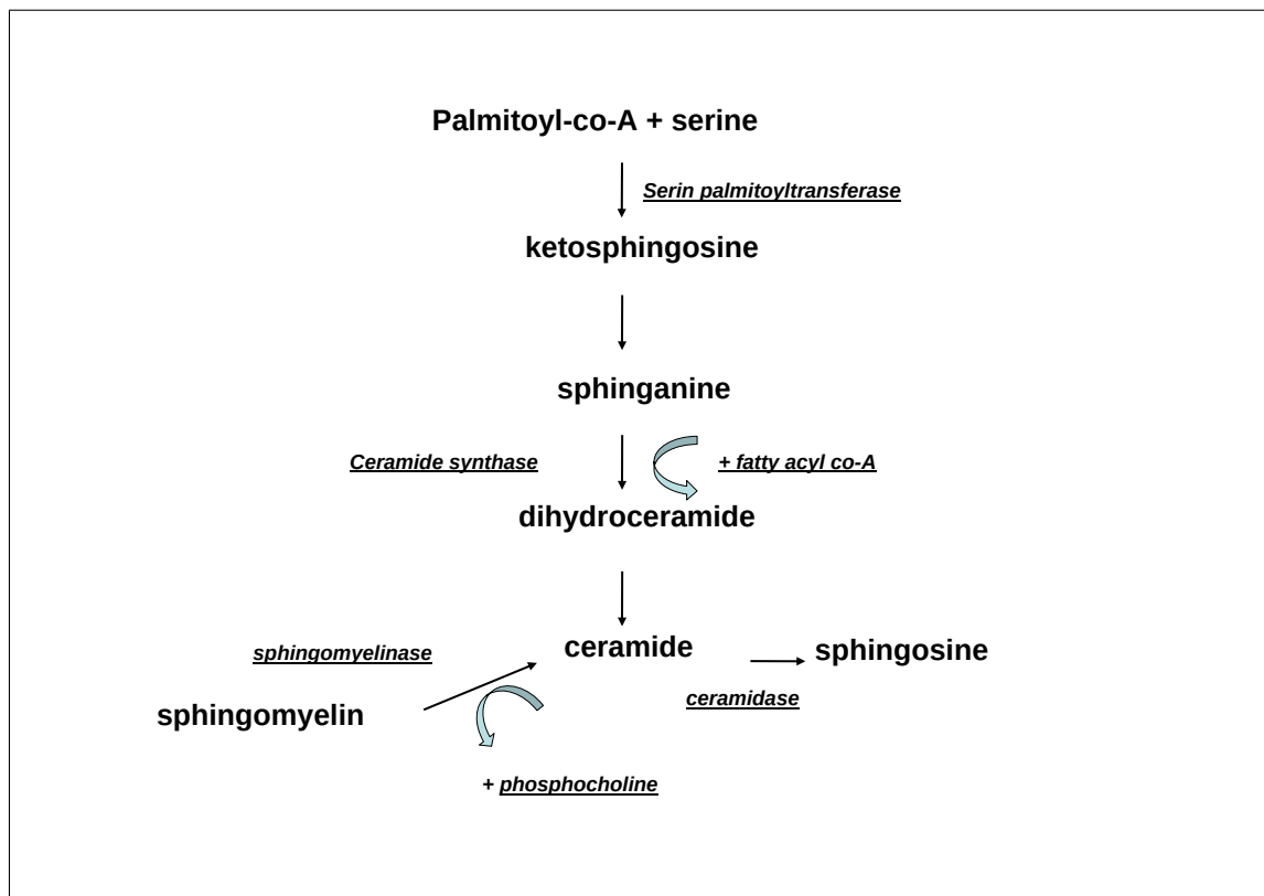
Figure 2.10 De novo synthesis of sphingolipids occurs at the cytosolic face of the endoplasmic reticulum, and starts by the condensation of serine and palmitoyl-CoA via serine palmitoyl-transferase. The resulting keto-sphinganine is reduced to form sphinganine, and N-acylated by ceramide synthase to dihydroceramide, which is then desaturated to yield ceramide (N-acylsphingosine). Ceramide can be transformed to sphingomyelin, the major sphingophospholipid, by addition of phosphocholine, or converted to glycolipids by addition of oligosaccharides. Catabolism of sphingolipids produces ceramide. Degradation of ceramide by ceramidase releases sphingoid bases, that can either be reutilized for complex sphingolipid biosynthesis or phosphorylated. Phosphorylation of sphingosine by sphingosine kinase yields sphingosine 1-phosphate, which is then dephosphorylated by a lipid phosphate phosphatase or cleaved by the sphingosine 1-phosphate lyase. Ceramide, sphingosine and S1P have all been demonstrated to be second messengers, conserved from yeast to man [28].
