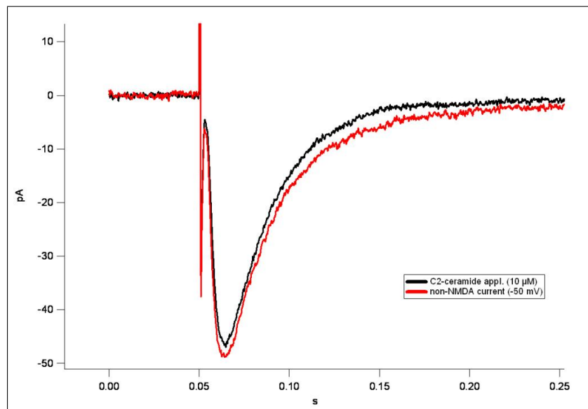
Figure 4.6 Effect of C2-ceramide ( 10 \mu\text{M} ) on non-NMDA current.
