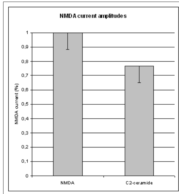
Figure 4.7 Change in NMDA current after C2-ceramide application.
