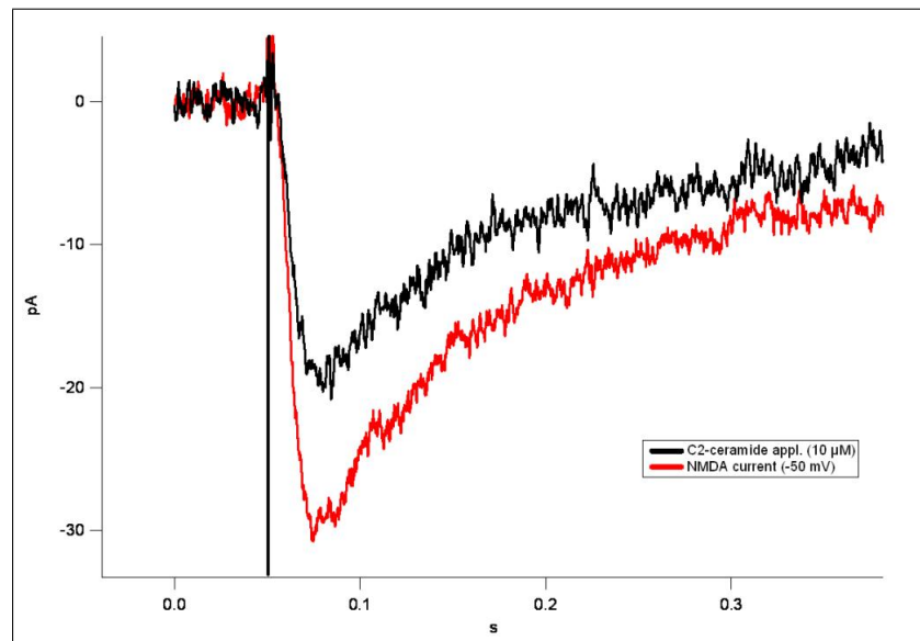
Figure 4.3 Modulatory effect of C2-ceramide (10 \mu M) on NMDA current.
