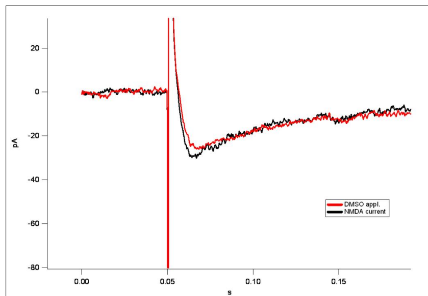
Figure 4.4 Control of the effect of DMSO on NMDA current
