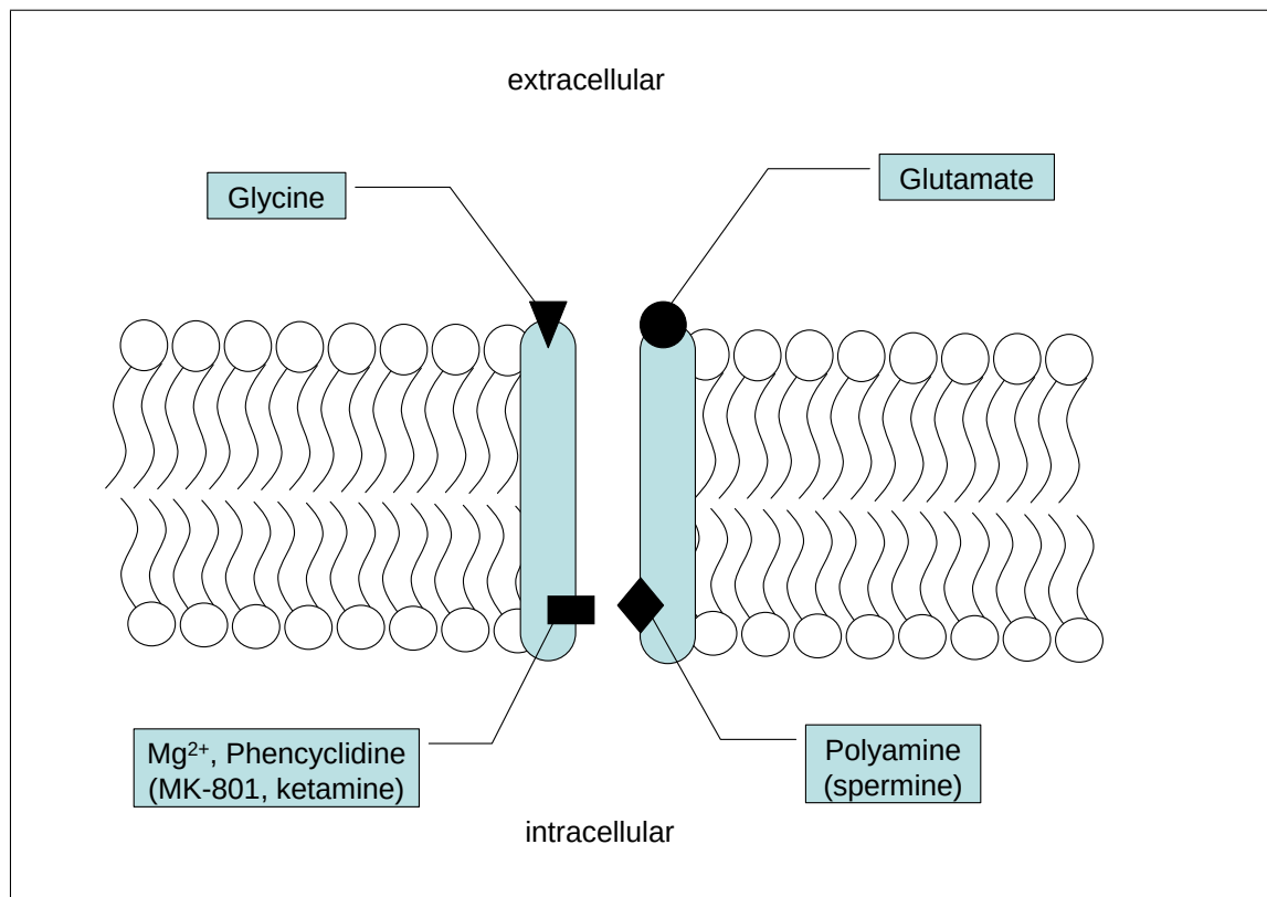
Figure 2.7 There are distinct binding sites for the modulation of NMDA receptor. The channel associated with the receptor is blocked by Mg^{2+} at resting potential ( -70 mV). Removal of Mg^{2+} block is necessary for receptor activation as well as the binding of glutamate and the co-agonist, glycine (ligand-gated). The different binding sites (glutamate, phencyclidine, polyamine, glycine) are shown, and together with antagonists at various sites. The polyamine site is an intracellular site which modulates the affinity of other agonists and antagonists.
