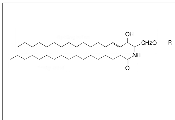
Figure 2.9 The sphingosine backbone is O-linked to a (usually) charged head group such as ethanolamine, serine or choline. The backbone is also amide-linked to an acyl group, such as a fatty acid.
