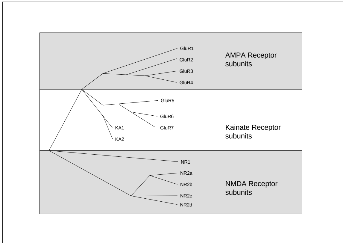
Figure 2.5 Subunits of ionotropic glutamate receptors. The ionotropic glutamate receptors are multimeric assemblies of four or five subunits, and are subdivided into three groups (AMPA, NMDA and Kainate receptors) [14].
