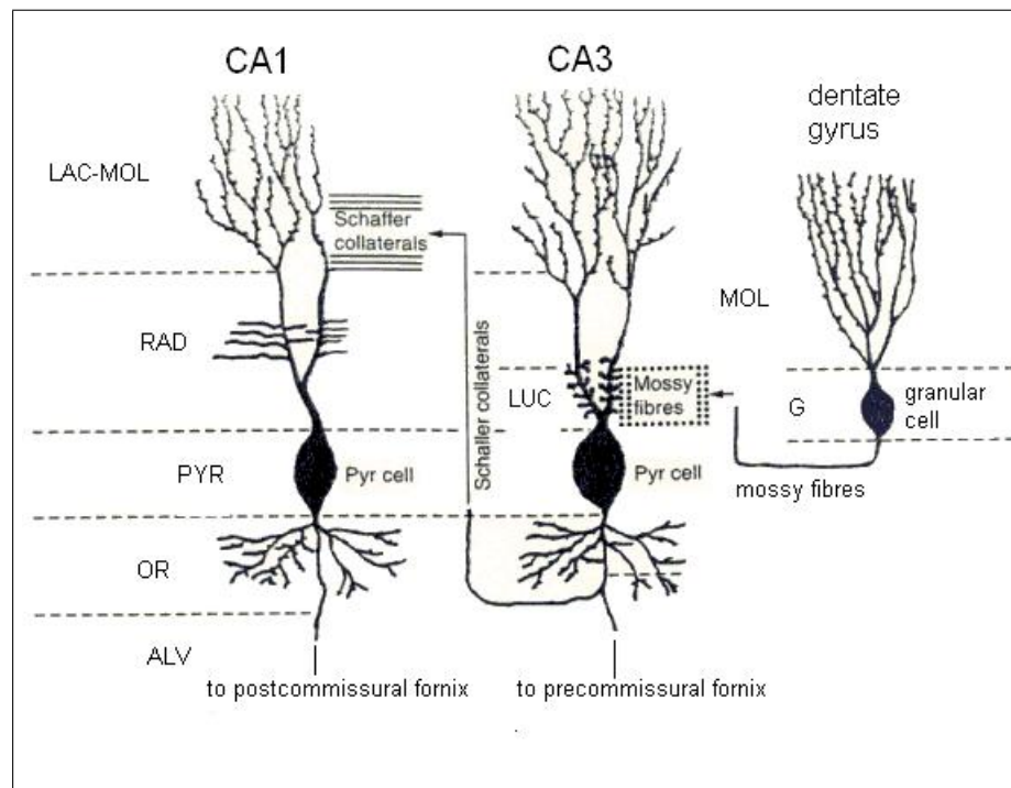
Figure 2.4 Trisynaptic circuit is composed pyramidal neurons placed in three different location: CA1, CA3 and dentate gyrus. Hippocampus is divided mainly into 4 main layers: stratum oriens (SO), stratum pyramidale (SP), stratum radiatum (SR) and stratum lacunosum-moleculare (SL). Axons of granular cells form mossy fibers. Axonal collaterals of CA3 pyramidal cells are called Schaffer collaterals (adapted from Hammond, 2001) [14].
