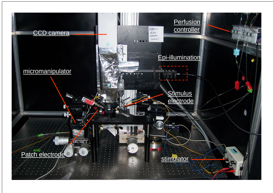
Figure 3.1 Setup for electrophysiological recording and fluorescence imaging.
