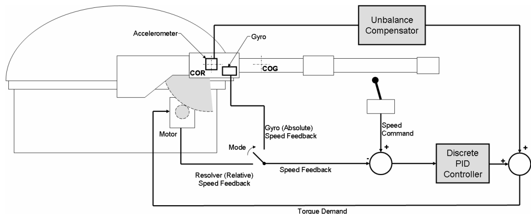
Figure 3.3 – Controller structure of a turret with discrete PID controller and unbalance compensation
