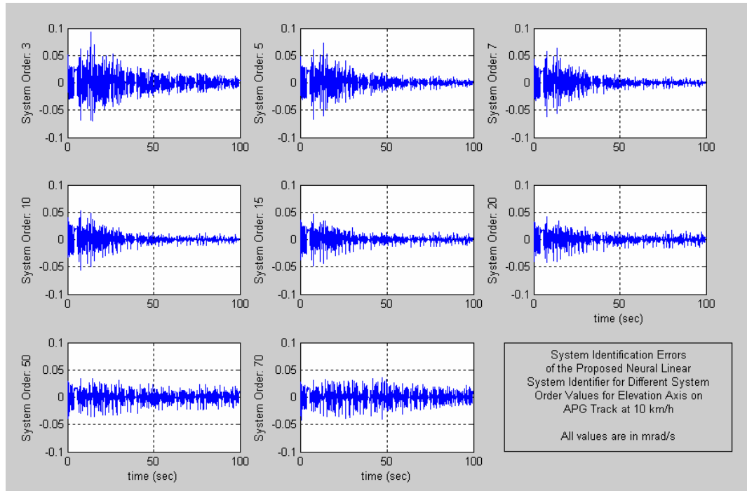
Figure 3.20 – System Identification Errors of the Proposed Neural Linear System Identifier for Different System Order Values for the Elevation Axis in APG Track at 10 km/h Speed
