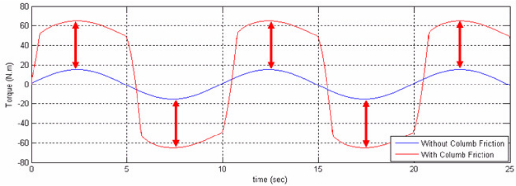
Figure 3.15 – Outputs of a PID Controller for Systems with and without Columb Friction
