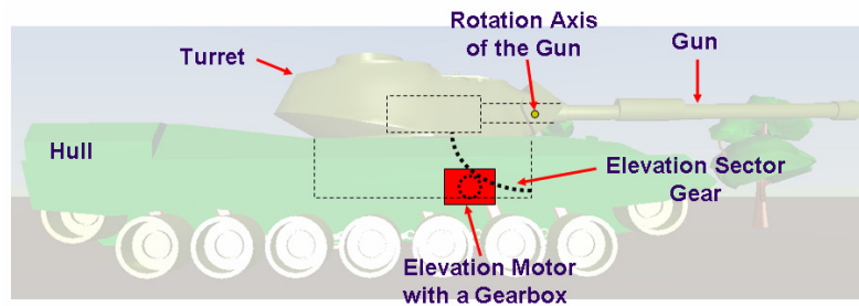
Figure 4.8 – Mechanical Structure of the Elevation Axis
