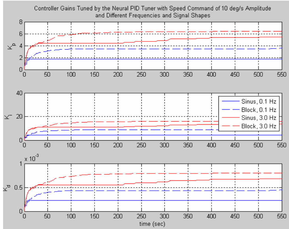
Figure 6.15 – Controller Parameters Tuned by the Neural PID Tuner with Speed Command of 10 deg/s Amplitude and Different Frequencies and Signal Shapes
