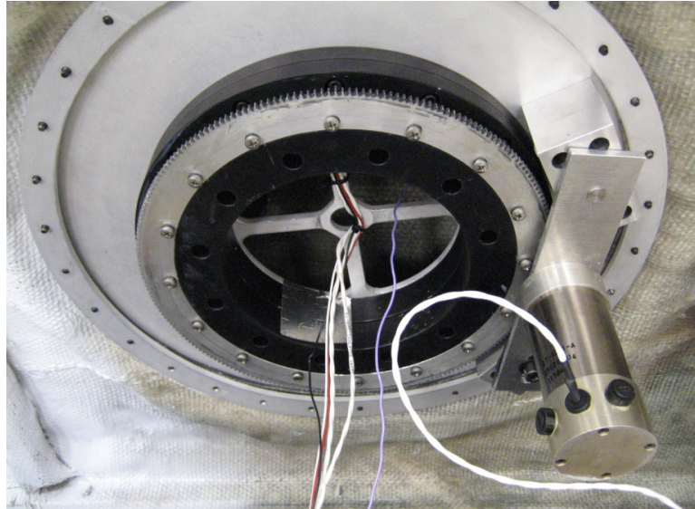
Figure 4.11 – Traverse Axis Actuation System of the Model Tank
