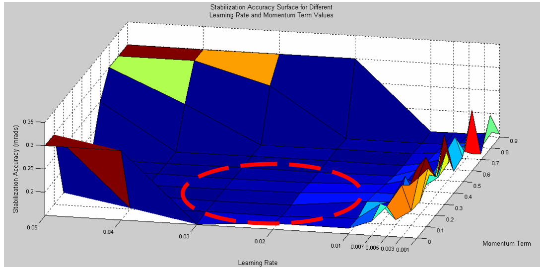
Figure 3.13 - Stabilization Accuracy Values Obtained for Different Learning Rate and Momentum Term Values, Trail 2 (0.3 mrad Shows Unstable Cases)
