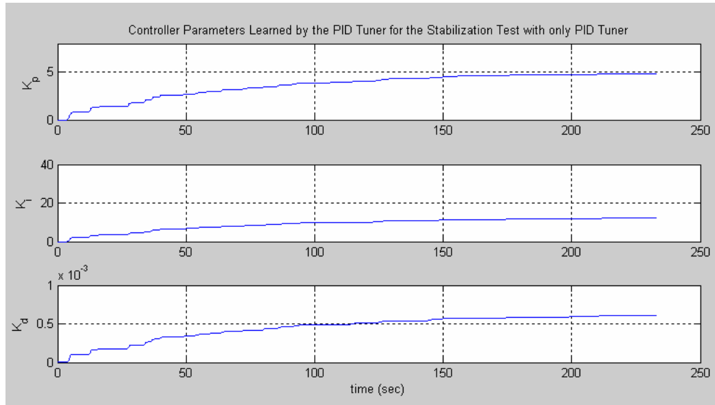
Figure 5.28 – Controller Gains Tuned by the Neural PID Tuner for the Stabilization Test with only the PID Tuner
