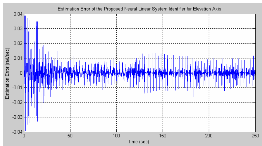
Figure 5.19 – Estimation Error of the Neural Linear System Identifier for the Elevation Axis on APG Track with 10 km/h for the Final Simulation
