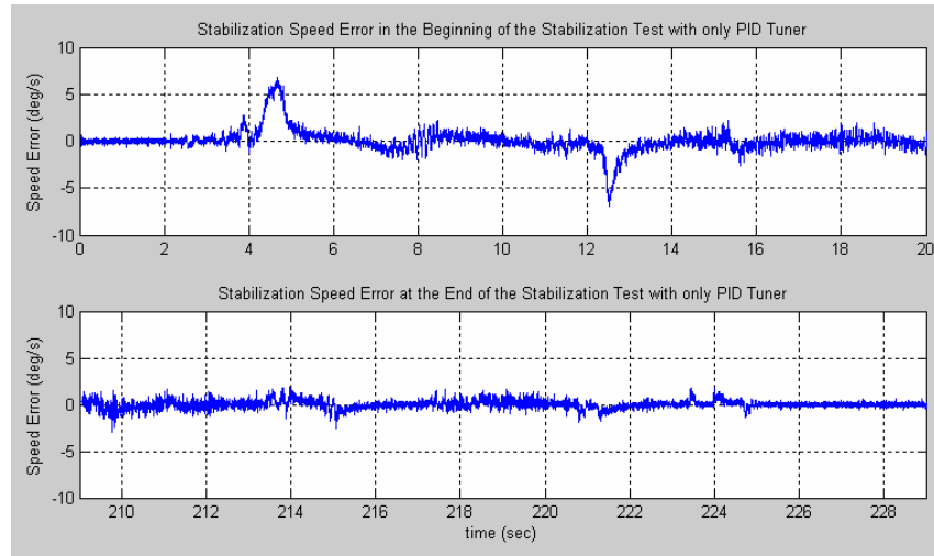
Figure 5.26 – Stabilization Speed Error for the Stabilization Test with only PID Tuner
