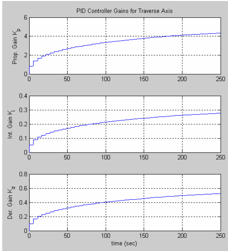
Figure 5.17 - Simulation Result for the Traverse Axis – PID Controller Parameters Learned Through the Simulation on Sinus Track with 10 km/h Speed
