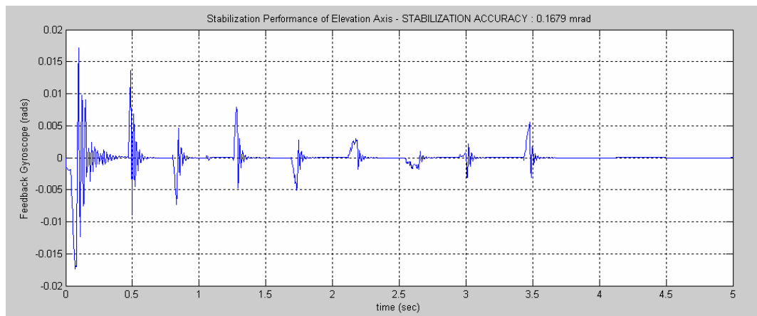
Figure 5.8 – Feedback Gyroscope Signal for Time Range 0 and 5 seconds
