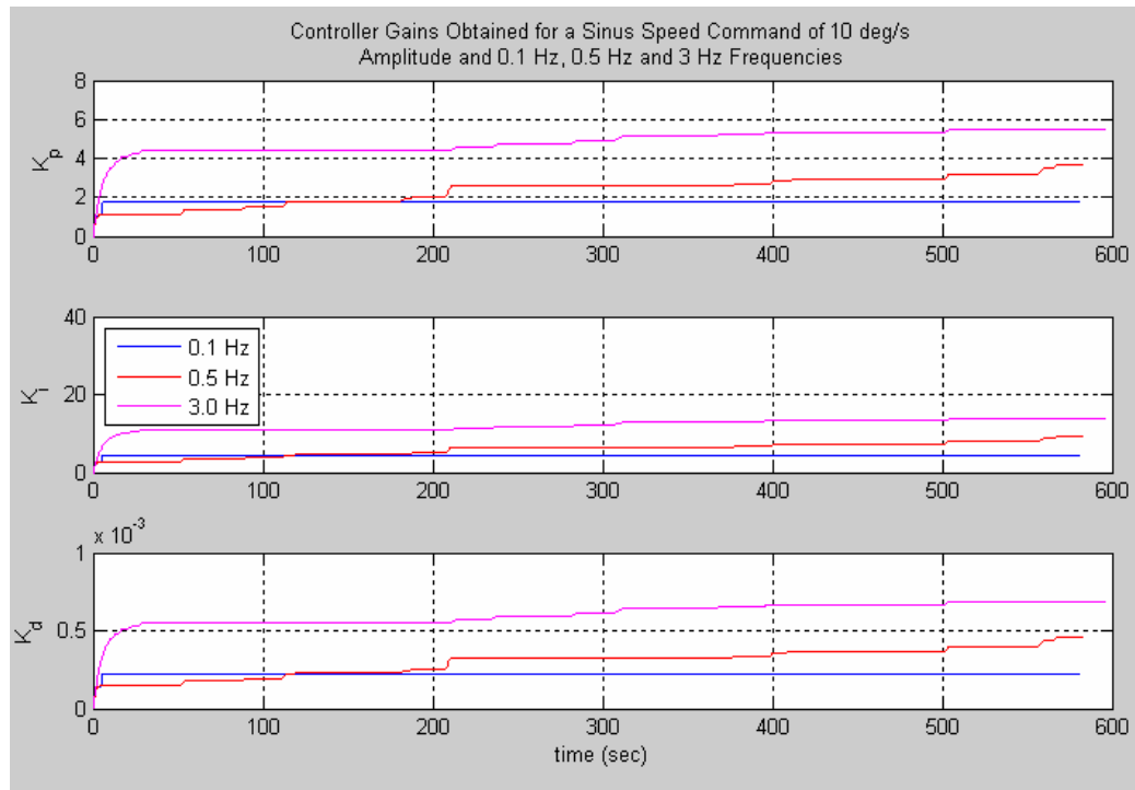
Figure 6.12 – Controller Gains Tuned by the Neural PID Tuner for a Sinus Speed Command of 10 deg/s Amplitude and Different Frequencies for the Traverse Axis of the Experimental Setup
