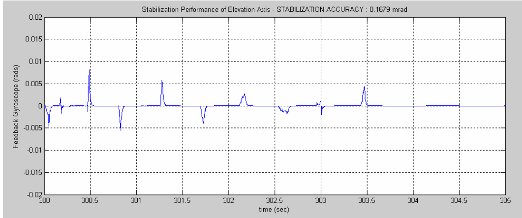
Figure 5.9 – Feedback Gyroscope Signal for Time Range 300 and 305 second
