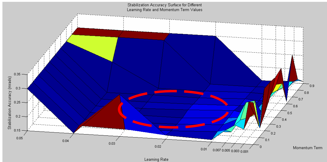
Figure 3.12 – Stabilization Accuracy Values Obtained for Different Learning Rate and Momentum Term Values, Trail 1 (0.3 mrad Shows Unstable Cases)
