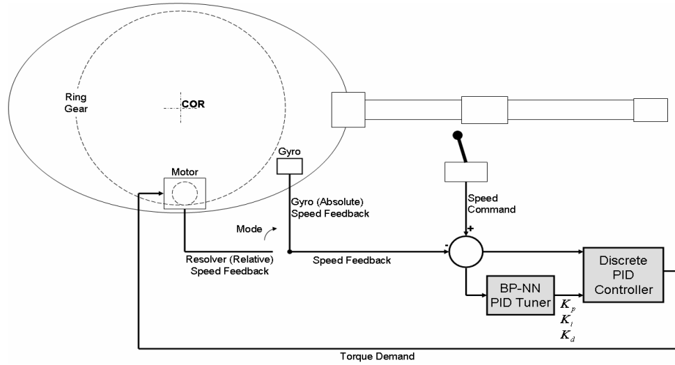
Figure 5.6 - Controller Architecture for Neural PID Tuner Simulations for Traverse Axis
