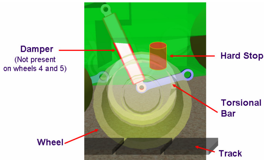
Figure 4.5 – Suspension System of Leopard 1 Tank
