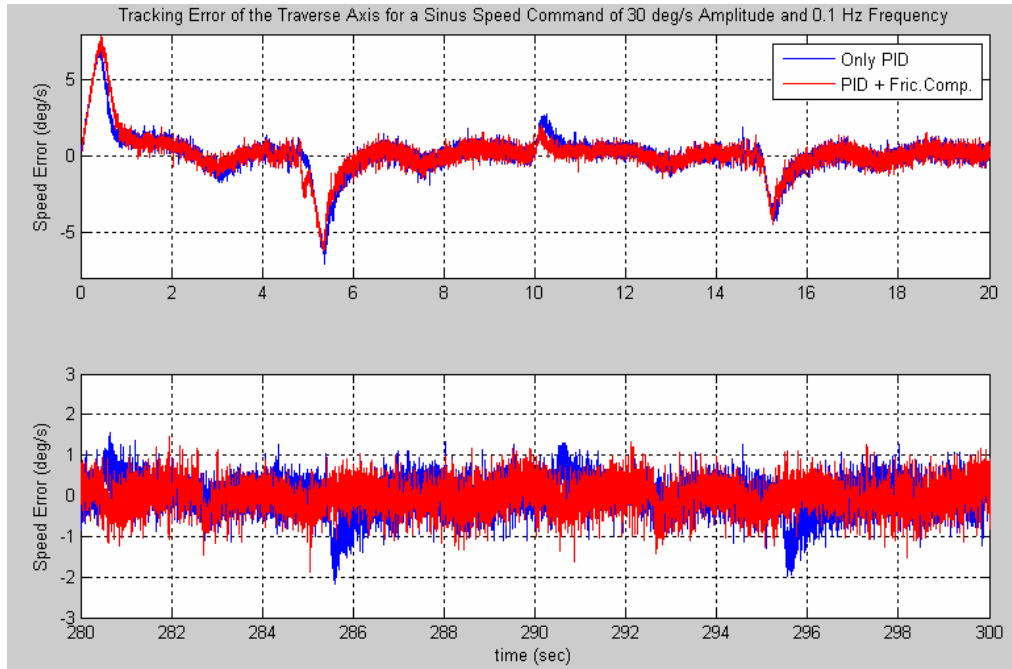
Figure 5.32 – Tracking Errors of the Traverse Axis of the Experimental Setup for Cases with PID Controller and PID Controller + Friction Compensator for a Sinus Speed Command of 30 deg/s Amplitude and 0.1 Hz Frequency
