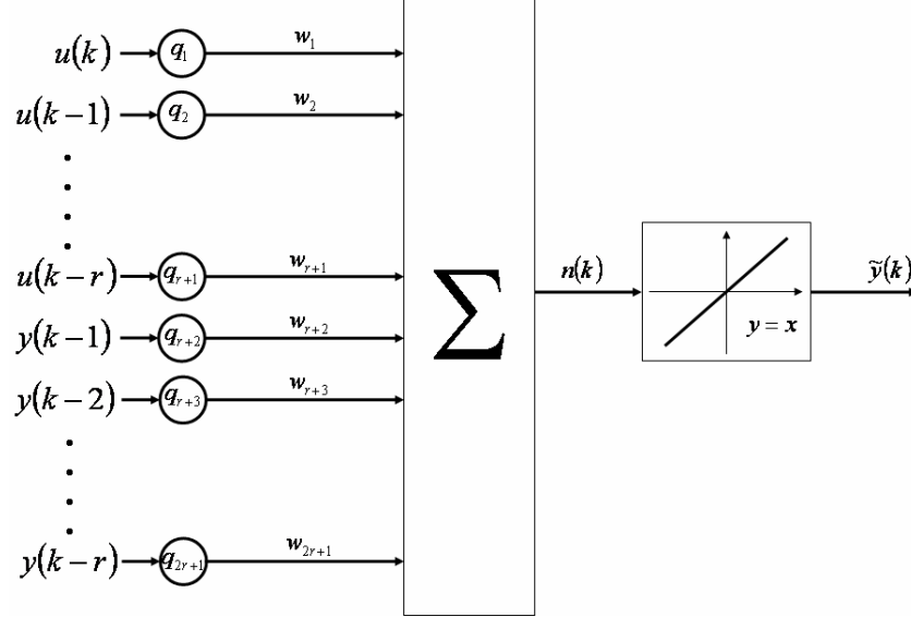
Figure 3.18 - Architecture of the neural linear system emulator
