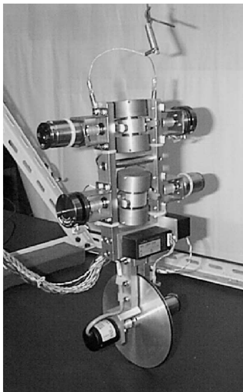
Figure 2.6 – Unicycle Robot in Motion
