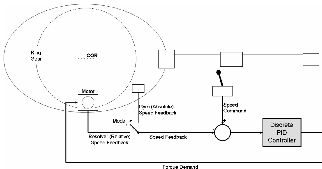
Figure 3.2 – Controller structure of a turret with discrete PID controller
