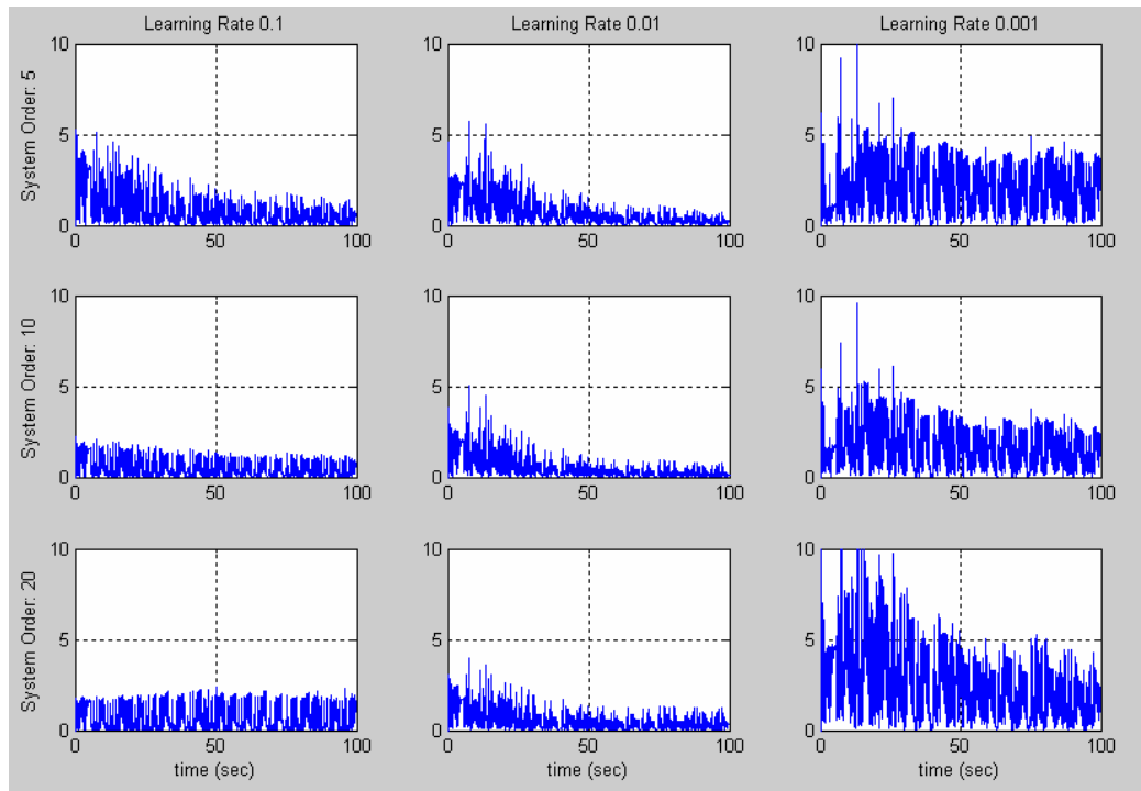
Figure 3.23 – Forgetting Sum of Identification Errors for Different System Orders and Different Learning Rates for the Elevation Axis on APG Track at 10 km/h
