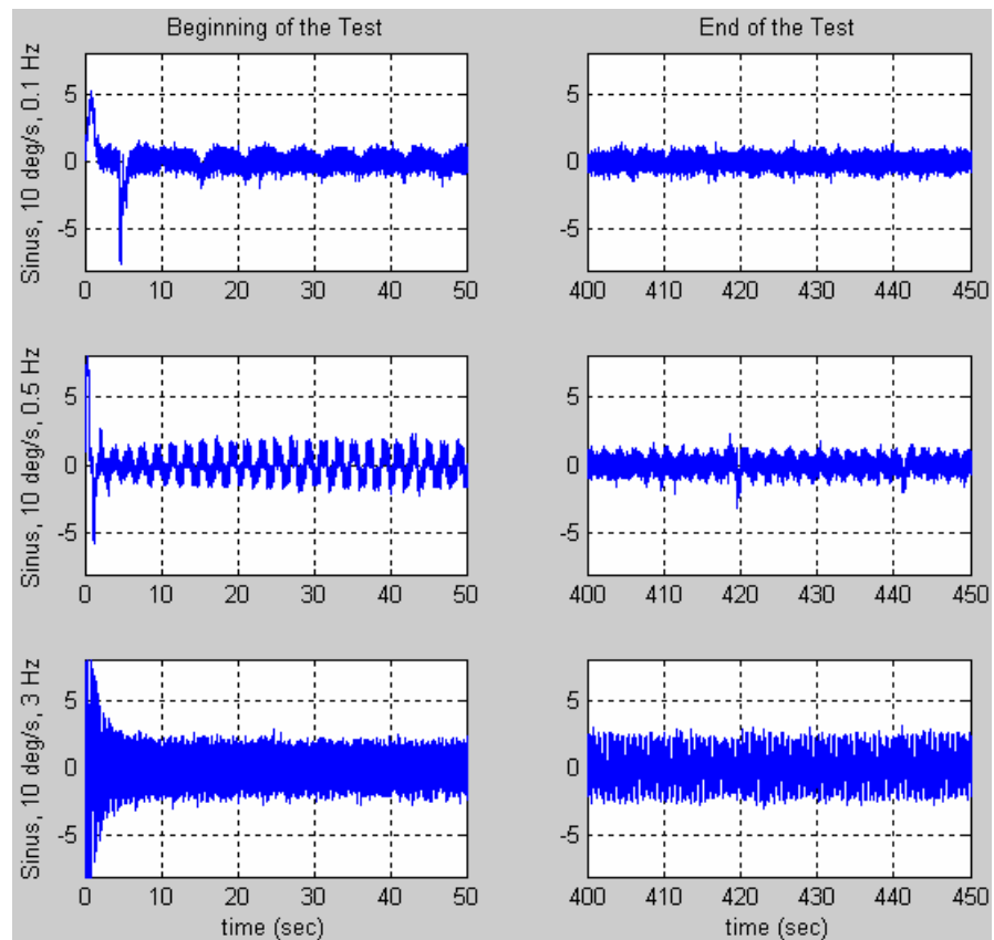
Figure 6.11 – Tracking Speed Errors of the Test for a Sinus Speed Command with 10 deg/s Amplitude for the Traverse Axis of the Experimental Setup
