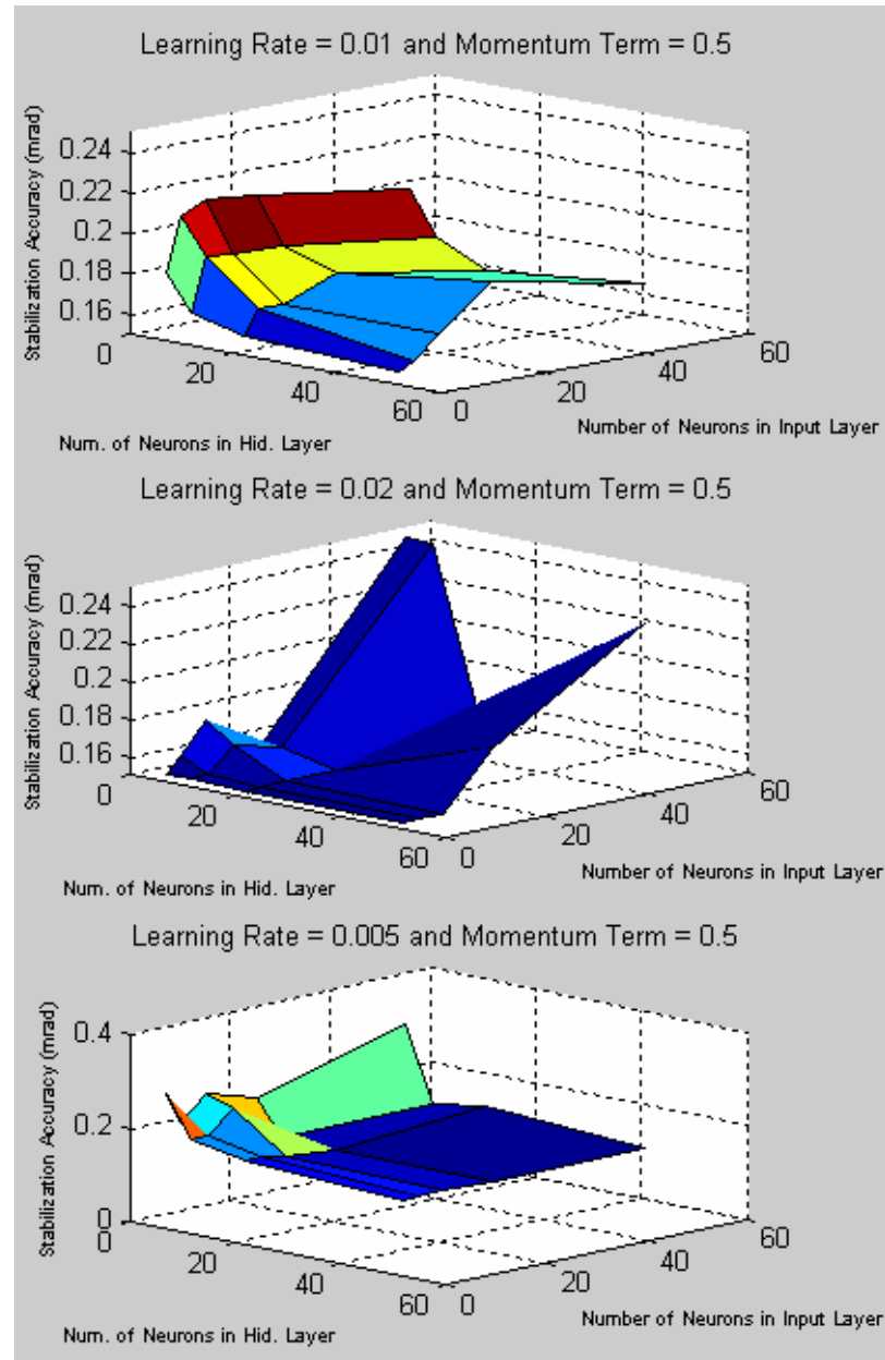
Figure 3.11 – Stabilization Accuracy Surfaces for Different Number of Neurons in the Input and Hidden Layers and for Different Learning Rate Values
