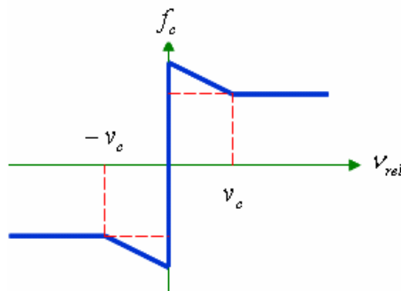
Figure 3.14 – Columb Friction Dependency on Relative Speed
