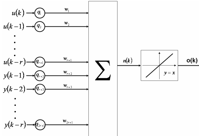
Figure 6.1 – Structure of the Proposed Neural Linear System Identifier
