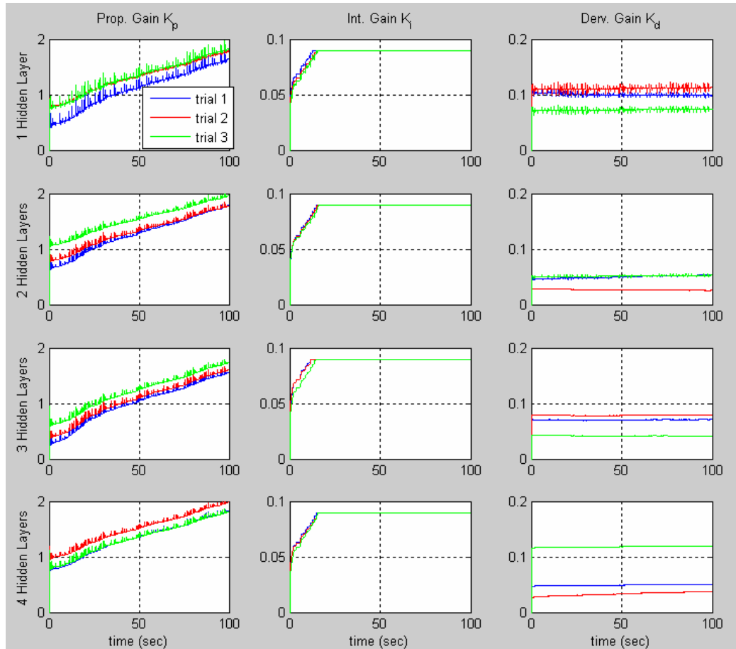
Figure 3.8 – Controller Gains Obtained for Different Number of Hidden Layers for the Tank Moving on APG Track with a Speed of 10 km/h
