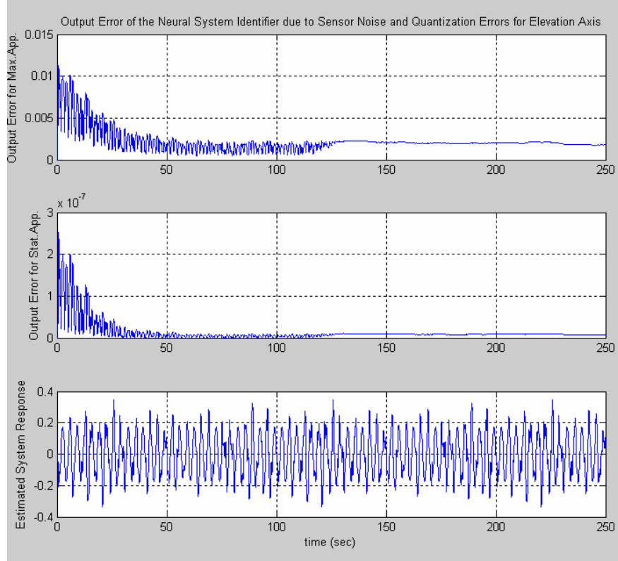
Figure 6.2 – Output Error of the Proposed Neural Linear System Identifier due to the Sensor Noise and Quantization Errors in the D/A Conversion for the Elevation Axis
