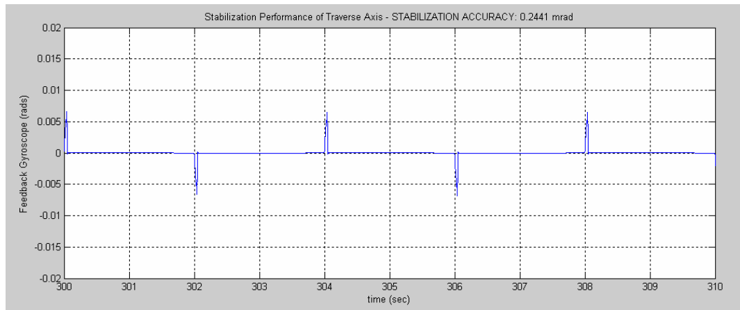
Figure 5.13 – Feedback Gyroscope Signal for Time Range 300 and 310 seconds
