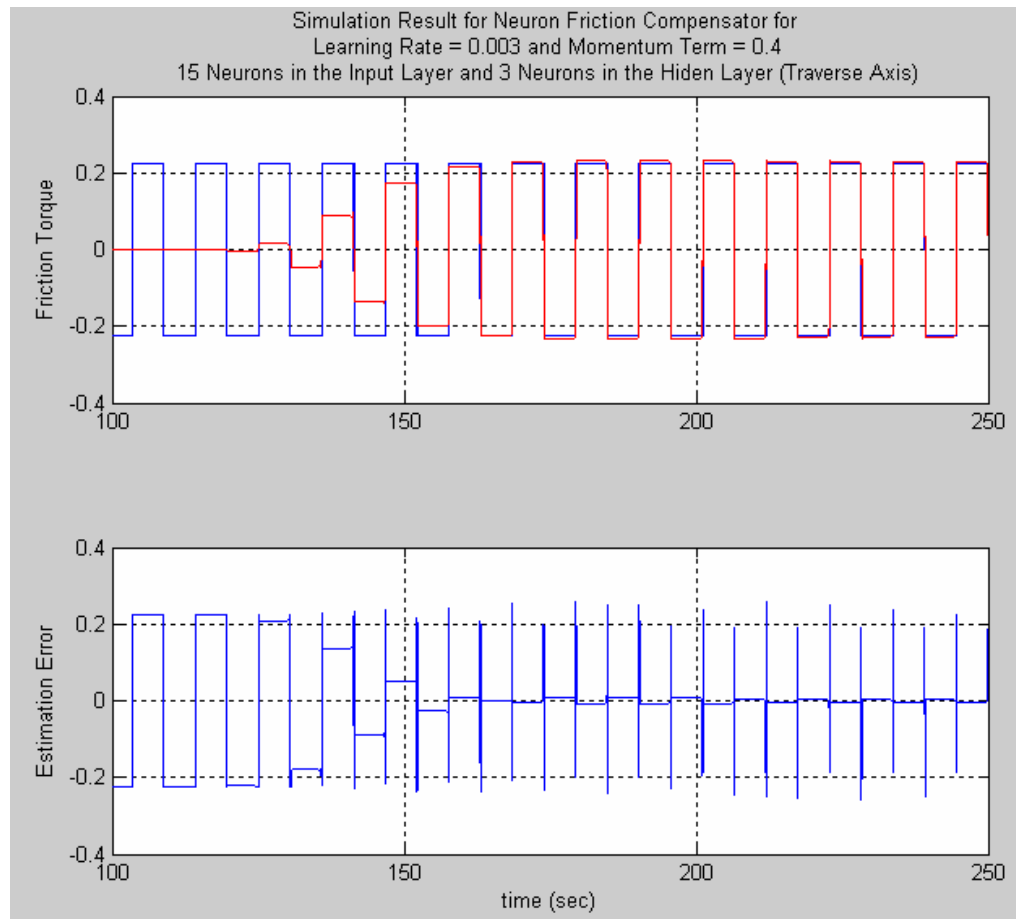
Figure 5.21 - Simulation Results for Neural Friction Compensator for Learning Rate \eta = 0.003 , momentum term \alpha = 0.4 , 15 Neurons in the Input Layer and 3 Neurons in the Hidden Layer for the Traverse Axis
