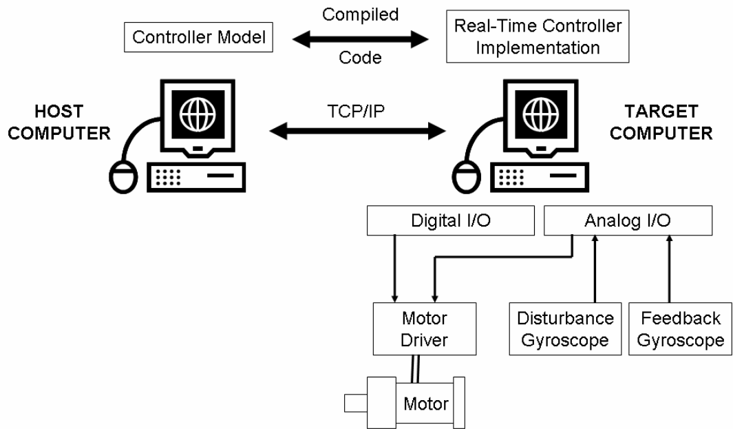
Figure 4.14 – xPC Target Implementation of the Proposed Neural Controller on the Model Main Battle Tank
