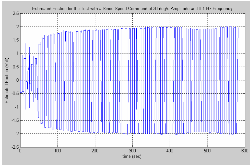
Figure 5.31 – Estimated Friction of the Traverse Axis of the Experimental Setup for a Sinus Speed Command of 30 deg/s Amplitude and 0.1 Hz Frequency
