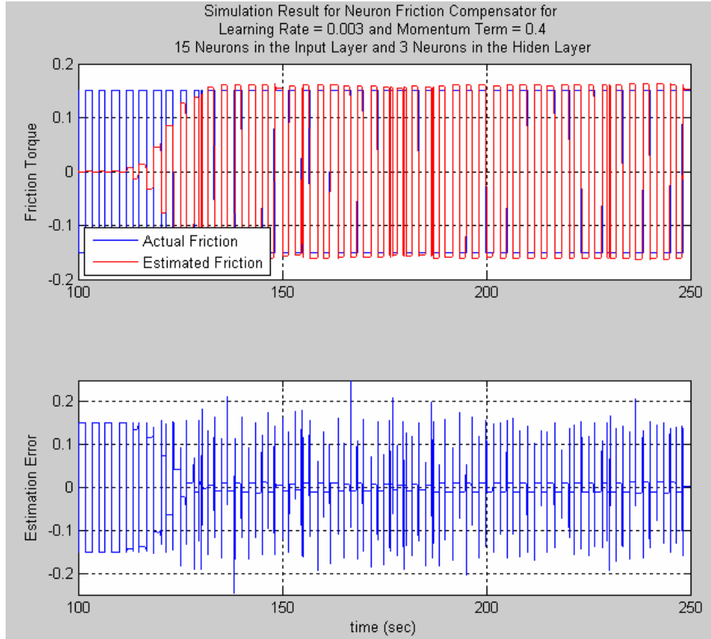
Figure 3.24 – Simulation Results for Neural Friction Compensator for Learning Rate \eta = 0.003 , momentum term \alpha = 0.4 , 15 Neurons in the Input Layer and 3 Neurons in the Hidden Layer for the Elevation Axis
