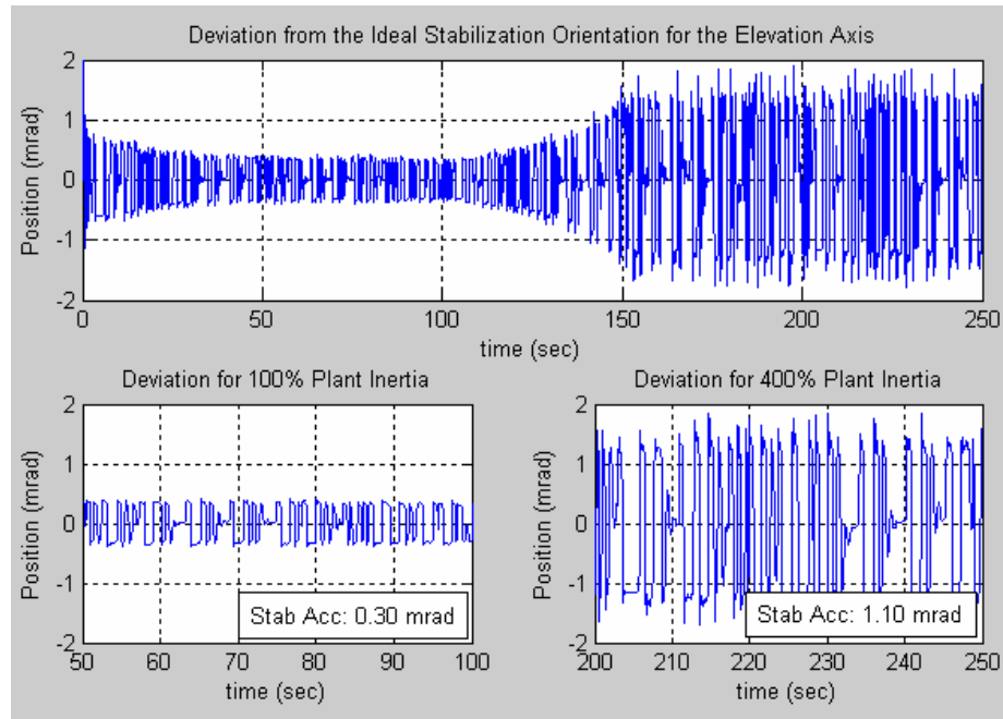
Figure 6.8 - Stabilization Performance of the Elevation Axis for Varying Elevation Axis Inertia on the APG Track (Fixed PID Parameters)
