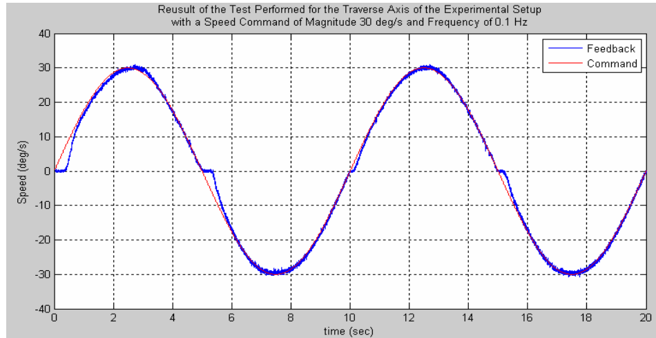
Figure 5.23 – Tracking Performance of the Traverse Axis for a Sinus Speed Command with 30 deg/s Amplitude and 0.1 Hz Frequency
