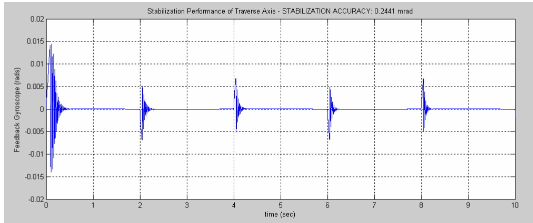
Figure 5.12 - Feedback Gyroscope Signal for Time Range 0 and 10 seconds
