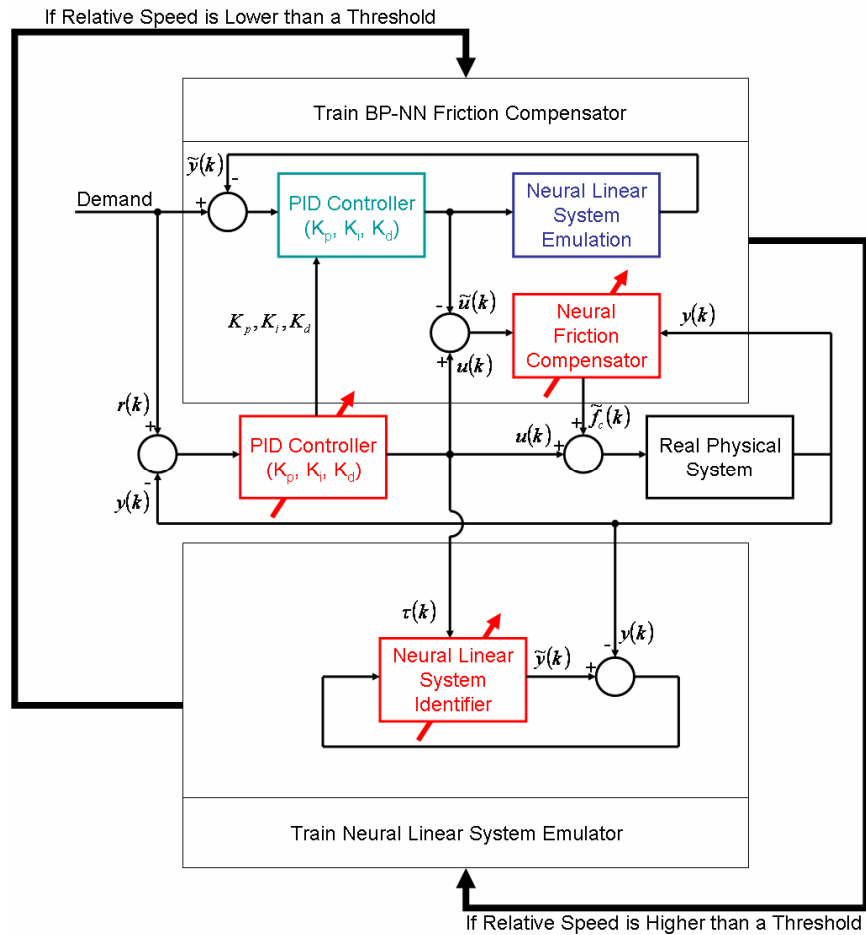
Figure 5.1 – Proposed Neuro Controller Architecture
