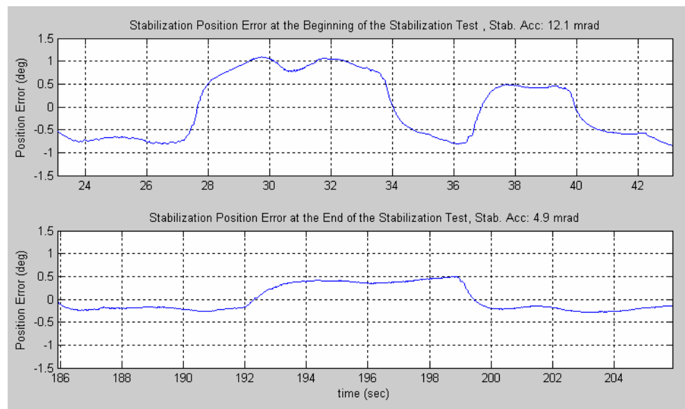
Figure 5.27 – Stabilization Position Error for the Stabilization Test with only PID Tuner
