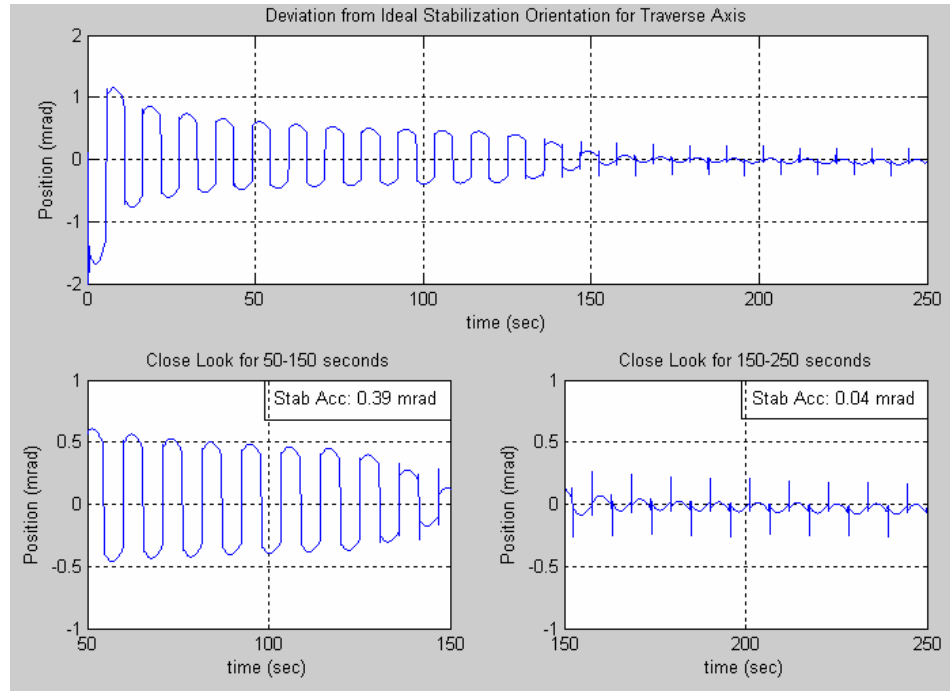
Figure 5.18 - Stabilization Performance of the Traverse Axis on Sinus Track with 10 km/h Speed for the Final Simulation
