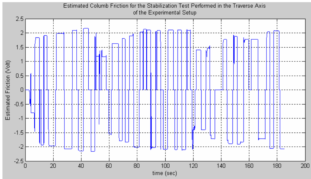
Figure 5.37 – Estimated Columb Friction in the Stabilization Test Performed for the Traverse Axis of the Experimental Setup
