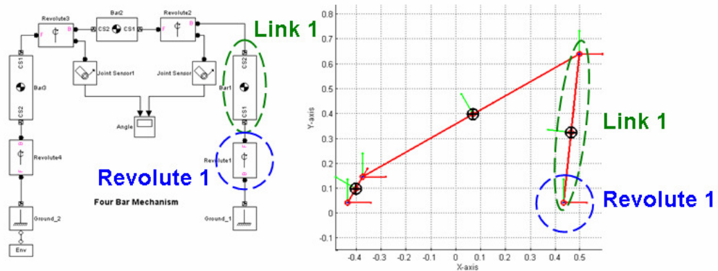
Figure 4.2 – Mathematical Modeling of a Four Bar Mechanism with SimMechanics
