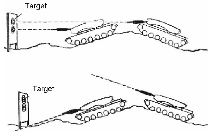
Figure 2.4 – Demonstration of gun stabilization on elevation axis
