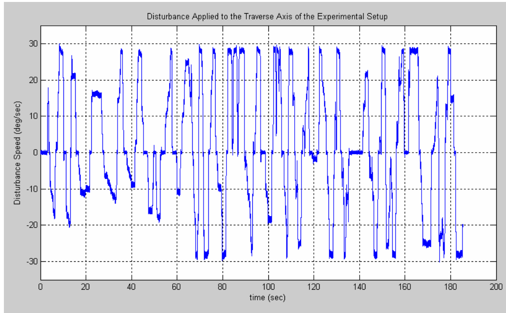
Figure 5.34 – Disturbance Speed Applied to the Traverse Axis of the Experimental Setup for the test of the Neural Friction Compensator
