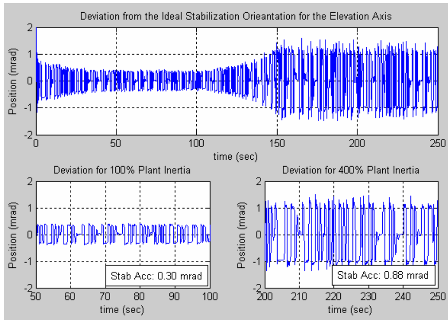
Figure 6.7 - Stabilization Performance of the Elevation Axis for Varying Elevation Axis Inertia on the APG Track
