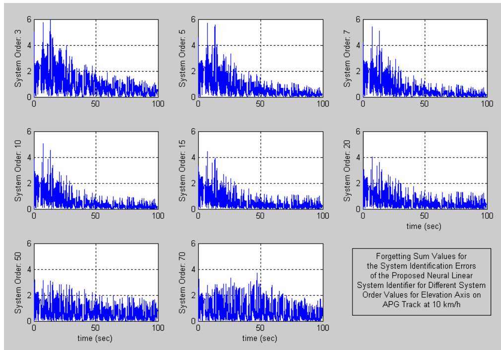
Figure 3.21 – Forgetting Sum Values for the System Identification Errors of the Proposed Neural System Identifier for Different System Order Values for the Elevation Axis on APG Track at 10 km/h Speed
