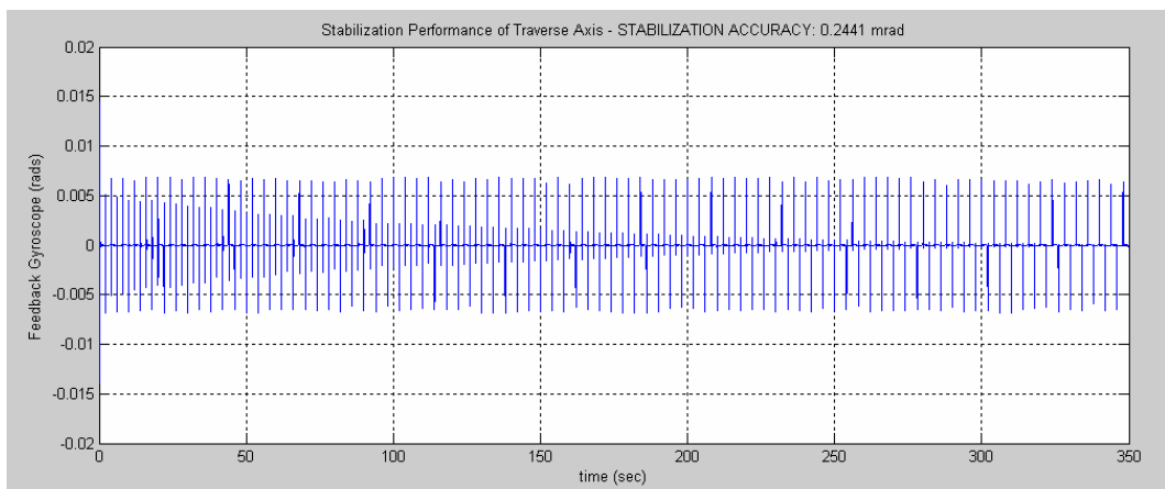
Figure 5.11 - Stabilization Performance of the PID Controller with Neural PID Tuner for the Traverse Axis
