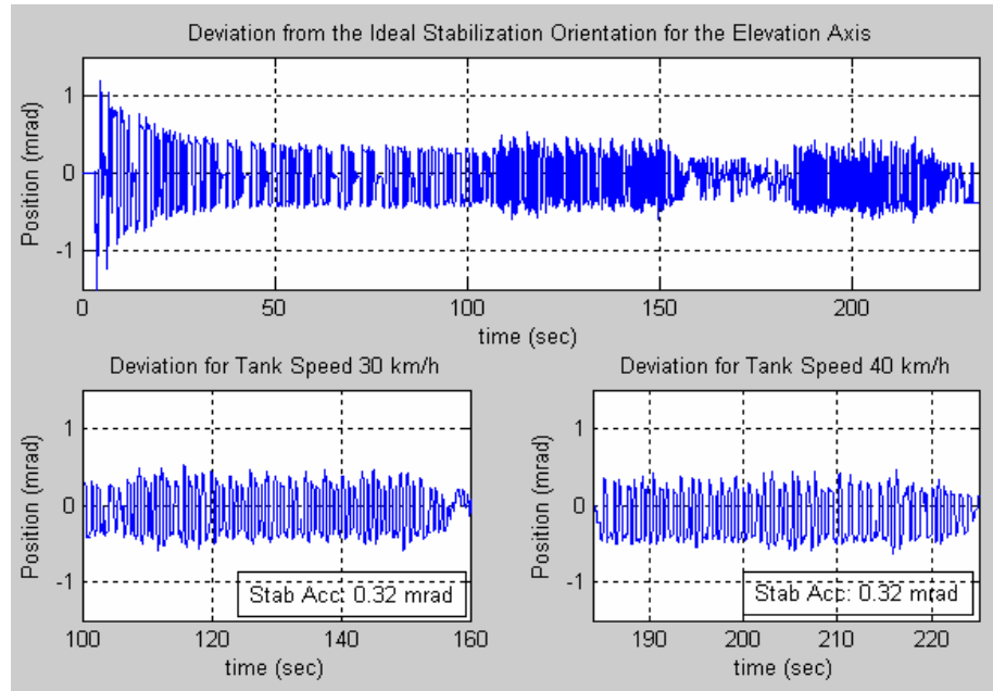
Figure 6.5 – Stabilization Performance of the Elevation Axis for Different Tank Speed on the APG Track
