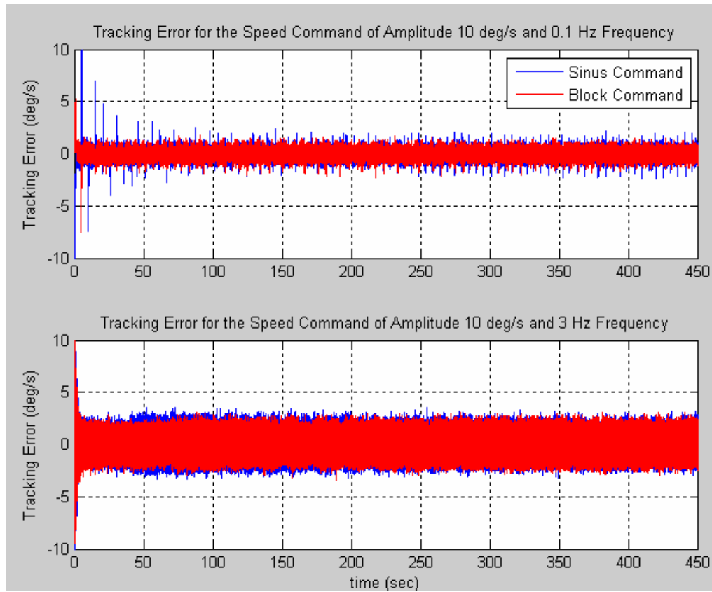
Figure 6.14 – Tracking Speed Errors for the Speed Command of 10 deg/s Amplitude and Different Frequencies for Different Signal Shapes for the Traverse Axis of the Experimental Setup
