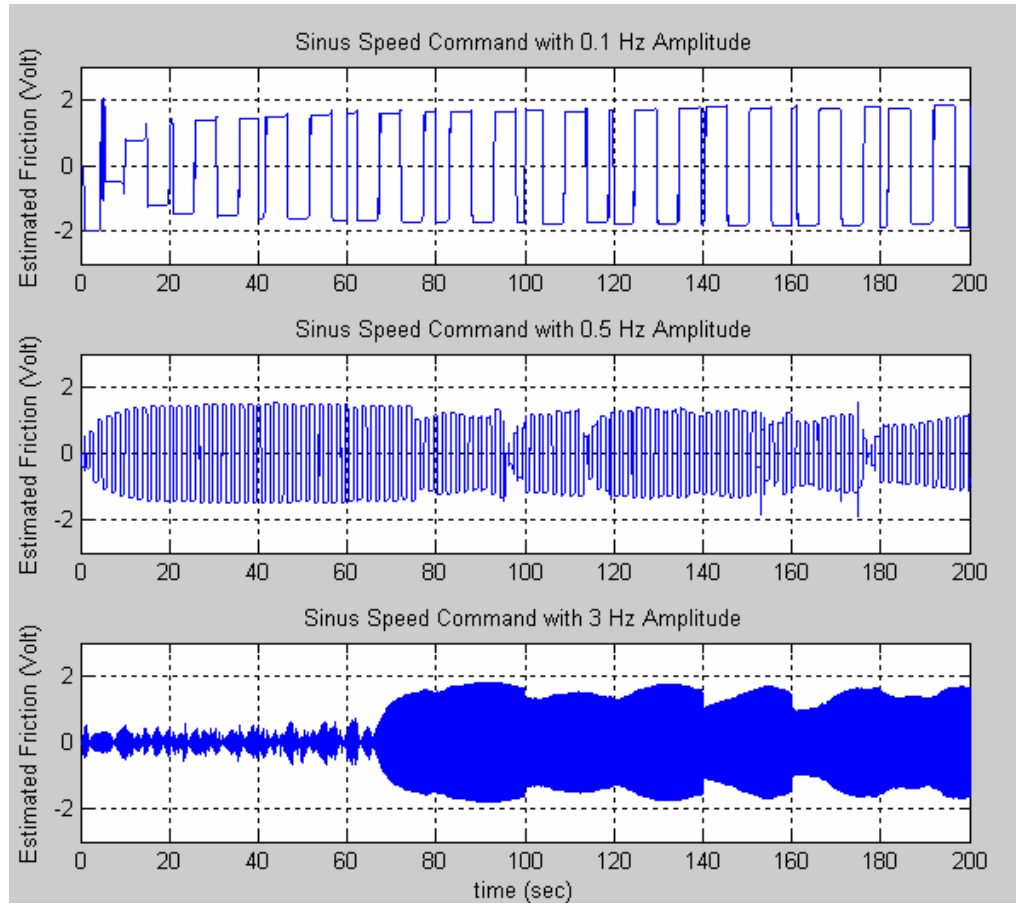
Figure 6.13 – Estimated Coulumb Friction for the Sinus Speed Command of 10 deg/s Amplitude and Different Frequencies for the Traverse Axis of the Experimental Setup
