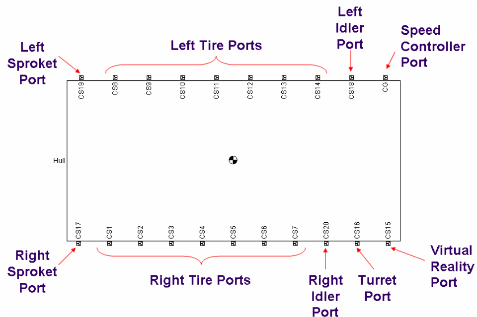
Figure 4.4 – Definition of The Joint Connections for the Hull of the Tank
