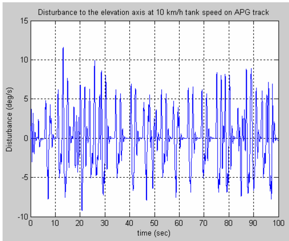
Figure 3.9 – Disturbance Speed for Elevation Axis on APG Track at 10 km/h
