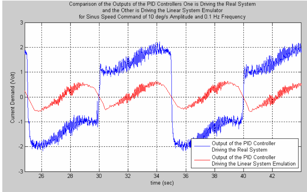
Figure 5.29 – Outputs of the PID Controllers One is Driving the Real System and the Other is Driving the Linear System Emulator for a Sinus Speed Command of 10 deg/s Amplitude and 0.1 Hz Frequency
