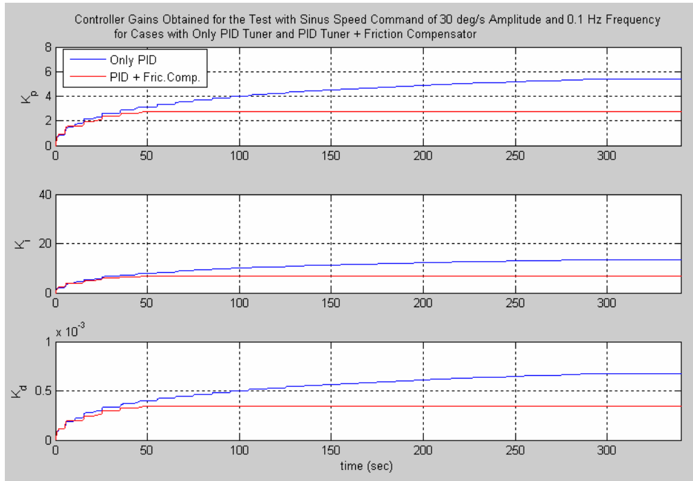
Figure 5.33 – Controller Gains Obtained for Cases with PID Tuner and PID Tuner + Friction Compensator
