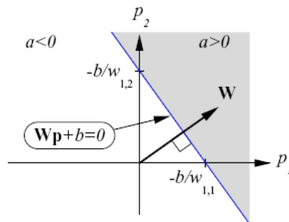
Figure 2.9 – Decision boundary representation for linear neural networks
