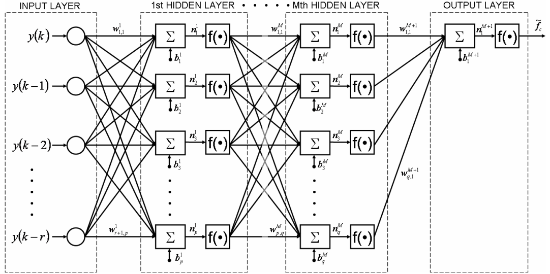
Figure 3.19 - Architecture of the neural friction identifier and compensator
