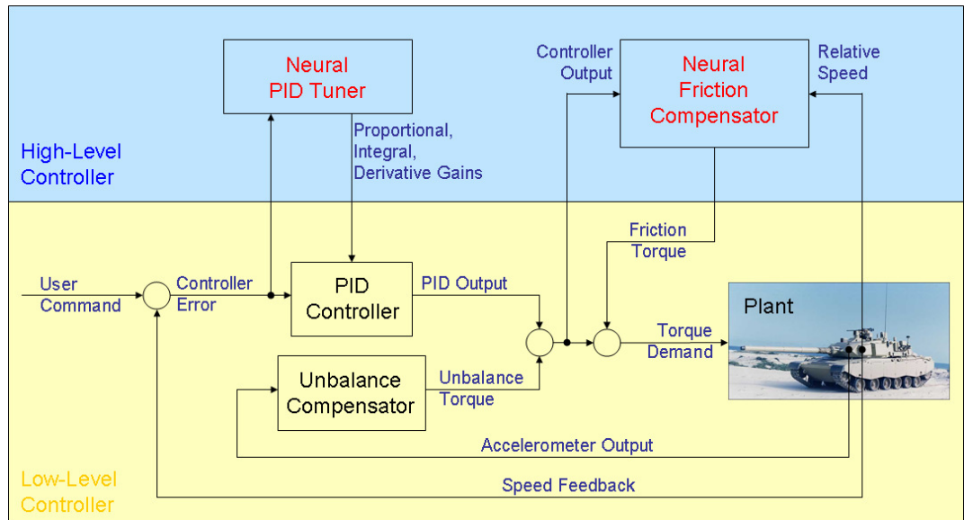
Figure 3.1 – Proposed Controller Architecture
