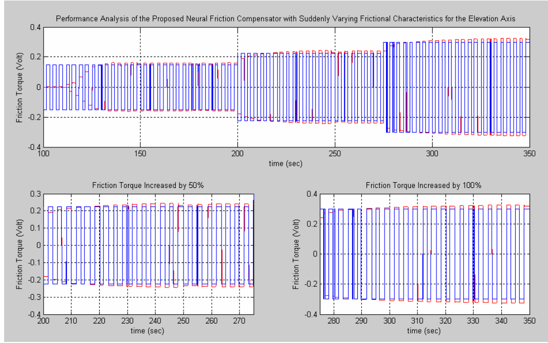
Figure 6.10 - Performance Analysis of the Proposed Neural Friction Compensator for Increasing Frictional Effects (Blue: Real Friction, Red: Estimated Friction)
