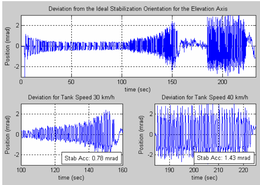
Figure 6.6 - Stabilization Performance of the Elevation Axis for Different Tank Speed on the APG Track (Fixed PID Parameters)
