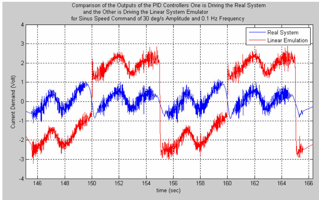
Figure 5.30 - Outputs of the PID Controllers One is Driving the Real System and the Other is Driving the Linear System Emulator for a Sinus Speed Command of 30 deg/s Amplitude and 0.1 Hz Frequency
