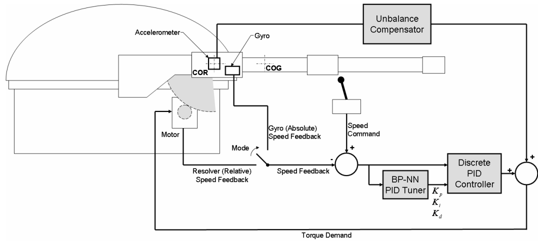
Figure 3.4 - Controller structure of a turret with unbalance compensation and PID controller tuned by a BP-NN PID tuner.
