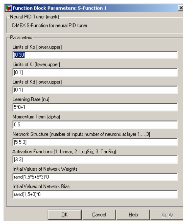
Figure 5.2 – Graphical User Interface for Neural PID Tuner
