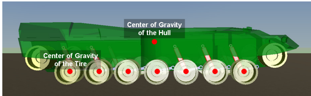
Figure 4.3 – Center of Gravity Representation of the Hull and the Wheels
