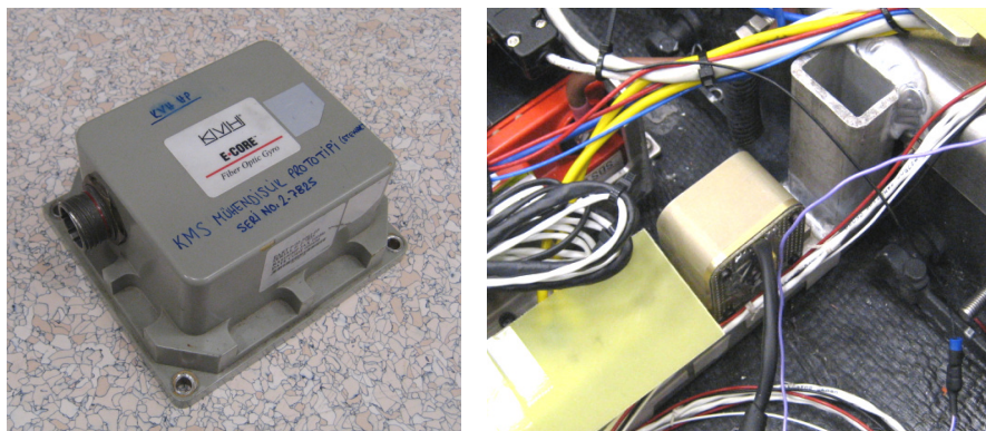
Figure 4.12 – Feedback Gyroscope (On the Left, Fiber optic) and Disturbance Gyroscope (On the Right, MEMS)
