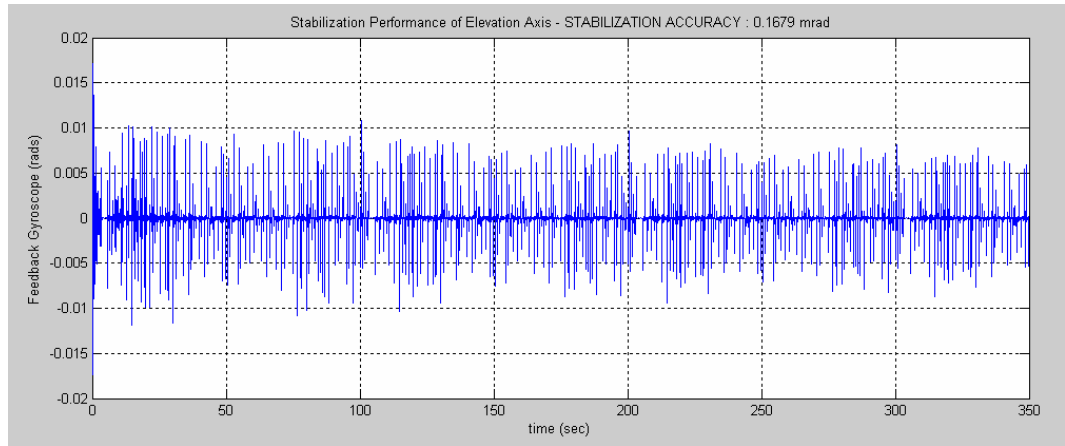
Figure 5.7 – Stabilization Performance of the PID Controller with Neural PID Tuner for the Elevation Axis
