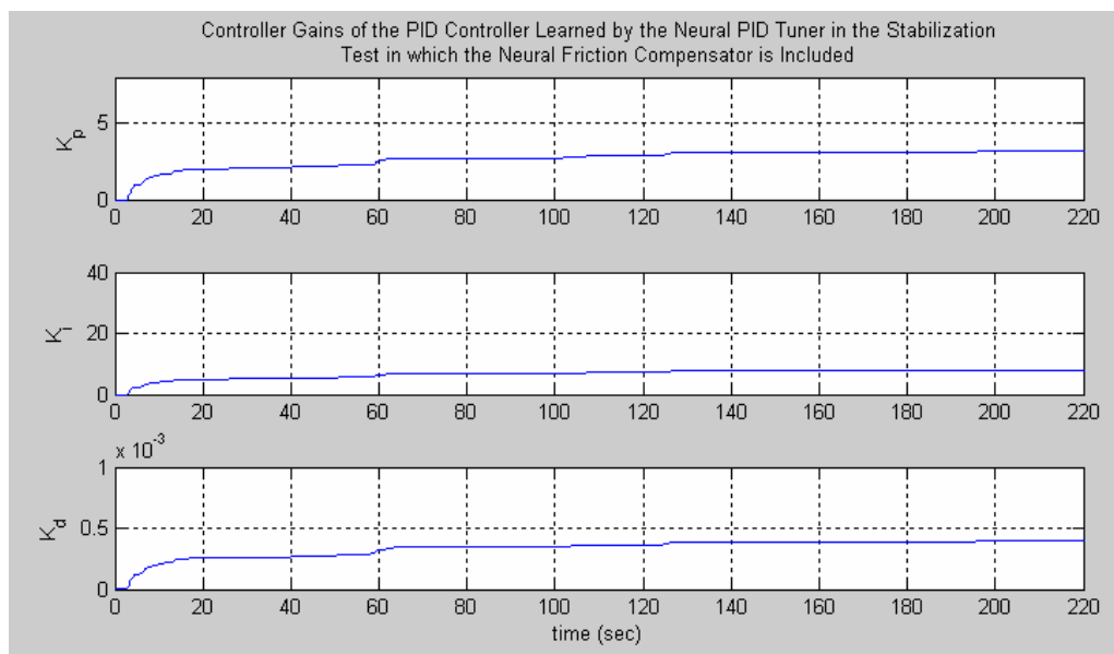
Figure 5.35 – Controller Gains of the PID Controller Tuned during the Stabilization Tests in which the Neural Friction Compensator is Included
