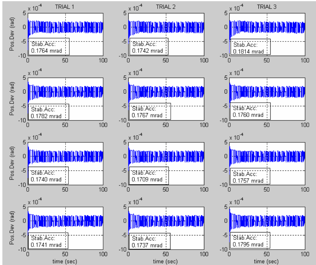
Figure 3.10 – Stabilization Accuracy of Elevation Axis on APG Track with Different Number of Hidden Layers
