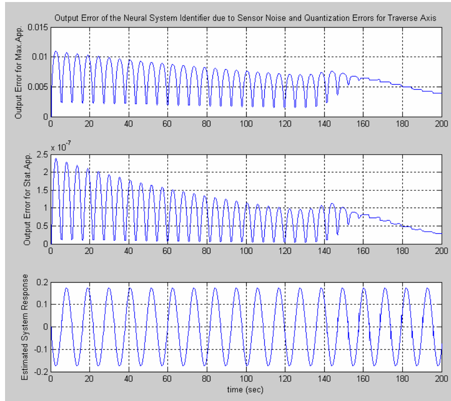
Figure 6.3 - Output Error of the Proposed Neural Linear System Identifier due to the Sensor Noise and Quantization Errors in the D/A Conversion for the Traverse Axis
