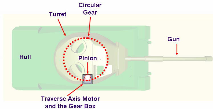
Figure 4.7 – Mechanical Structure of the Traverse Axis
