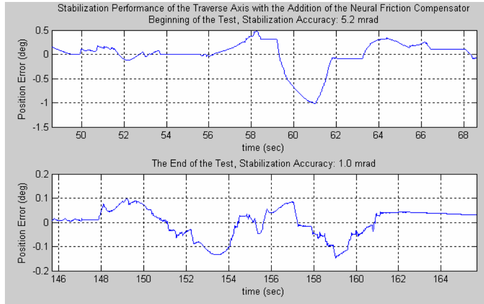
Figure 5.36 – Stabilization Performance of the Traverse Axis Including the Proposed Neural Friction Compensator
