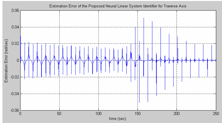
Figure 5.20 - Estimation Error of the Neural Linear System Identifier for the Traverse Axis on Sinus Track with 10 km/h for the Final Simulation
