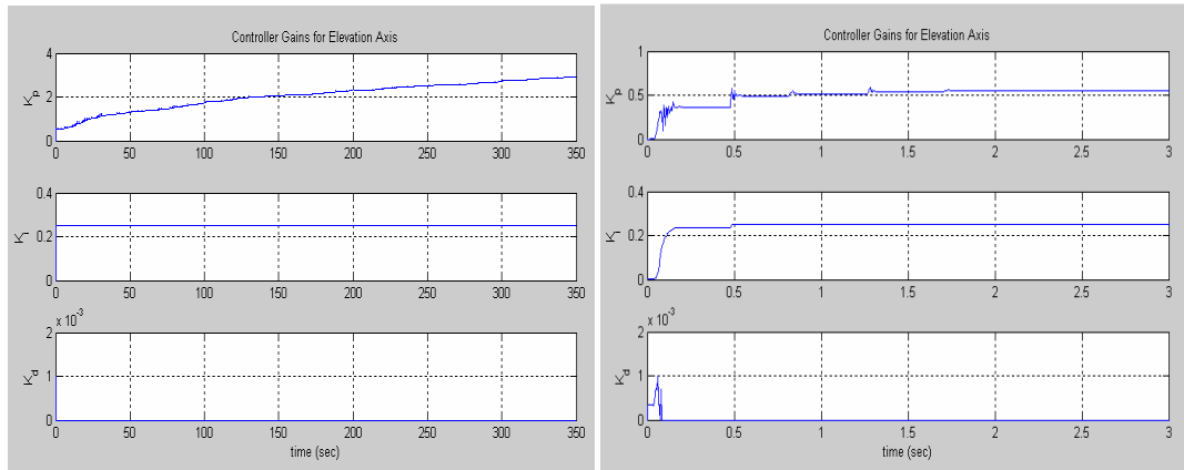
Figure 5.10 – Controller Gains for the Elevation Axis Simulations
