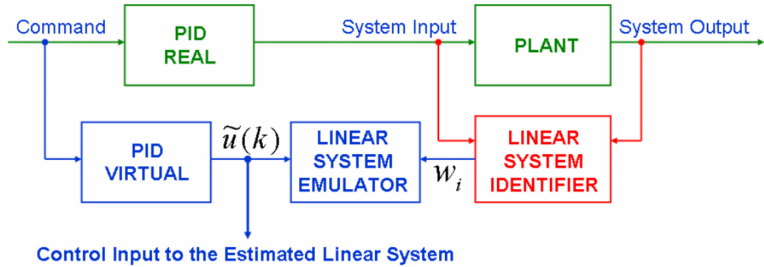
Figure 3.17 – Block Diagram for the Estimation of the Linear Dynamics of the System and Emulation of the Virtual Linear System
