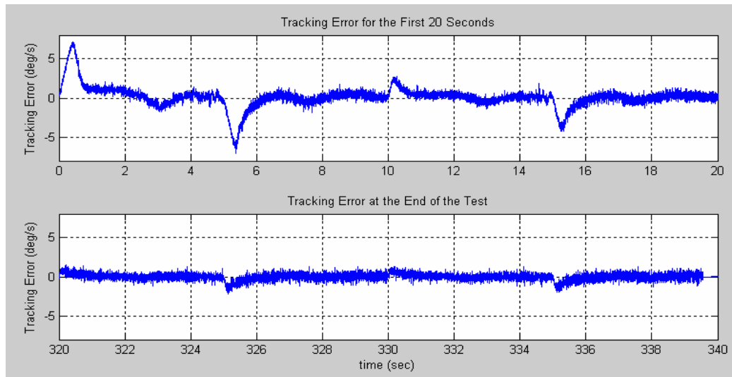
Figure 5.24 – Tracking Errors for the Test with Sinus Speed Command with 30 deg/s Amplitude and 0.1 Hz Frequency
