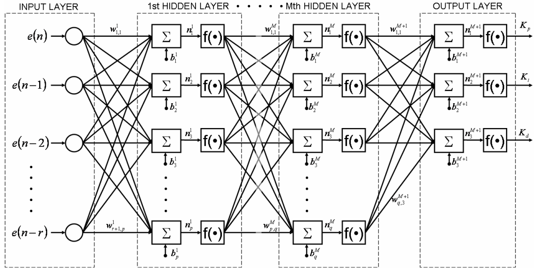
Figure 3.5 – Architecture of the neural PID tuner
