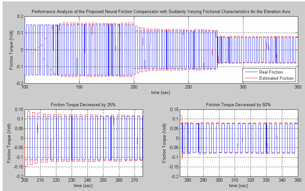
Figure 6.9 – Performance Analysis of the Proposed Neural Friction Compensator for Decreasing Frictional Effects
