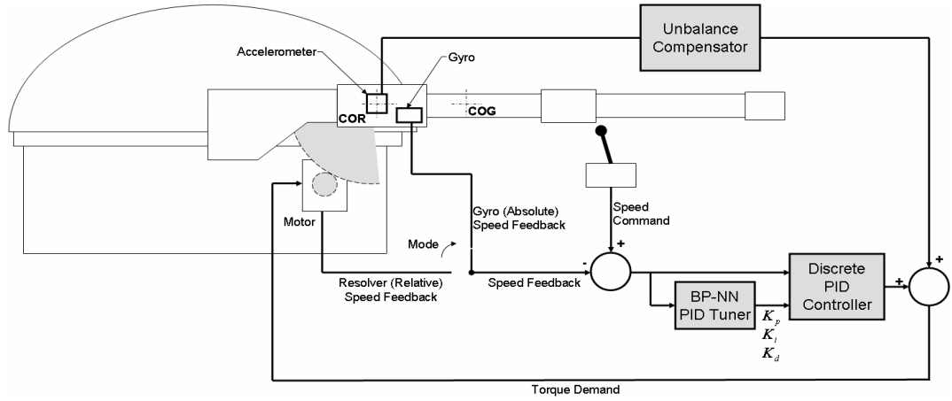
Figure 5.5 – Controller Architecture for Neural PID Tuner Simulations for Elevation Axis
