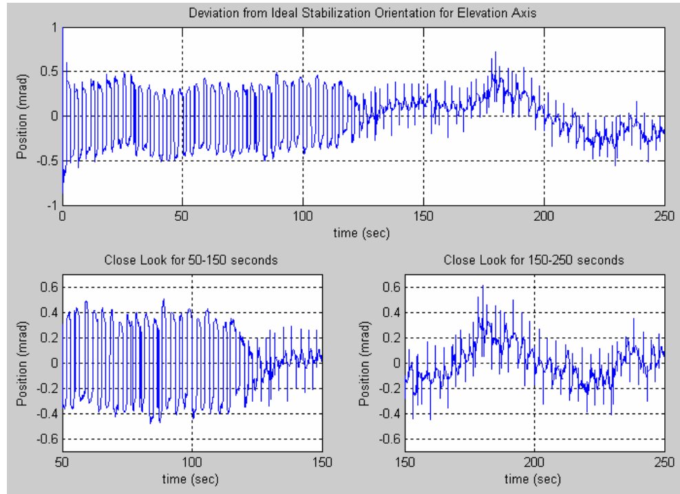
Figure 5.16 – Stabilization Performance of the Elevation Axis on APG Track with 10 km/h Speed for the Final Simulation
