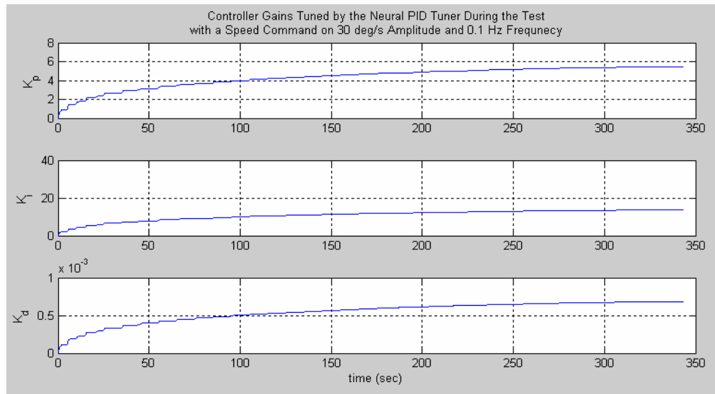
Figure 5.25 – Controller Gains Tuned by the Neural PID Tuner for the Test with Sinus Speed Command of 30 deg/s Amplitude and 0.1 Hz Frequency
