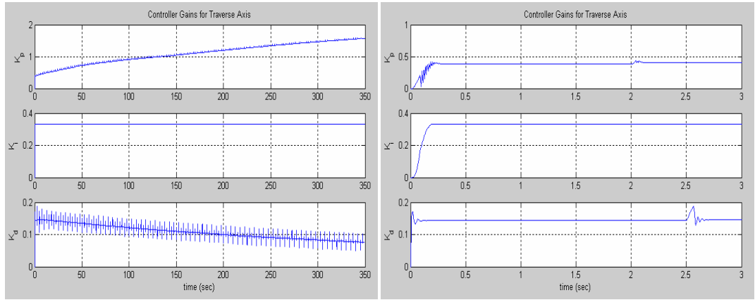
Figure 5.14 - Controller Gains for the Traverse Axis Simulations
