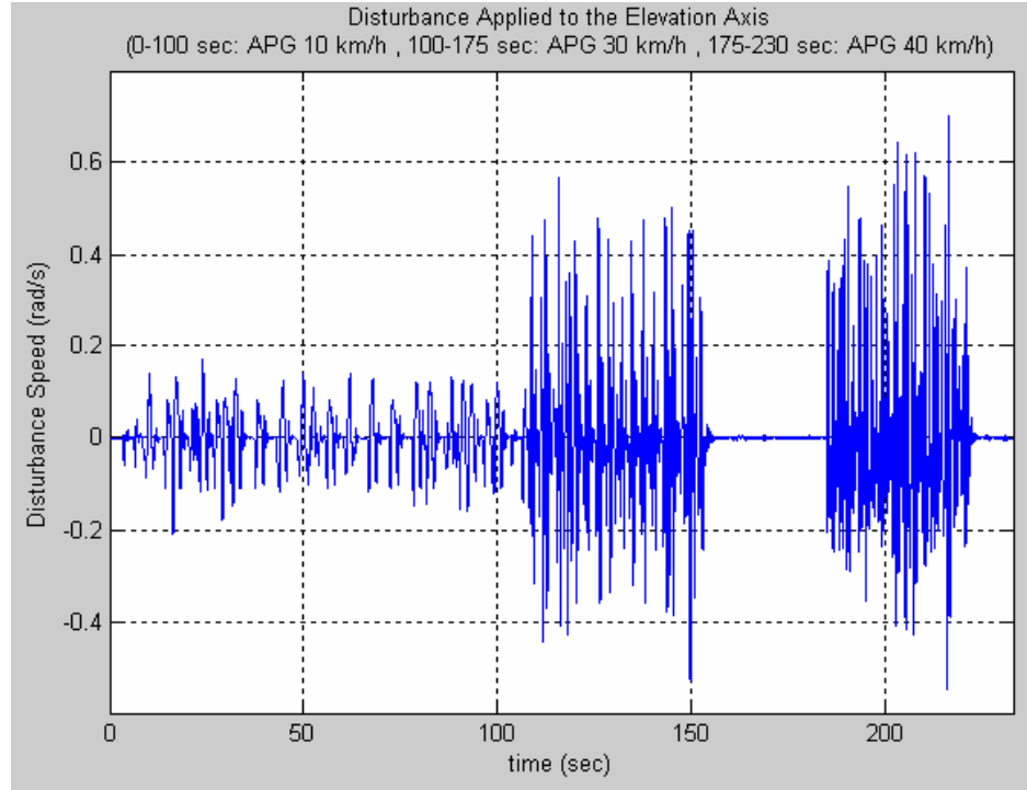
Figure 6.4 – The Disturbance Speed Excerpted on the Elevation Axis for the Performance Analysis of the Neural PID Tuner
