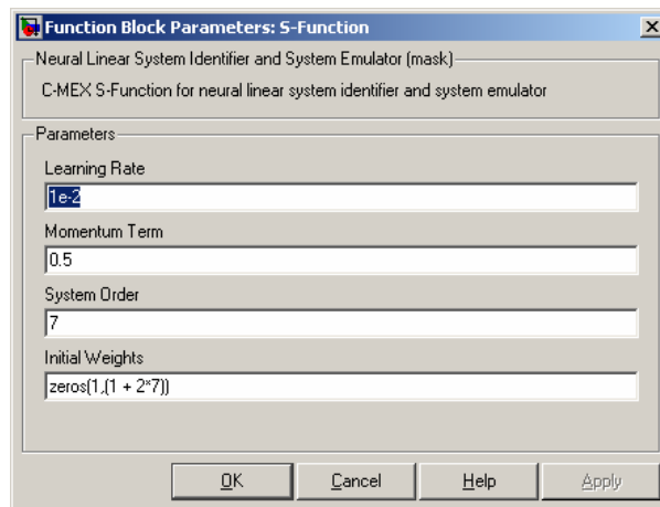
Figure 5.3 - Graphical User Interface for Neural Linear System Identifier and System Emulator
