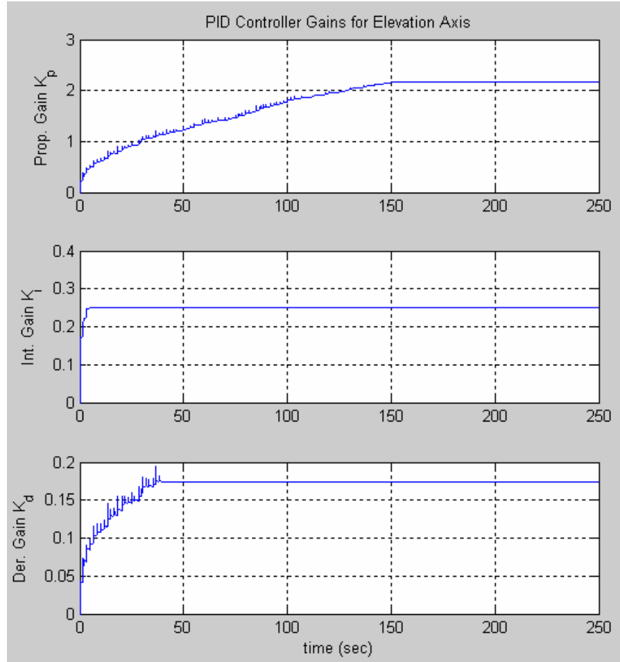
Figure 5.15 – Simulation Result for the Elevation Axis – PID Controller Parameters Learned Through the Simulation on APG Track with 10 km/h Speed
