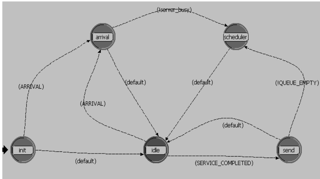
Figure 5-2 State Transition Diagram of Virtual Clock Router
