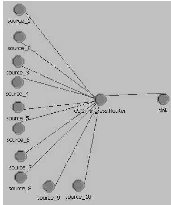
Figure 5-12 CSGT Ingress Router Simulation Topology-1
