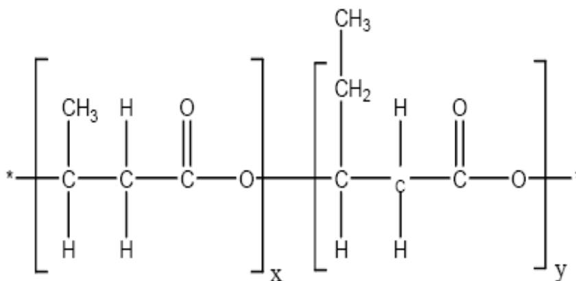
Figure 11. Poly(3-hydroxyalkanoate) (P3HA).
