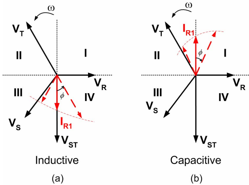
Figure 2.7 Phasor diagram of CSC in a lossless system (transient-state representation) (a) for inductive (b) capacitive reactive power generation
