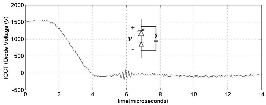
(b) current and voltage waveforms of incoming device under load turn-on
