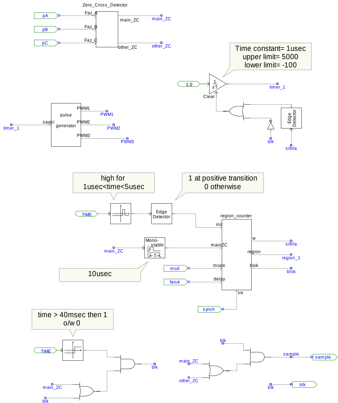
Figure C.8 Details of “STATCOM_Control” block shown in Fig.C.1
