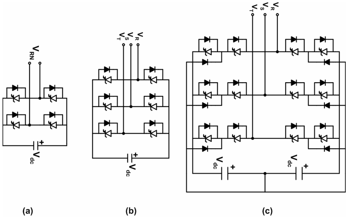
Figure 1.8 Basic converter schemes used for STATCOM [3]
