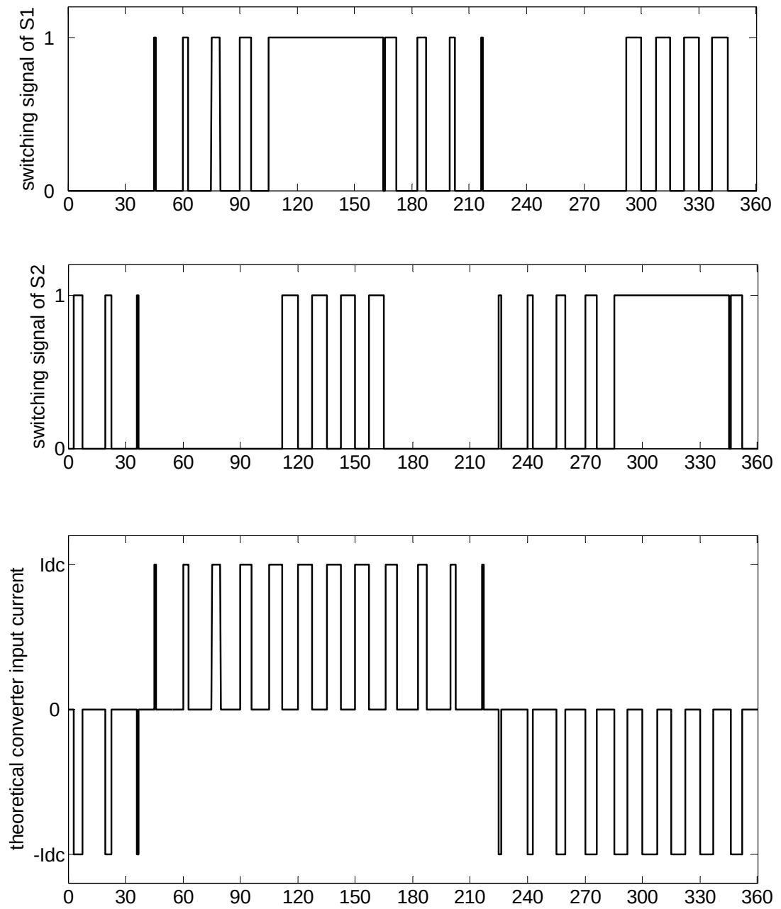
Figure 2.12 Typical switching patterns for SVPWM ( M=0.5 , f_{carrier}=1200\text{Hz} )
