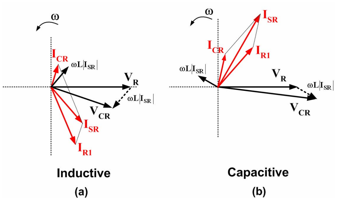
Figure 2.10 Illustration of variations in converter input voltage, V_{CR} with the generated reactive power of CSC
