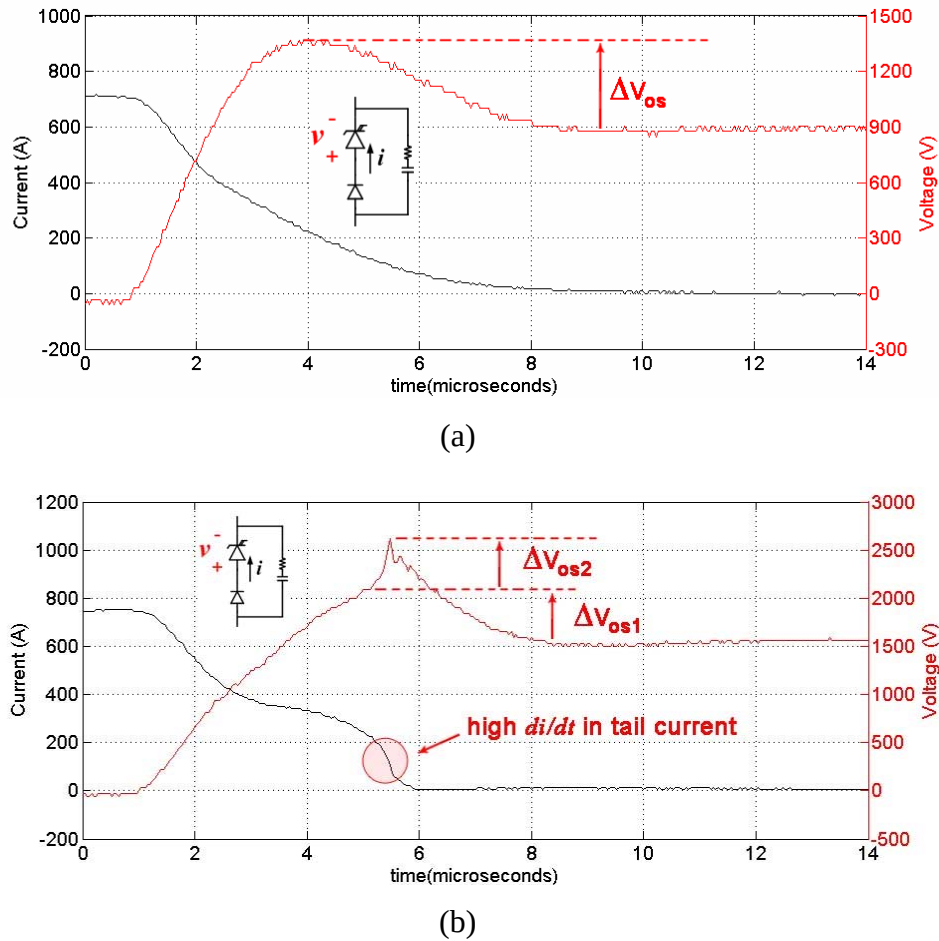
Figure 4.5 Non-linear switching characteristics of IGCT (a) smooth forced turn-off of IGCT, (b) undesired forced turn-off of IGCT, where high di/dt exists in “tail” part of IGCT current (sampling rate= 25MS/sec)
