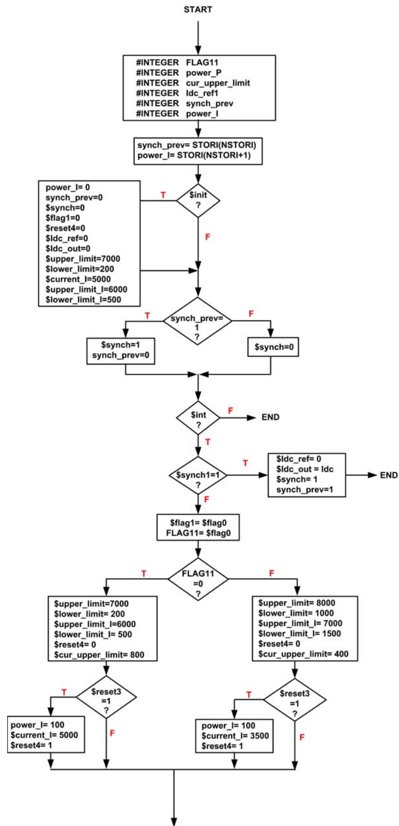
Figure C.6 Flowchart of “Reactive Power Controller” block in Fig.C.1
