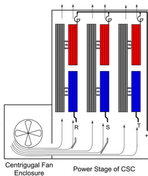
Figure 3.29 Utilization of ventilation for Low Voltage Container for cooling power stage of CSC
