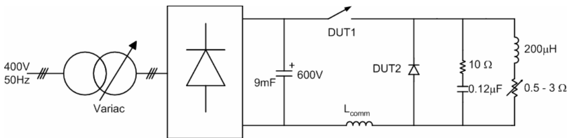
Figure 3.9 Test circuit for obtaining the switching characteristics of power semiconductors
