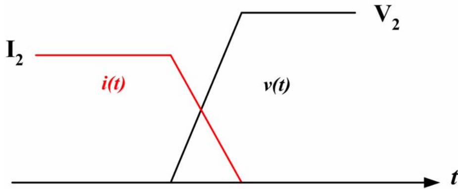
Figure E.3 Typical voltage and current waveforms of fully controllable power semiconductor during forced turn-off in PSCAD/EMTDC (not-to-scale)
