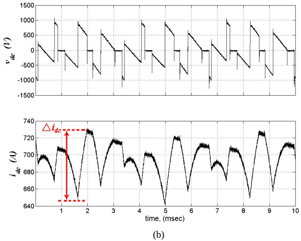
Figure 4.15 DC link waveforms of CSC for (a) 500kVAr capacitive and (b) 500kVAr inductive reactive power generation of STATCOM (sampling rate= 1MS/sec)
