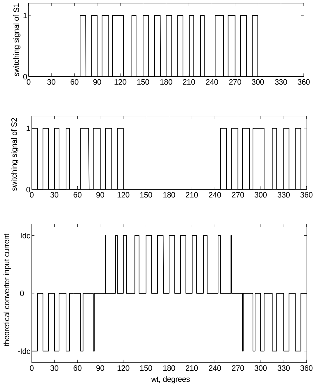
Figure 2.11 Typical switching patterns for MSPWM ( M=0.5 , f_{\text{carrier}}=1200\text{Hz} )
