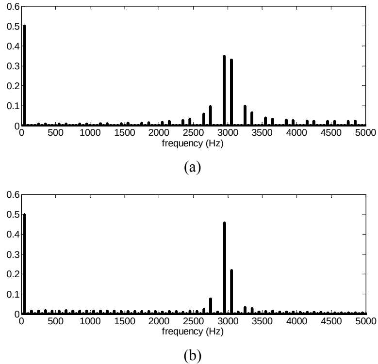
Figure 2.15 Normalized harmonic spectra of converter input current w.r.t. dc-link current (a) for MSPWM (b) for SVPWM when carrier frequency, f_{\text{carrier}} = 3\text{kHz}
