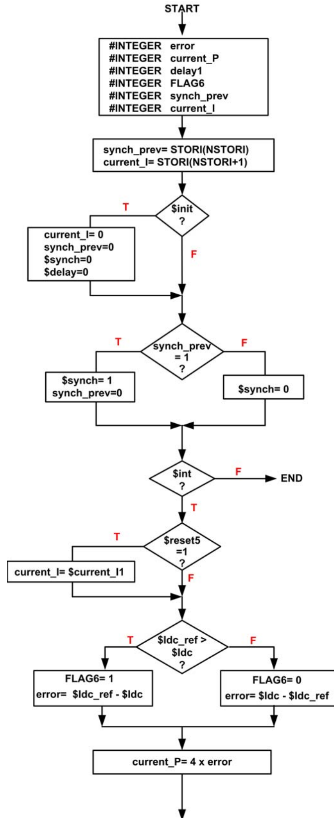
Figure C.7 Flowchart of “Current Controller” block in Fig.C.1
