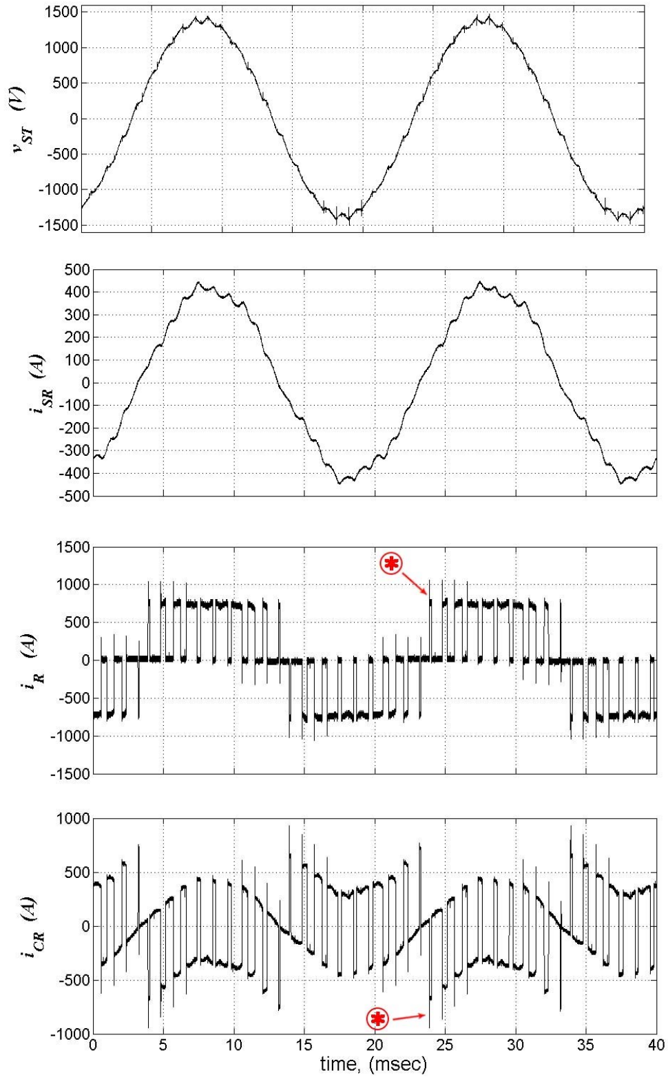
Figure 4.11 AC side waveforms of CSC based STATCOM at 1kV during 550kVAr inductive reactive power generation of STATCOM ( * - reverse recovery current of diode under load turn-off through IGCT under device turn-on and capacitor) (sampling rate= 1MS/sec)
