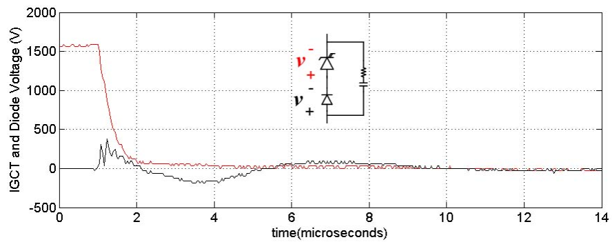
(b) current and voltage waveforms of incoming device under device turn-on
