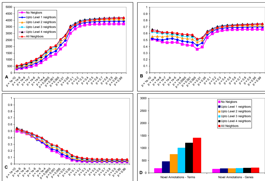
Figure 7.6. Homology, biological process terms
