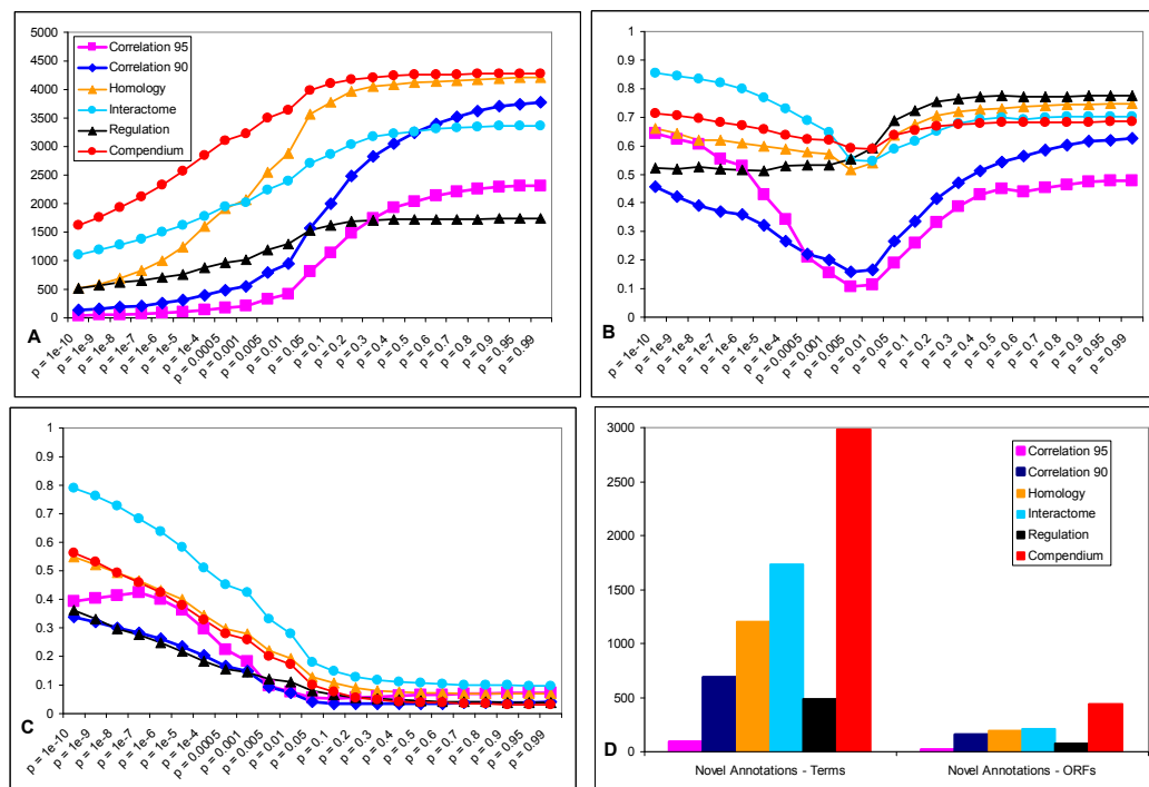
Figure 7.14. Comparison of all networks including 4 neighbors, biological process terms
