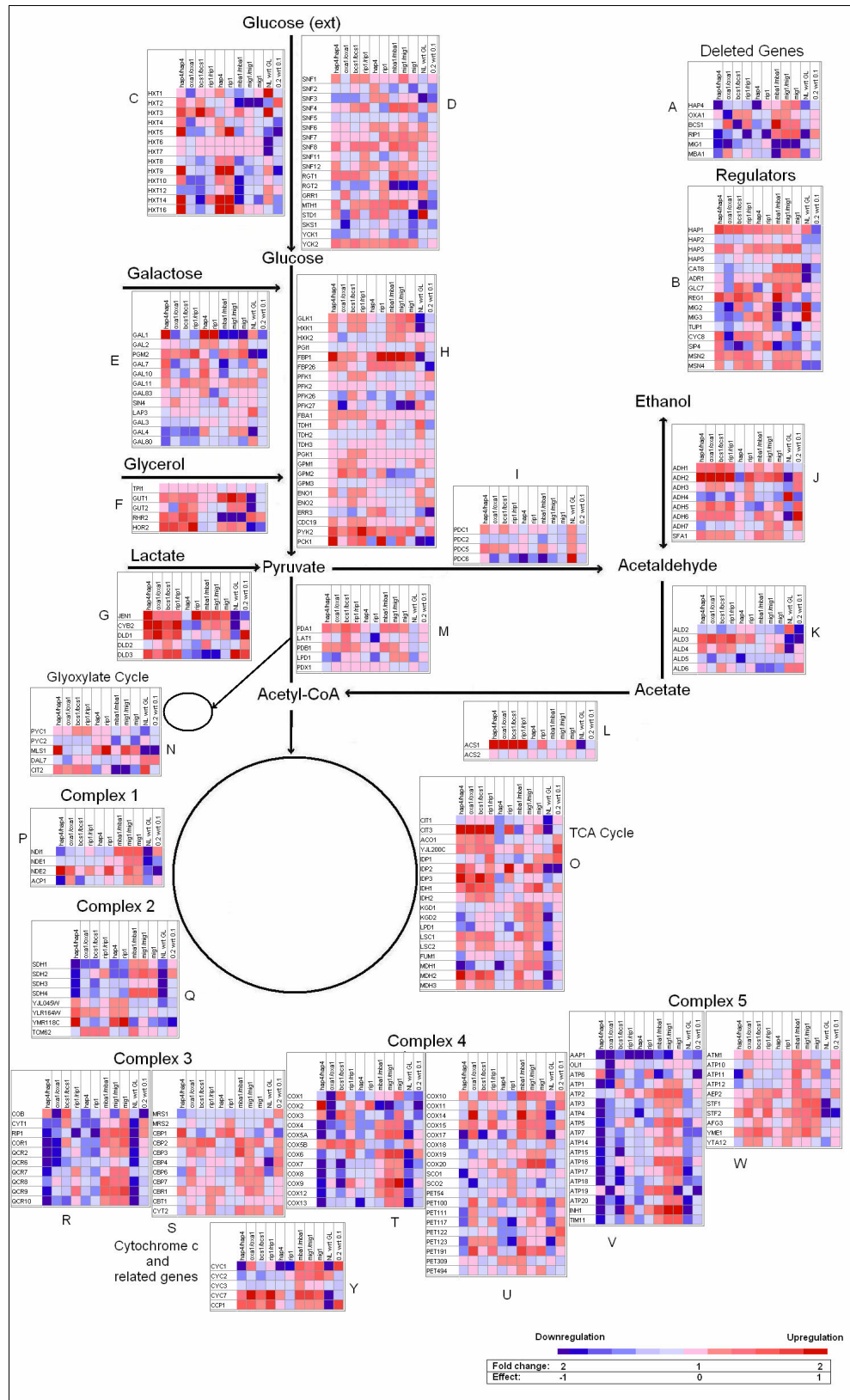
Figure 4.1. Expression profiles of selected genes.
