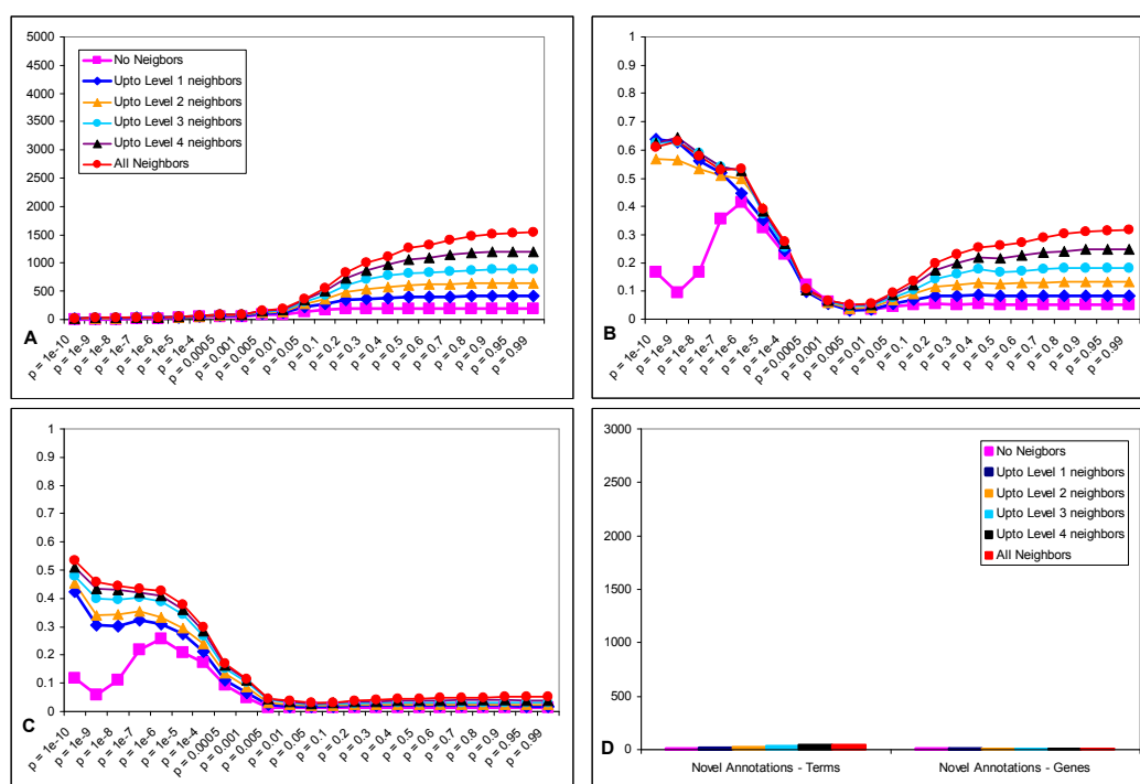
Figure 7.4. Expression correlation ( \rho > 0.95 ), molecular function terms
