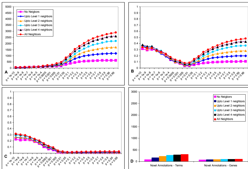
Figure 7.5. Expression correlation ( \rho > 0.90 ), molecular function terms
