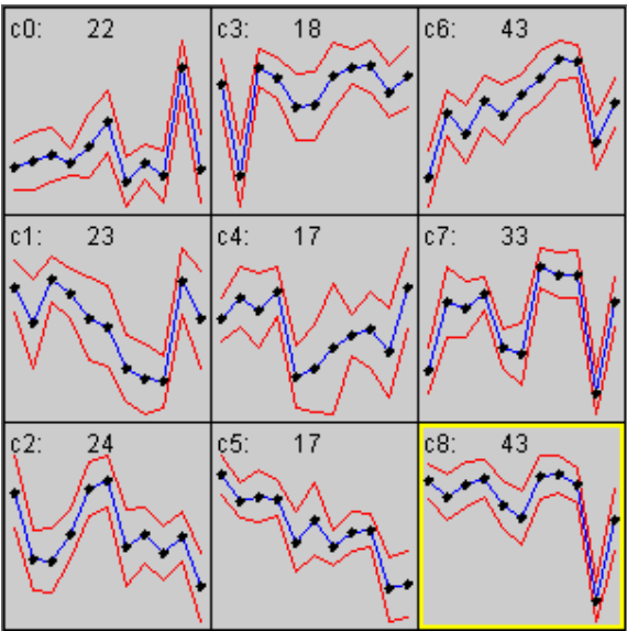
Figure 4.4. Centroids of clusters of central metabolism genes.
