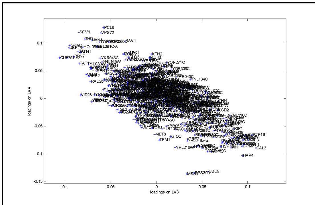
Figure 5.9. Loadings of ORFs on third and fourth LVs.
