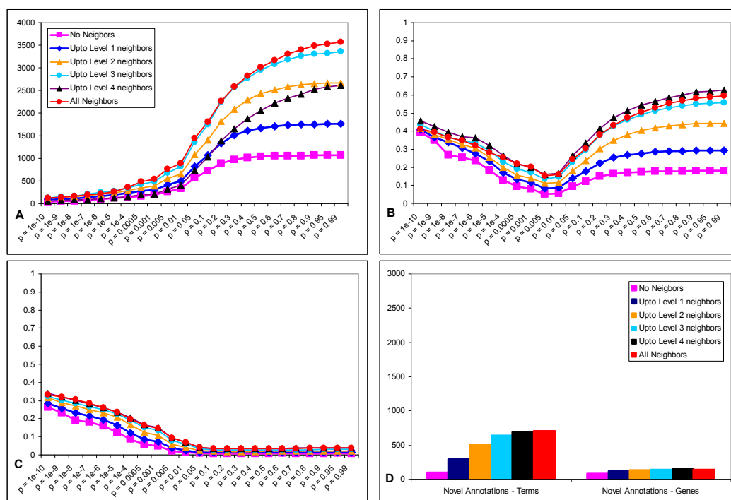
Figure 7.3. Expression correlation ( \rho > 0.90 ), biological process terms
