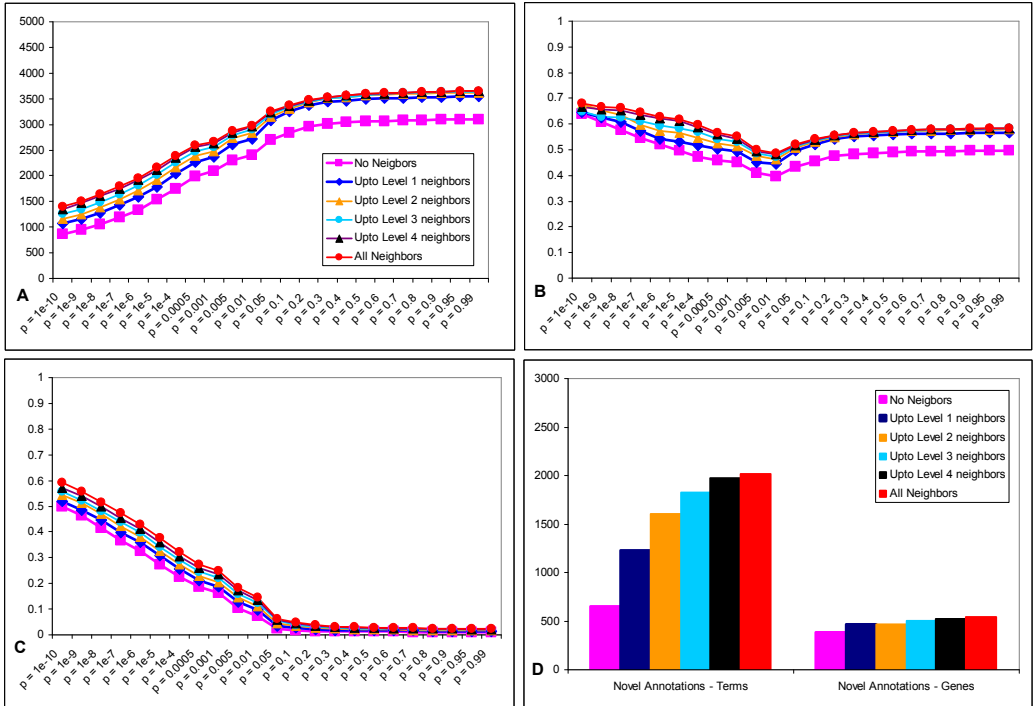
Figure 7.13. Compendium network, molecular function terms
