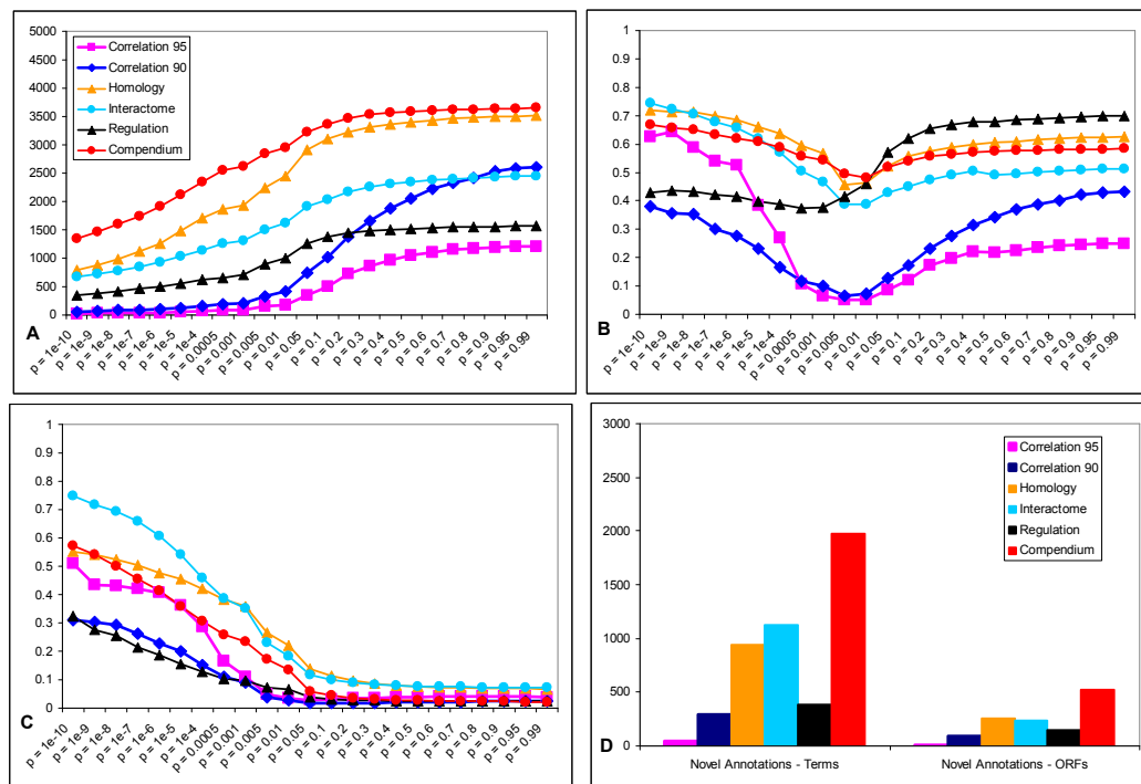
Figure 7.15. Comparison of all networks including 4 neighbors, molecular function terms
