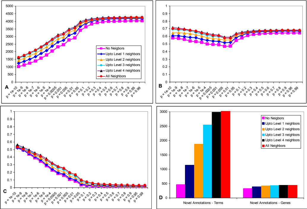
Figure 7.12. Compendium network, biological process terms
