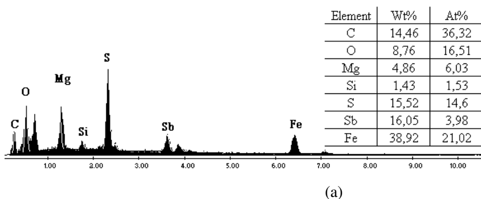
Figure 4.6. The EDX analyses results of the specimen surfaces shown in Figure 4.5,
