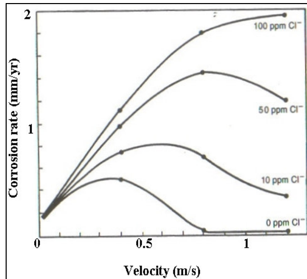
Figure 2.10. Effect of water velocity and chloride concentrations on corrosion of carbon steel. Distilled water+NaCl, 50 °C, 14 days (Herce 1995).
