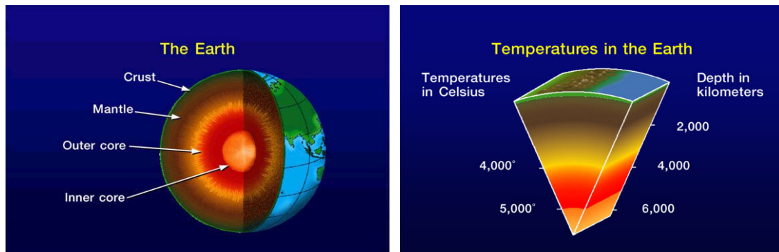
Figure 1.3. Temperatures in Earth and layer of the Earth (Nemzer and Carter 2000).
