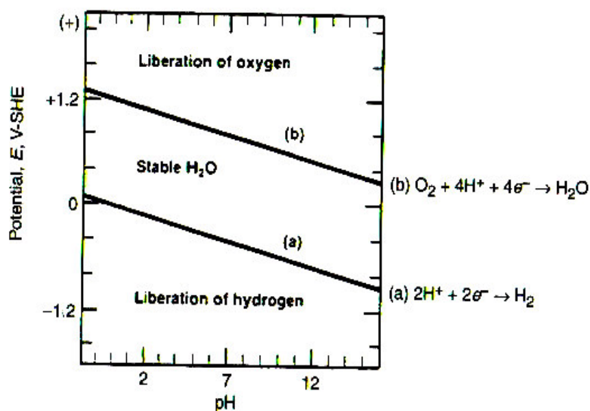
Figure 2.4. Potential-pH diagram for water (Davis 2003).
