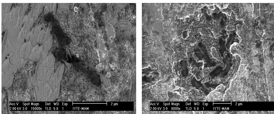
Figure 4.14. SEM images of the SRB inside the pits after (a) 336 h and (b) 1207 h exposure.
