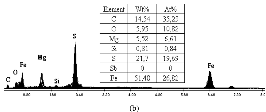
Figure 4.8. The EDX analyses results of the cross-section shown in Figure 4.7, (a) section A and (b) section B.
