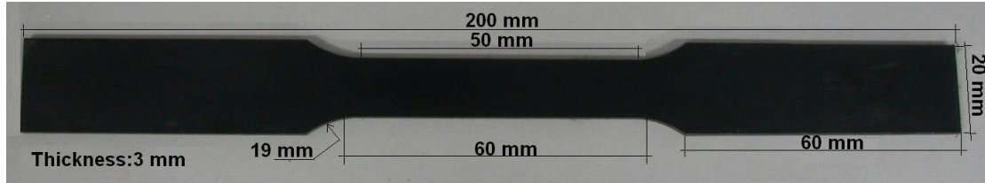
Figure 3.5. St-37 steel tensile test specimen machined according to ASTM E-8 and dimensions.
