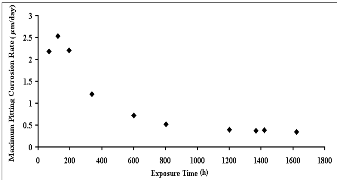
Figure 4.39. Maximum pitting corrosion rates vs. exposure time of St-37 steel at 9.6 m/s fluid velocity.
