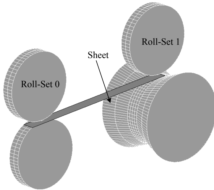
Figure 3.4 Geometry of the model
