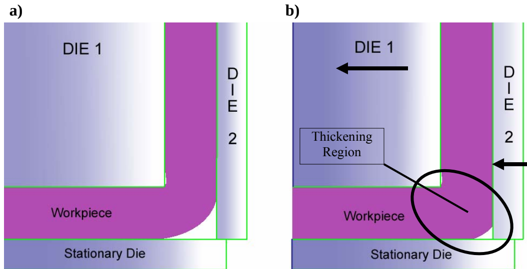
Figure 5.30 The new roll-forming simulation method: a) at the end of a bending process b) at the end of thickening stage
