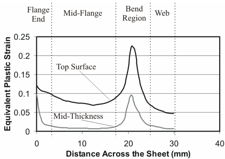
Figure 4.5 Plastic strain distribution on the sheet from flange end to web center
