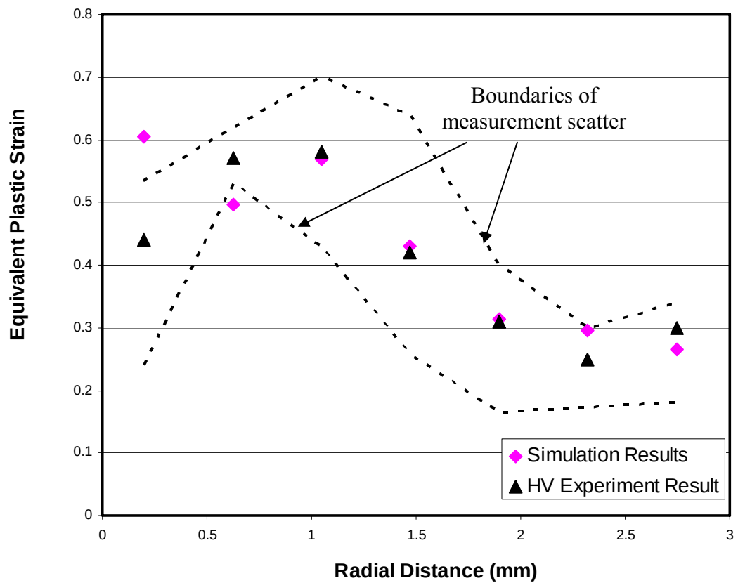
Figure 5.32 Strain distributions obtained from the new forming simulations and HV measurements for the Type-1 90° bend
