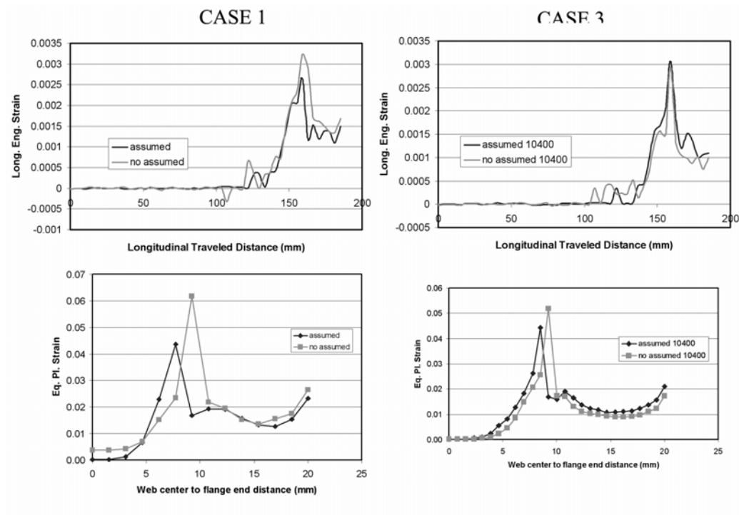
Figure A.4 Effect of Assumed Strain Formulation
