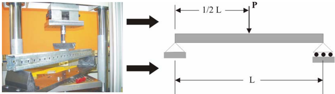
Figure B.1 Idealization of the bending experiment
