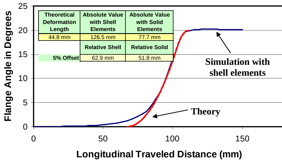
Figure 3.17 Theoretical and numerically found bend angle curve and the deformation length of the sheet
