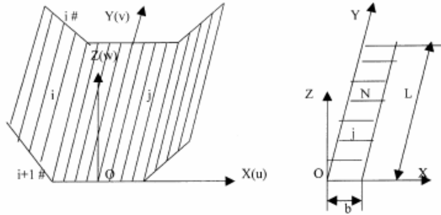
Figure 2.11 Stage is divided into finite strips and B-splines [17]
