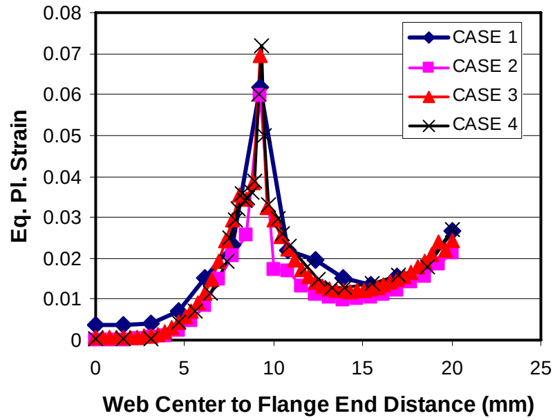
Figure 3.13 Strain hardening on the sheet surface along the transverse direction
