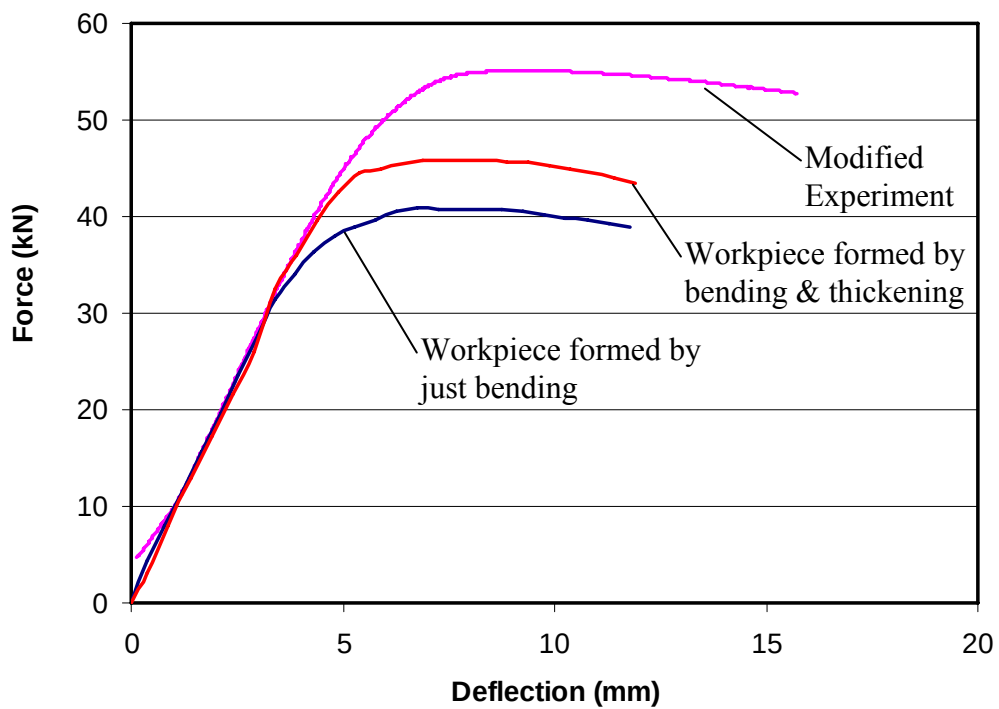
Figure 5.35 Comparison of bending simulation results and the bending experiment data
