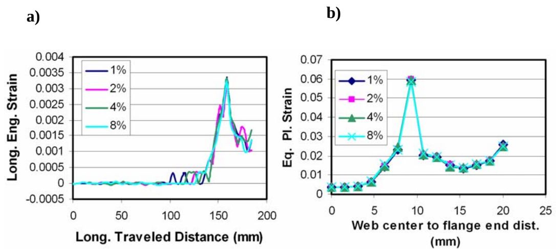
Figure A.2 Effect of contact tolerances. a) Longitudinal engineering strain b) strain hardening on the sheet surface
