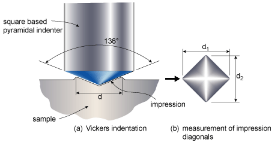
Figure 2.20 Vickers Hardness Indenter
