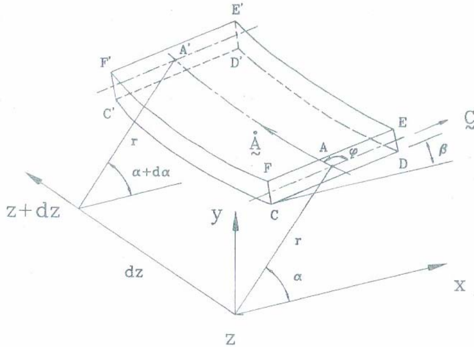
Figure 2.7 Small element in shear [13]
