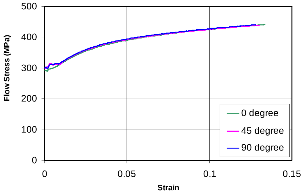
Figure 5.2 Tension flow curves in different orientations
