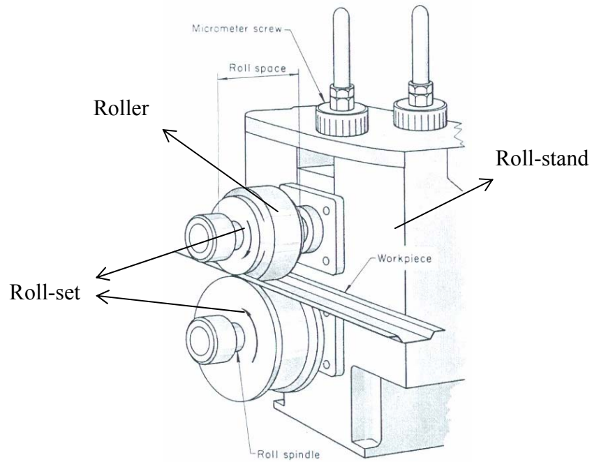
Figure 1.6 Roll-forming machine with overhung spindle [4]
