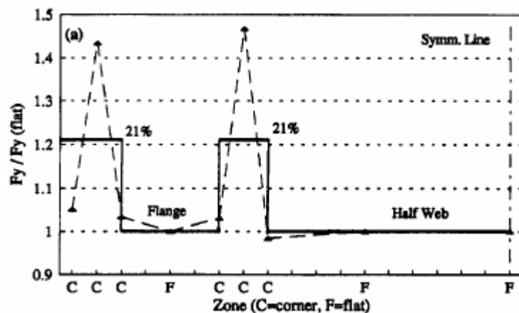
Figure 2.17 Idealization of the yield strengths for the flat and curved parts [20]
