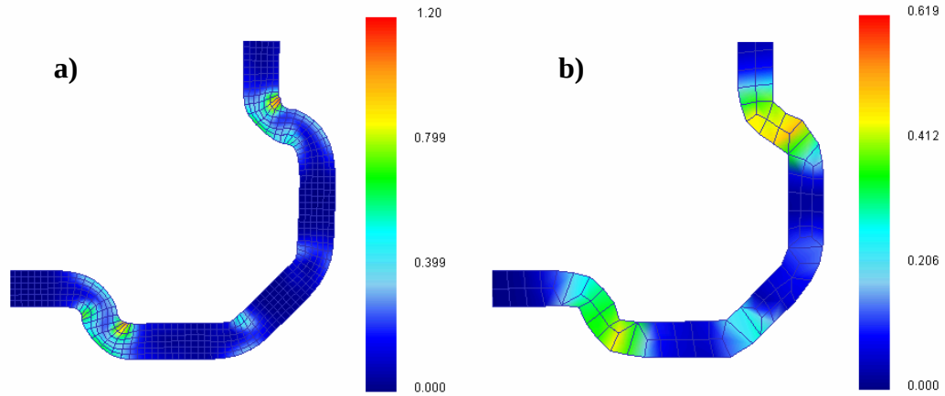
Figure 5.24 Equivalent Plastic Strain distribution and final geometry of simulations with a) 1500 and b) 200 elements
