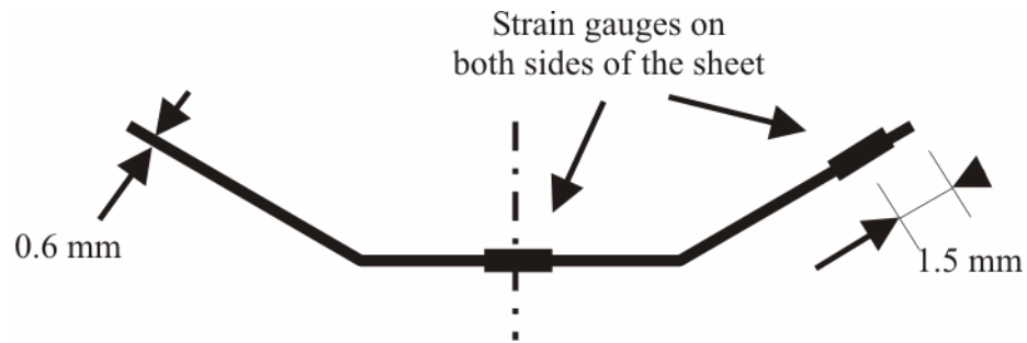
Figure 3.1 Investigated channel section and the locations of the strain gauges
