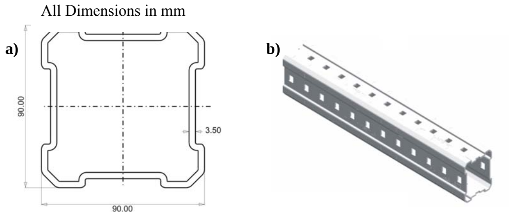
Figure 5.1 Case study product: a) Cross-section and b) Perspective view
