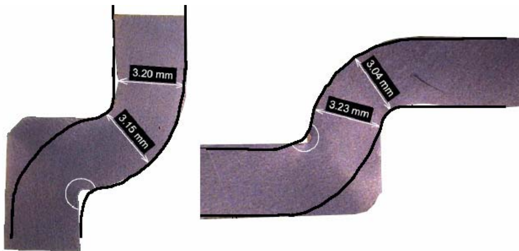
Figure 5.28 Geometrical comparison of simulation results (solid lines) with actual product
