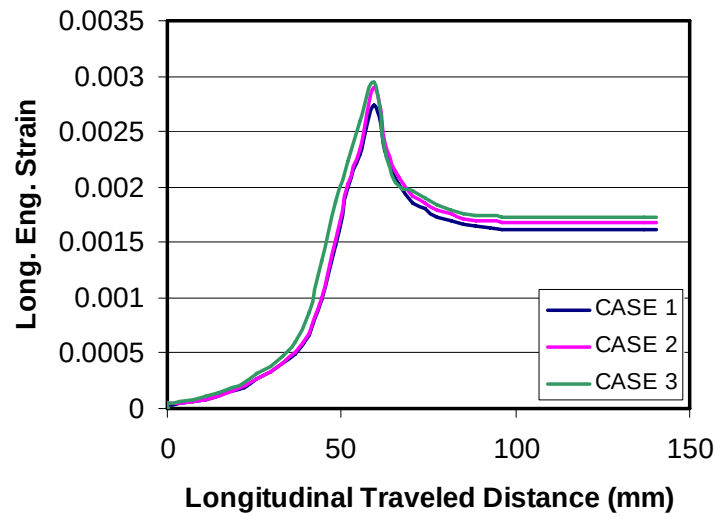
Figure 3.14 Long. eng. strain development in simulations with shell elements
