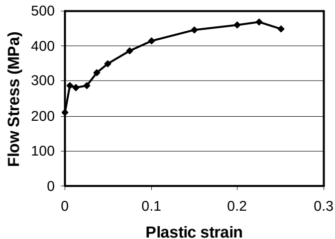
Figure 3.7 Flow Curve of SAE 1020 steel
