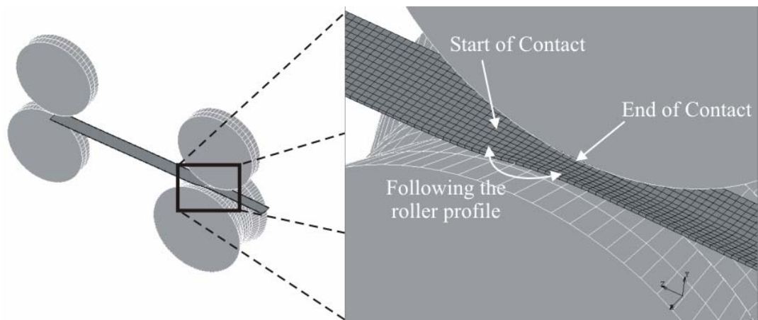
Figure 3.8 Deformation behavior of the nodes
