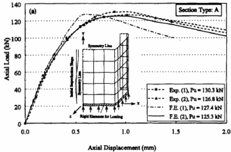
Figure 2.19 Comparison of two finite element models with the experiment [20]
