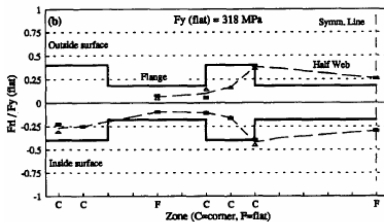
Figure 2.18 Idealization of the residual stress for the flat and curved parts [20]
