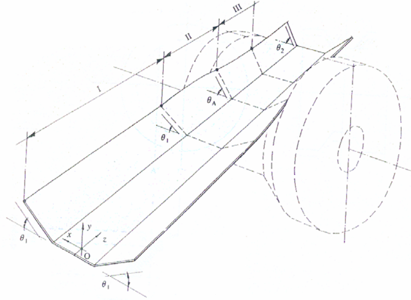
Figure 2.4 Three regions of deforming sheet [12]
