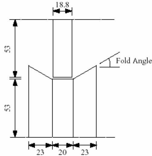
Figure 3.2 Geometry of the rollers
