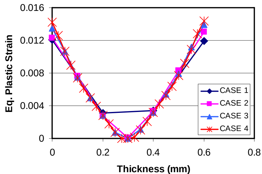
Figure 3.20 Equivalent plastic strain distribution through the thickness
