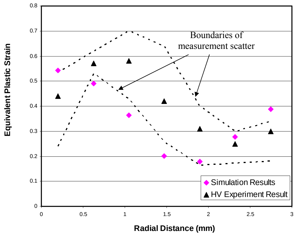
Figure 5.26 Strain distributions obtained from the simulations and HV measurements for the Type-1 90° bend
