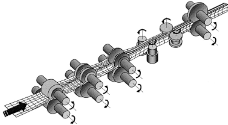
Figure 1.3 Schematic representation of roll-forming [3]
