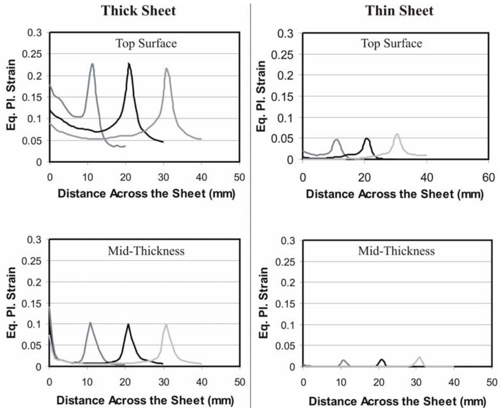
Figure 4.6 Plastic strain distribution across the sheet for thick and thin sheets for flange lengths of 10 mm, 20mm and 30 mm
