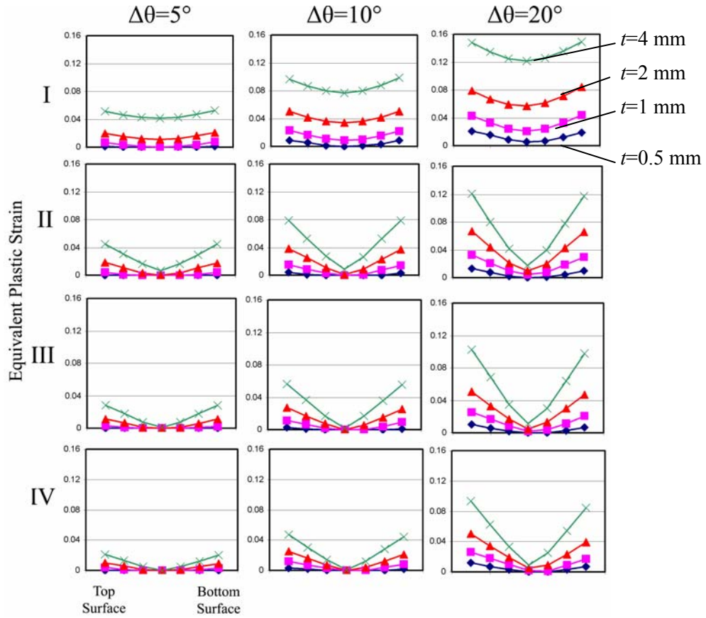
Figure 4.4 Effects of \Delta\theta and t
