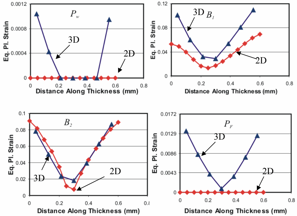
Figure 3.22 Equivalent plastic strain through the thickness at selected locations
