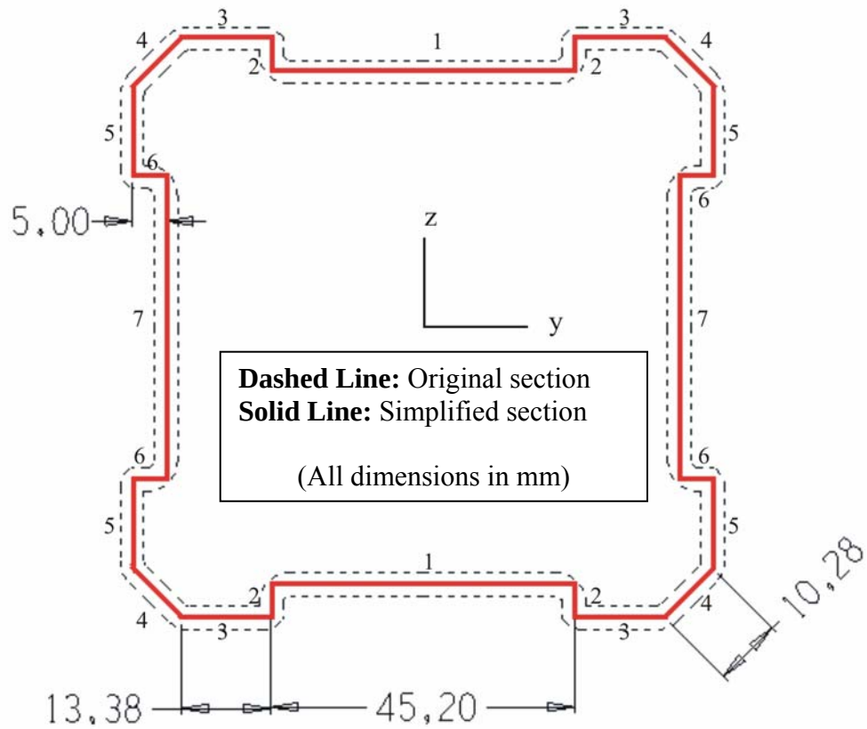
Figure B.2 Simplified section of the product
