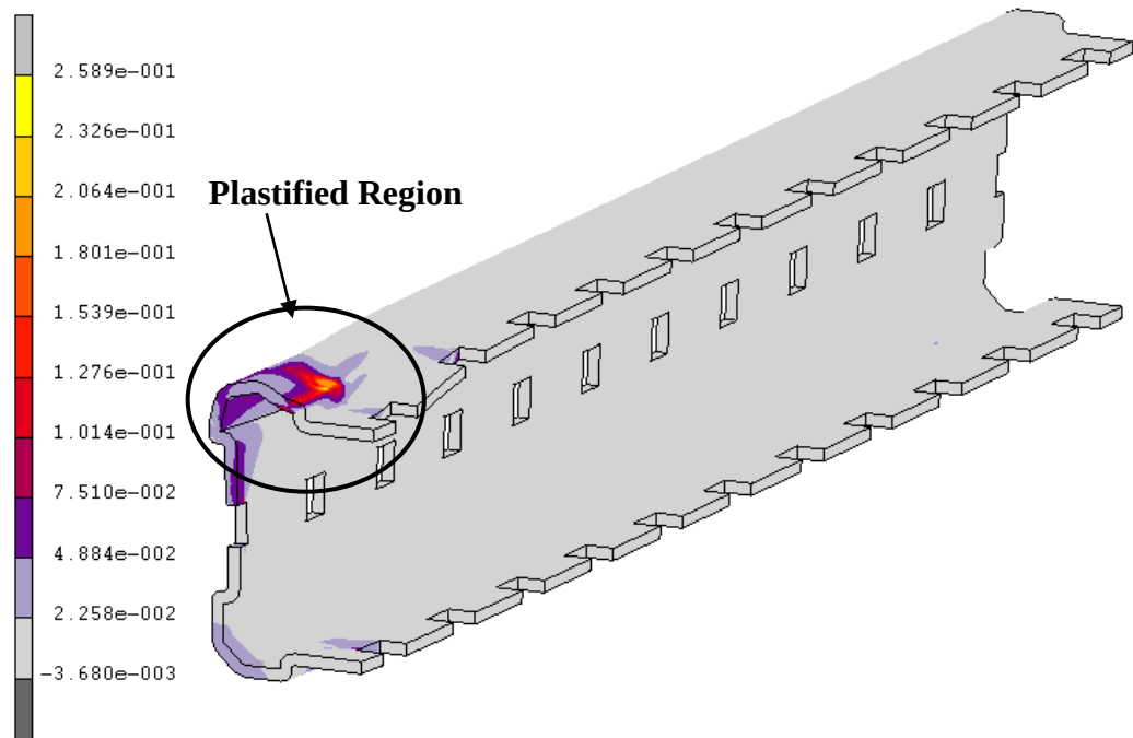
Figure 5.17 Equivalent plastic strain around the localized deformation region
