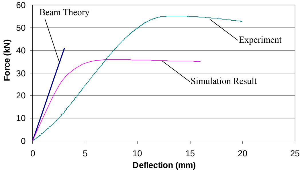
Figure 5.19 Comparison of theory, simulations and experiments
