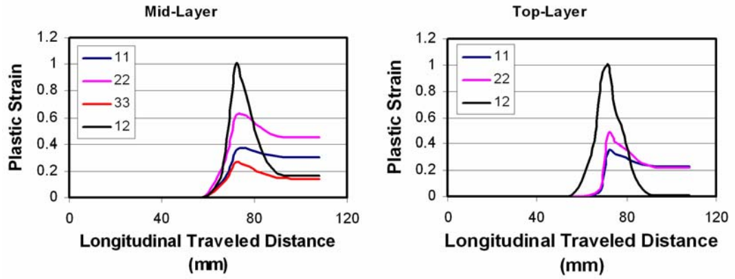
Figure 3.24 Plastic strain tensor component histories in 3D simulation with shell elements at point P_F
