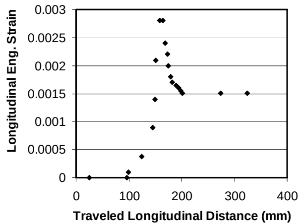
Figure 3.3 Longitudinal engineering strain measurement results for the 20^\circ bend angle
