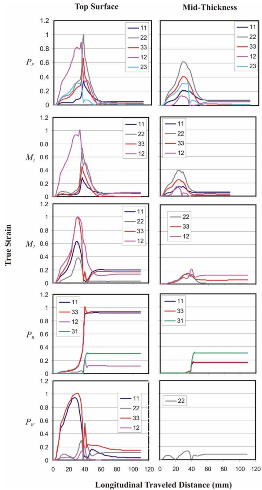
Figure 4.10 True strain values at the specified locations of the 0.5 mm thick sheet
