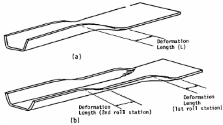
Figure 2.3 Deformation length in roll-forming [11]
