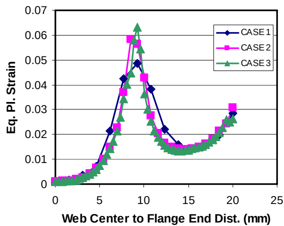
Figure 3.15 Equivalent Plastic Strain distribution on the sheet surface
