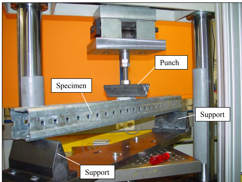
Figure 5.5 Bending experiment setup
