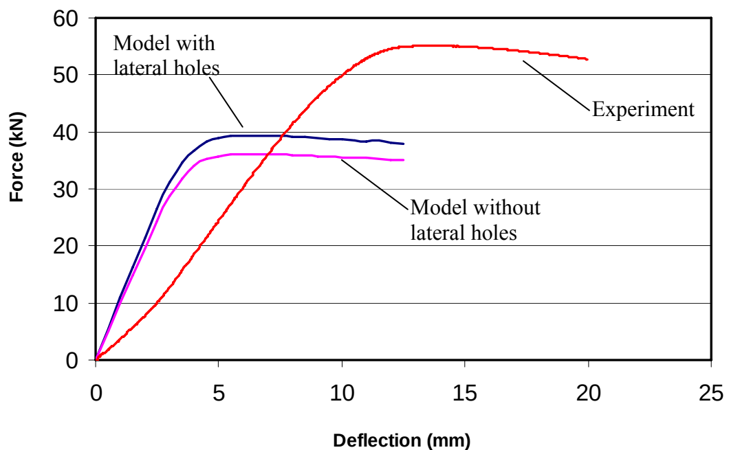
Figure 5.14 Punch force vs. punch displacement curves
