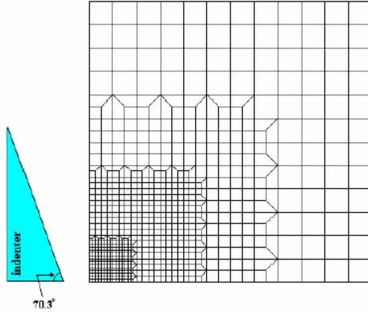
Figure 2.21 Finite element mesh and conical indenter used in Vickers Hardness simulations [27]
