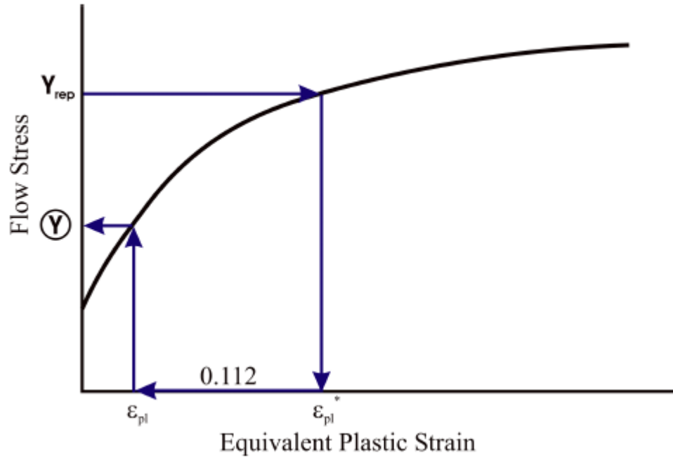
Figure 2.22 Procedure to find the actual yield stress of the material
