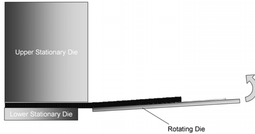
Figure 3.19 Plane strain model of the roll-forming process
