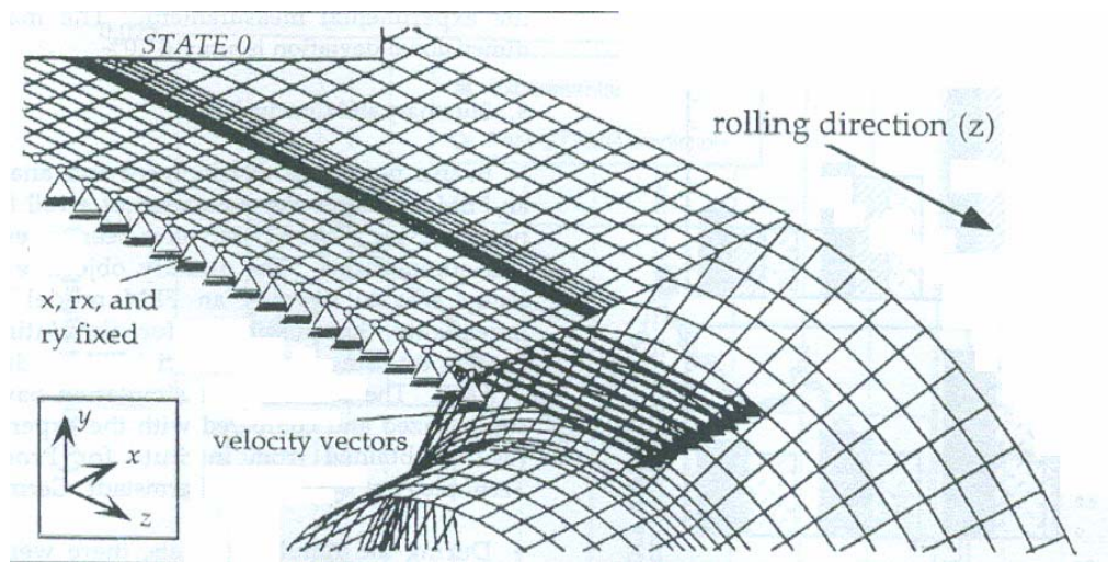
Figure 2.9 Undeformed sheet and the velocity field imposed to the nodes [15]
