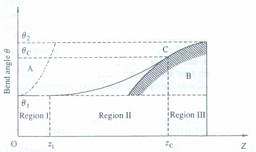
Figure 2.5 Bend angle diagram [12]
