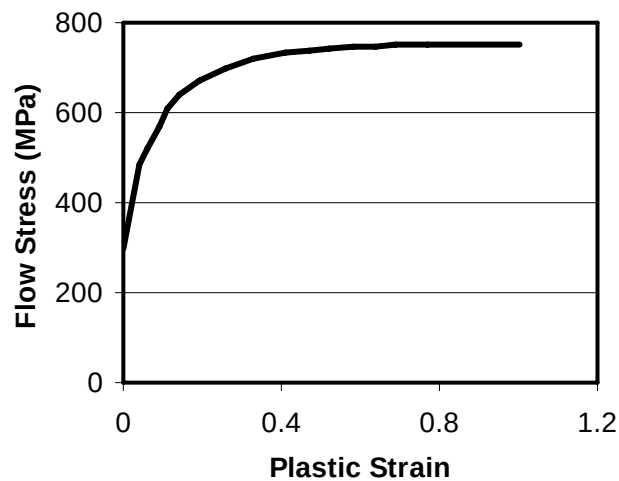
Figure 4.1 Flow curve of C15 steel
