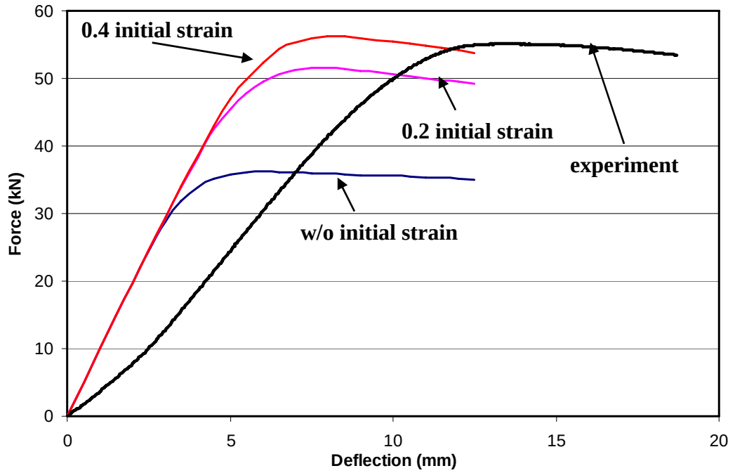
Figure 5.16 Effect of strain hardening
