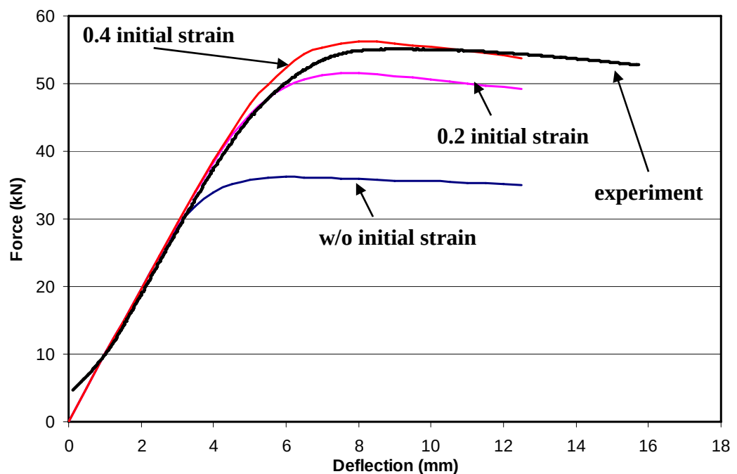
Figure 5.21 Modified experiment data and curves for different initial strain values
