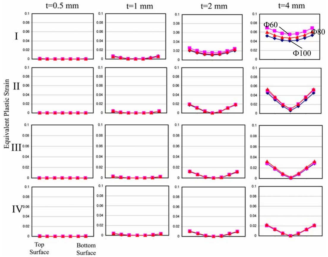
Figure 4.3 Effect of roller diameter
