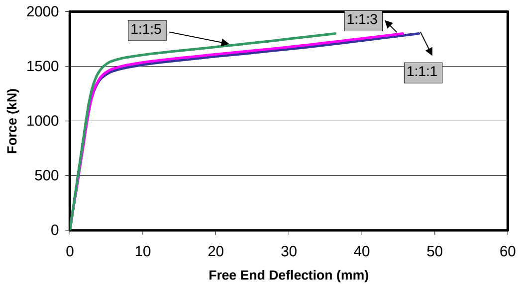
Figure 5.10 Effect of aspect ratio
