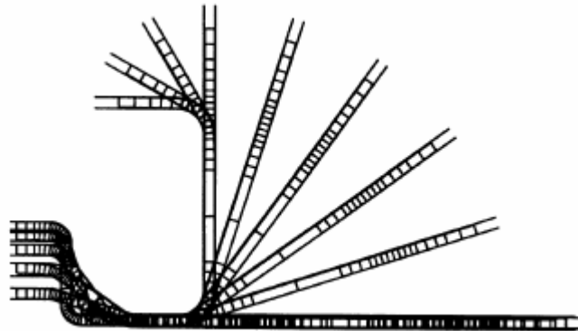
Figure 2.13 Deformed meshes of 2D cross-section analysis [19]
