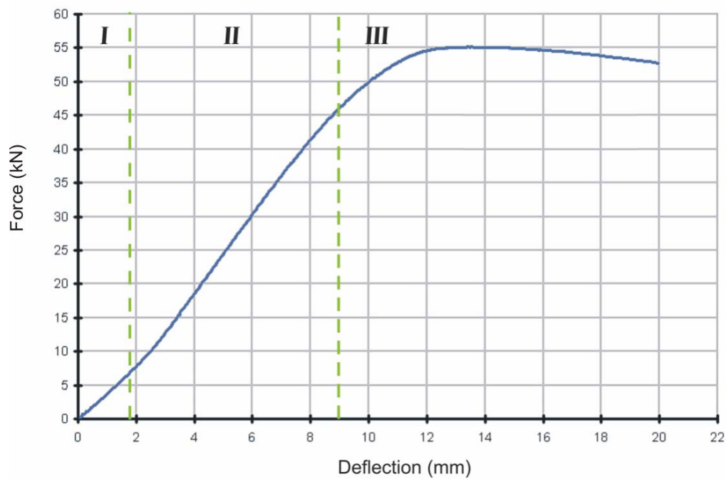
Figure 5.6 Bending experiment result
