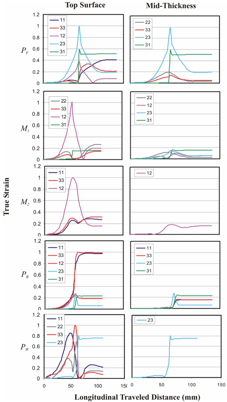
Figure 4.9 True strain values at the specified locations of the 4 mm thick sheet
