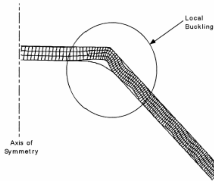
Figure 2.10 Plane strain simulation of roll-forming by vertically moving dies [16]
