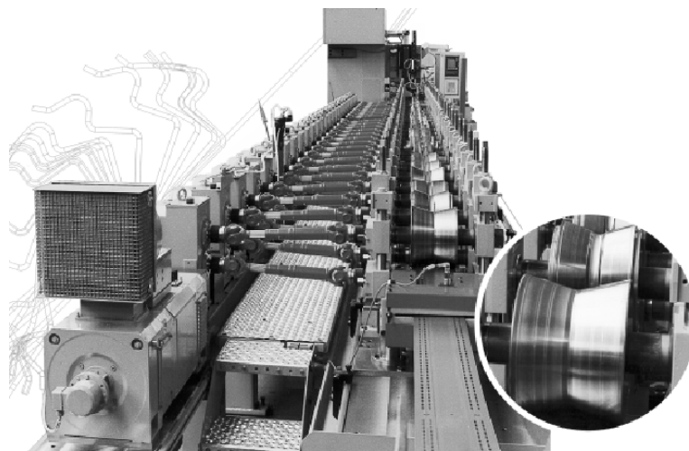
Figure 1.7 Roll-forming machine with outboard support [8]
