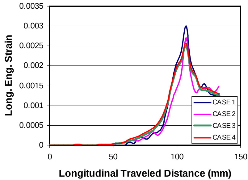
Figure 3.12 Longitudinal strain development with four mesh densities
