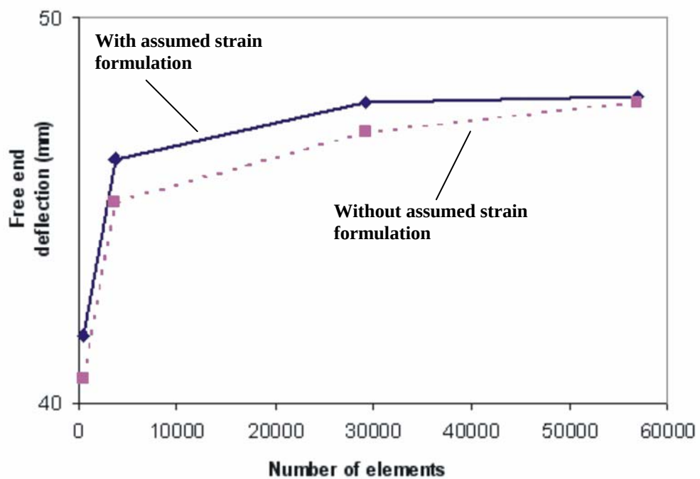
Figure 5.11 Significance of assumed strain formulation
