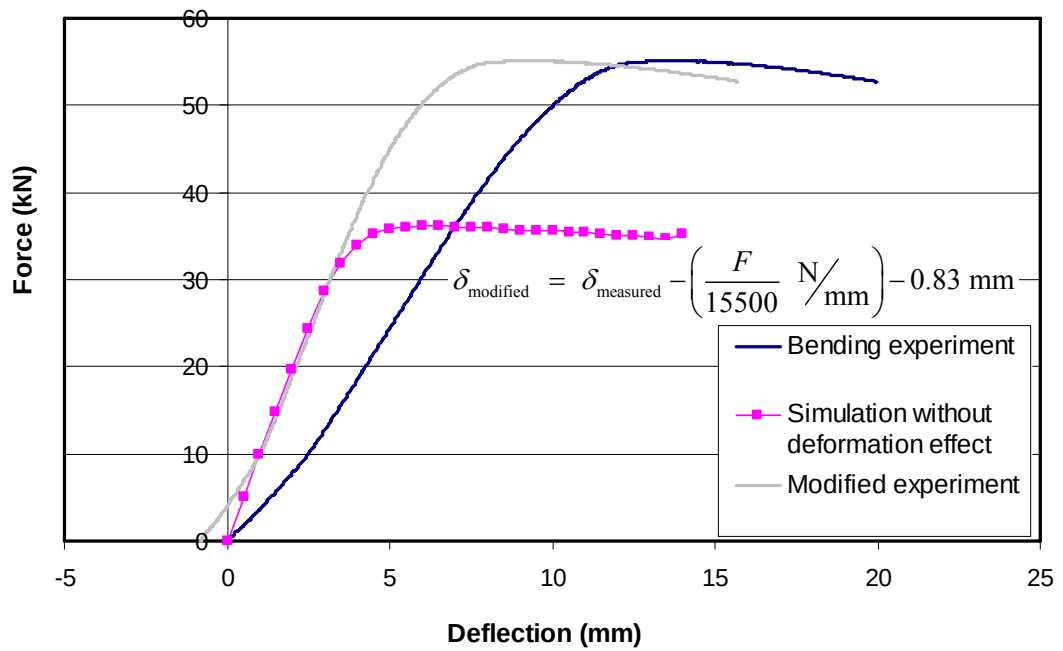
Figure 5.20 Modification of the bending experiment results
