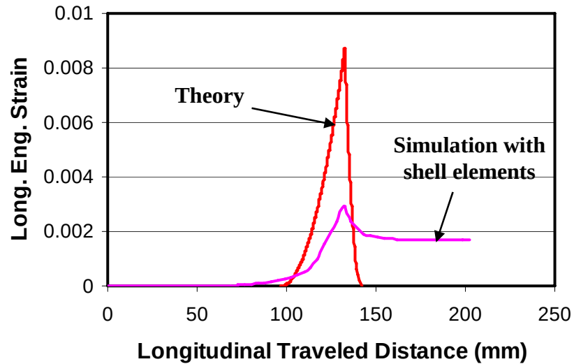
Figure 3.18 Theoretical, experimental and numerically found longitudinal engineering strain curves
