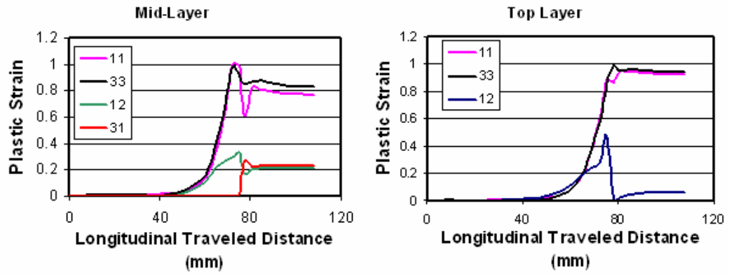
Figure 3.25 Plastic strain tensor components histories in 3D simulation with shell elements at point B 2
