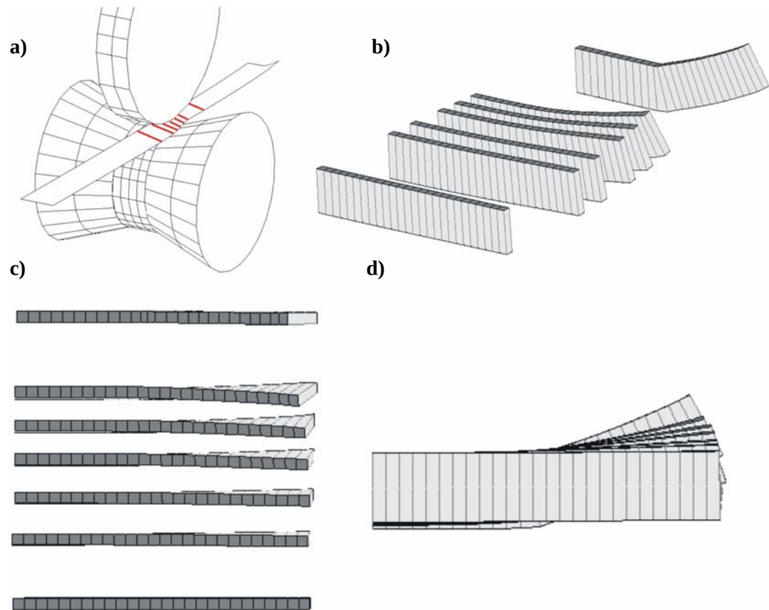
Figure 4.11 Geometry of the sheet passing through the roller. a) Examined sections b) Perspective view of the sections c) Top view d) Front view
