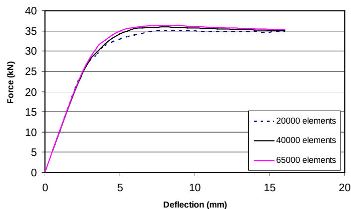
Figure 5.13 Convergence analysis according to number of elements
