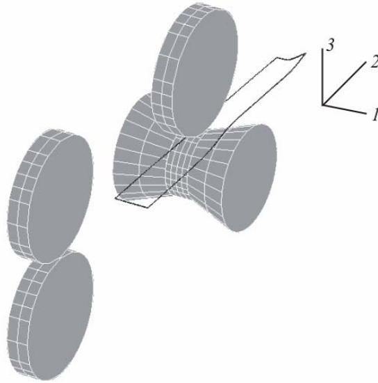
Figure 4.8 Directions of the tensorial components
