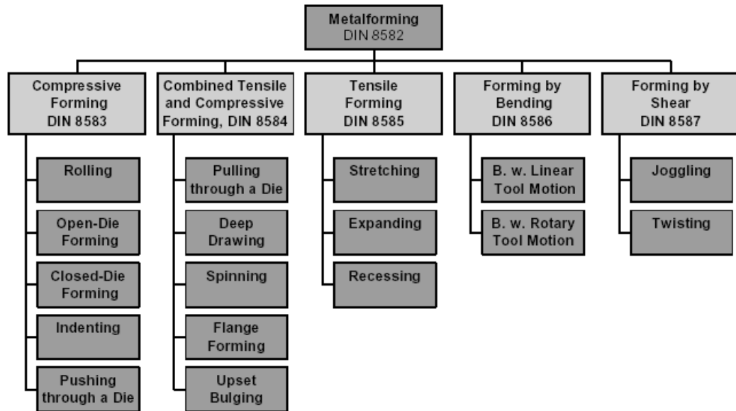
Figure 1.2 Classification of metal forming according to the primary stress in the deformation zone [1]
