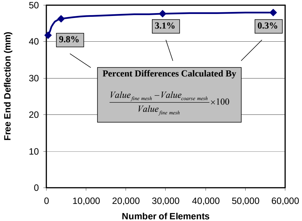
Figure 5.8 Result of the convergence analysis
