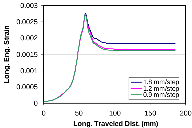
Figure A.6 Effect of step size
