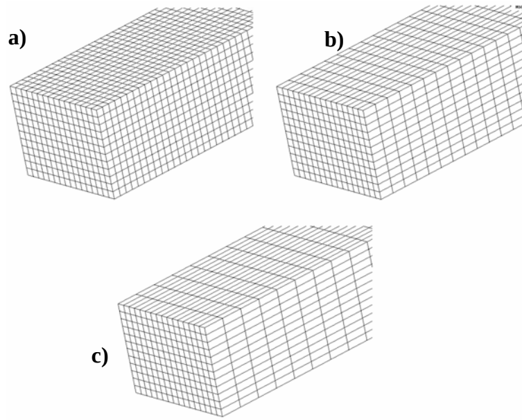
Figure 5.9 Meshes with different aspect ratios: a) 1:1:1, b) 1:1:2, c) 1:1:3
