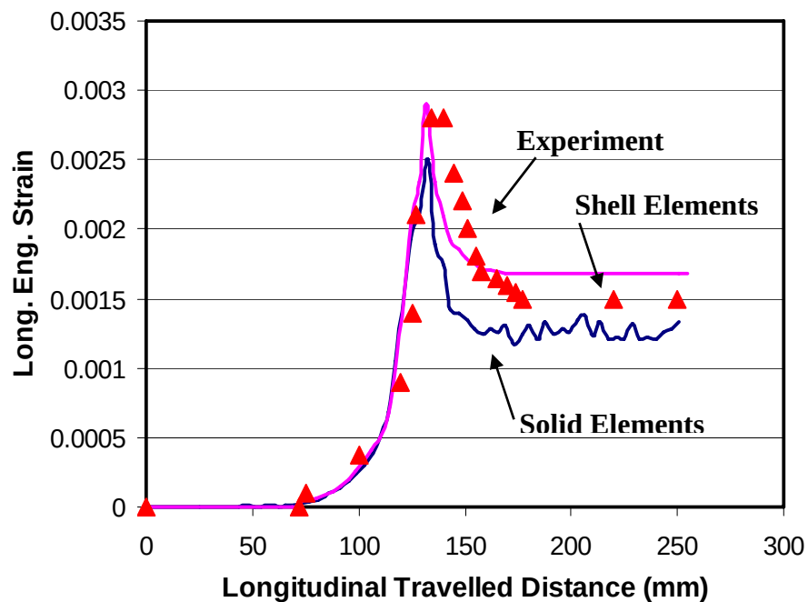
Figure 3.16 Long. eng. strain development in simulations and experiment
