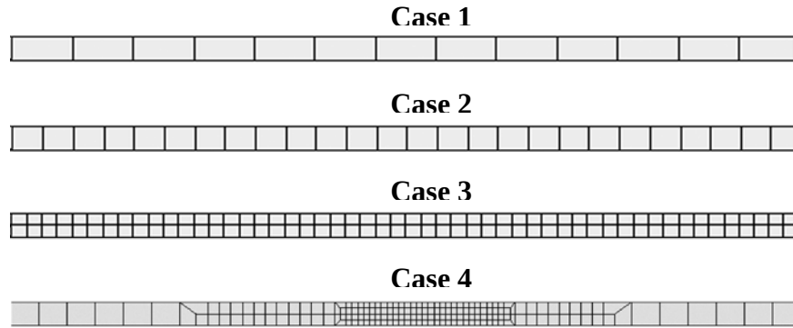
Figure 3.11 Cross-sections of the sheet with different mesh densities
