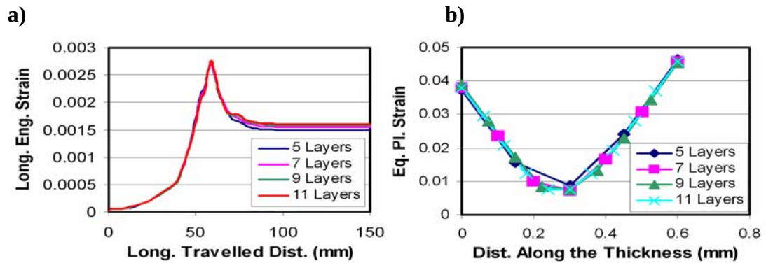
Figure A.5 Effect of number of layers: a) on longitudinal engineering strain b) on strain hardening on the sheet surface
