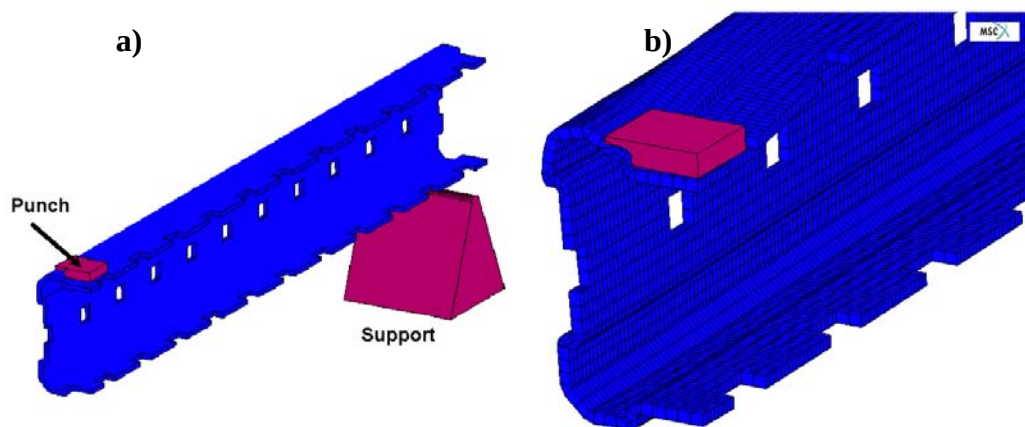
Figure 5.12 a) The model for the simulations with lateral holes b) Close view of the deformed region
