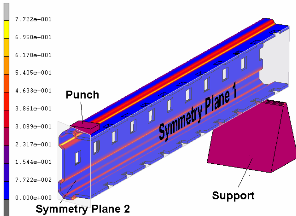
Figure 5.34 Initial plastic strain distribution along the workpiece
