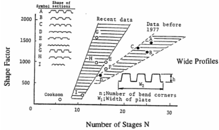
Figure 2.2 Shape Factor Method [10]
