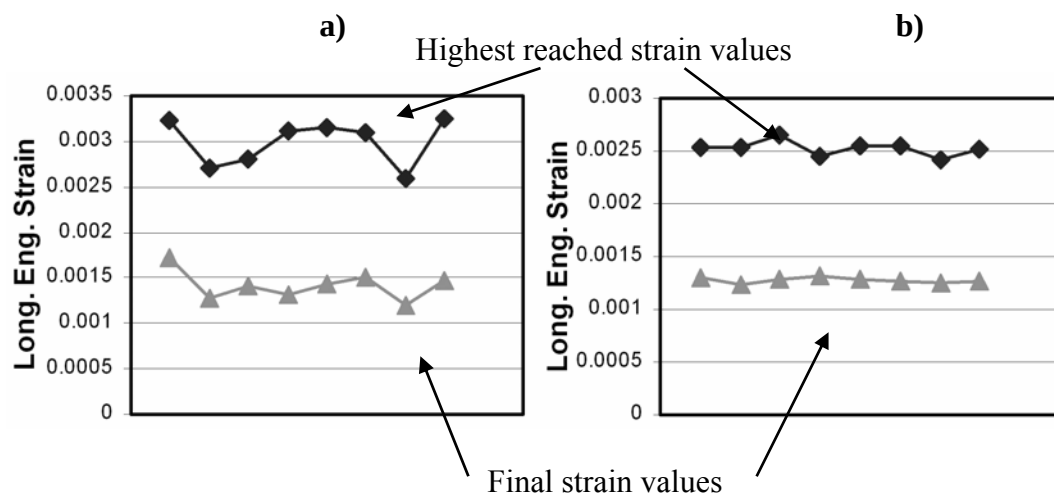
Figure 3.9 Oscillations in results a) with coarse mesh b) with fine mesh
