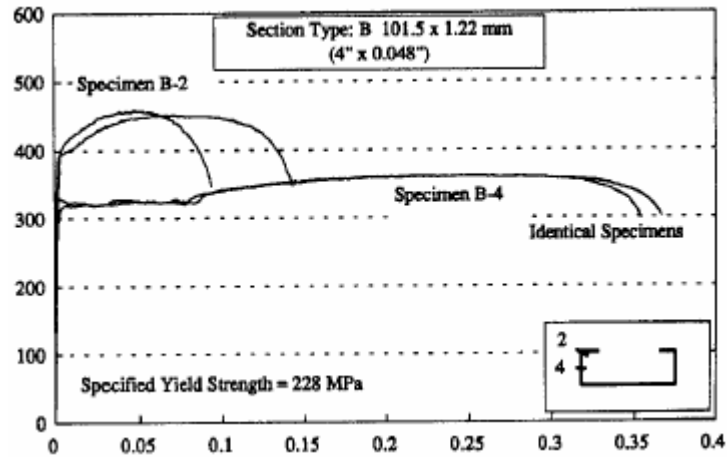
Figure 2.16 Sample tensile test results of specimens cut from flat and curved regions of the cross-section [20]
