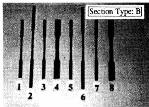
Figure 2.15 a) The roll-formed steel member and regions that the tensile test coupons are cut from b) Tensile test coupons taken from the cross-section [20]
