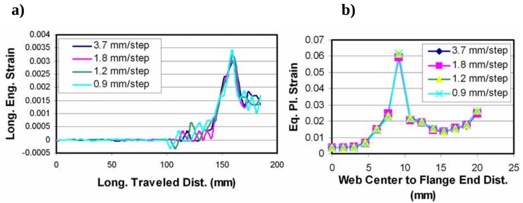
Figure A.3 Effect of step size: a) on longitudinal engineering strain b) on strain hardening on the sheet surface
