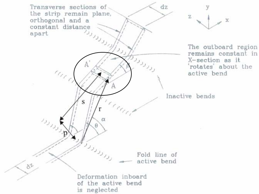
Figure 2.6 Small element investigated under different deformation types [13]
