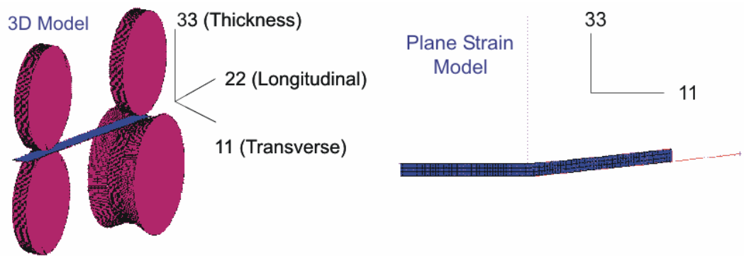
Figure 3.23 Directions of the tensorial notation
