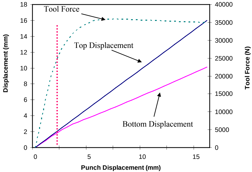
Figure 5.18 Deflection of upper and lower parts of MI-90
