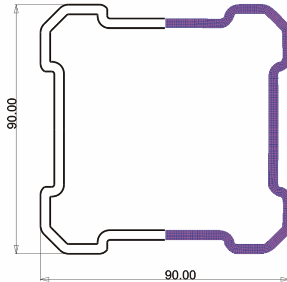
Figure 5.29 Overall geometry comparison
