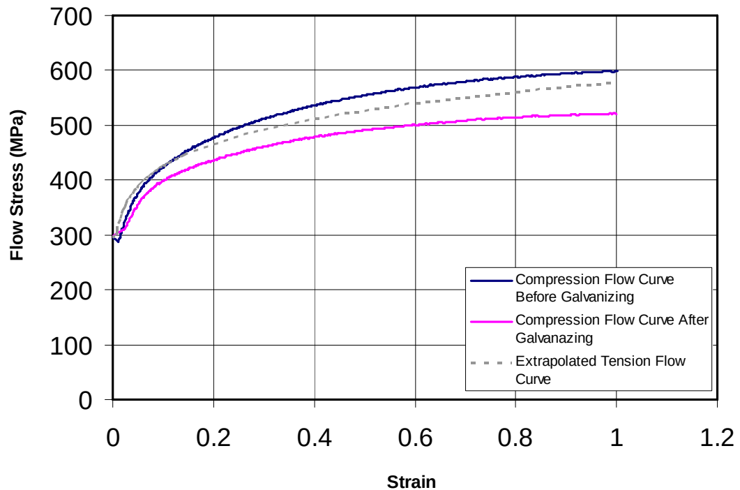
Figure 5.3 Compression test results and tension test results extended with Ludwik Equation
