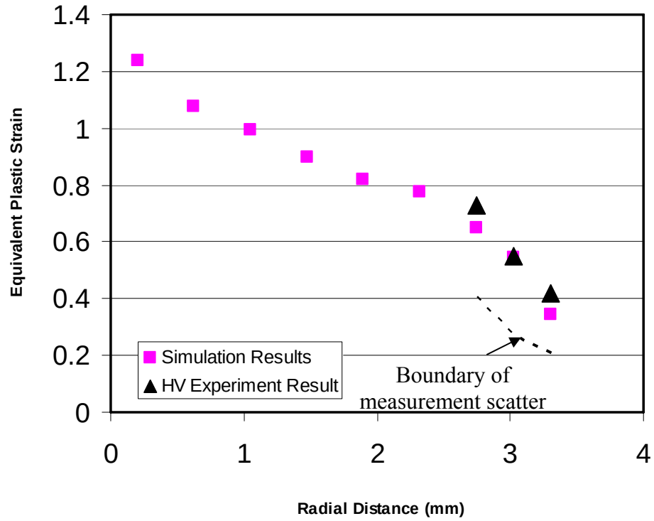
Figure 5.33 Strain distributions obtained from the new forming simulations and HV measurements for the Type-2 90° bend
