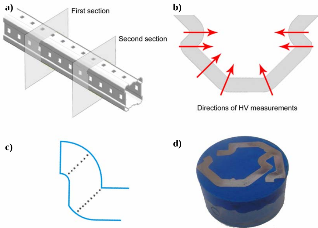
Figure 5.4 HV measurement locations: a) Two sections, b) Directions of the measurements, c) location of the measurements, d) HV Test specimen
