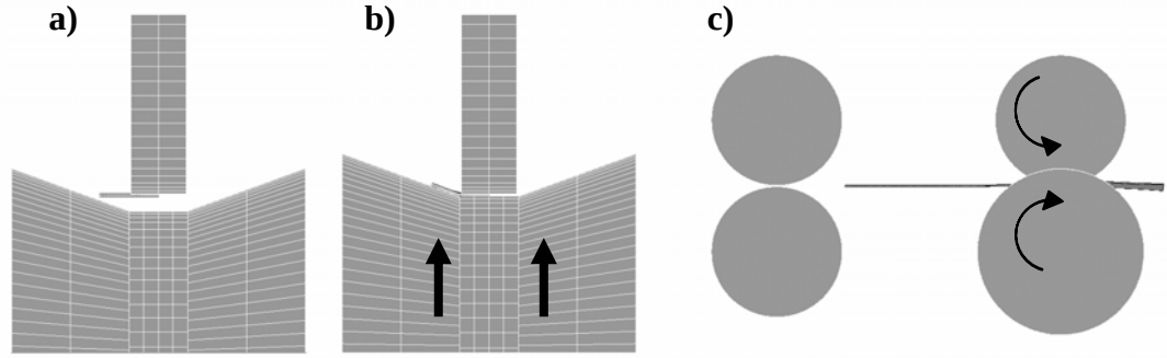
Figure 3.5 Forming sequence in computations
