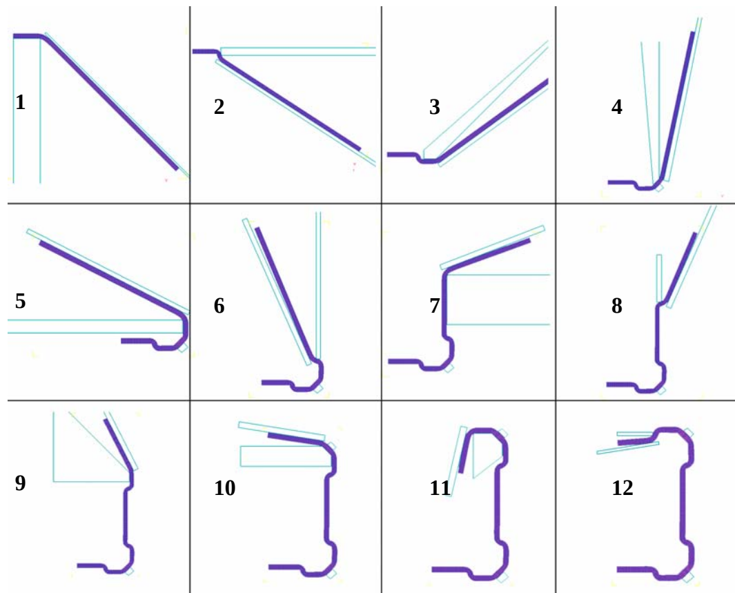
Figure 5.23 Forming sequence of the channel
