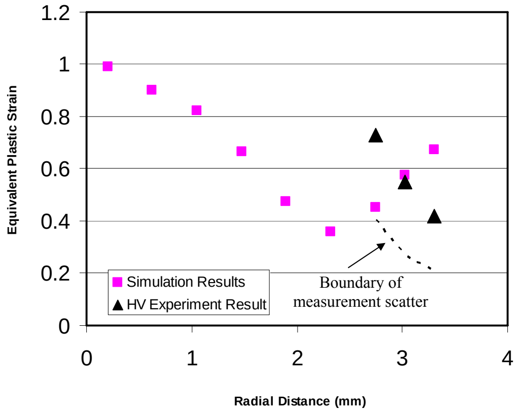
Figure 5.27 Strain distributions obtained from the simulations and HV measurements for the Type-2 90° bend
