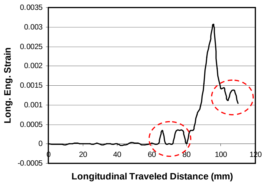
Figure 3.10 A sample longitudinal engineering strain curve
