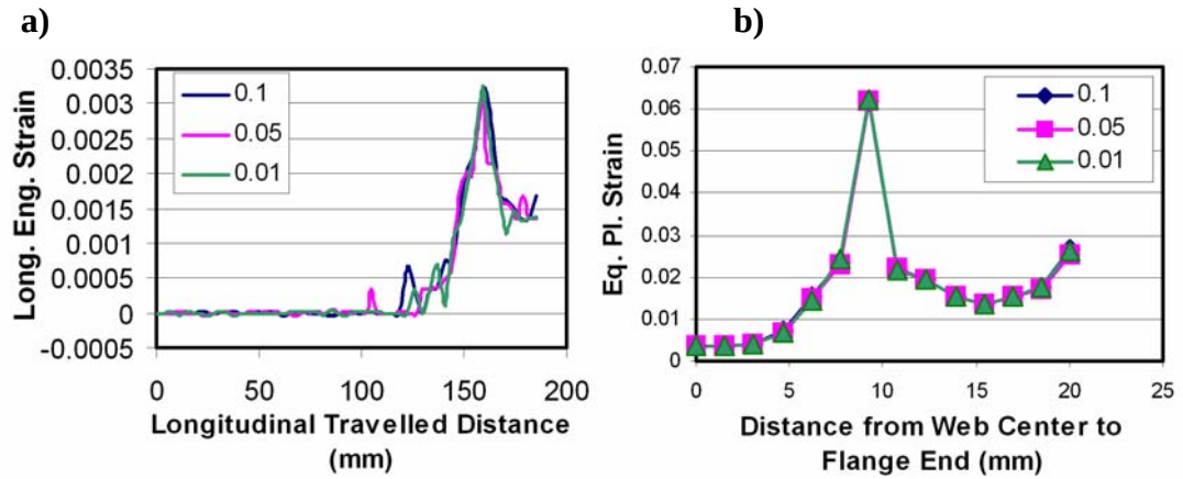
Figure A.1 Effect of convergence tolerances. a) Longitudinal engineering strain b) strain hardening on the sheet surface
