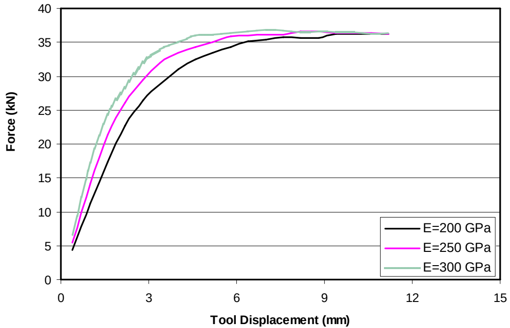
Figure 5.15 Elastic modulus effect
