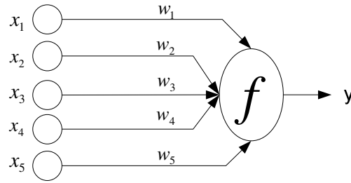
Figure 22 A Perceptron
