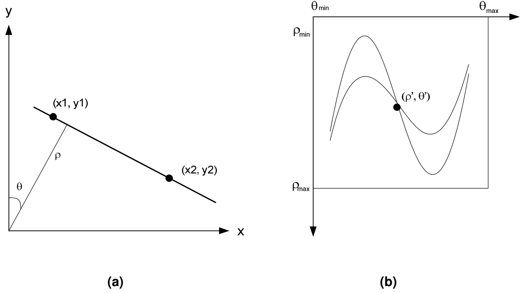
Figure 16 a) Normal representation of a line and (b) accumulator array in \rho - \theta parameter space
